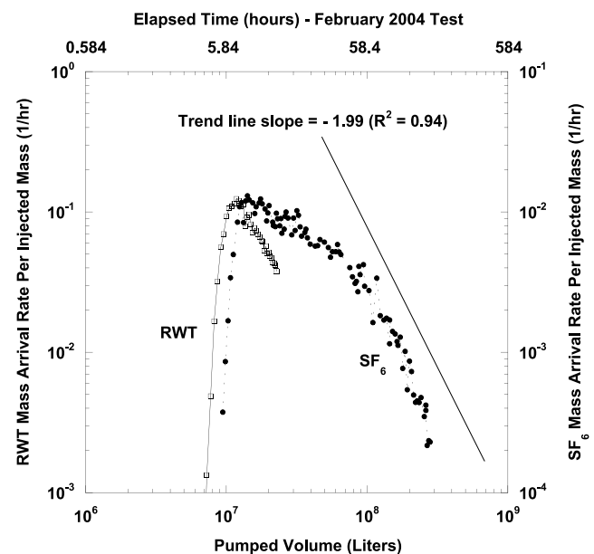
Figure 5. The logarithm of concentrations of RWT from the April 2003 tracer test [ Renken et al., 2008 ] and \text{SF}_6 from the February 2004 tracer test at the tracer recovery well, S-3164, plotted as a function of the logarithm of the pumped volume at the tracer recovery well.
