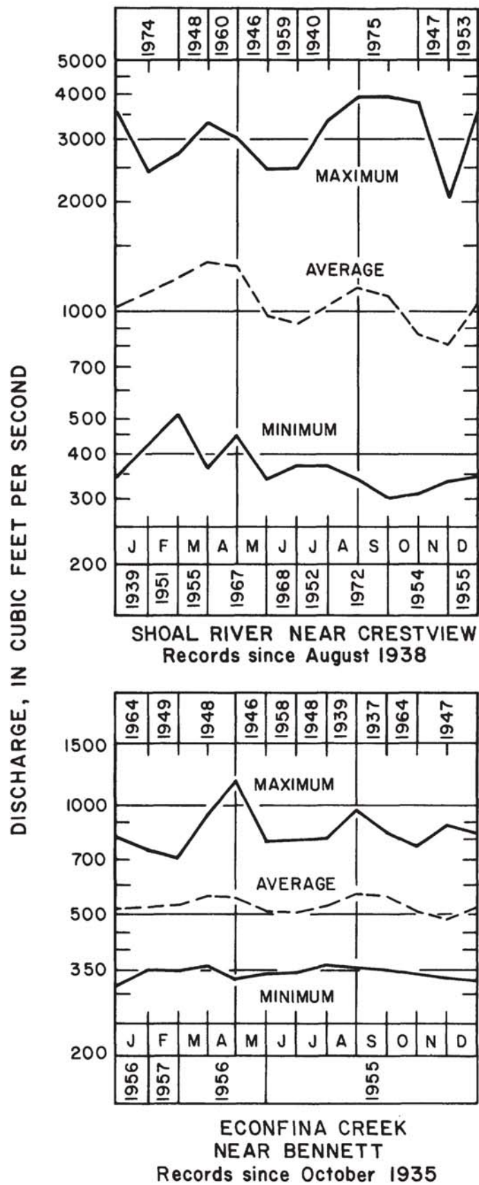
Figure 51.--Maximum, minimum, and average monthly mean discharge and years of extremes for Shoal River and Econfina Creek, Florida.
