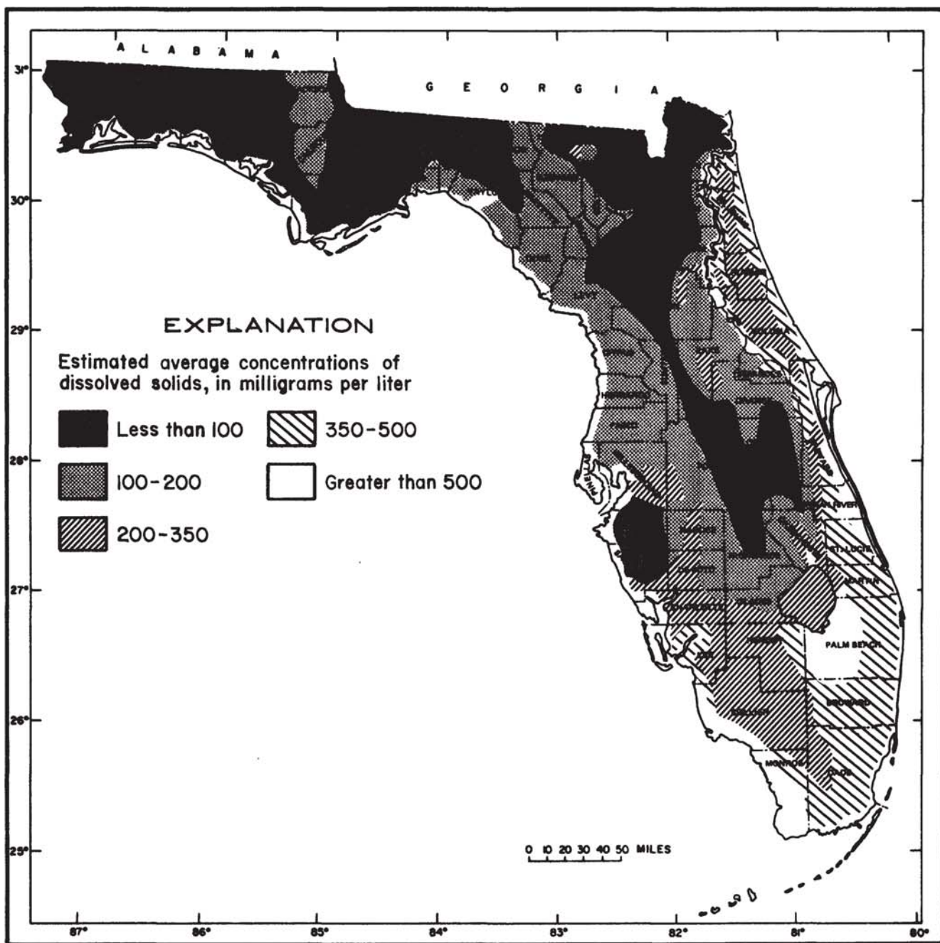
Figure 70.--Dissolved-solids concentrations in Florida surface waters (modified from Dysart and Goolsby, 1977).
