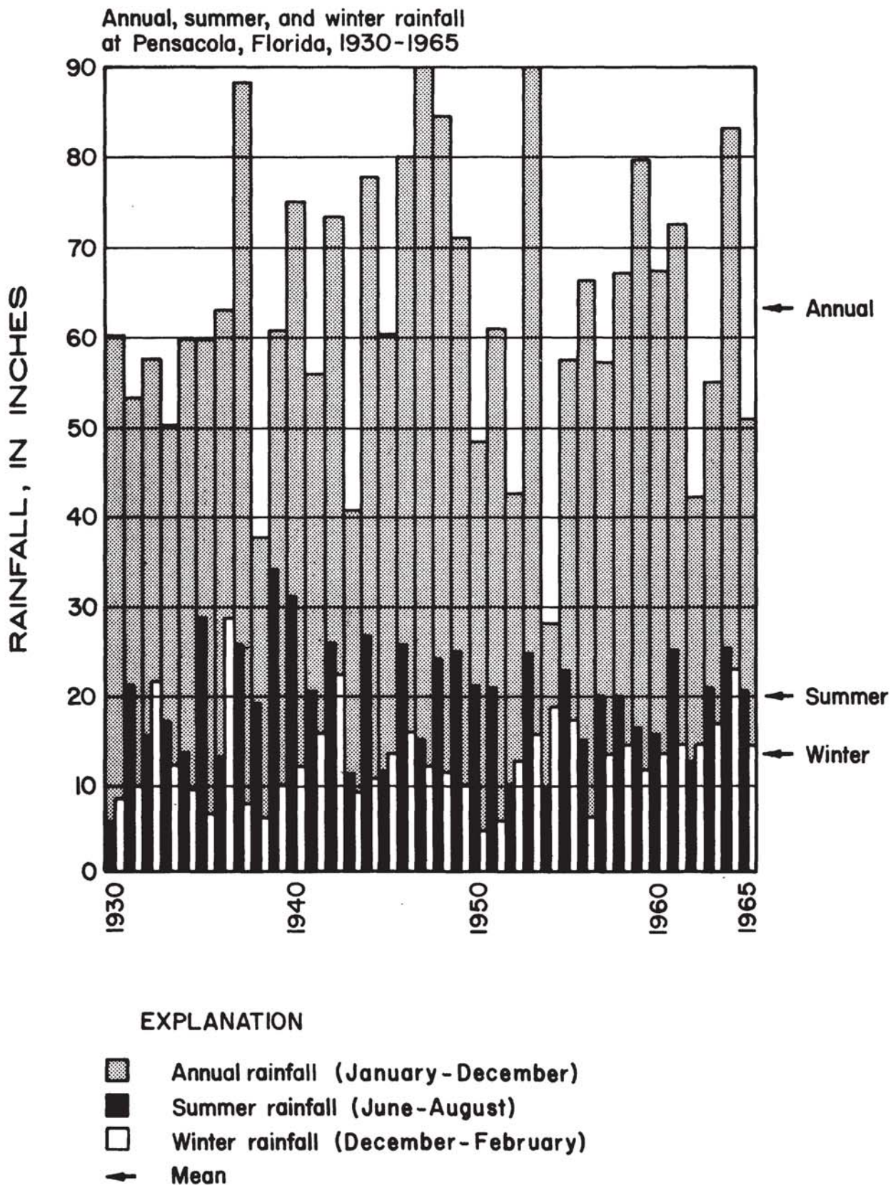
Figure 10.--Variation of rainfall during period 1930-65 at Pensacola, Florida (modified from Hughes and others, 1971).
