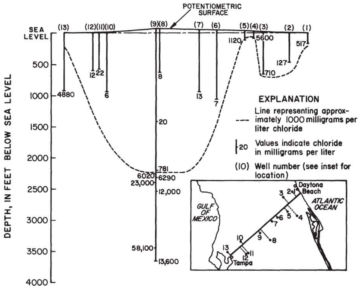
Figure 72.--Vertical distribution of chloride concentrations of water in wells across central Florida (modified from Shampine, 1965a).
