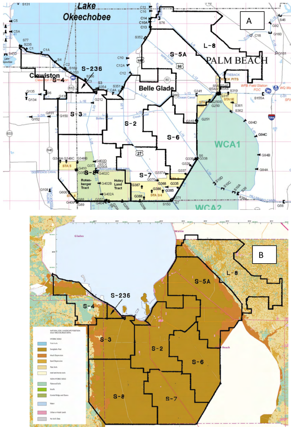
Figure C-4. A. Major sub-basins, canals, and structures in the EAA watershed.
