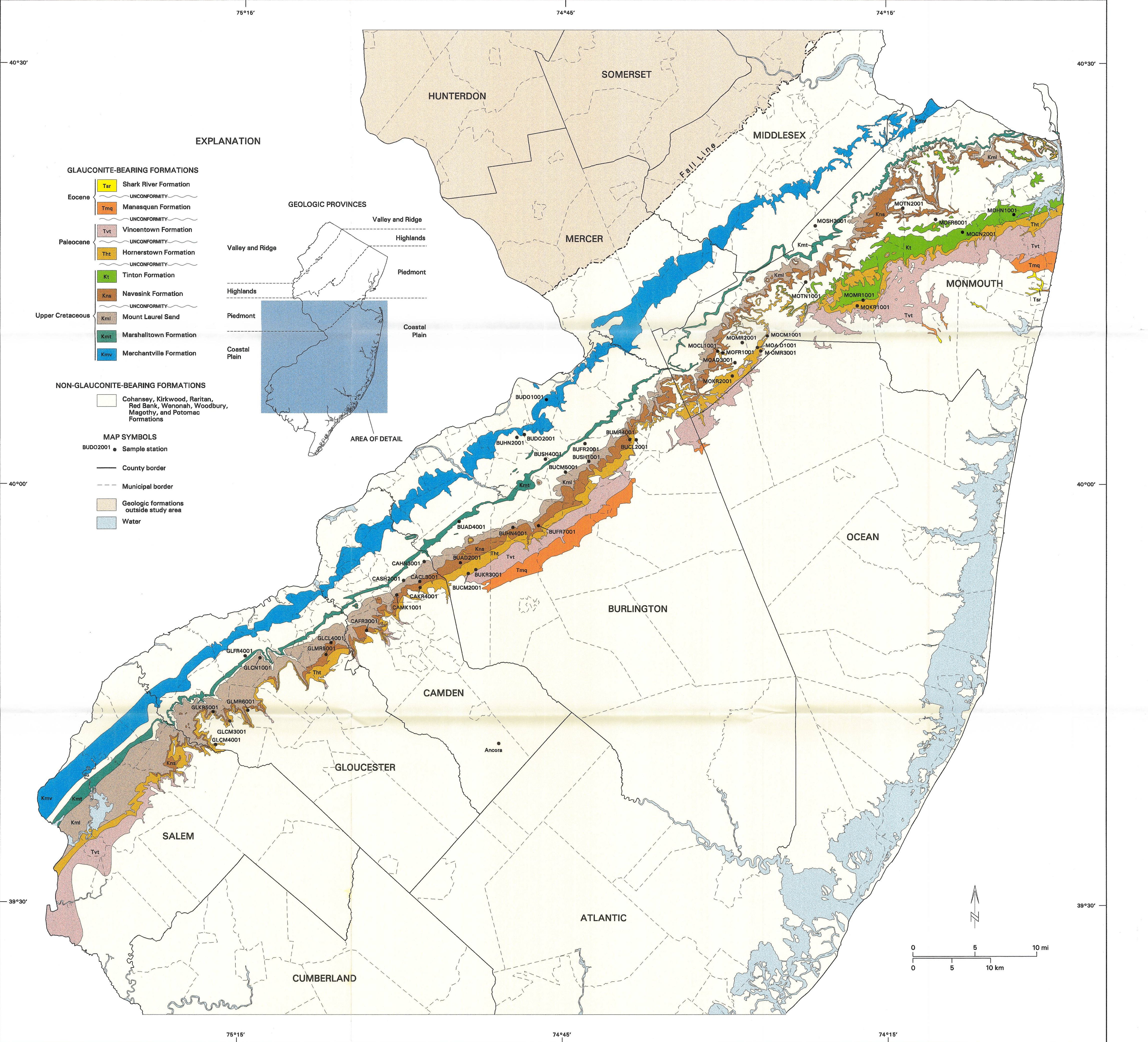
Figure 1. Geologic map showing the soil sampling stations and their relation to glauconite-bearing parent sediments in the New Jersey Coastal Plain physiographic province.
