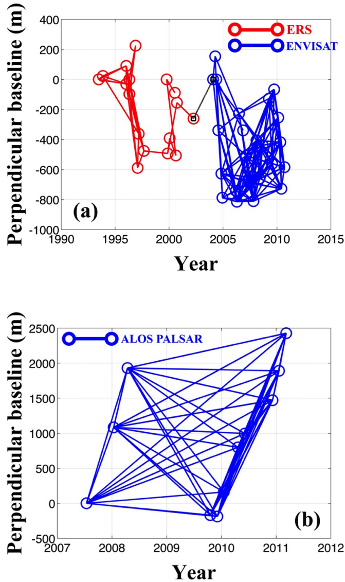
Figure 4.3. Diagram of a perpendicular baseline and InSAR pairs ((a) ERS and ENVISAT InSAR pairs; red circles and lines are ERS pairs, and blue circles and lines are ENVISAT pairs. Dotted black line represents simulated temporary InSAR pair to fill up data gap. (b) ALOS PALSAR InSAR pairs).
