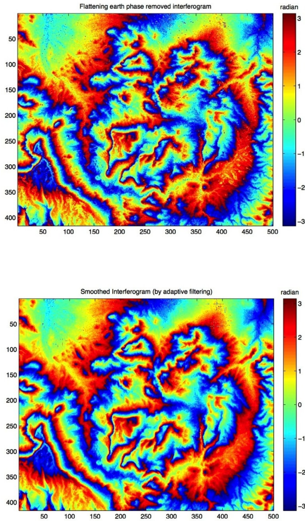
Figure 1.3. (Top) Wrapped interferogram before smoothing. (Bottom) Wrapped interferogram after smoothing. The smoothing was applied by Goldstein adaptive filtering.
