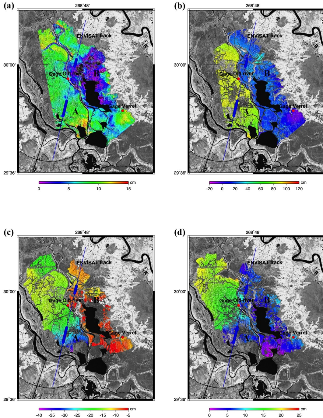
Figure 2.10. Maps of the absolute water level change over the swamp forest generated from the integration of ENVISAT altimetry with PALSAR L-band InSAR (a) Jun 28 2007 – Feb 13 2008 (b) Feb 13 2008 – Mar 30 2008, and Radarsat-1 C-band InSAR (c) Dec 31 2006 – Feb 17 2007 (d) Dec 26 2007 – Jan 19 2008. Blue line is the altimetry track and the blue dots indicate the data points used as the vertical reference. Red dots show the locations of water level gauges. Old river gauge is located in the river channel and Verret gauge is located within the swamp forest.
