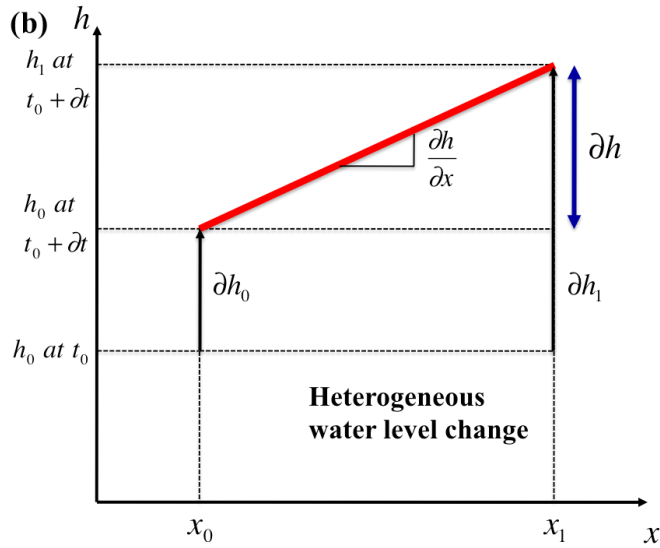
Figure 2.2. (a) Homogeneous water level change. x and h axes represent a spatial domain and the water level, respectively. During \partial t time interval at two points, x_0 and x_1 in the spatial domain, the water level increases constantly as much as \partial h (= h_1 - h_0) . (b) Heterogeneous water level change within swamp forests. During \partial t time interval, the water level at point x_0 increases by dh_0 , and the water level at point x_1 increases by dh_1 . The difference dh_1 - dh_0 is denoted as \partial h .
