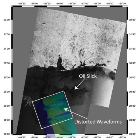
Figure 1.11. Oil slick detected by ALOS PALSAR ScanSAR image, and the oil slick looks darker than other oil-free ocean surfaces.
