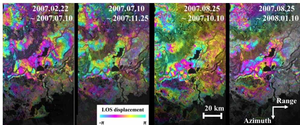
Figure 1.4. ALOS PALSAR ScanSAR-ScanSAR interferograms (in radar geometry) over Louisiana wetland.
