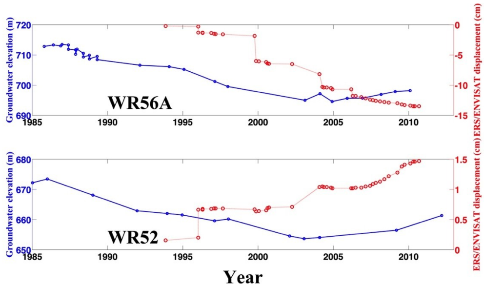
Figure 4.14. Time-series vertical deformation (red circles and lines) from ERS/ENVISAT SBAS processing and groundwater elevation (blue dots and lines) measured in WR56A and WR52.
