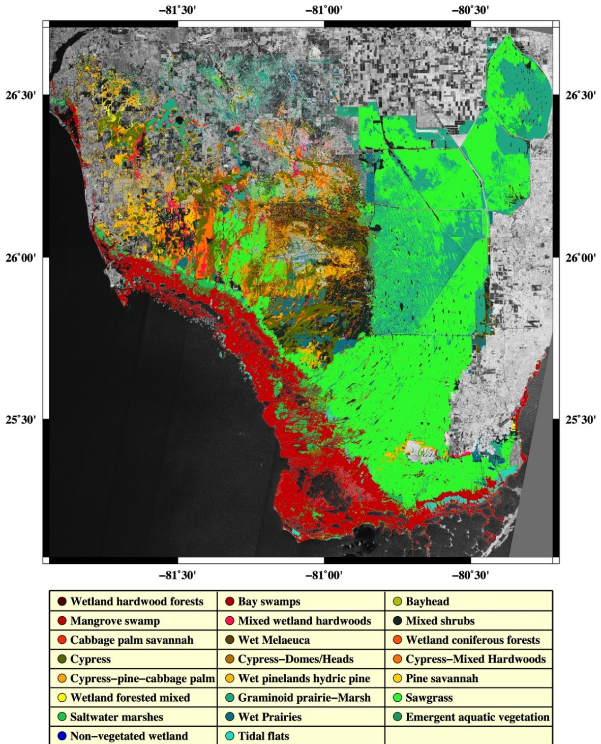
Figure 3.2. Land classification map in the wetlands of the Everglades, Florida. Each colored region represents vegetation types and the classification map includes inland and coastal marshes, and swamp forests. Background gray image is an intensity data from ALOS PALSAR ScanSAR mode.
