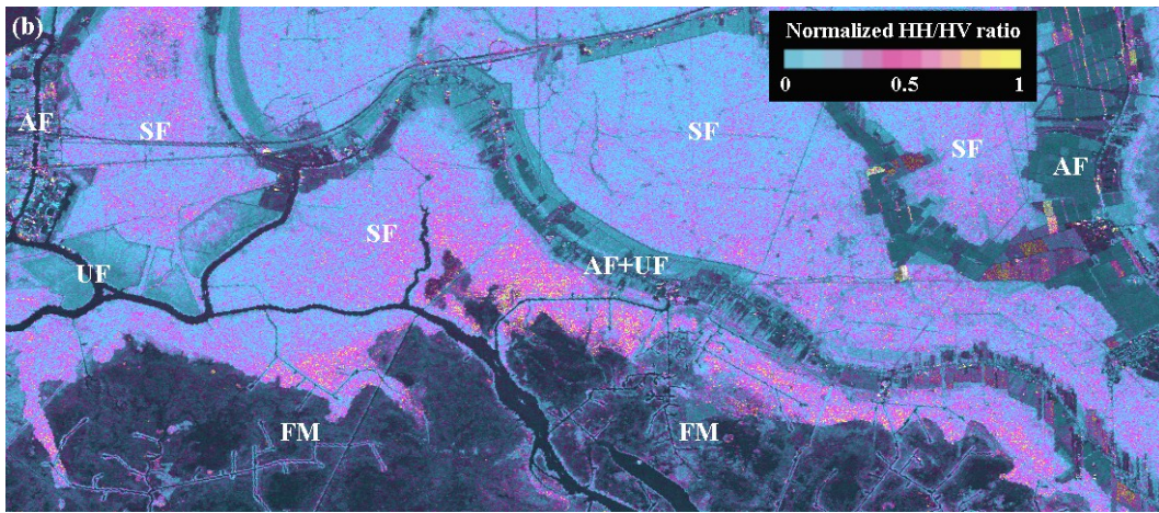
Figure 2.6. (a) Landsat ETM+ image (B: band 1, G: band 2, R: band 3, Aug 3 2001) over the area indicated by a blue box in Figure 2.1. (b) Normalized HH:HV ratio (PALSAR, Jun 30 2008); SF: Swamp forest, AF: Agricultural field, FM: Fresh marsh, UF: Upland forest.
