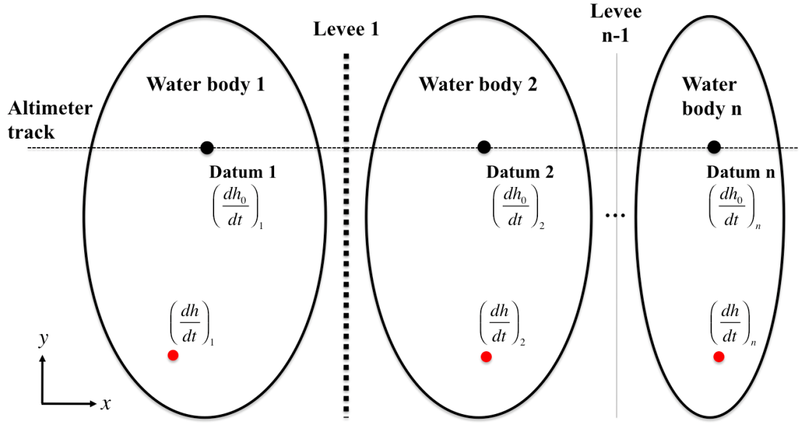
Figure 2.3. Schematic view of the Louisiana wetlands separated by several levees.
