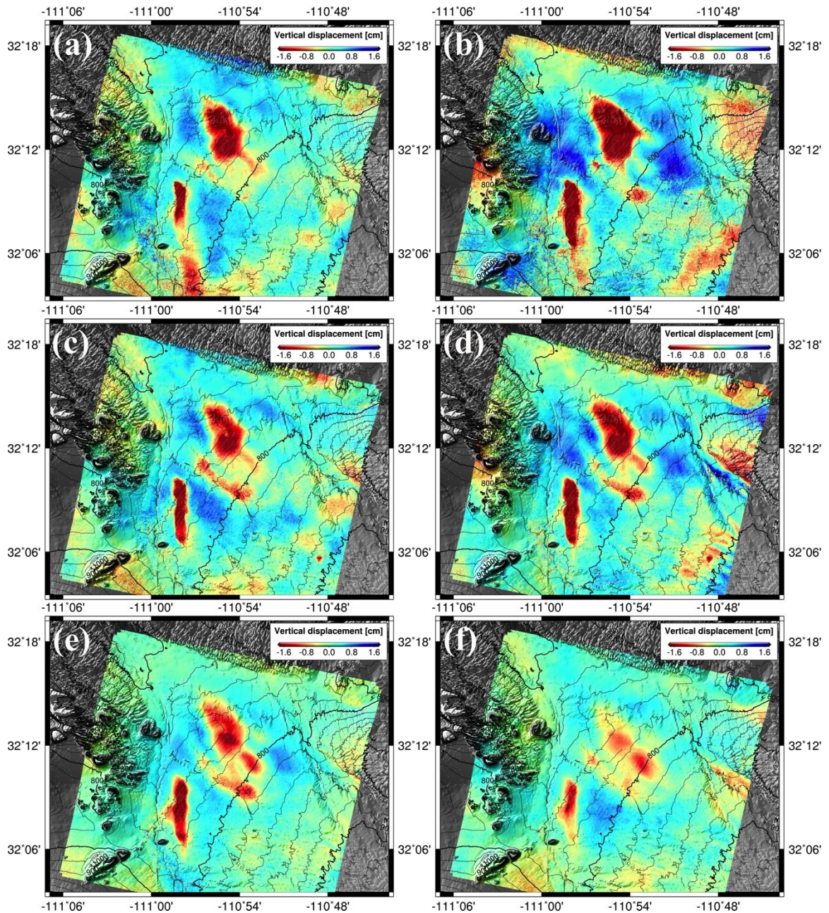
Figure 4.16. Three-year interval vertical deformation of (a) 1993.11.09 ~ 1996.11.22, (b) 1996.11.22 ~ 1999. 11. 12, (c) 1999.11.12 ~ 2002.04.05, (d) 2002.04.05 ~ 2004.12.10, (e) 2004.12.10 ~ 2007.10.26, and (f) 2007.10.26 ~ 2010.09.10.
