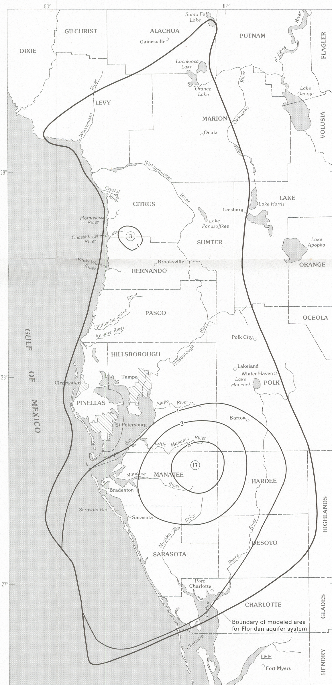
SIMULATED CHANGE IN 1976 POTENTIOMETRIC SURFACE AFTER SUPERIMPOSING WITHDRAWALS OF 30 MILLION GALLONS PER DAY, HERNANDO AND MANATEE COUNTIES
