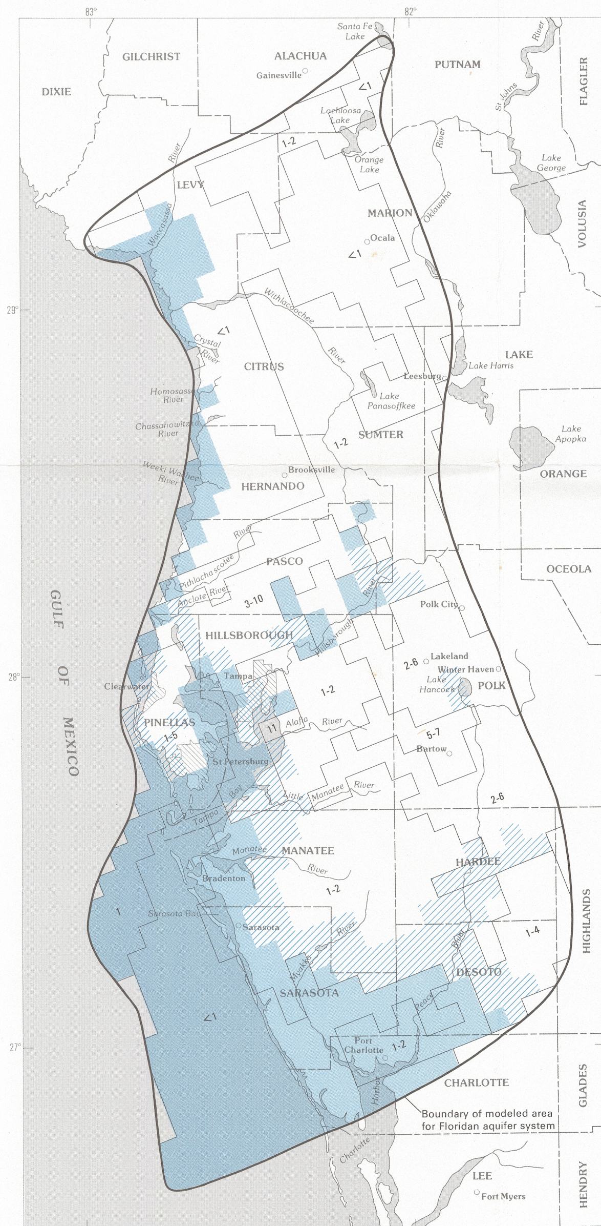
SIMULATED CHANGE IN RATES OF RECHARGE, PREDEVELOPMENT TO 1976
