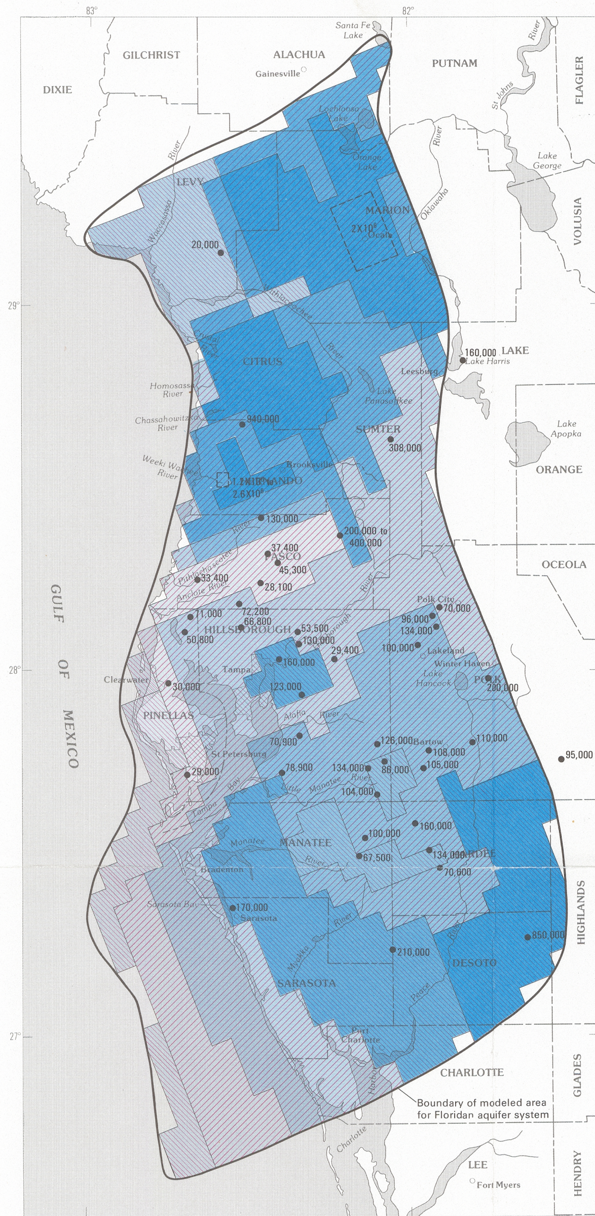
FIELD AND MODEL-DERIVED TRANSMISSIVITY
