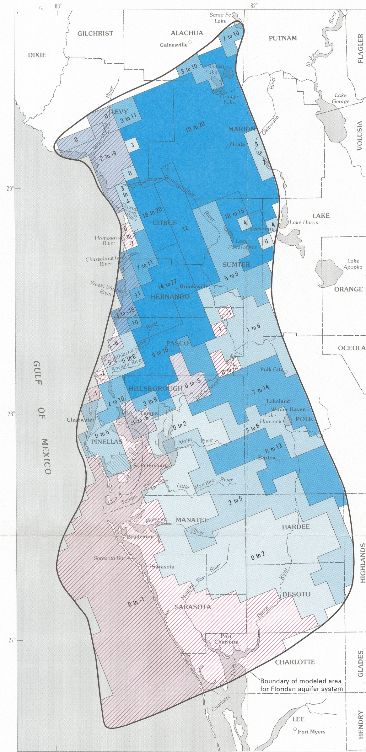
RECHARGE AND DISCHARGE IN THE CALIBRATED MODEL, EXCLUDING SPRINGFLOW, 1976
