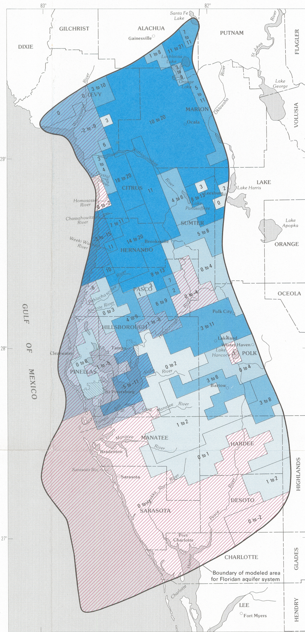
PREDEVELOPMENT RECHARGE AND DISCHARGE IN THE CALIBRATED MODEL, EXCLUDING SPRINGFLOW
