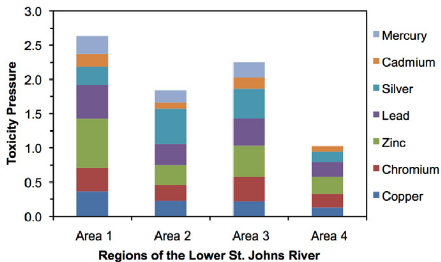
Figure 5.10 Toxicity pressure of metals in sediments from 2000-2007 in the four areas of the LSJR. Area 1 – western tributaries; Area 2 – north arm; Area 3 – north main stem; Area 4 – south main stem. Note no mercury data were available from 2000-2007 in Area 4. See text in Section 5.2 for data sources.
