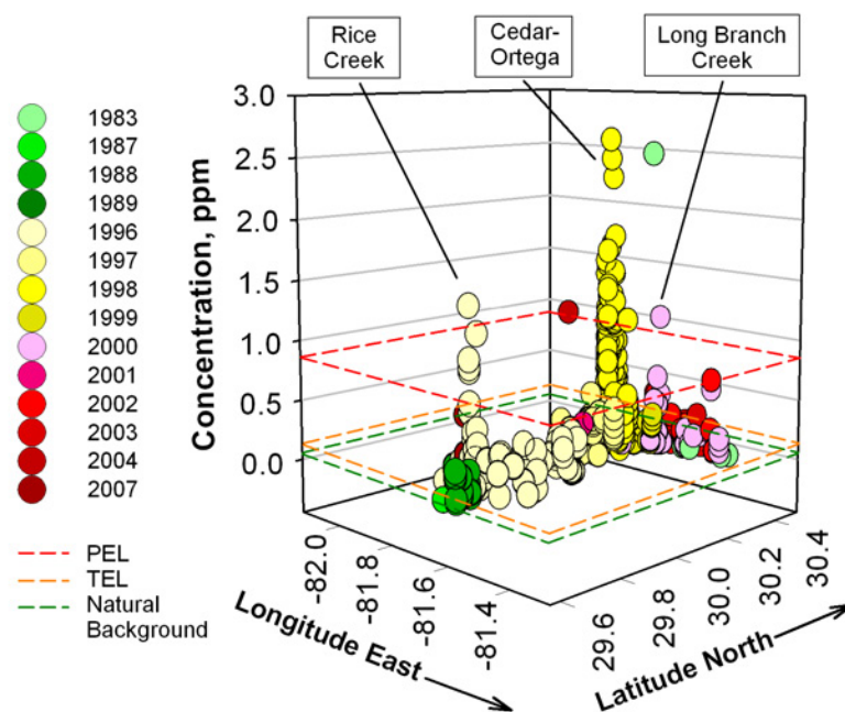
Figure 5.17 Mercury Sediment Quality Guidelines and LSJR sediment hot spots (scale of mercury concentrations does not show Rice Creek 2007 maxima). See text in Section 5.2 for data sources.
