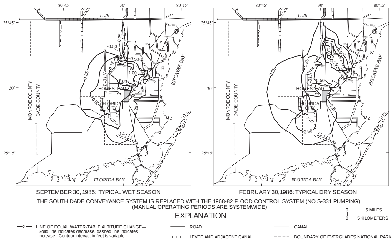
Figure 47. The change in the altitude of the computed water table at selected times when the post-1983 South Dade Conveyance System is replaced in the model with the 1968-82 flood-control system
