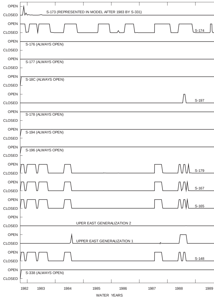
Figure 44. The simulated control-structure openings during water years 1983-89.
