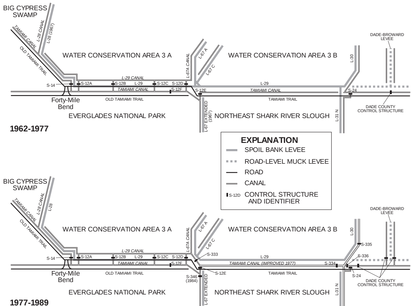
Figure 18. The system of surface-water control in the vicinity of the Tamiami Trail between Levee 28 and the Dade-Broward Levee, 1962-89 water years.
