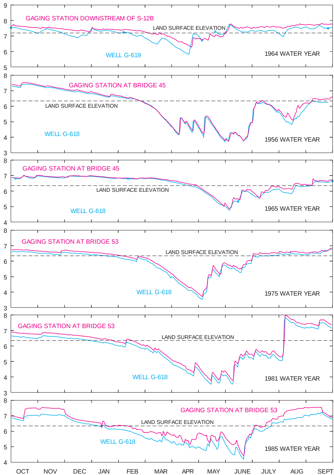
Figure 23. Canal stages and water levels in wells at selected sites in southern Dade County in selected water years.
