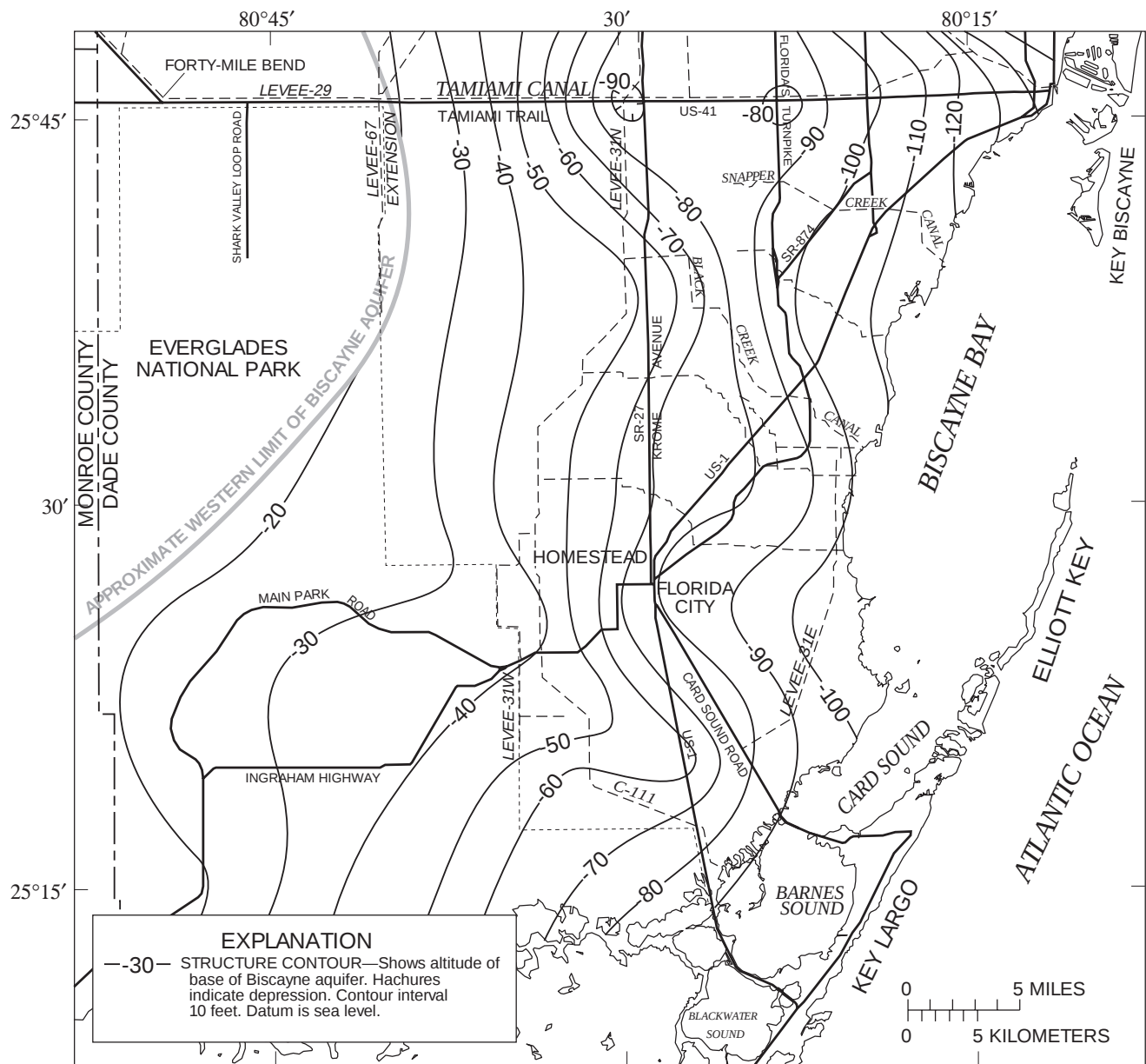
Figure 5. Configuration of the base of the Biscayne aquifer in southern Dade County.
