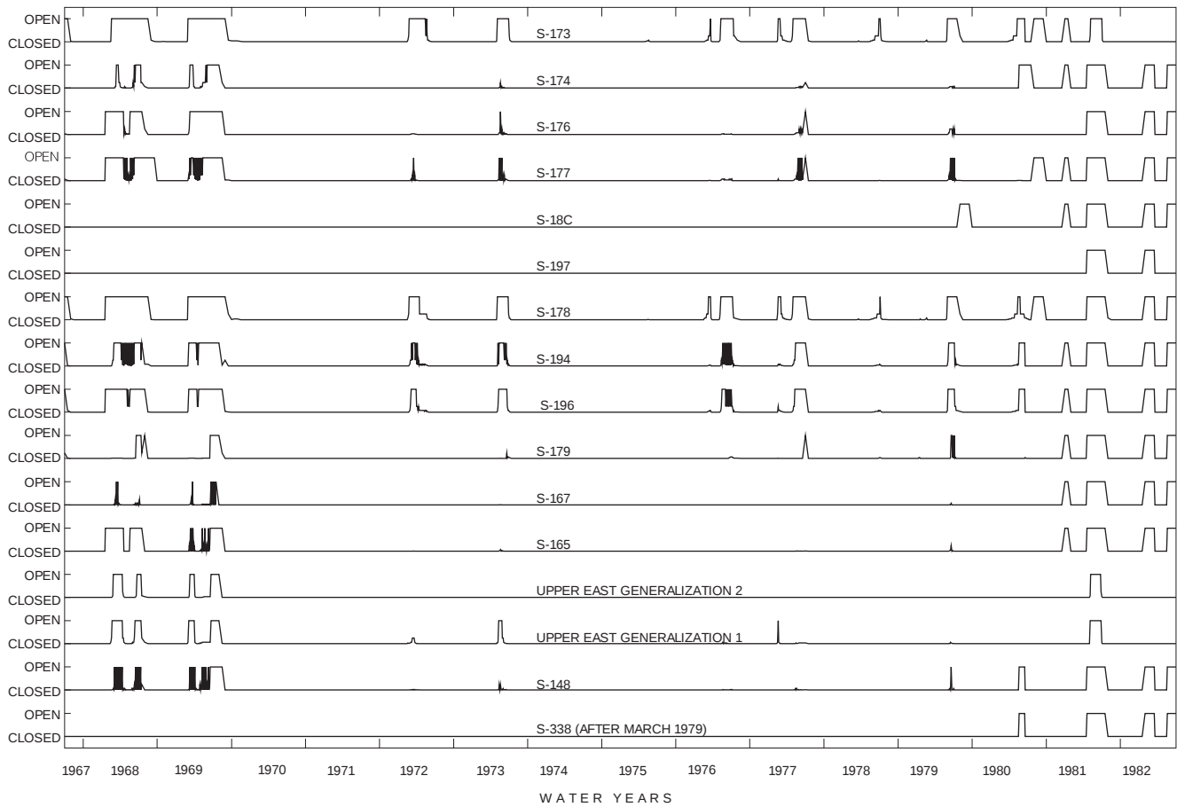
Figure 42. The simulated control-structure openings during water years 1968-82.
