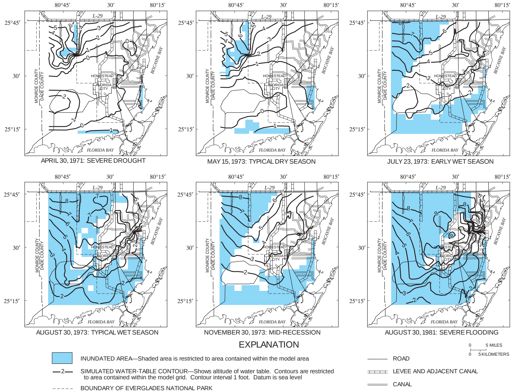
Figure 41. The water-table altitude and the area of inundation in the study area at selected times, as depicted by the calibrated model for water years 1968-82.
