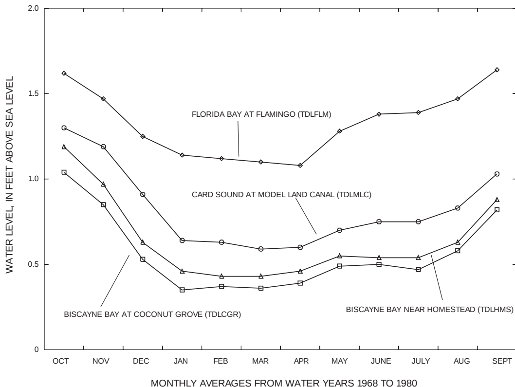
Figure 13. Long-term average monthly stages at tidal gaging stations in southern Dade County.
