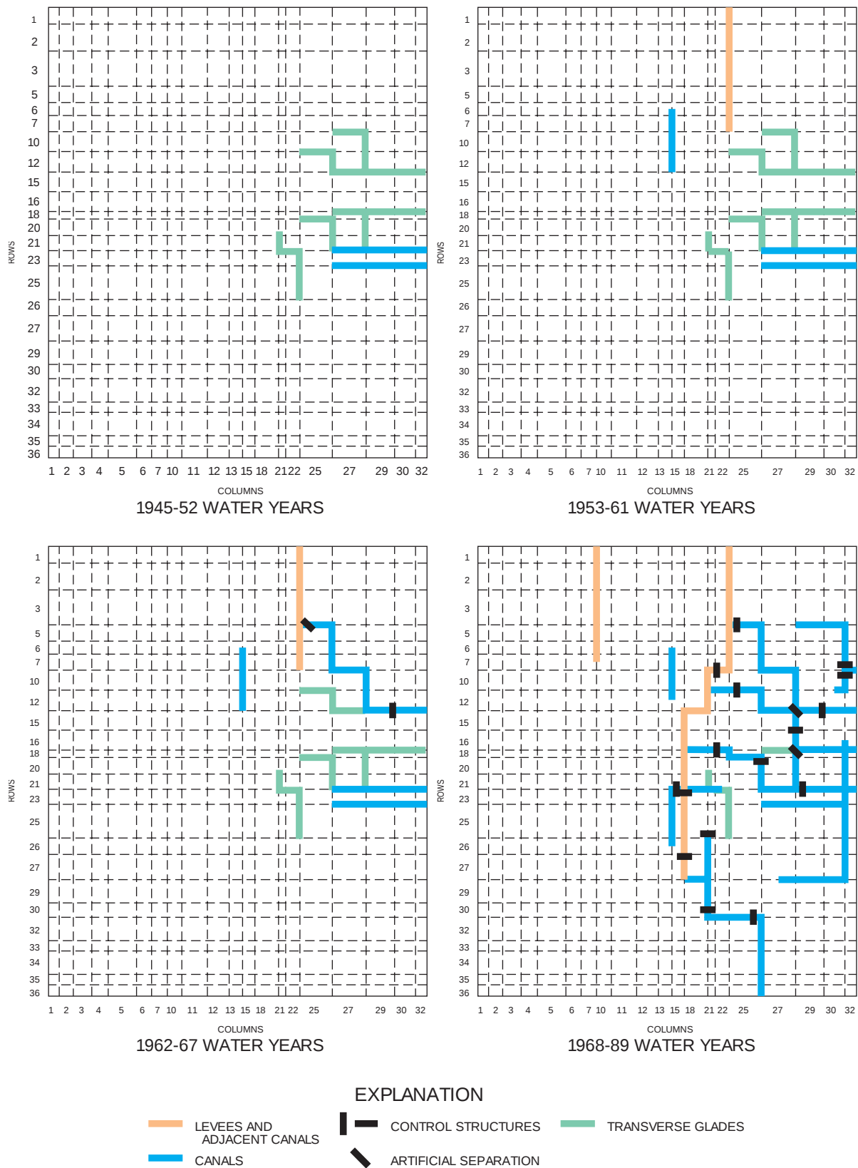
Figure 35. Model representation of transverse glades, canals, levees, and control structures in the successive water-management time periods.
