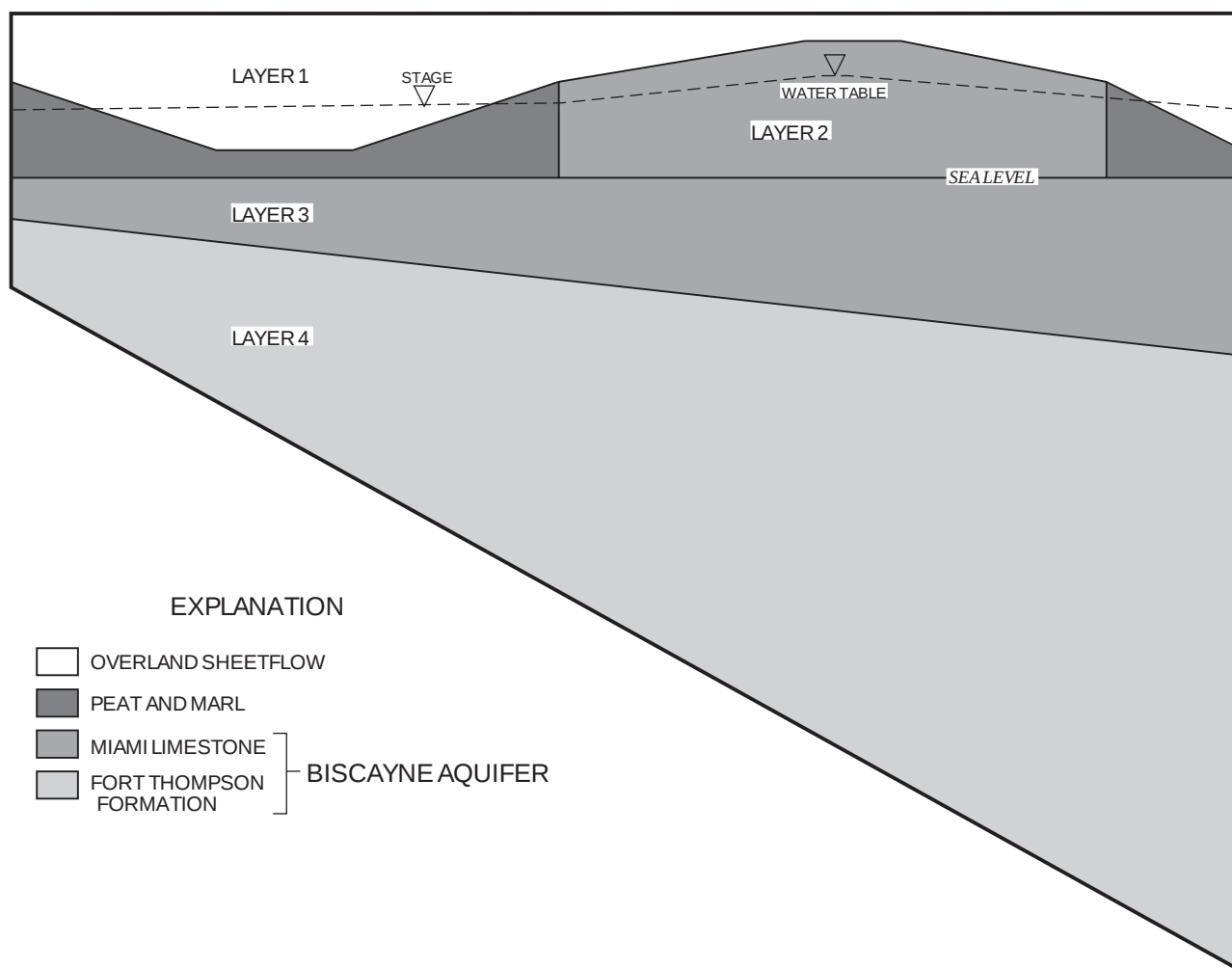
Figure 27. The vertical discretization of the model of flows in the Biscayne aquifer in southern Dade County.
