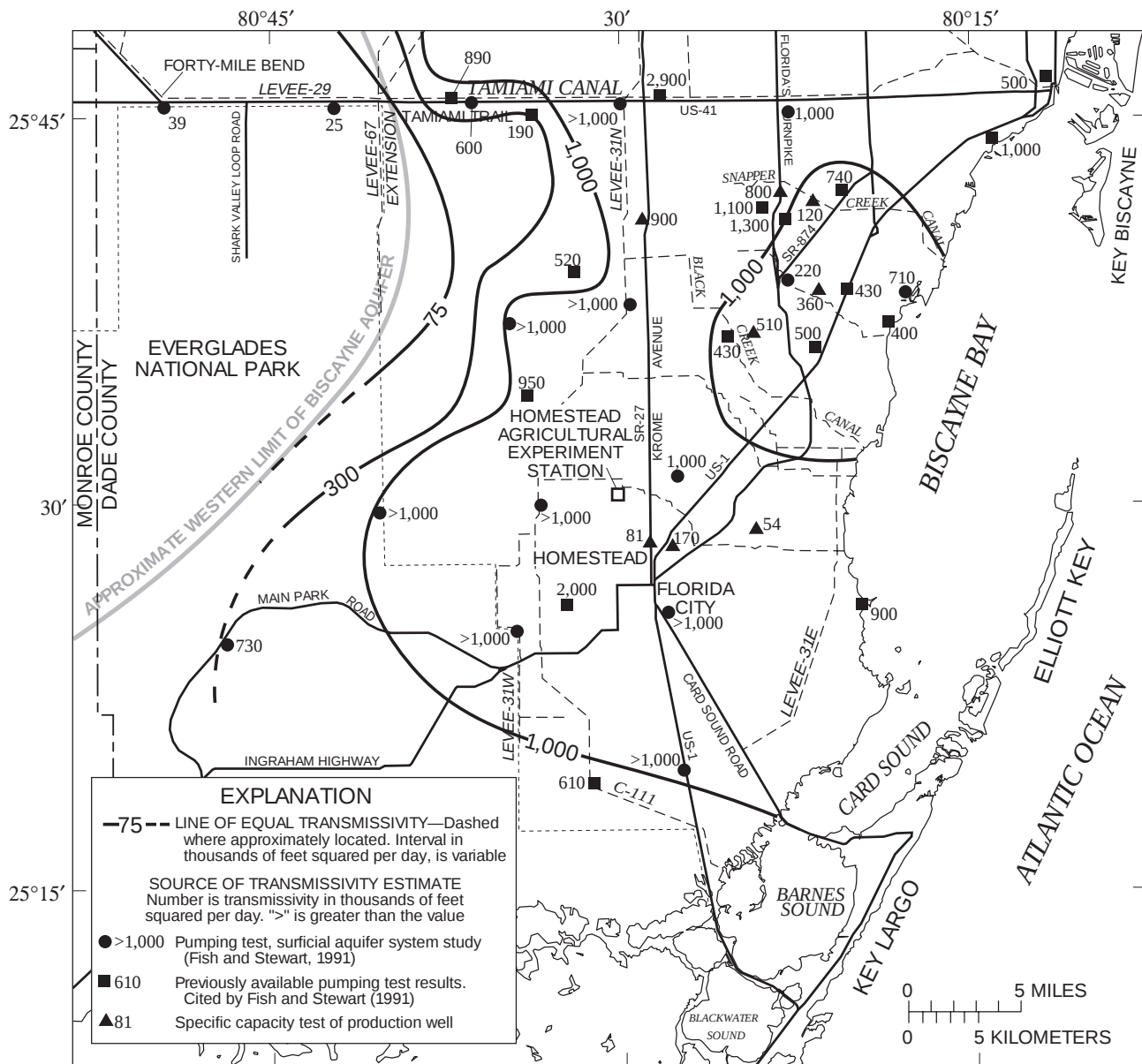
Figure 6. Generalized distribution of transmissivity of the Biscayne aquifer in southern Dade County.
