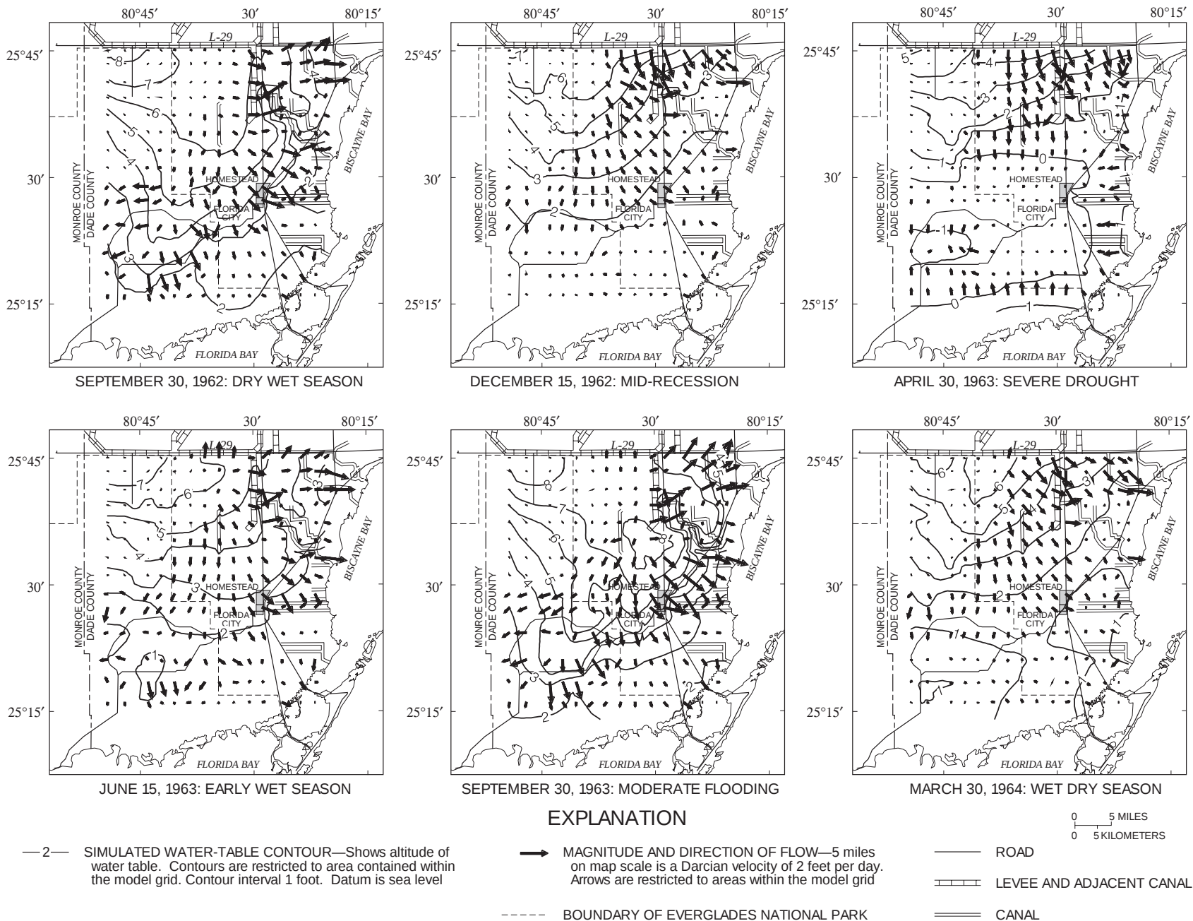
Figure 40. The magnitude and direction of flow in the Biscayne aquifer in the study area at selected times, as depicted by the calibrated model for water years 1962-67.
