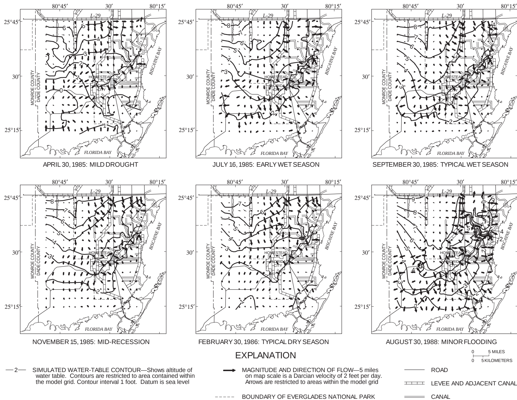
Figure 46. The magnitude and direction of flow in the Biscayne aquifer in the study area at selected times, as depicted by the calibrated model for water years 1983-89.
