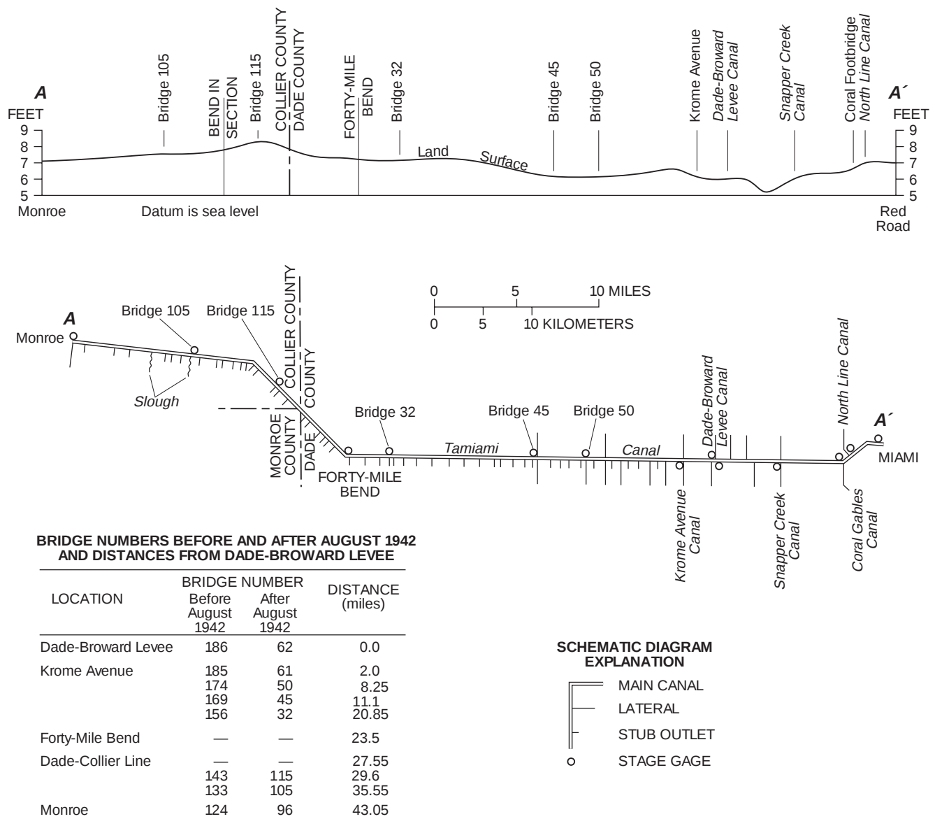
Figure 10. Tamiami Canal bridges, outlets, and gaging stations before 1962 and land-surface elevation along the canal.
