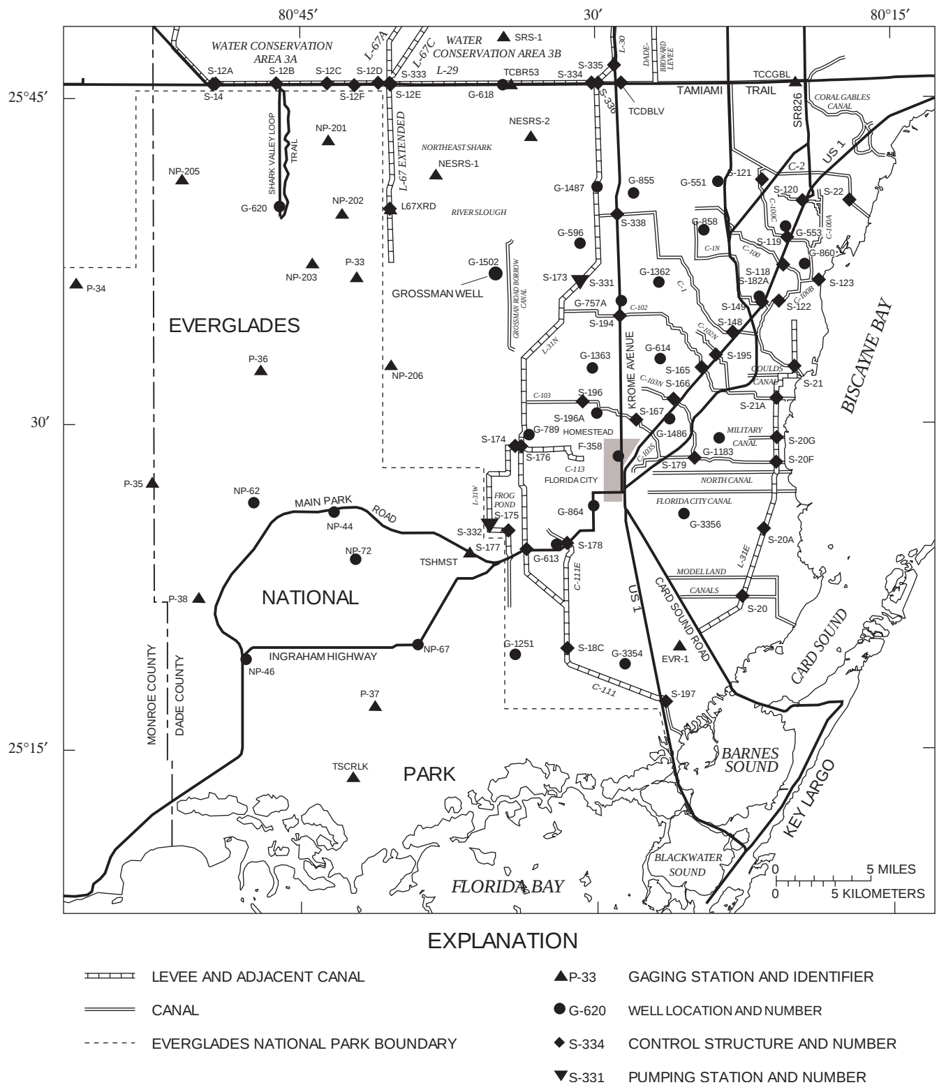
Figure 21. The canal-levee system in southern Dade County as it existed in water years 1983-89, and locations of wells and gaging stations providing continuous water-level and stage data during that period.
