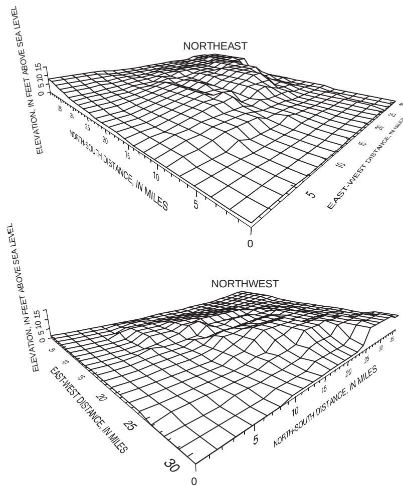
Figure 28. Three-dimensional representation of land surface in the modeled region.
