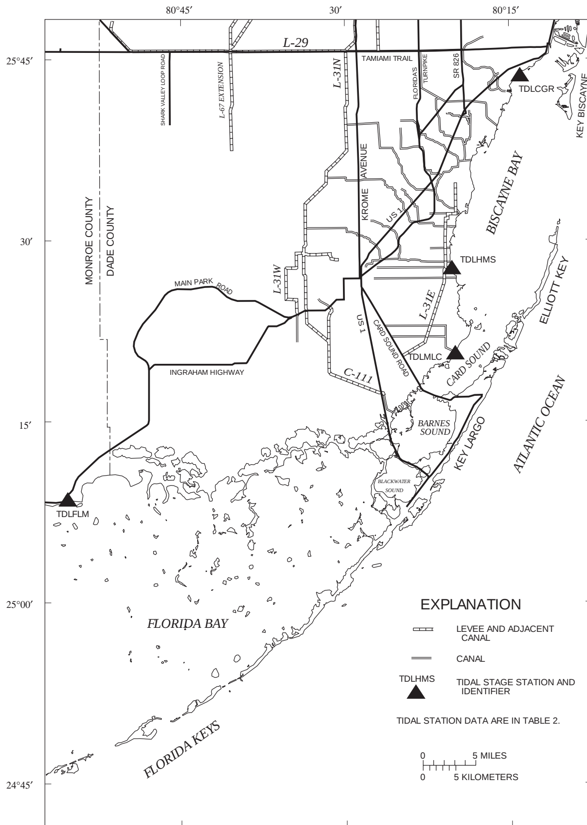
Figure 12. Locations of tidal gaging stations in southern Dade County used for model construction.
