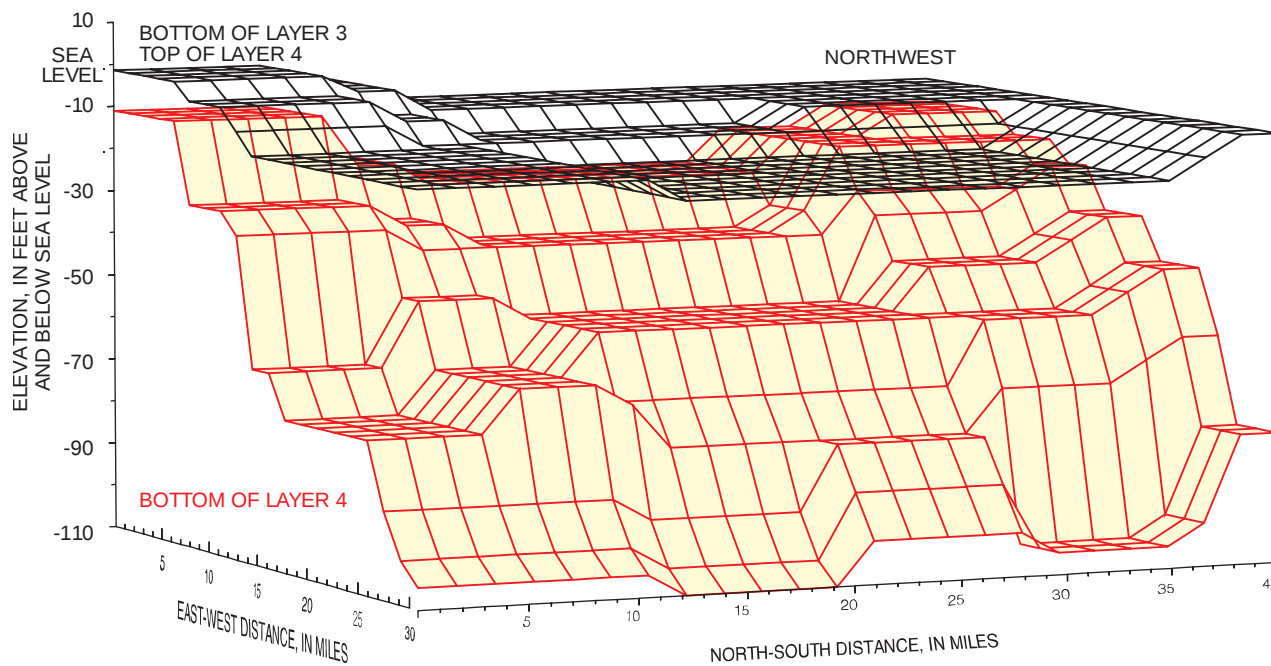
Figure 31. Three-dimensional representation of the bottoms of layers 3 and 4.
