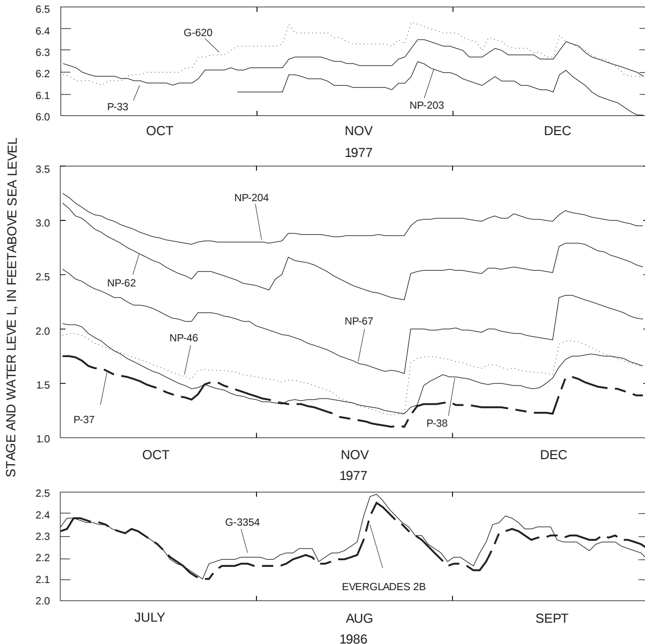
Figure 15. Ground-water levels and surface-water stages at selected pairs of wells and gaging stations in southern Dade County.
