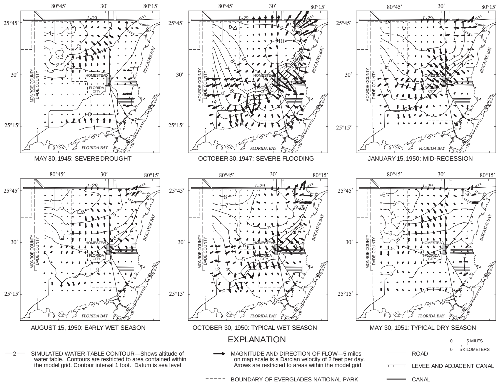
Figure 33. The magnitude and direction of flow in the Biscayne aquifer in the study area at selected times, as depicted by the calibrated model for water years 1945-52.
