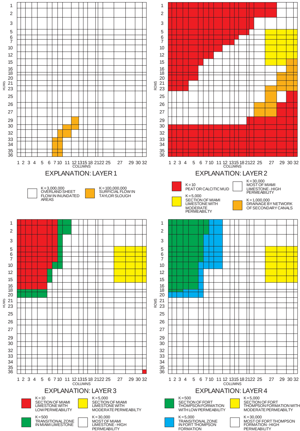
Figure 30. Distribution of assigned hydraulic conductivity values in each layer of the model.
