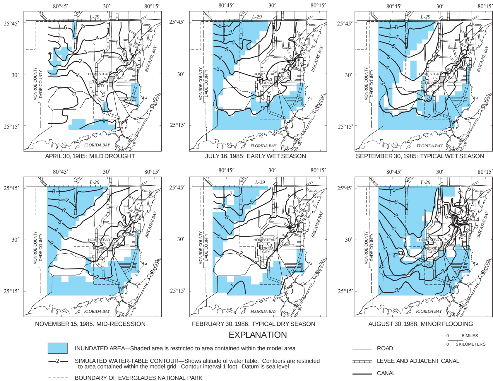
Figure 45. The water-table altitude and the area of inundation in the study area at selected times, as depicted by the calibrated model for water years 1983-89.
