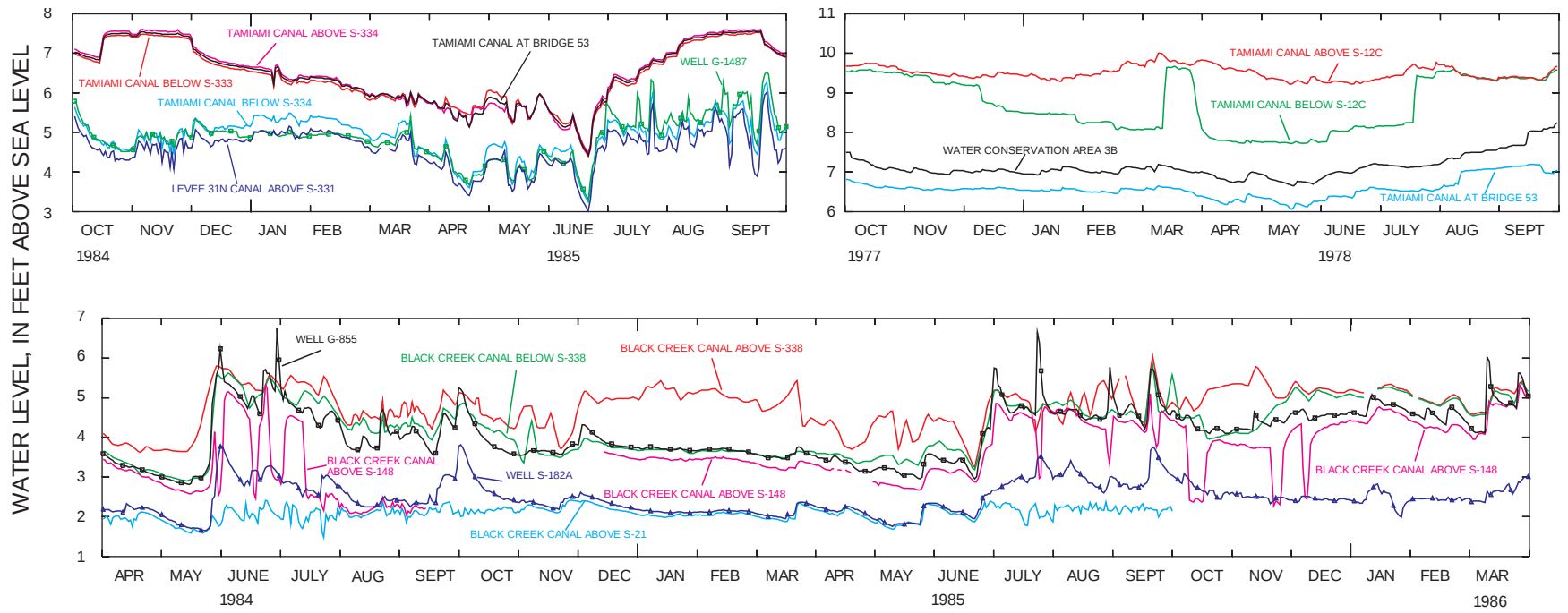
Figure 24. Surface-water stages upstream and downstream of selected canal control structures, upstream and downstream of Levee 29, and water levels in selected wells in selected water years.
