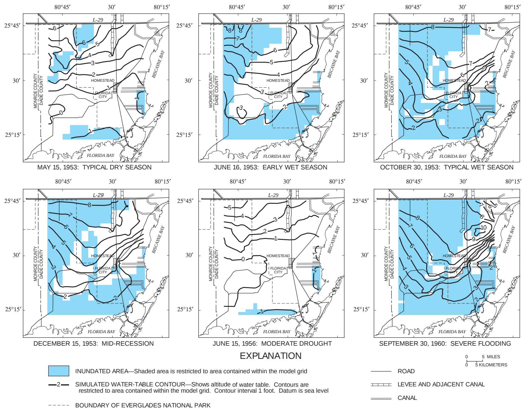
Figure 34. Map showing the water-table altitude and the area of inundation in the study area at selected times as depicted by the calibrated model for water years 1953-61.
