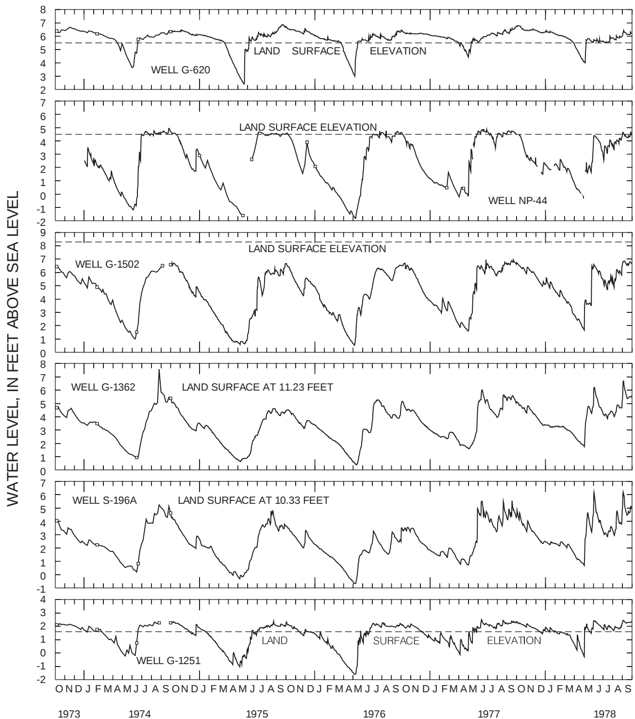
Figure 7. Water-level fluctuations in selected wells in southern Dade County for water years 1974-78.
