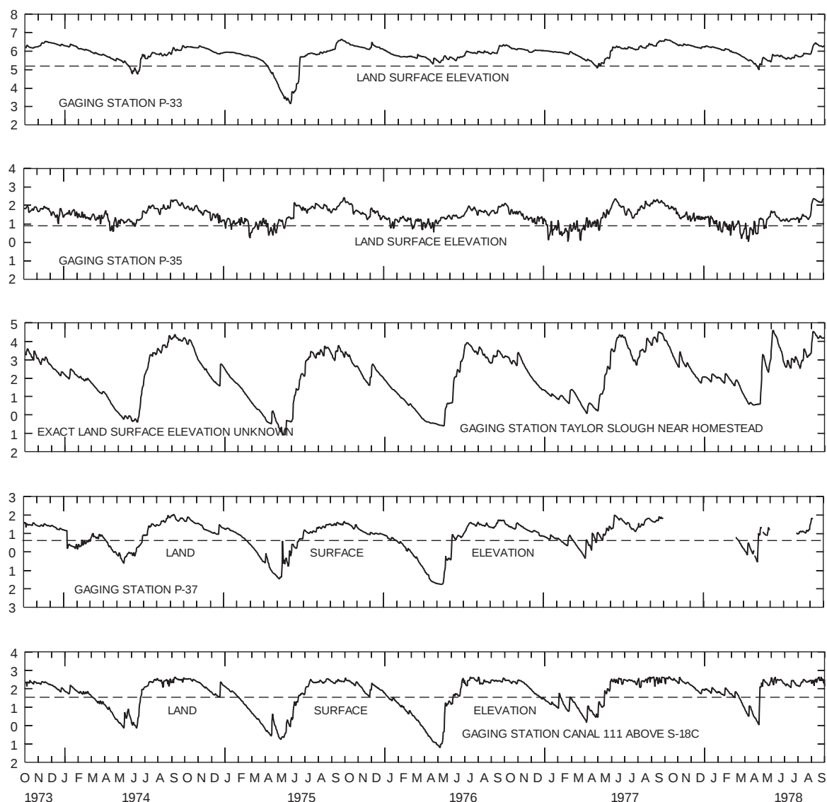
Figure 11. Stage fluctuations at selected gaging stations in southern Dade County for water years 1974-78.
