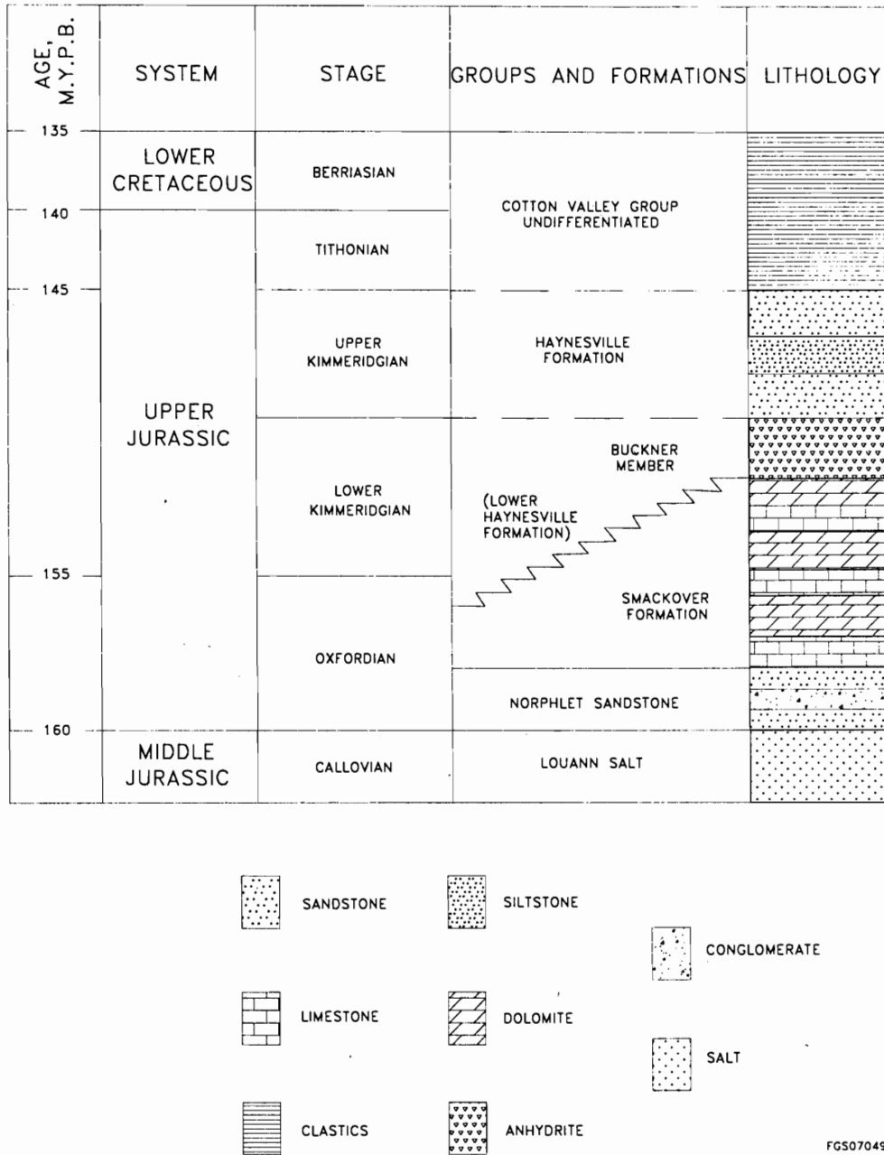
Figure 4. Stratigraphic nomenclature, Middle Jurassic to Lower Cretaceous, northwest Florida.
