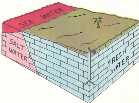
Fresh-salt water balance in a coastal area under natural conditions altered slightly by ground-water withdrawal.
