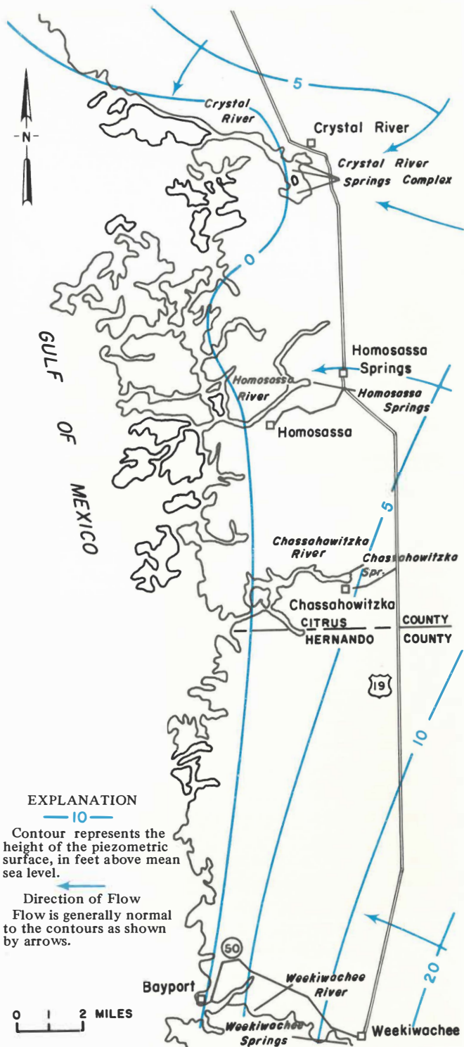
Figure 11. Piezometric surface of the Floridan aquifer, Sun Coast area, August-September 1965.
