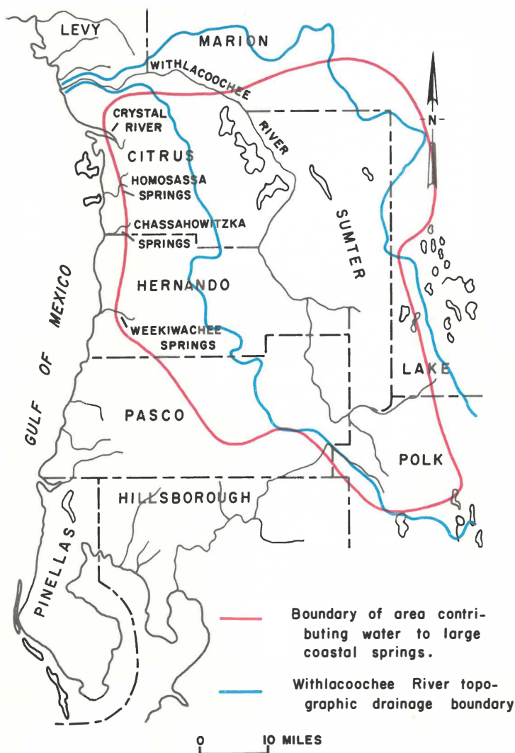
Figure 10. Water contributing area for large coastal springs and topographic drainage divide of the Withlacoochee River.
