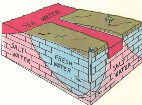
Fresh-salt water interface migrates farther inland as ground water withdrawals increase and canal is extended. Can cause saline contamination of a previously fresh supply.
