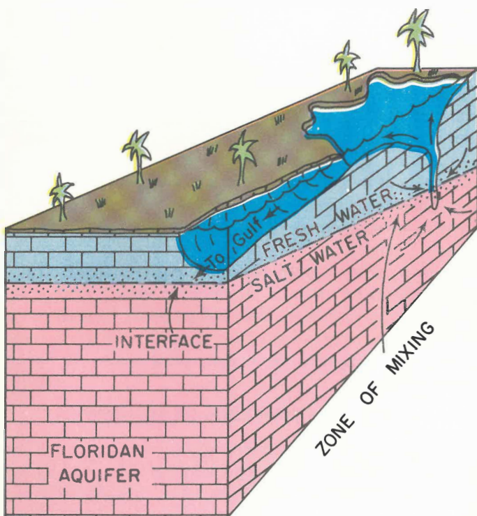
B. Low fresh-water levels.
