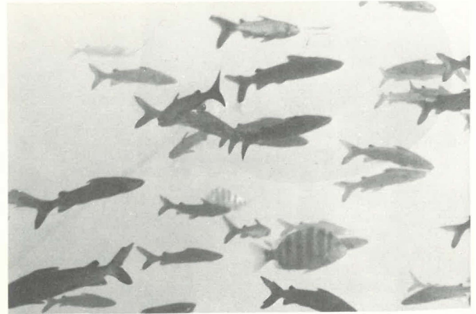
Figure 2. Thousands of fish of many kinds gather at "Nature's Giant Fishbowl"—Homosassa Springs. The vertically striped fish are sheepshead, a favorite of fishermen.
