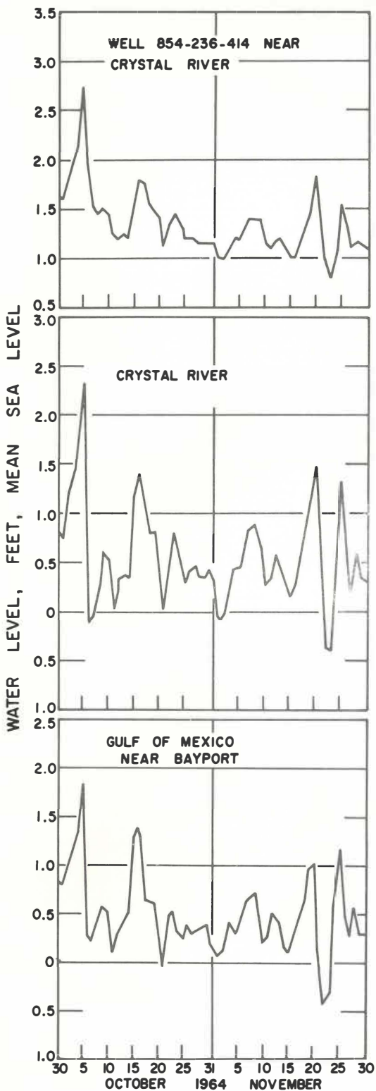
Figure 14. Comparison of water levels in the Floridan aquifer, Crystal River and the Gulf of Mexico.
