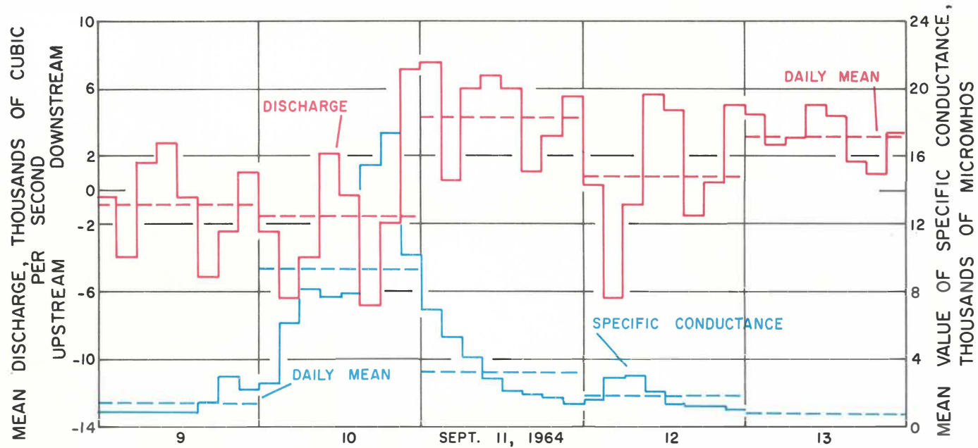
Figure 8. Variation in specific conductance and discharge for three-hour intervals at Crystal River near Crystal River, Florida, September 9-13, 1964.
