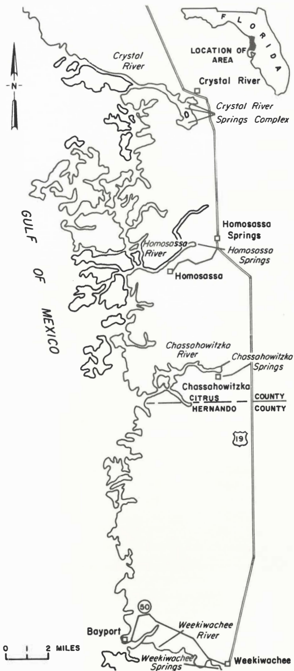
Figure 1. "Sun Coast" springs area of Florida.
