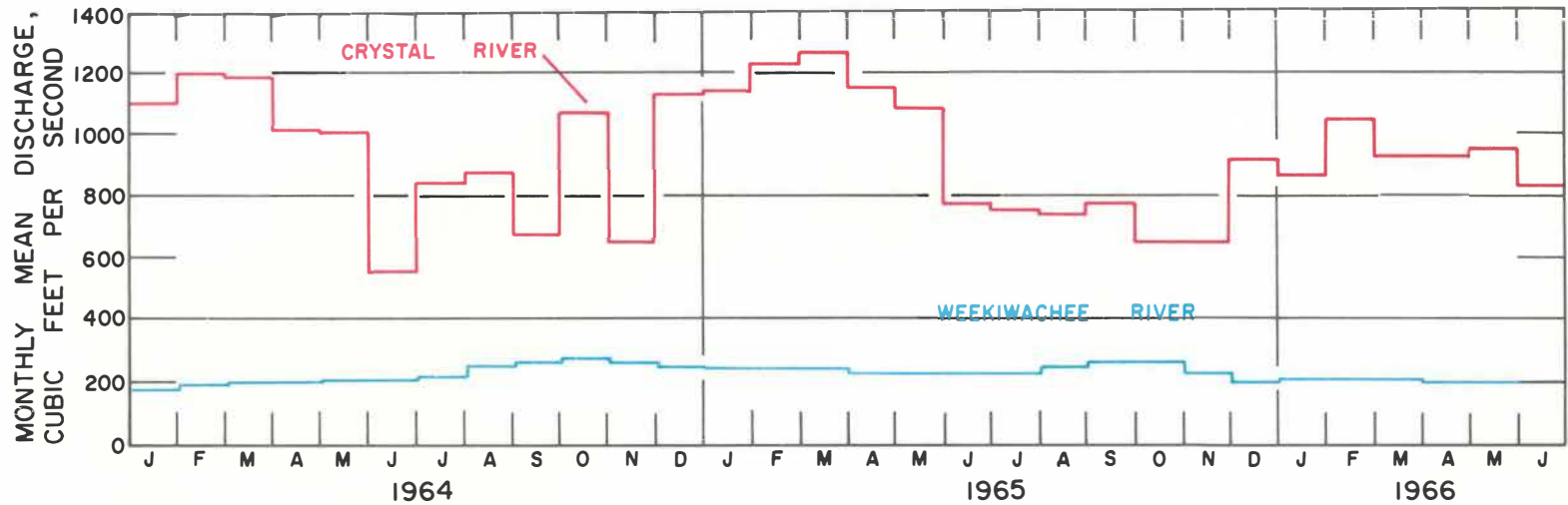
Figure 7. Monthly mean flow of Crystal River and Weekiwachee River, January 1964 - June 1966.
