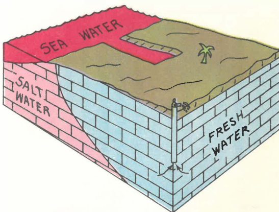
Inland migration of fresh-salt water interface as a result of construction of an uncontrolled tidal canal which allows increased discharge of fresh water from the aquifer and inland movement of salt water through the canal.
