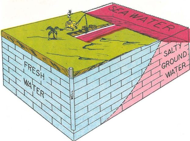
The construction of uncontrolled tidal canals causes sea-water intrusion in two ways: it lowers fresh-water levels, and it provides open channels to convey sea water inland. The salt front in the aquifer shifts inland adjacent to the new canal.
