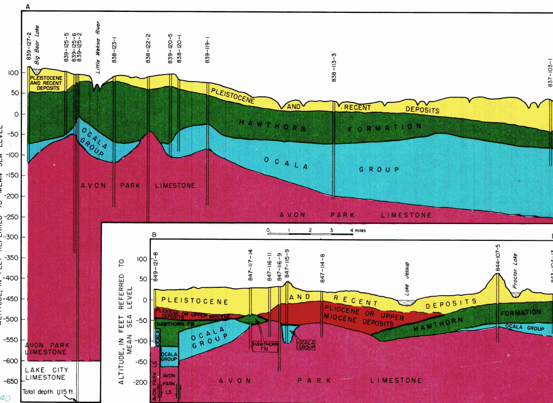
Geologic units penetrated by water wells.
