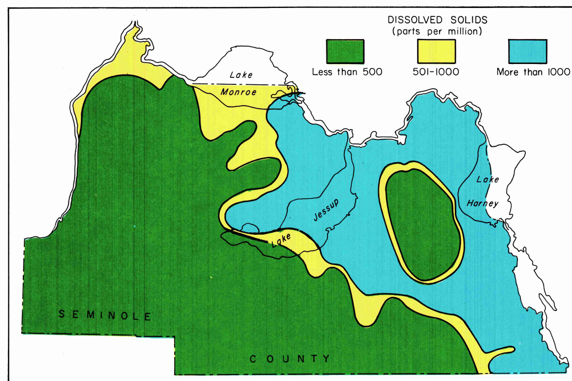
Dissolved-solids content of the water.
