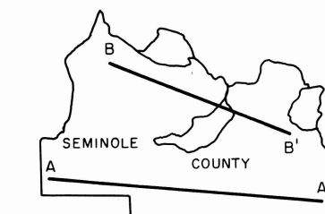
Location of geologic sections.
