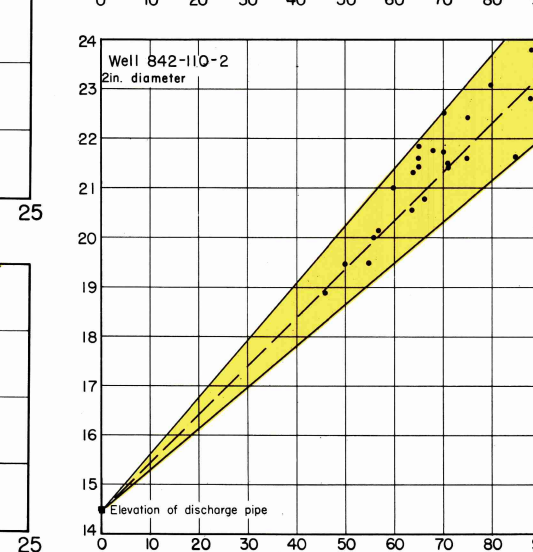
Relation between the static head and the yield of flowing wells.
