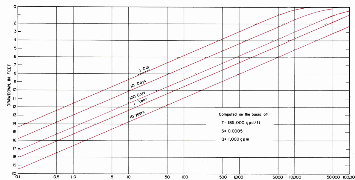
Theoretical drawdowns in the vicinity of a pumping well for selected periods of time.
