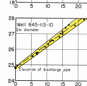
Relation between the static head and the yield of flowing wells.
