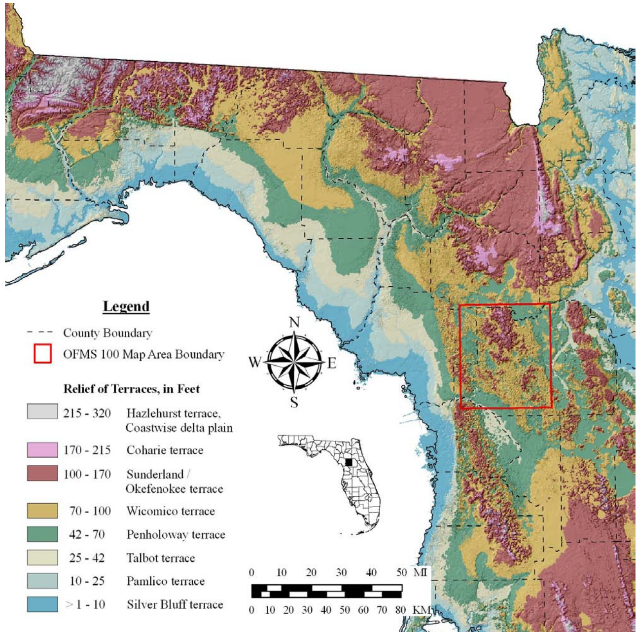
Figure 4. Terraces in Florida (after Healy, 1975).
