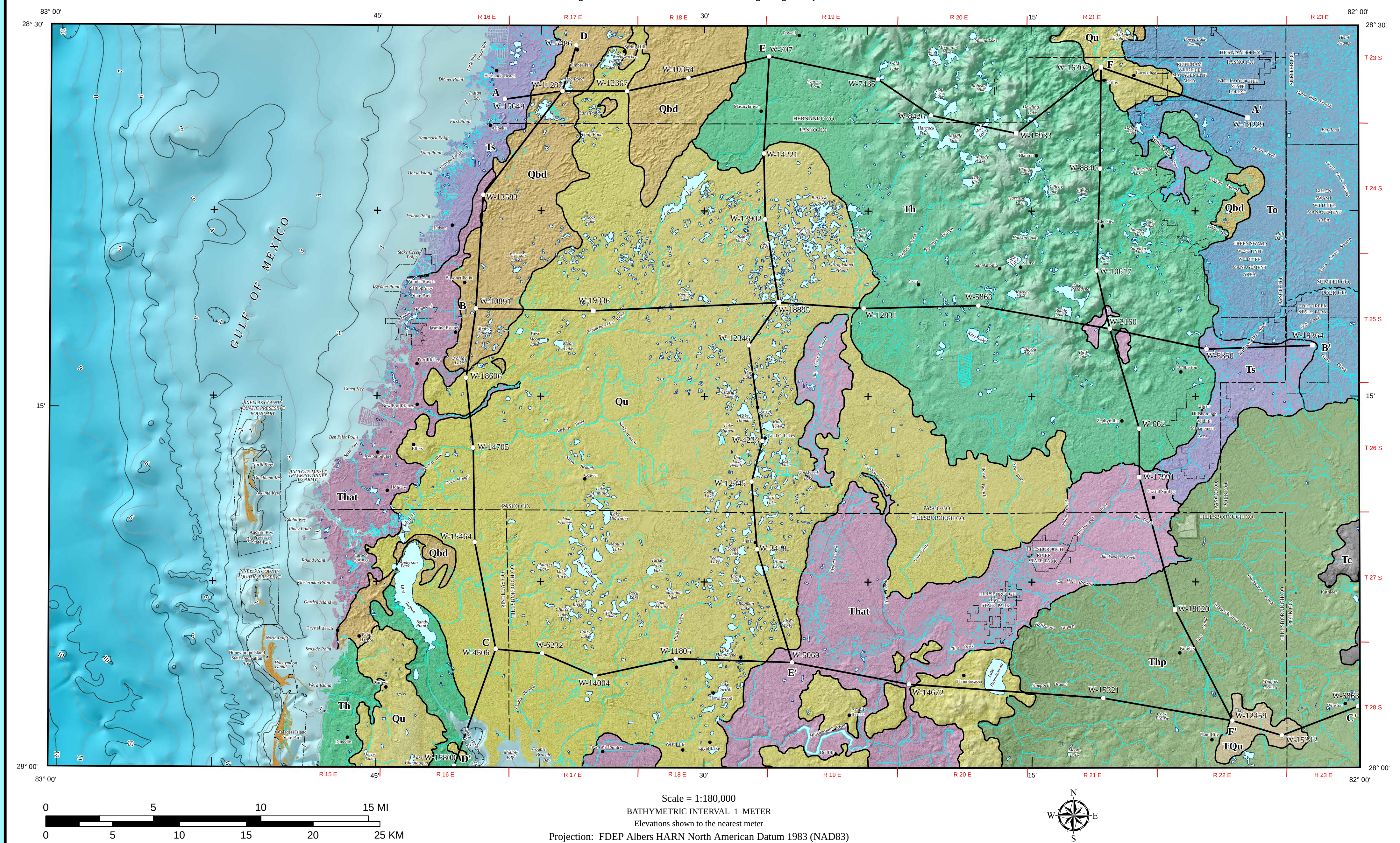
Figure 1. Location of cross-sections on geologic map.
