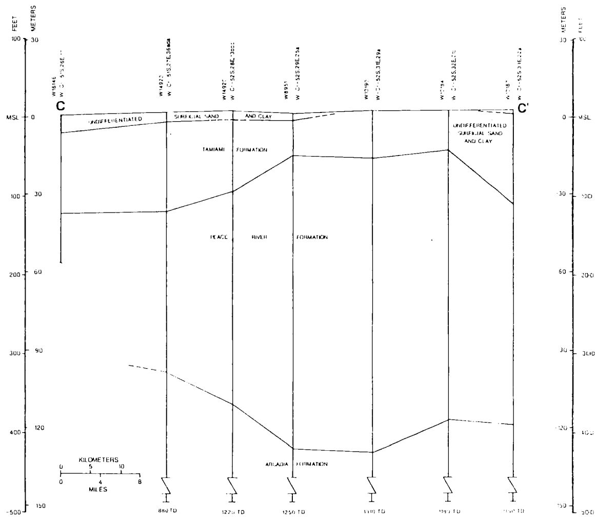
FIGURE 5 VERTICAL EXAGGERATION 400:1 WELL NUMBERS ARE FLORIDA GEOLOGICAL SURVEY ABBREVIATIONS
