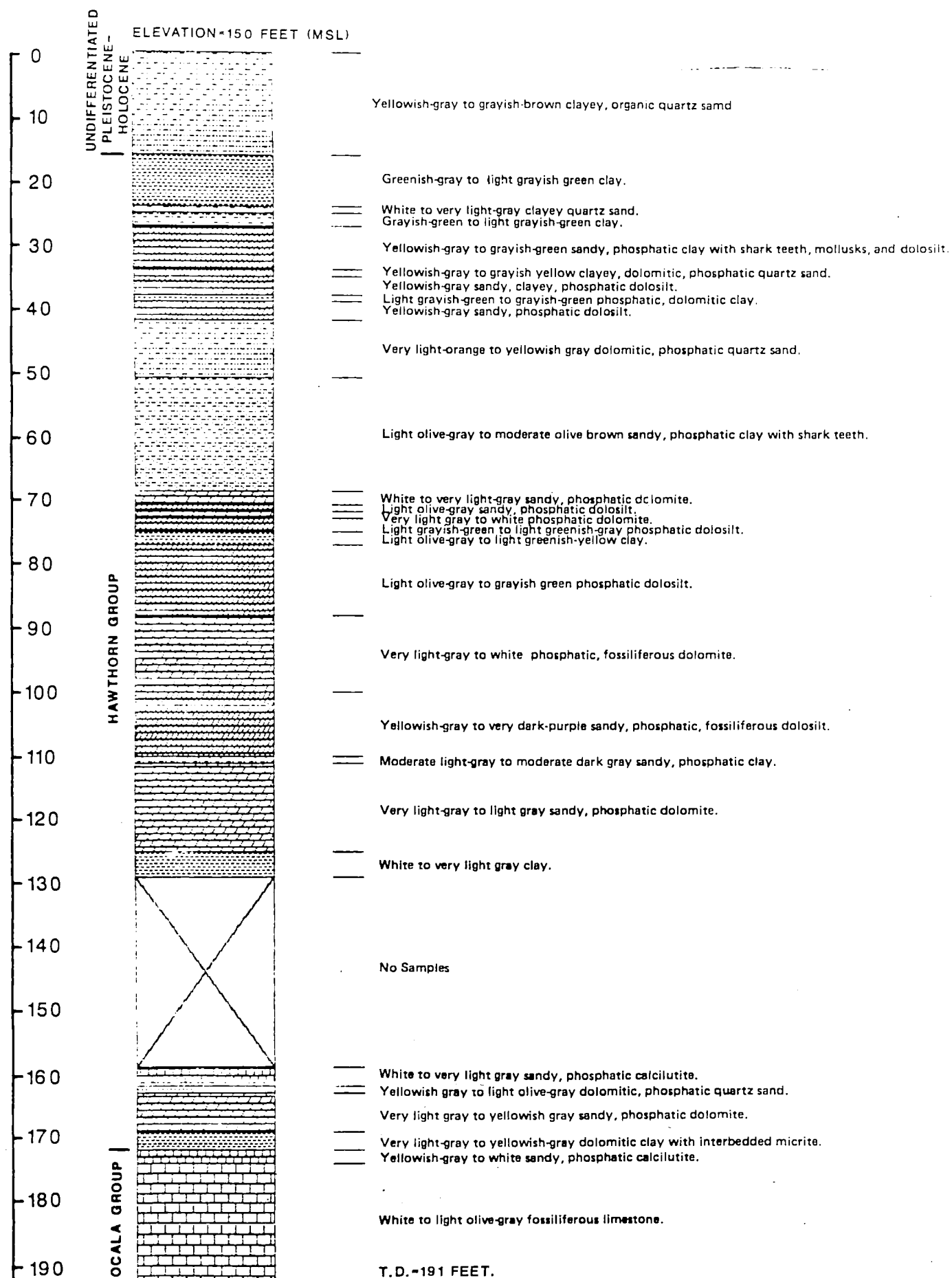
Figure 12: Columnar section for well #10 (W-16207).
