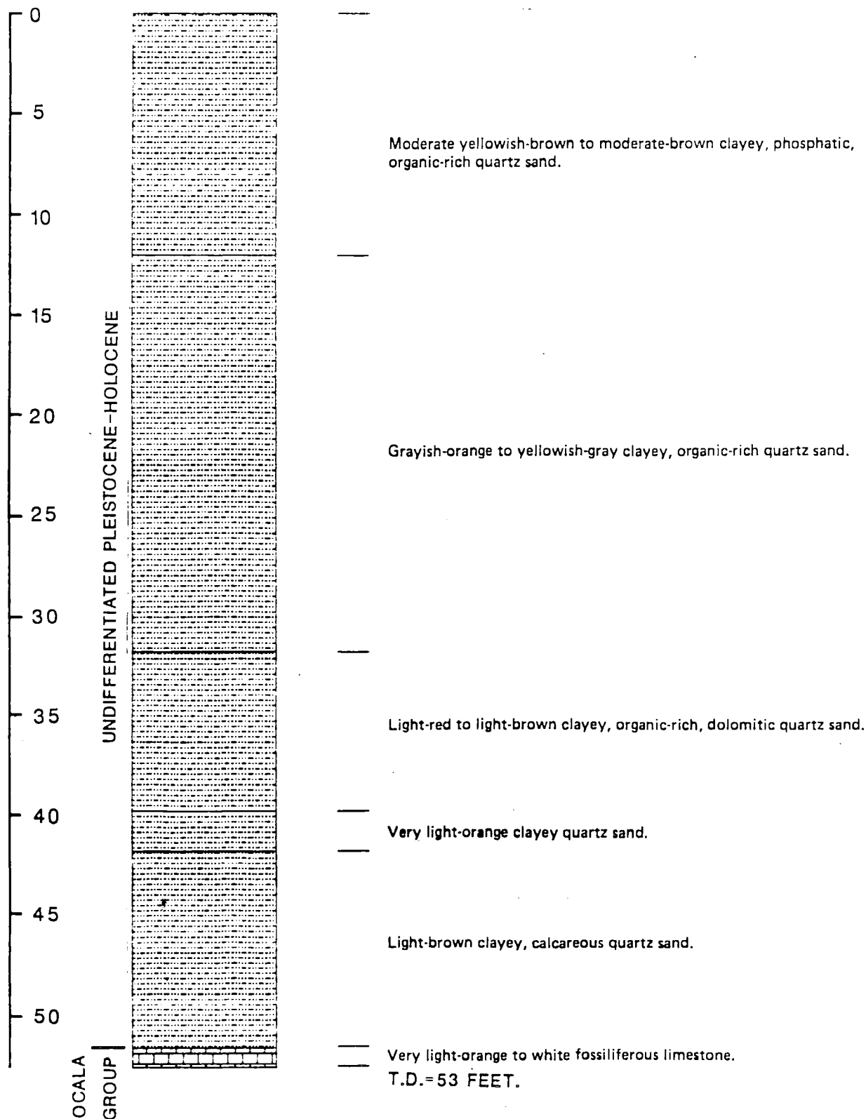
Figure 6: Columnar section for well #4 (W-16201).
