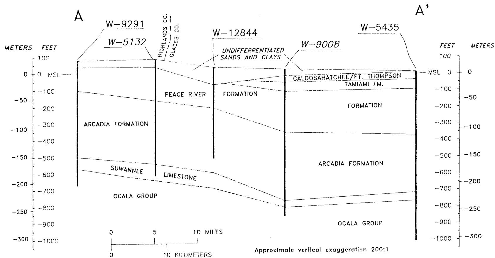
Figure 3 : Cross Section A - A'
