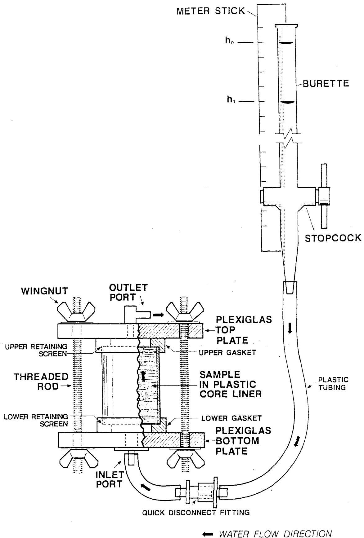
Figure 5. Falling head permeameter (Green et al. 1989).
