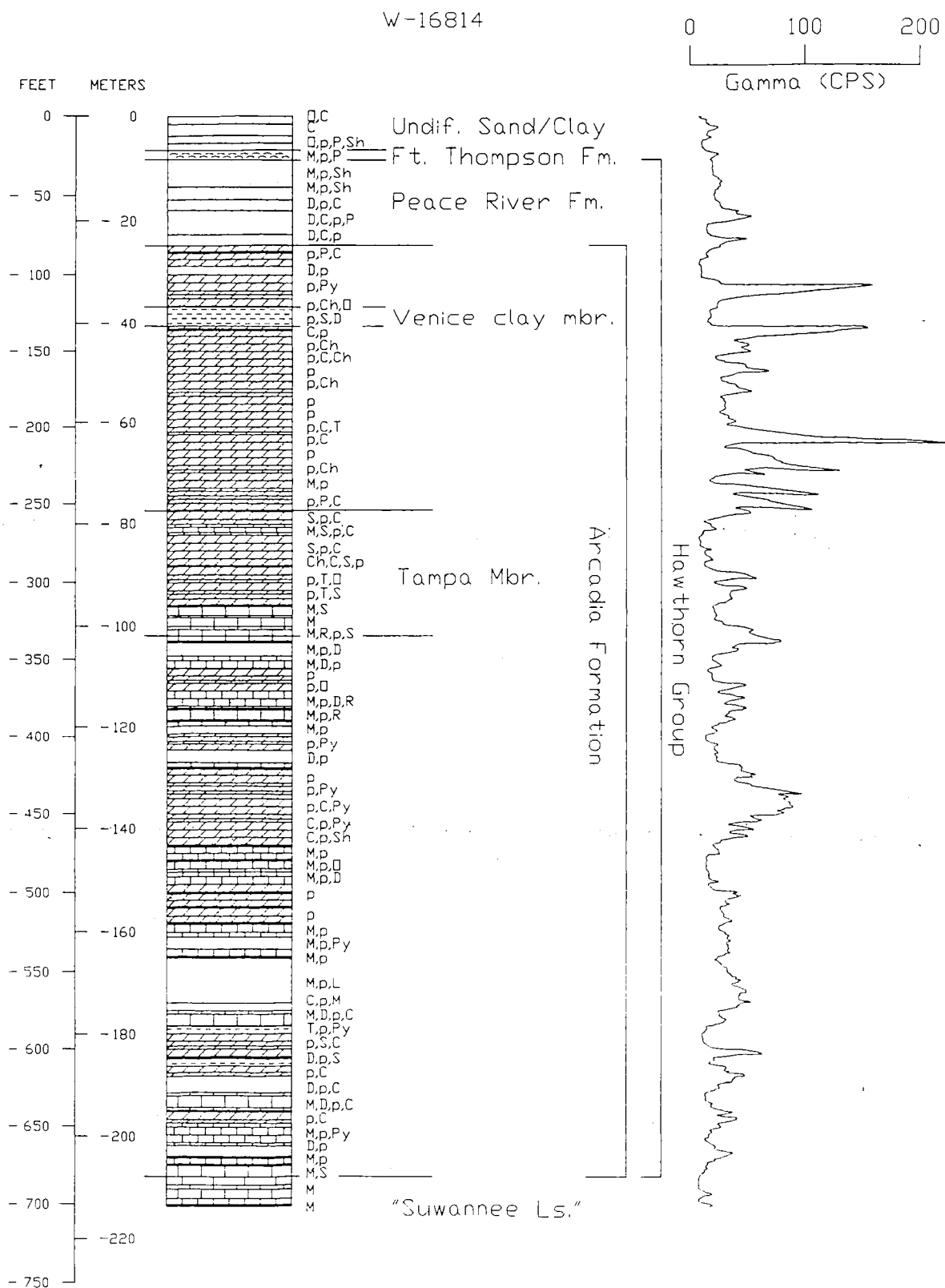
Figure 4: Stratigraphic column and gamma-ray log for South Venice Core.
