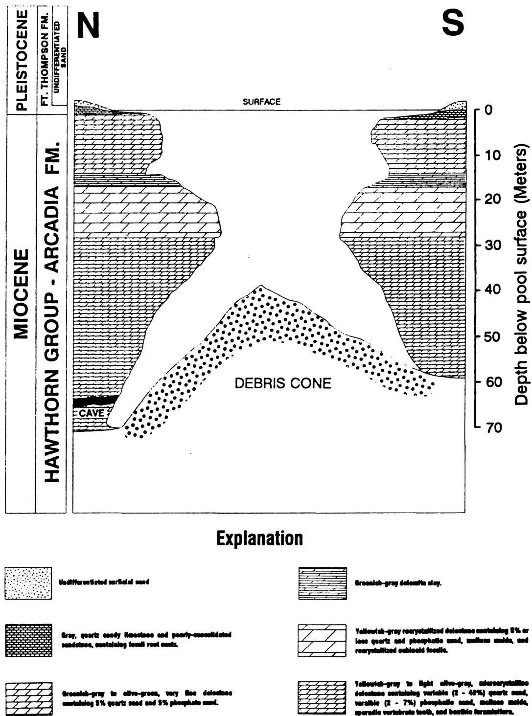
Figure 2. Geologic section in Warm Mineral Springs.
