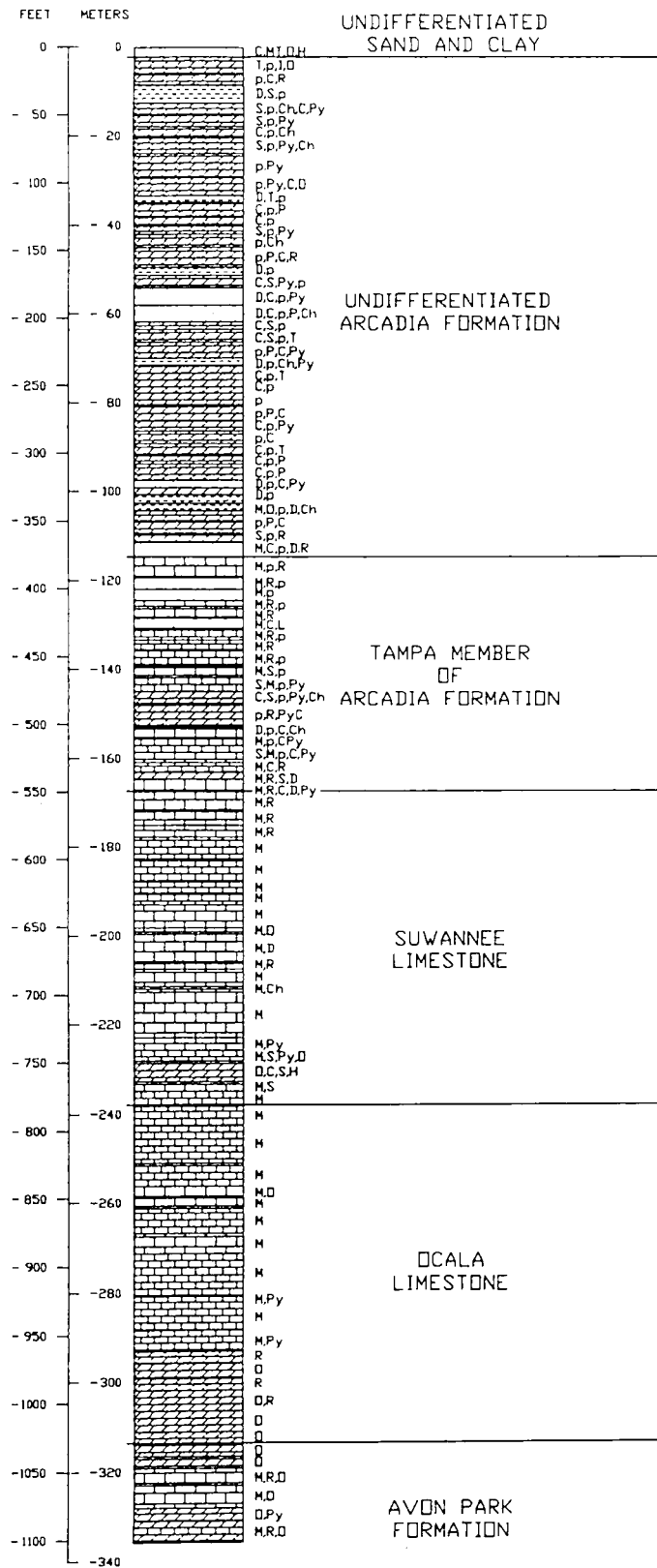
Figure 3. Stratigraphic column of W-16999
