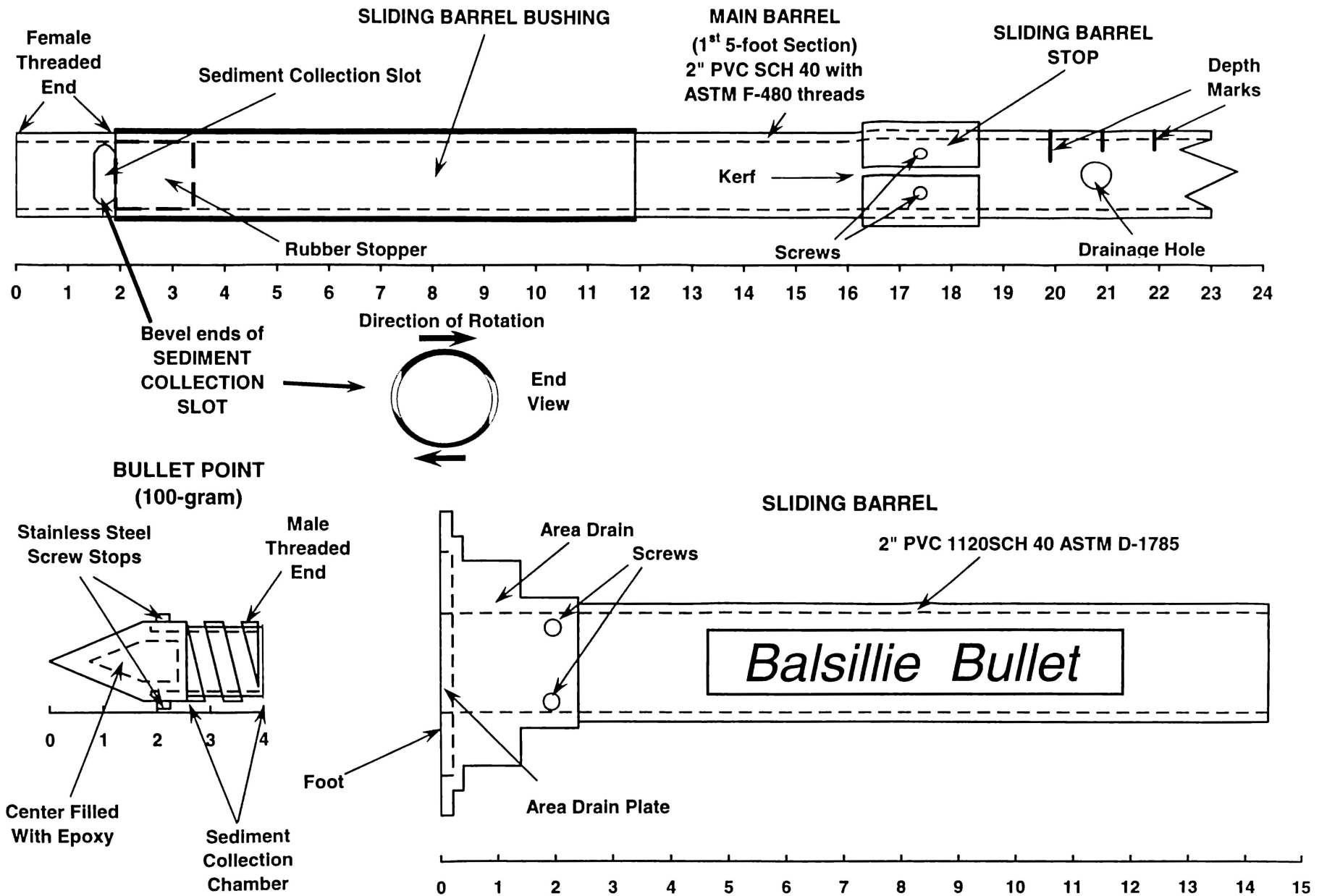
Figure 2. Schematic of dimensions of the bullet sampler; dimensions are in inches.
