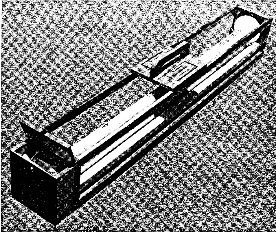
Figure 5. Bullet surface sediment sampler in its carrying case with storage box open.
