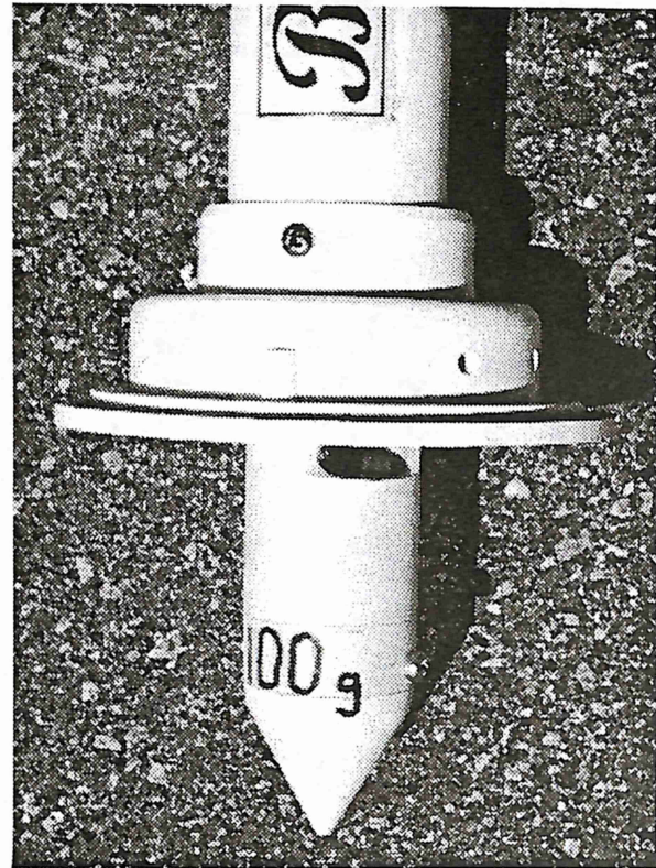
Figure 4. Detailed image of tip of the bullet surface sediment sampler showing the sliding barrel in position for sample collection (to be rotated in a clockwise direction only), one of two sediment collection slots, and the 100-gram bullet point sediment collection chamber. Upon extraction of the sampler, the sliding barrel slips down being stopped by the screw heads in the bullet point, thereby protecting the sample from being disturbed.
