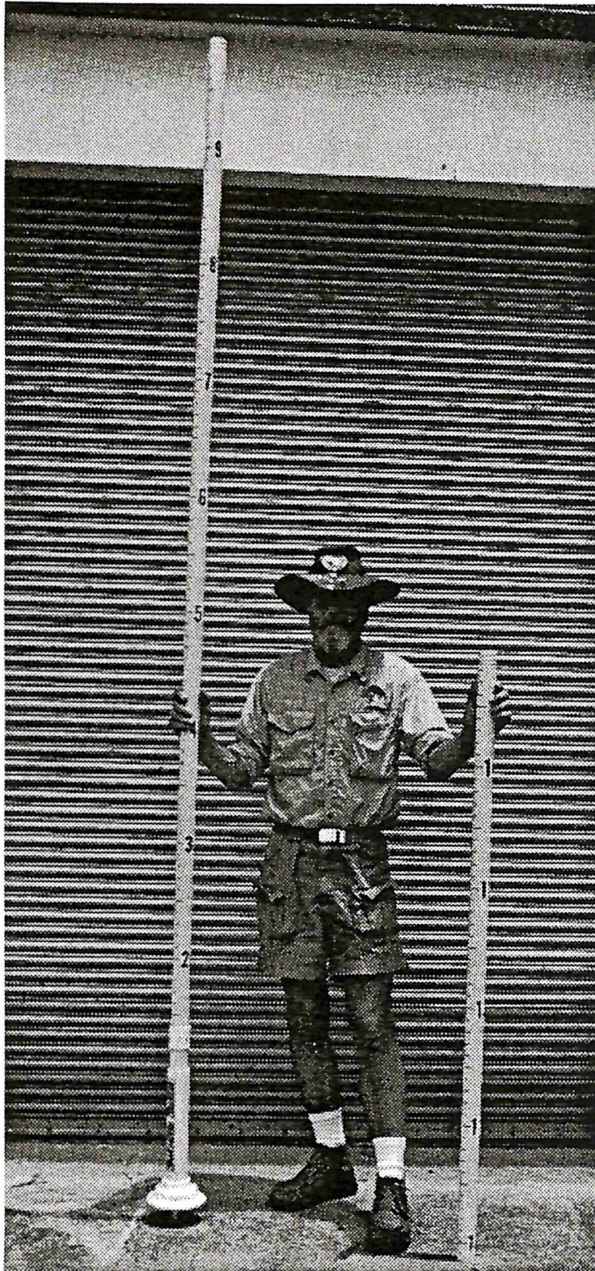
Figure 3. The author with a 10-foot length (two five-foot segments) of the bullet surface sediment sampler (left) with an additional five-foot segment of main barrel (right) that can be threaded onto the top of the 10-foot length for sampling in a water depth of 15 feet.
