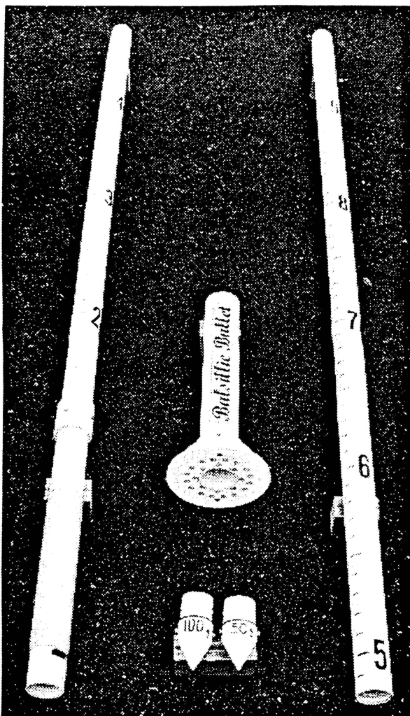
Figure 1. Basic components of bullet surface sediment sampler showing first five-foot segment (left) with fittings, second five-foot segment main barrel segment (right) that threads onto the first segment for sampling in water depths of up to 10 feet, sliding barrel (top middle), and 50-gram and 100-gram bullet points housing the sediment collection chamber (bottom middle).
