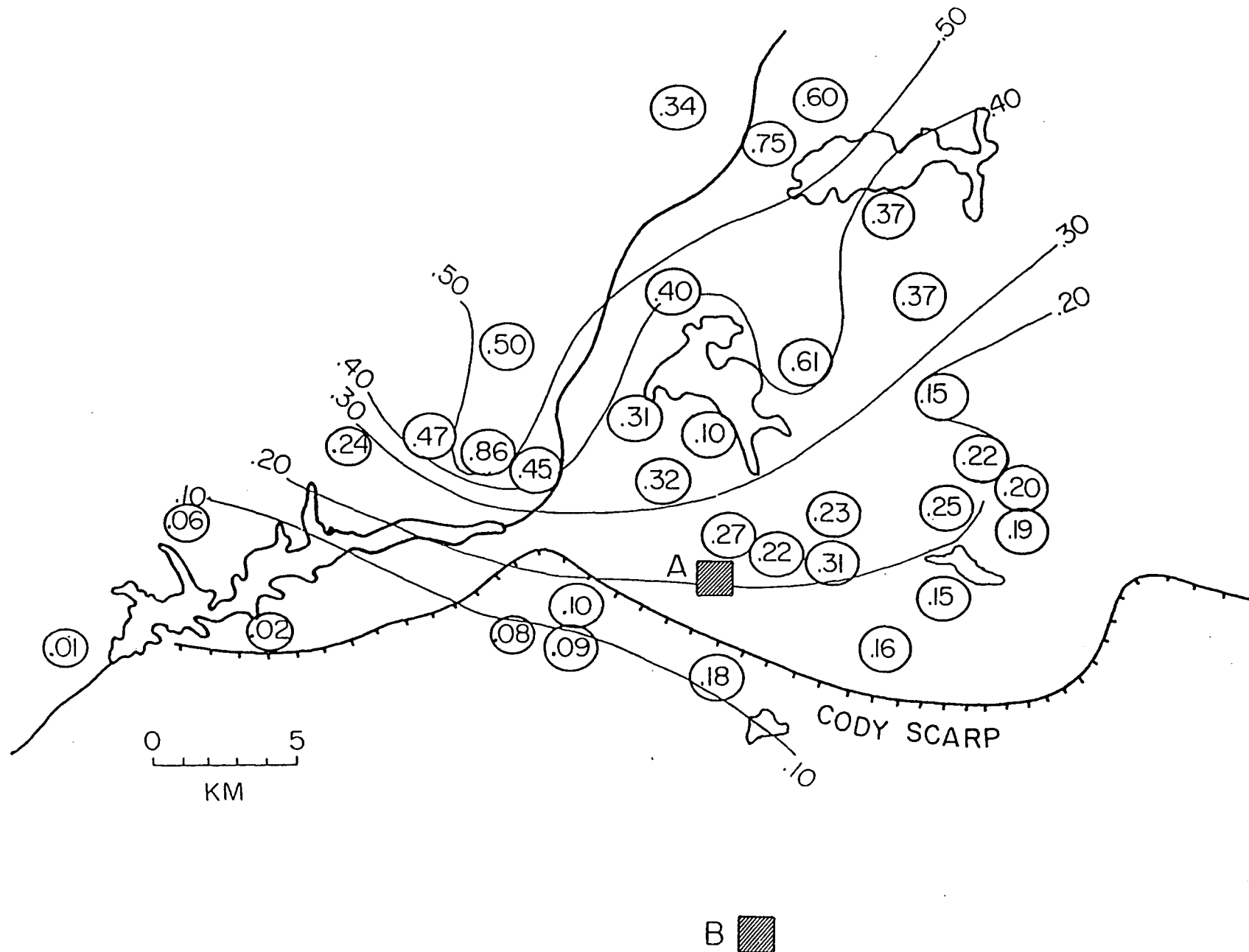
Figure 8. Regional variations of excess ^{234}\text{U} in the study area. Data points from wells in Leon and Gadsden counties are plotted. For orientation, the FSU campus (A) and Wakulla Springs (B) are shown. Infiltration from the surface causes the aquifer water to be diluted with respect to its conservative excess ^{234}\text{U} . As a result the regional variation shows aquifer flow direction, generally from north to south.
