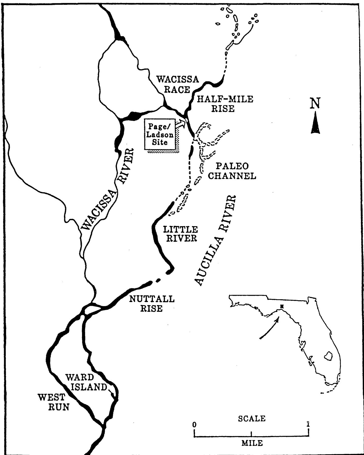
Figure 1. Location map for middle reaches of Aucilla River.
