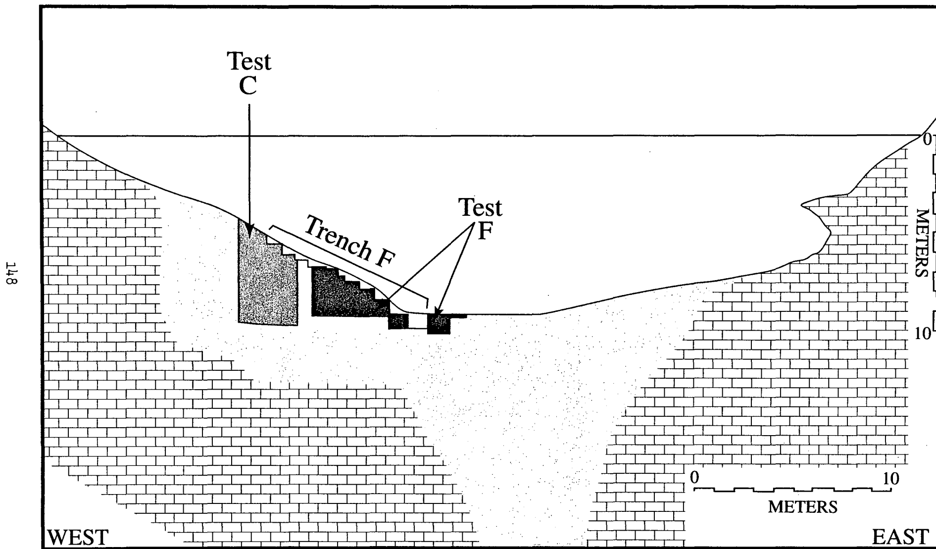
Figure 2. West-East Cross Section, Aucilla River, Page-Ladson Site
