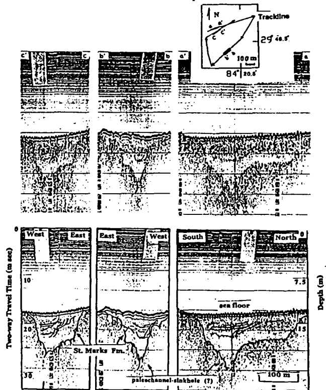
Figure 3. Sub-bottom seismic profiles south of Alligator Point (see Figure 1). The figure shows three crossings of the same isolated karst trough or paleochannel, separated by approximately 50 m and 300 m, respectively. The track lines of these crossings are shown in the map on top of the figure. Note the direction indicators on this figure (see Figure 1 for location). The three images indicate that the feature has been influenced by karstification. Evidence of subsidence can be observed in the disturbed sediment that has filled the feature.
