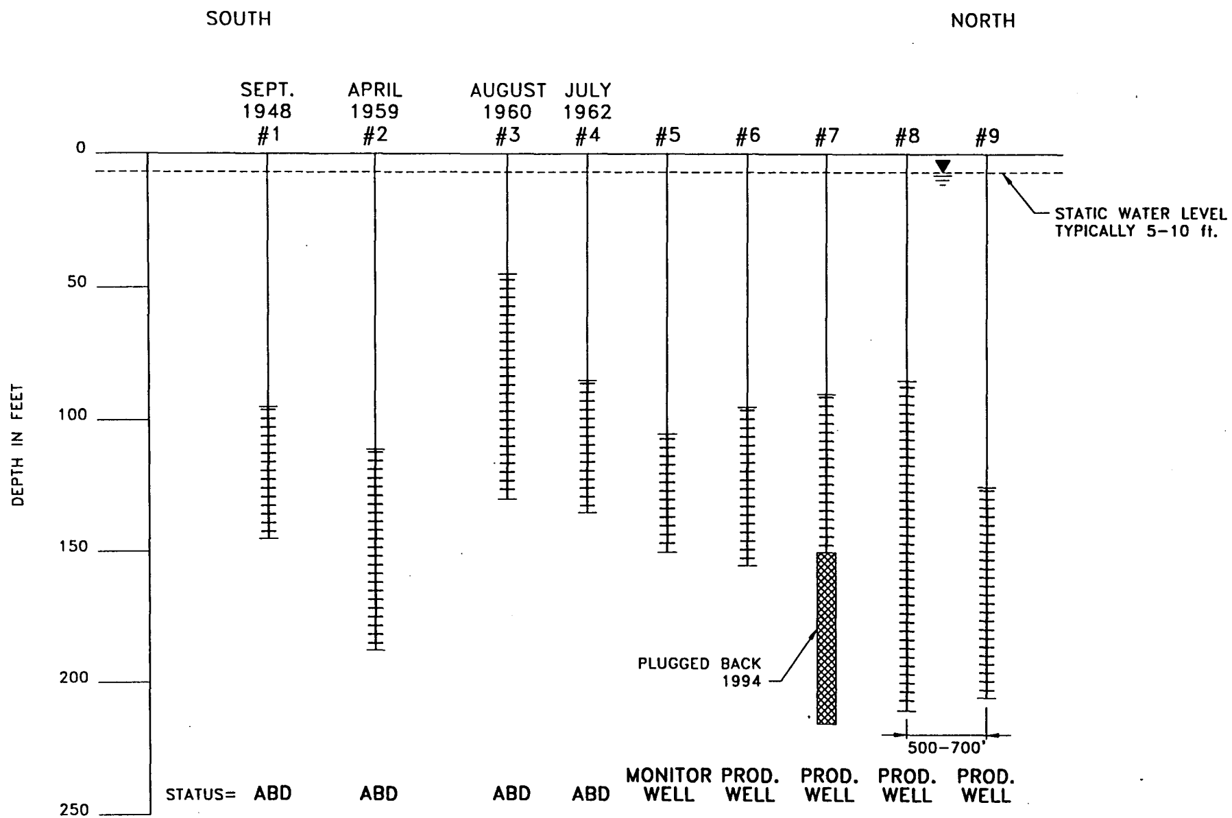
FIG-3: PROFILE OF PRODUCTION WELL CONSTRUCTION SPECIFICATIONS
