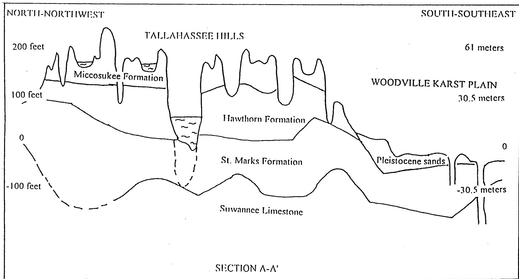
Figure 6. Hydrostratigraphic profile of the study area. The St. Marks and Suwannee Limestones constitute the Upper Floridan Aquifer, while the Hawthorn and Miccosukee Formations are aquicludes.
