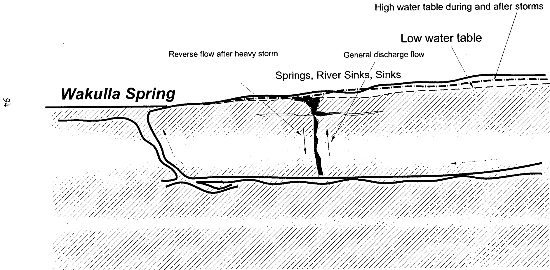
Figure 1. Wakulla Karst Plain Conceptual Flow Model
