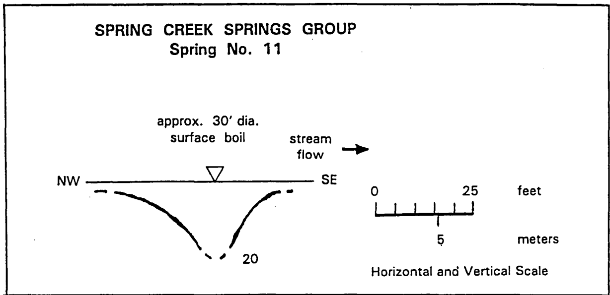
Figure 9. Cross section of Spring 11, in main channel of Spring Creek.
