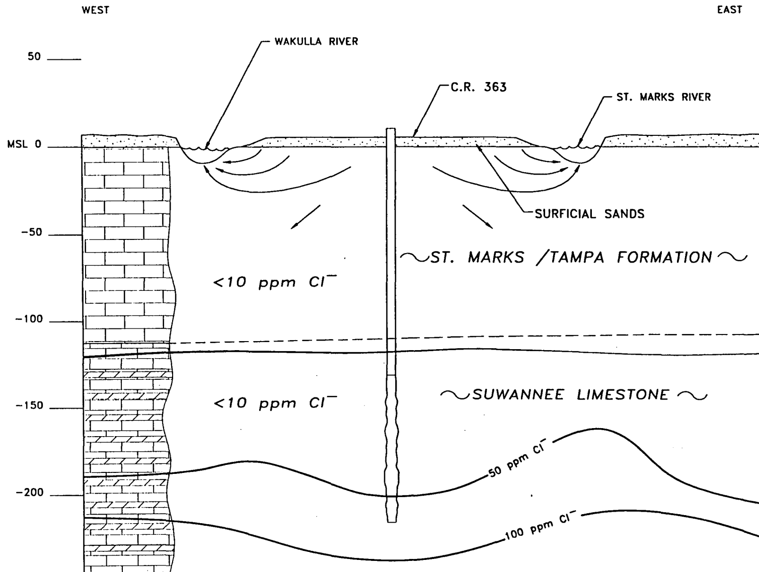
FIG-2: HYDROGEOLOGIC CROSS-SECTION THROUGH ST. MARKS PENINSULA
