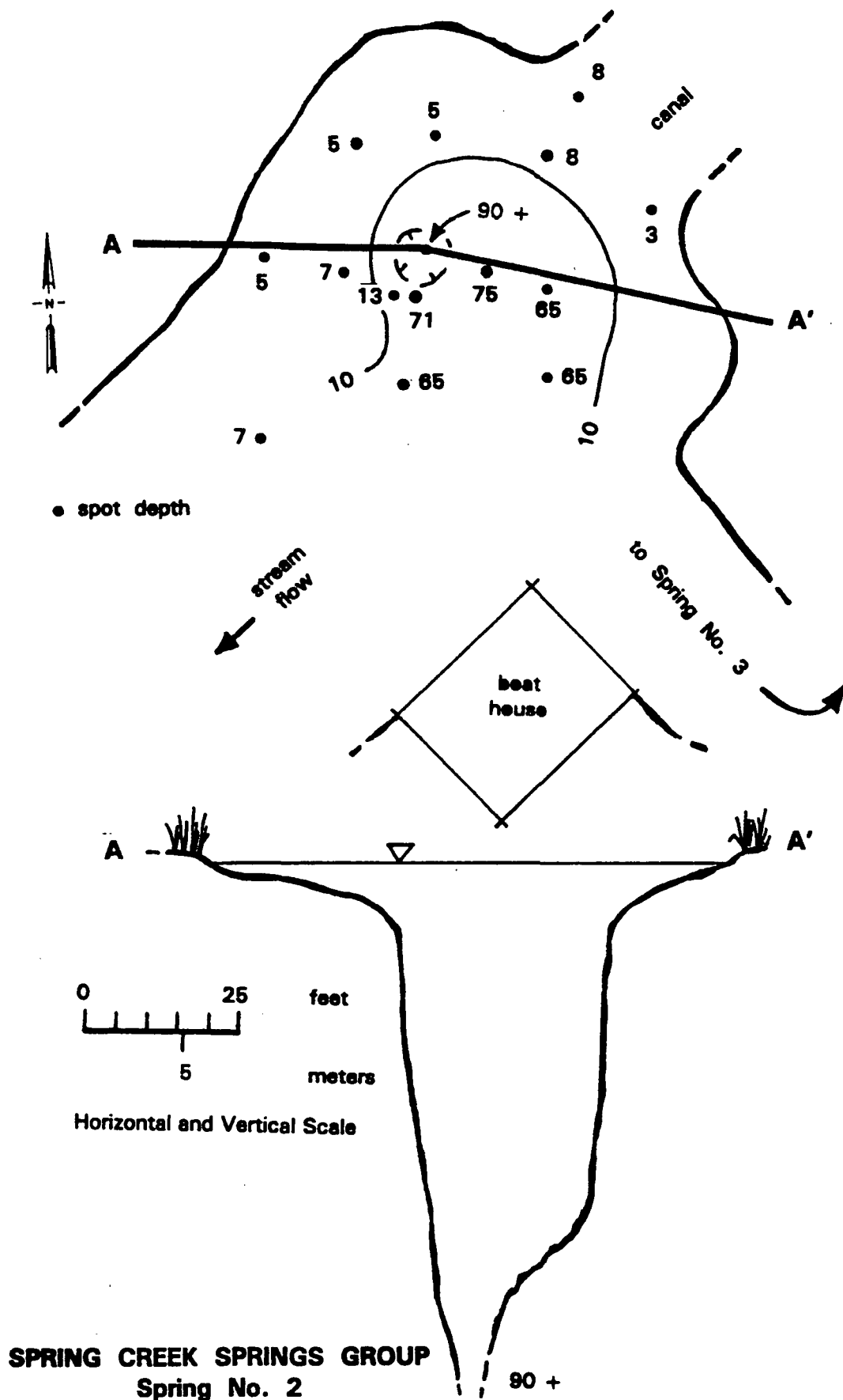
Figure 5. Plan and cross section of Spring 2.
