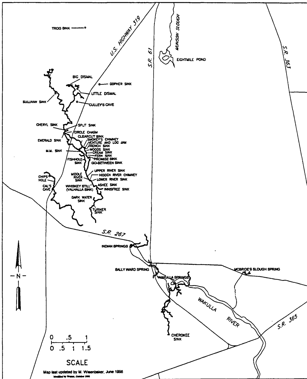
Figure 1. Plan view map of western Woodville Karst Plain illustrating of the Leon Sinks cave system (comprising northernmost Sullivan sink and Big Dismal sink to southernmost Turner sink), Chips Hole cave, Indian Springs cave, Sally Ward Spring cave, McBride's Slough Spring cave and Wakulla Springs cave system.
