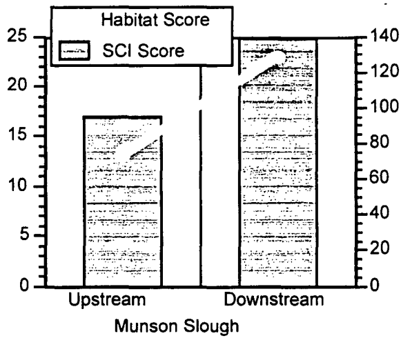
Figure 10: Improvements in the Stream Condition Index as observed between upstream and downstream stations in Munson Slough and Lafayette Creek. These improvements are believed to be related to the effects of impoundments (water quality improvements, flow attenuation) and also to observed improvements in habitat.
