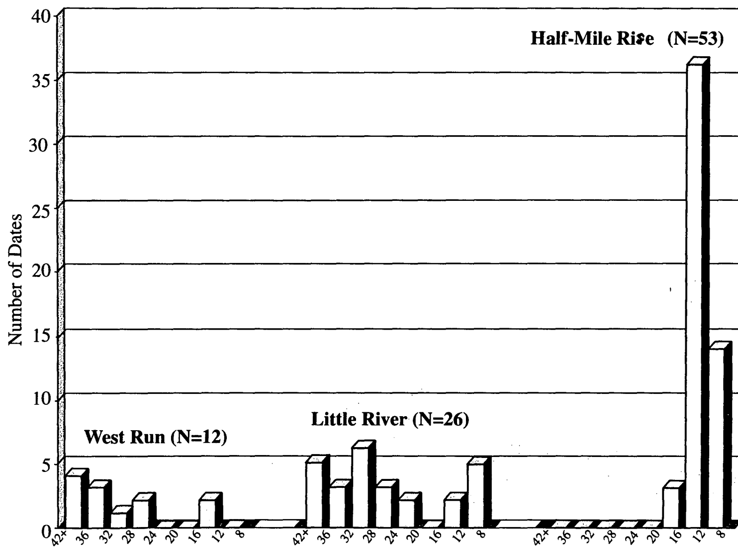
Figure 7. Carbon Date Distribution in three segments of the Aucilla River
