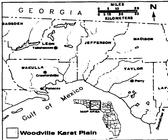
Figure 1. Location of the Woodville karst Plain.
