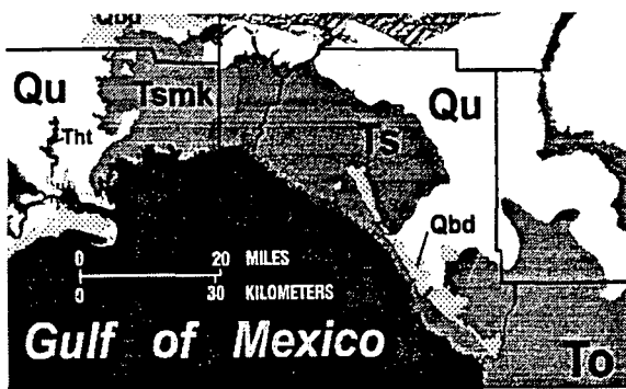
Figure 5. Geologic map of the eastern Florida panhandle (from Scott, 1998a).
