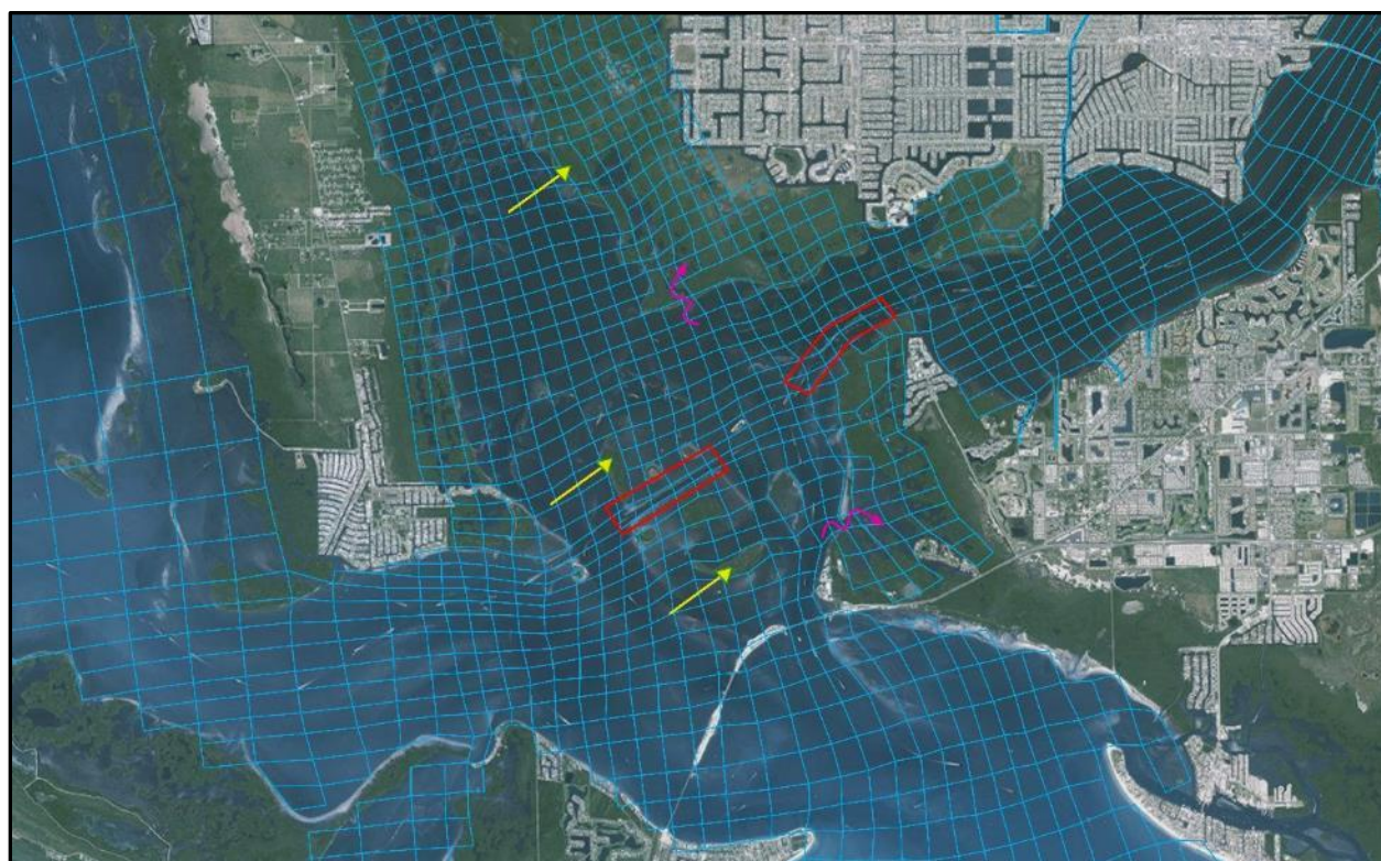
FIGURE 45: EXAMPLE OF UPDATES TO THE 2017 EFDC MODEL GRID
