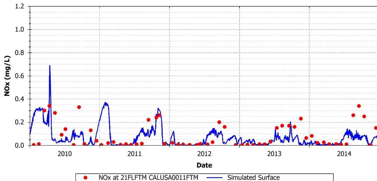
FIGURE 111: SIMULATED AND OBSERVED NO x AT 21FLFTM CALUSA0011FTM
