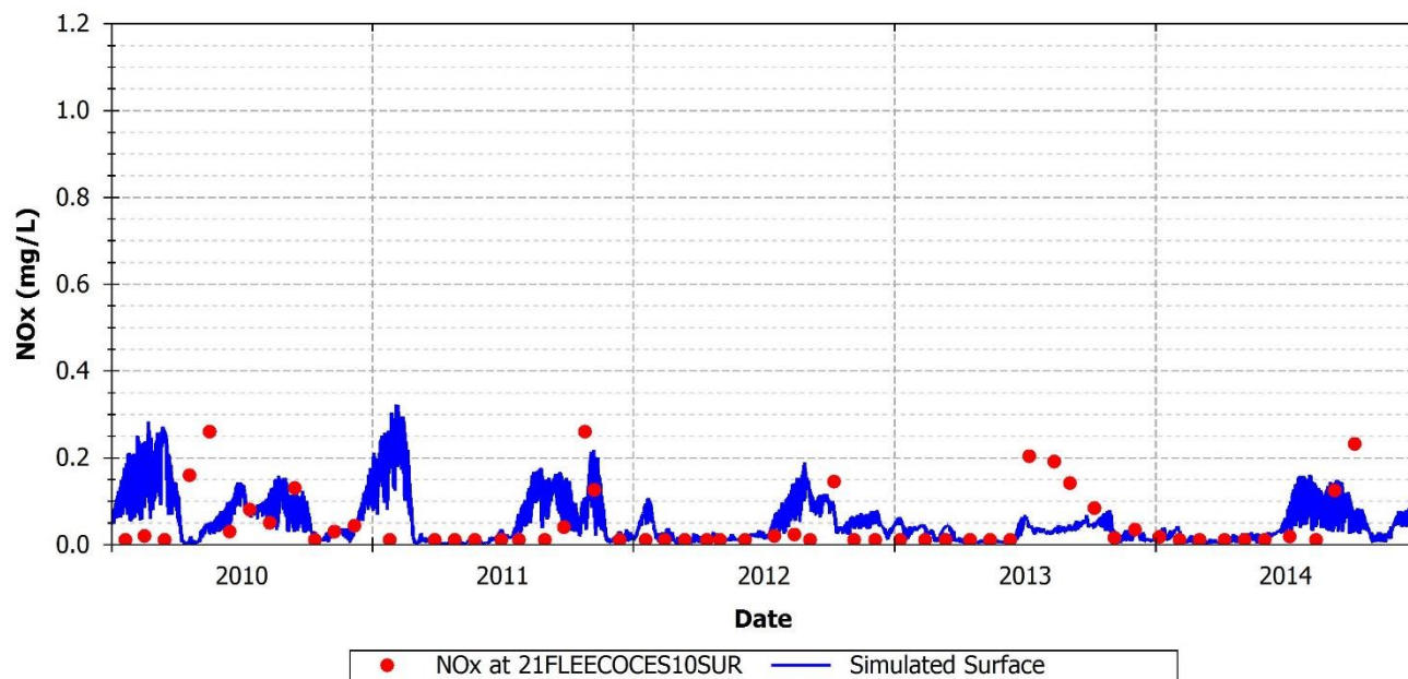
FIGURE 113: SIMULATED AND OBSERVED NO x AT 21FLEECOCES10SUR
