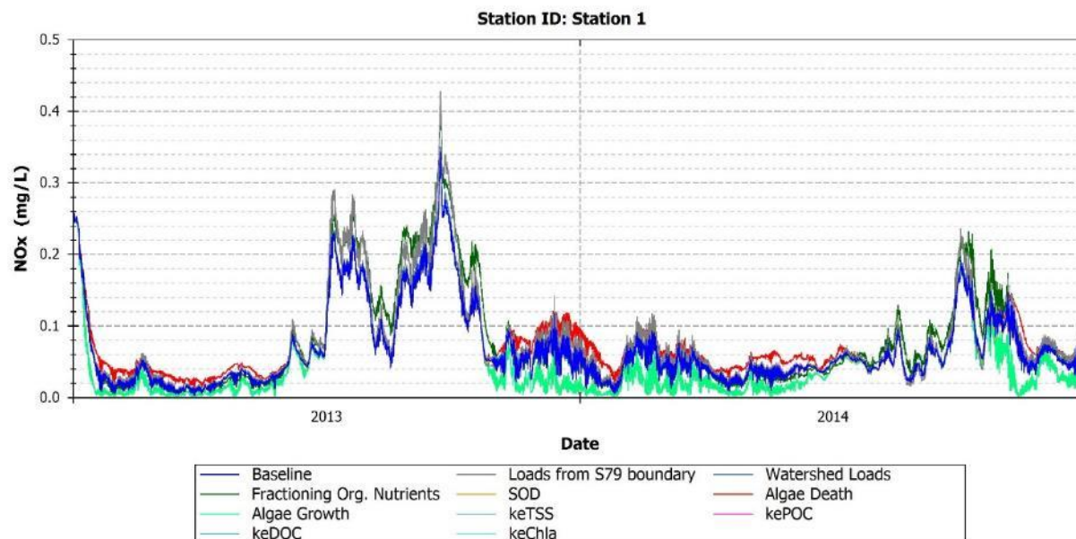
FIGURE 162: MODEL PREDICTIONS OF NO x FOR BASELINE AND PERTURBED MODEL CONDITIONS - STATION 1
