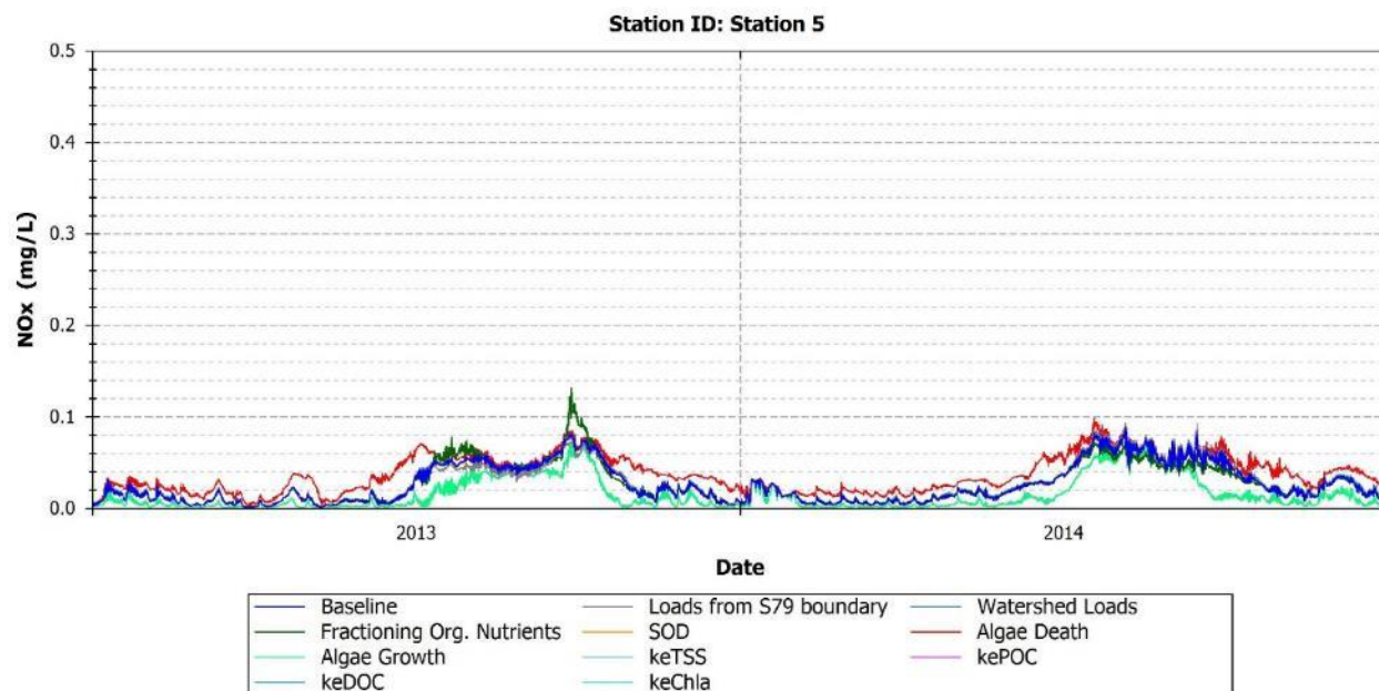
FIGURE 166: MODEL PREDICTIONS OF NO x FOR BASELINE AND PERTURBED MODEL CONDITIONS - STATION 5
