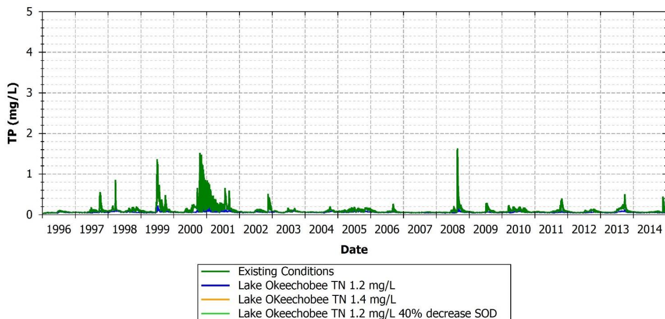
FIGURE 160: TP COMPARISON BETWEEN EXISTING AND SCENARIOS AT 21FLEECOCES10SUR, CALOOSAHATCHEE WATERWAY NEAR MOUTH
