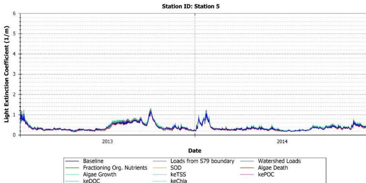
FIGURE 178: MODEL PREDICTIONS OF KE FOR BASELINE AND PERTURBED MODEL CONDITIONS - STATION 5
