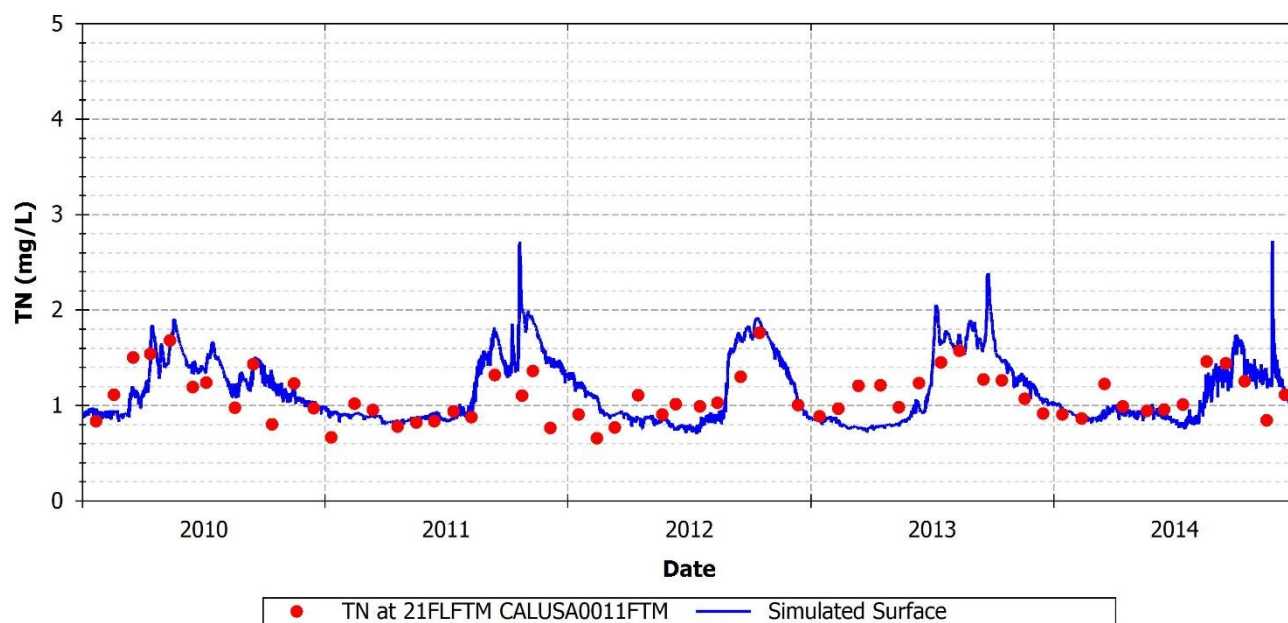
FIGURE 107: SIMULATED AND OBSERVED TN AT 21FLFTM CALUSA0011FTM
