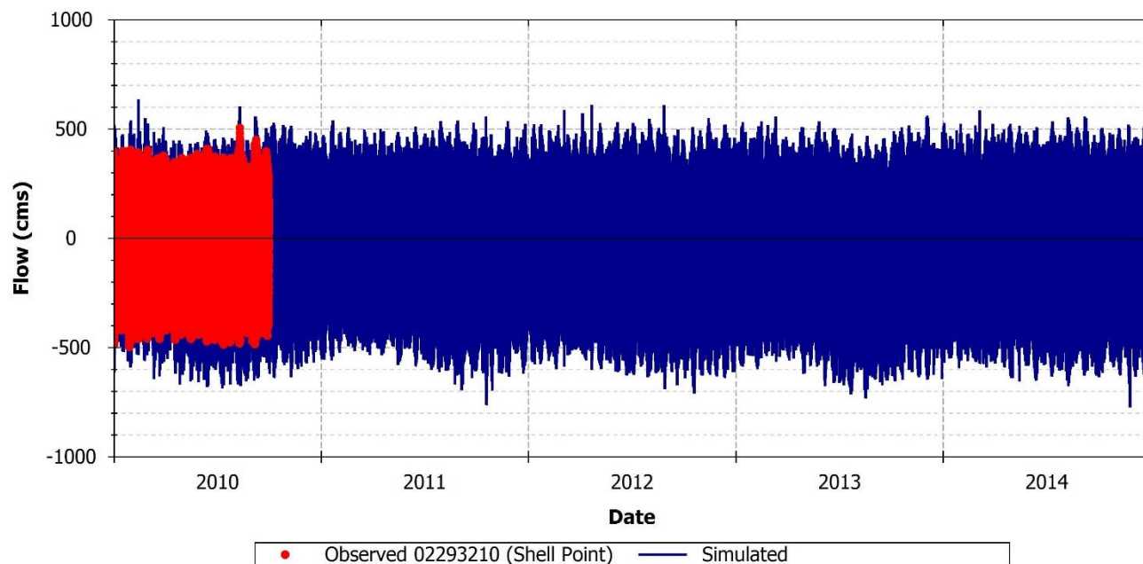
FIGURE 93: SIMULATED AND OBSERVED FLOW AT USGS 02293210 (SHELL POINT), 2010 – 2014
