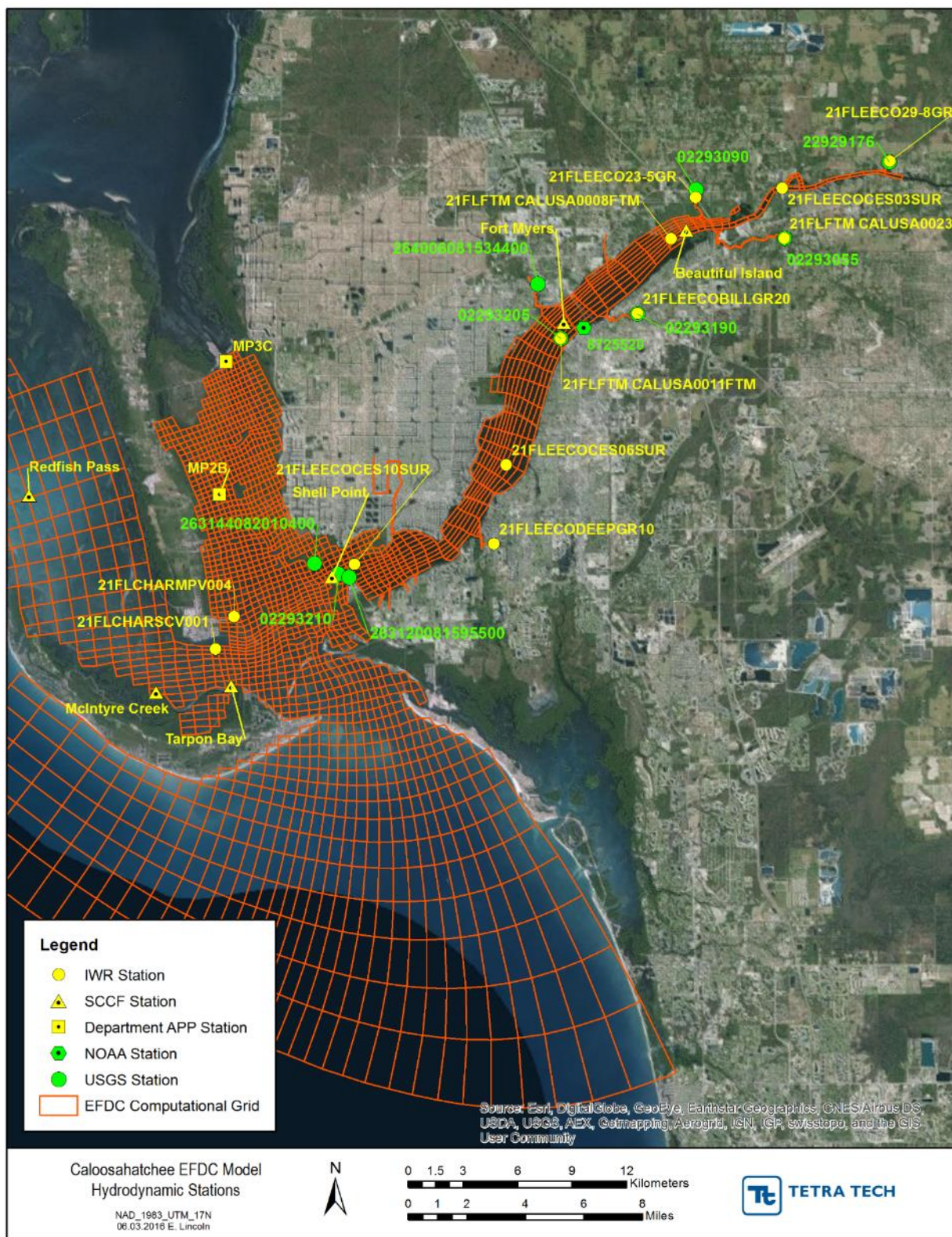
FIGURE 71: 2017 EFDC MODEL HYDRODYNAMIC RESULTS COMPARISON STATION LOCATIONS
