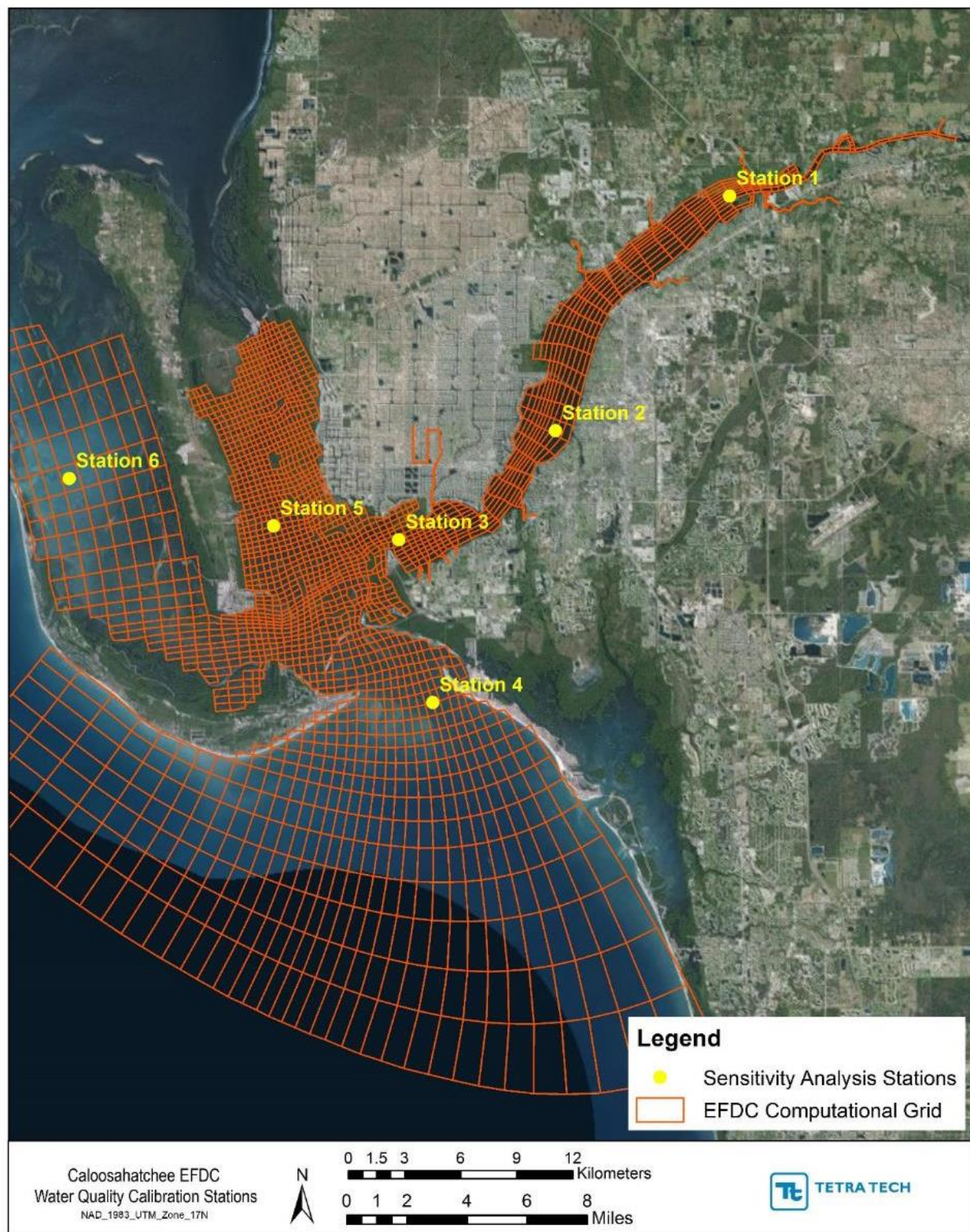
FIGURE 143: SELECTED LOCATIONS FOR THE SENSITIVITY ANALYSIS
