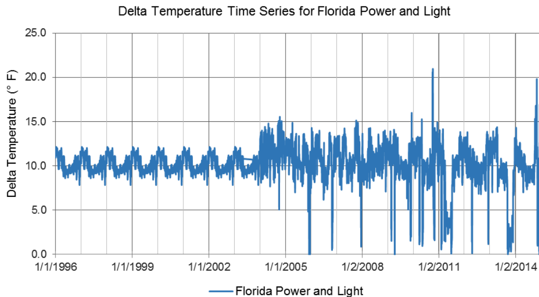
FIGURE 70: TIME SERIES OF DELTA TEMPERATURES PRESCRIBED IN THE 2017 EFDC MODEL FOR FL0001490
