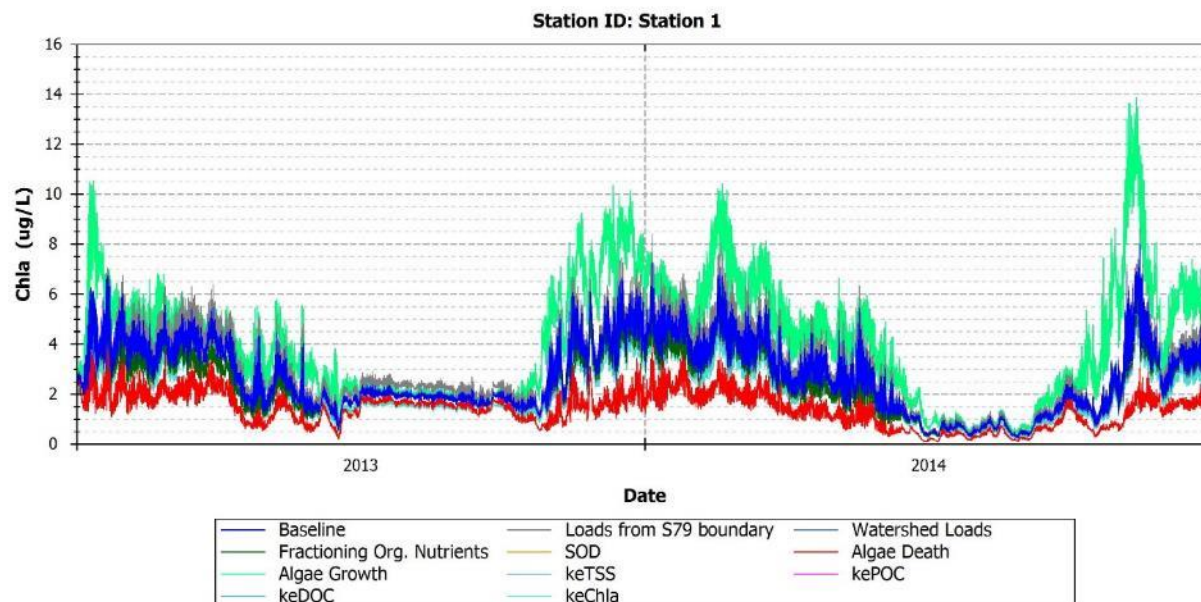
FIGURE 150: MODEL PREDICTIONS OF PHYTOPLANKTON BIOMASS FOR BASELINE AND PERTURBED MODEL CONDITIONS - STATION 1
