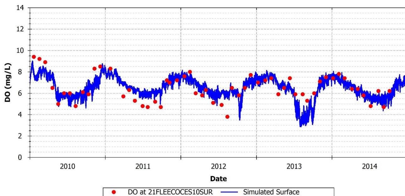
FIGURE 100: SIMULATED AND OBSERVED DO AT 21FLEECOCES10SUR
