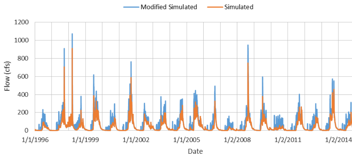
FIGURE 33: SIMULATED TIME SERIES VS. MODIFIED SIMULATED TIME SERIES THAT INCLUDES CALCULATED EXTERNAL SOURCE AT JACKS BRANCH DEP GAGE (01/01/1996 – 12/31/2014)
