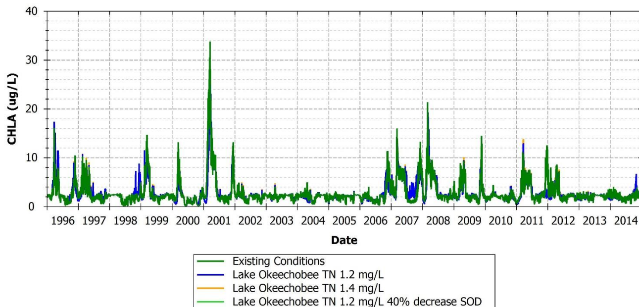
FIGURE 164: PHYTOPLANKTON BIOMASS COMPARISON BETWEEN EXISTING AND SCENARIOS AT 21FLEECOCES03SUR, CALOOSAHATCHEE WATERWAY, ROUTE 31
