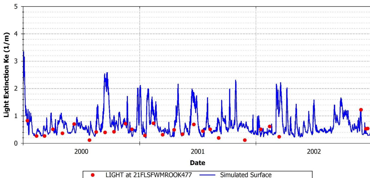
FIGURE 136: OBSERVED VERSUS PREDICTED LIGHT EXTINCTION AT 21FLSWMROOK477
