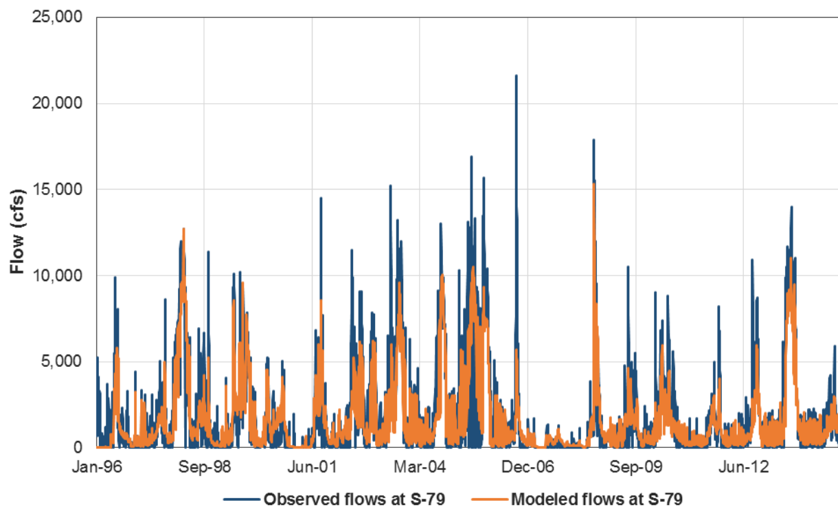
FIGURE 51: COMPARISON BETWEEN OBSERVED FLOWS AT USGS 02292900 VERSUS MODELED FLOWS FROM HSPF AT S-79
