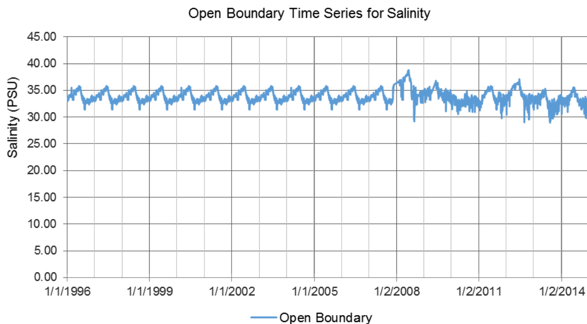
FIGURE 56: NORTHERN BOUNDARY 2017 MODEL INPUT TIME SERIES FOR SALINITY (PSU)
