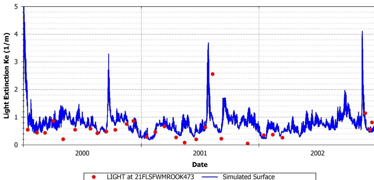
FIGURE 132: OBSERVED VERSUS PREDICTED LIGHT EXTINCTION AT 21FLSWMROOK473
