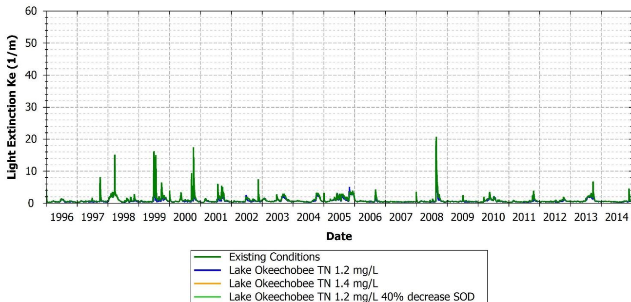
FIGURE 185: LIGHT EXTINCTION COMPARISON BETWEEN EXISTING AND SCENARIOS AT 21FLEECOCES06SUR, CALOOSAHATCHEE WATERWAY, MARKER 66
