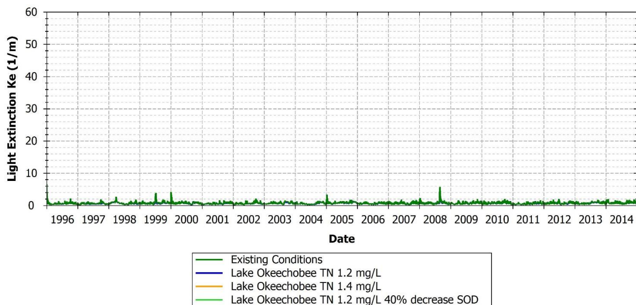
FIGURE 183: LIGHT EXTINCTION COMPARISON BETWEEN EXISTING AND SCENARIOS AT 21CHARMPV004, MATLACHA PASS
