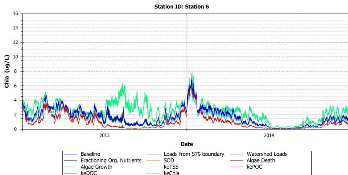
FIGURE 155: MODEL PREDICTIONS OF PHYTOPLANKTON BIOMASS FOR BASELINE AND PERTURBED MODEL CONDITIONS - STATION 6
