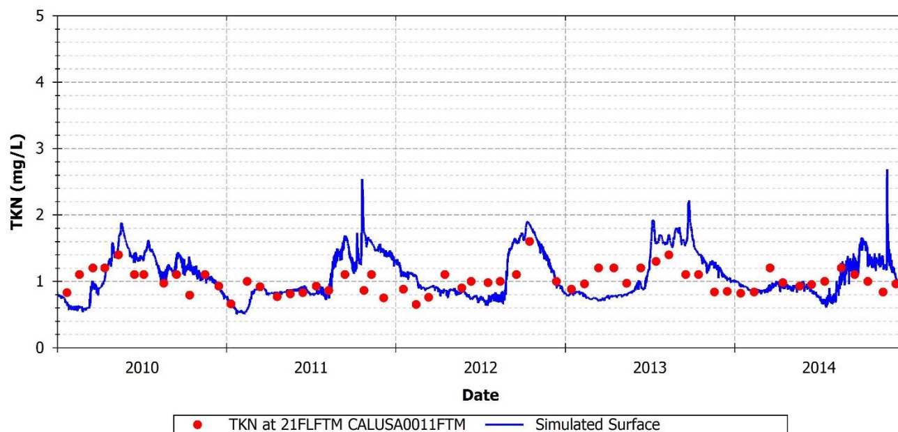
FIGURE 118: SIMULATED AND OBSERVED TKN AT 21FLFTM CALUSA0011FTM
