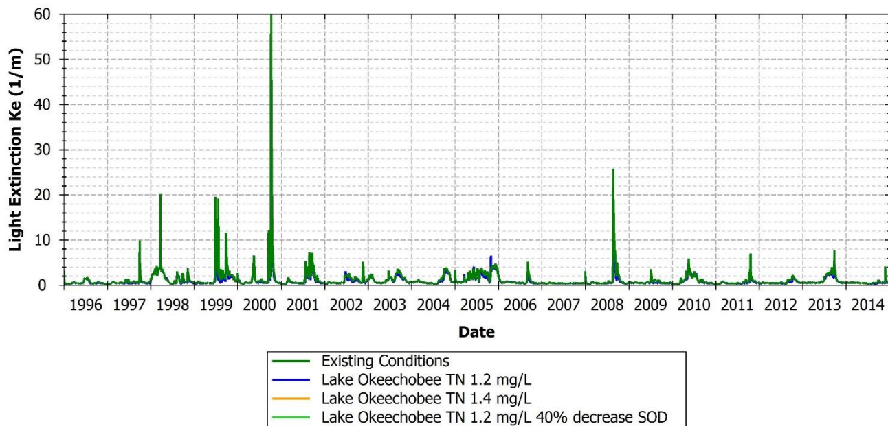
FIGURE 188: LIGHT EXTINCTION COMPARISON BETWEEN EXISTING AND SCENARIOS AT 21FLFTM CALUSA0011FTM, CALOOSAHATCHEE WATERWAY, MARKER 52
