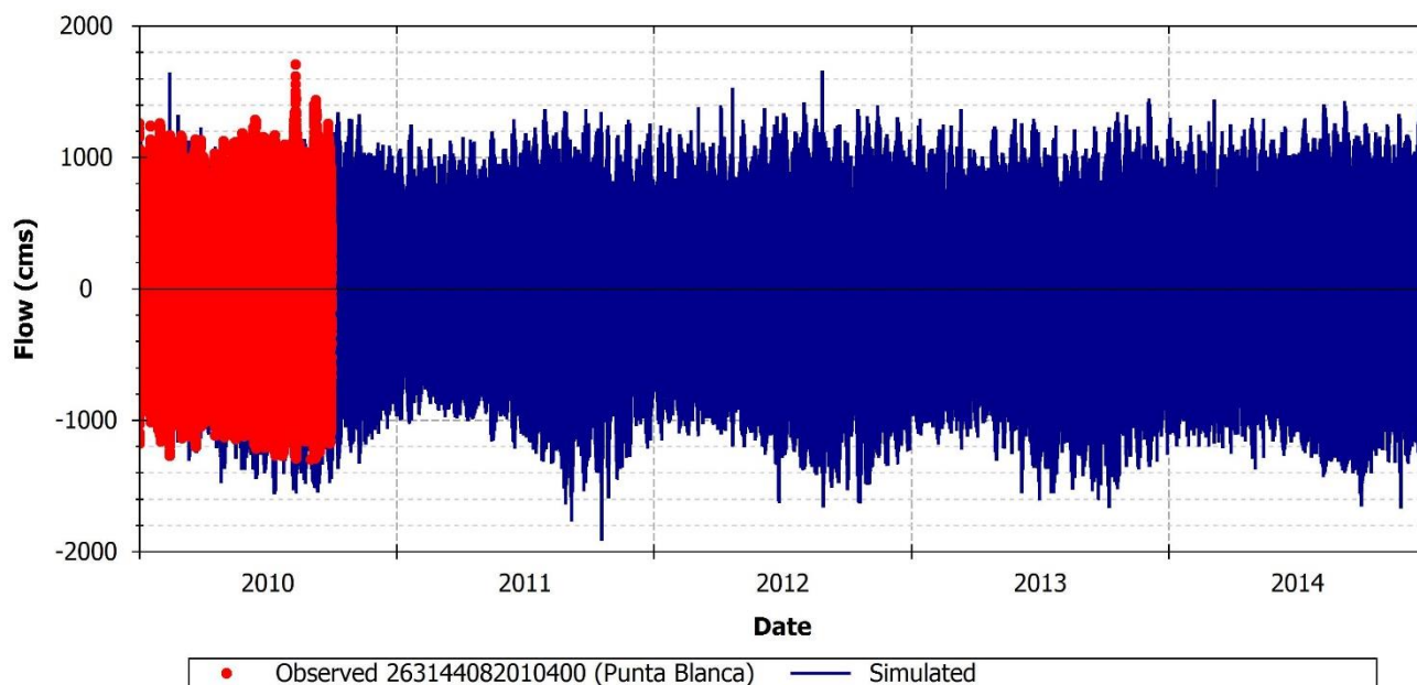
FIGURE 92: SIMULATED AND OBSERVED FLOW AT STATION 2631440820810400 (PUNTA BLANCA), 2010 – 2014
