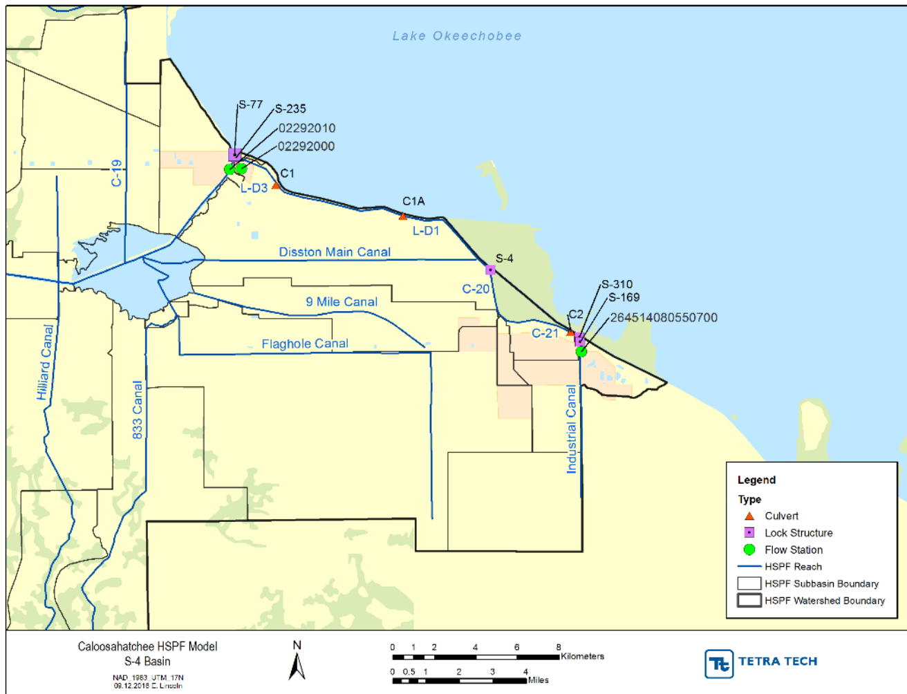
FIGURE 30: S-4 BASIN CANALS, LOCK STRUCTURES, AND CULVERTS
