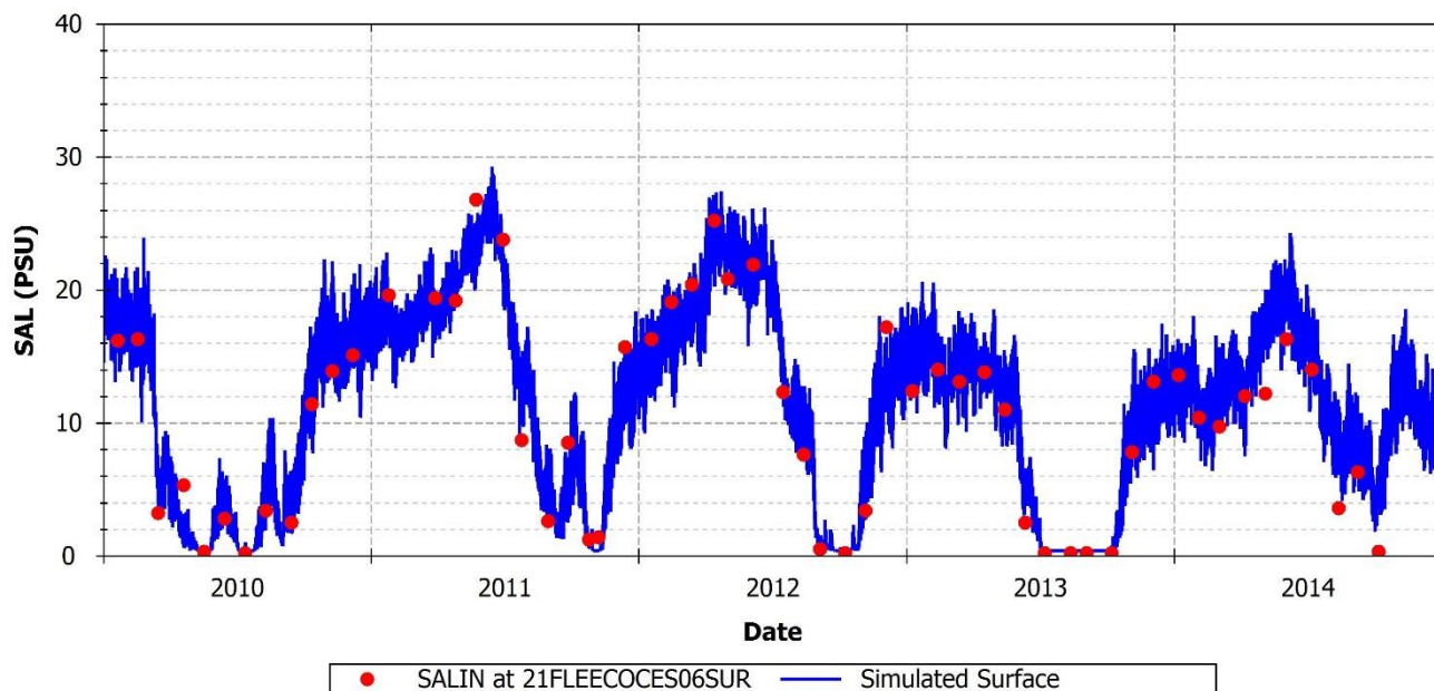
FIGURE 86: SIMULATED AND OBSERVED SALINITY AT 21FLEECOCES06SUR
