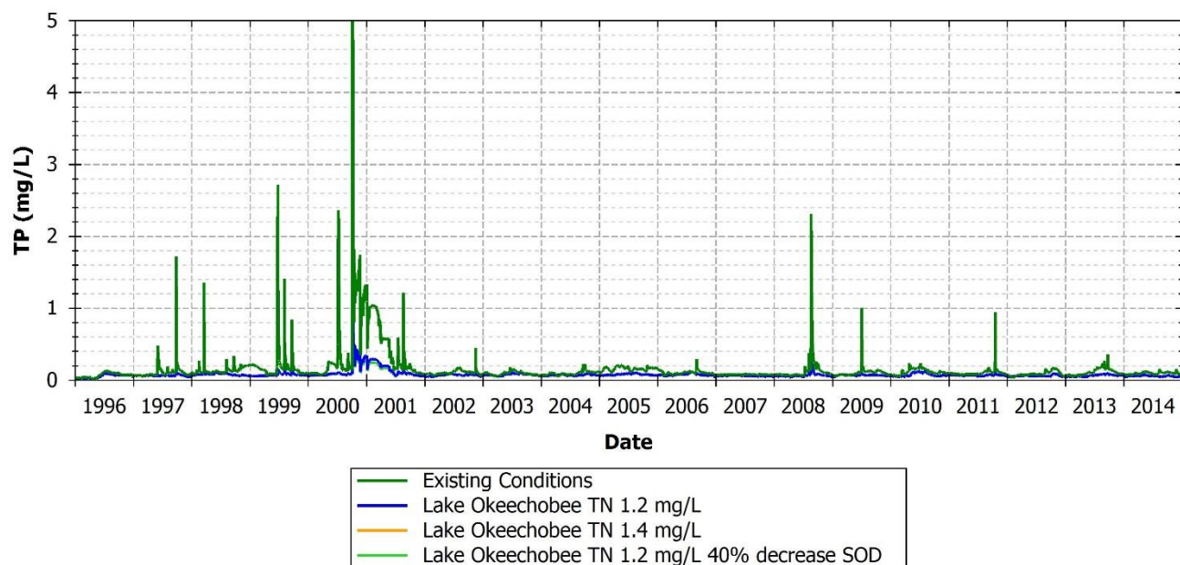
FIGURE 158: TP COMPARISON BETWEEN EXISTING AND SCENARIOS AT 21FLEECOCES03SUR, CALOOSAHATCHEE WATERWAY, ROUTE 31
