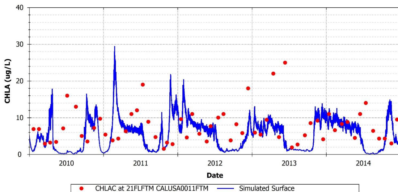
FIGURE 103: SIMULATED AND OBSERVED PHYTOPLANKTON BIOMASS AT 21FLFTM CALUSA0011FTM
