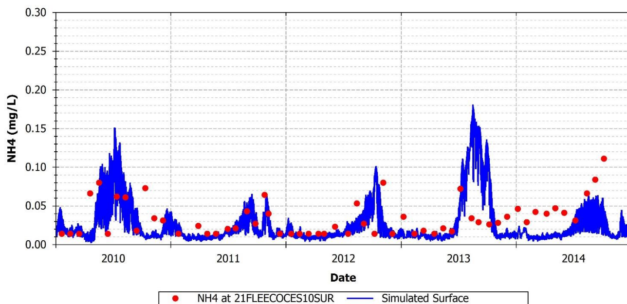
FIGURE 115: SIMULATED AND OBSERVED NH 4 AT 21FLEECOCES10SUR
