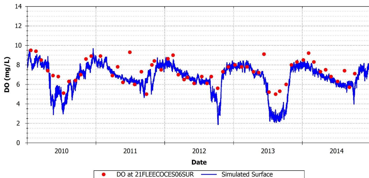
FIGURE 99: SIMULATED AND OBSERVED DO AT 21FLEECOCES06SUR
