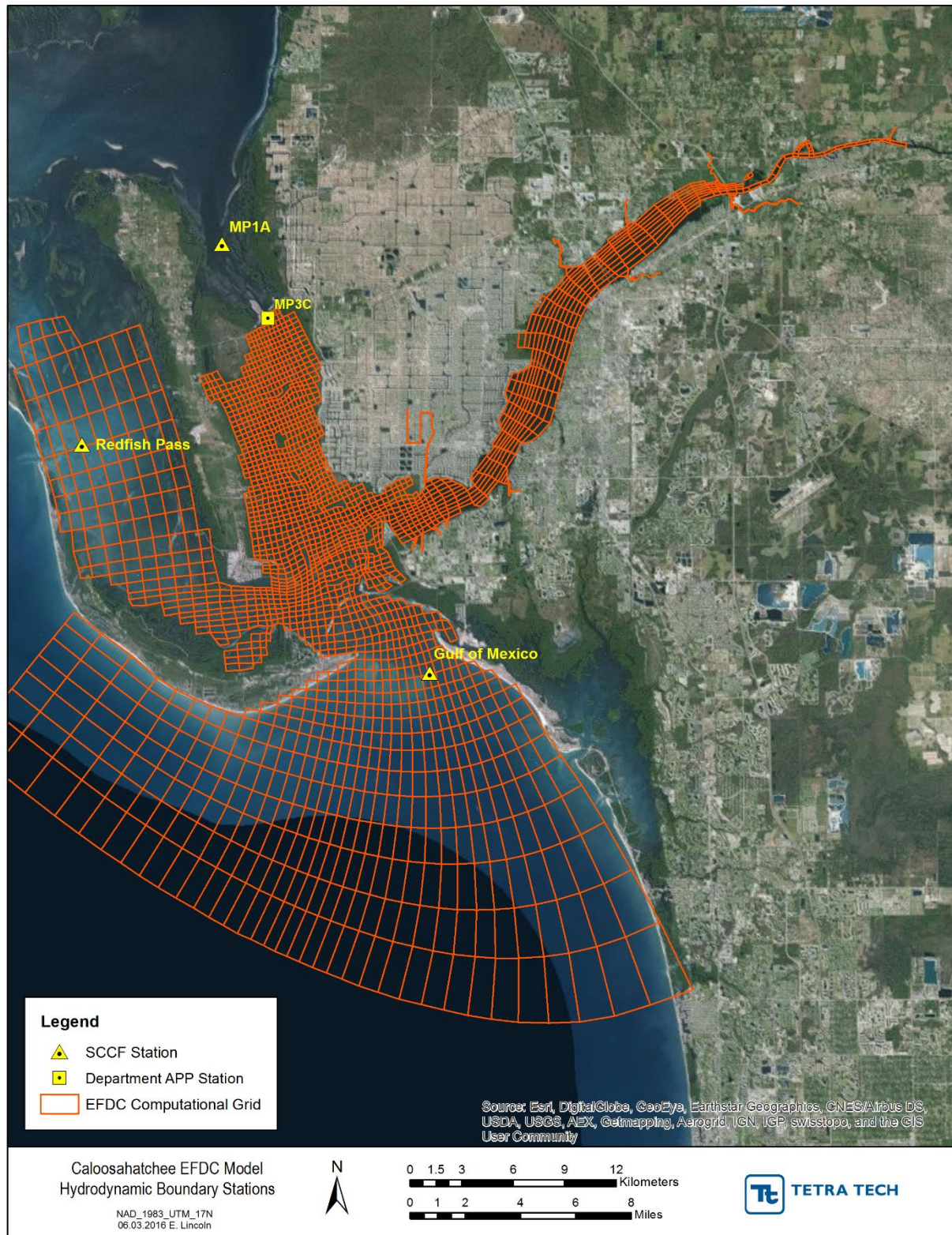
FIGURE 53: 2017 EFDC MODEL OPEN BOUNDARY HYDRODYNAMIC STATION LOCATIONS
