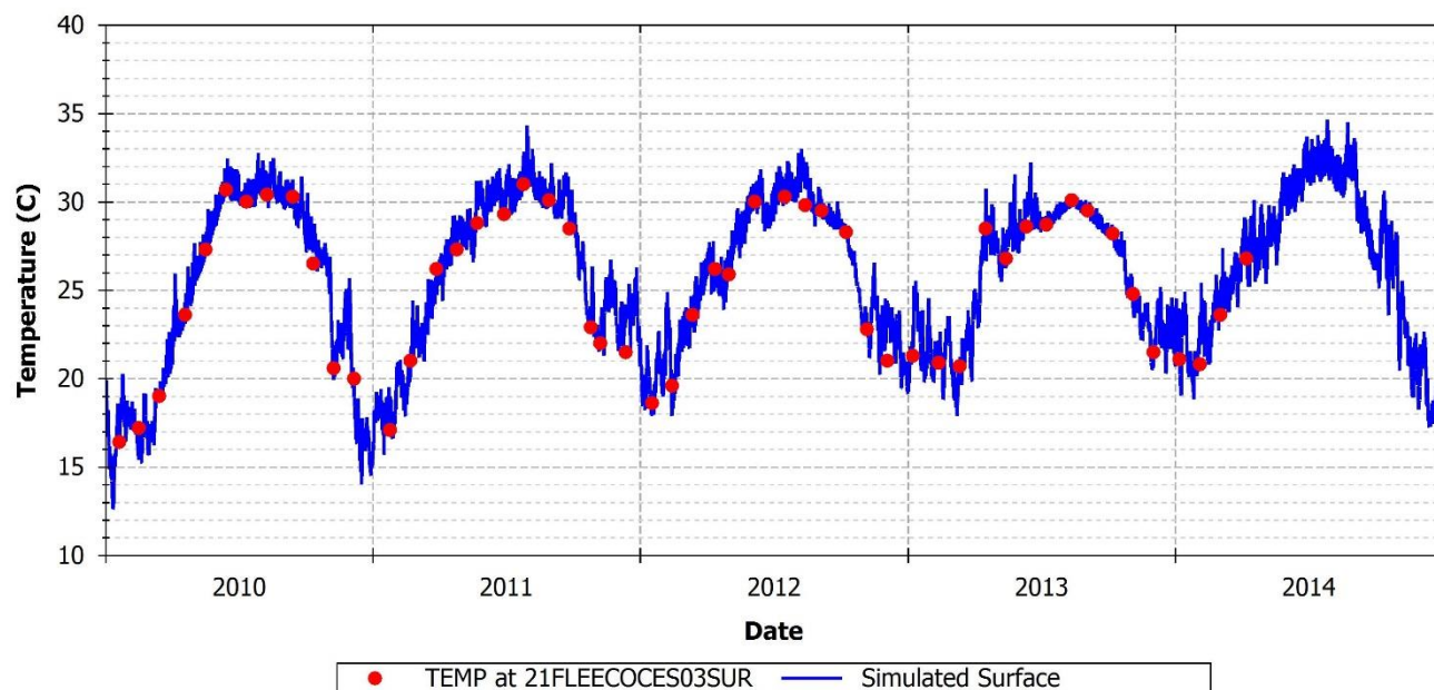
FIGURE 77: SIMULATED AND OBSERVED TEMPERATURE AT 21FLEECOCES03SUR
