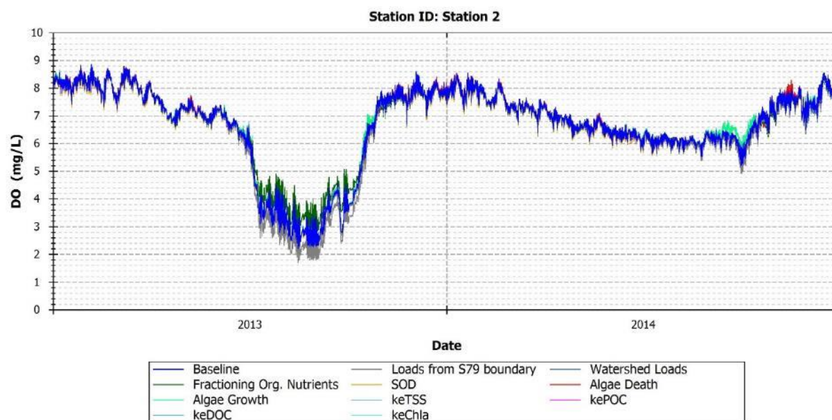
FIGURE 145: MODEL PREDICTIONS OF DO FOR BASELINE AND PERTURBED MODEL CONDITIONS - STATION 2
