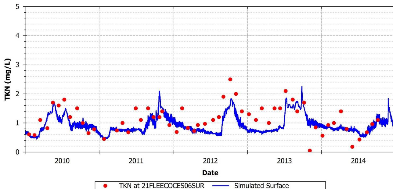
FIGURE 119: SIMULATED AND OBSERVED TKN AT 21FLEECOCES06SUR
