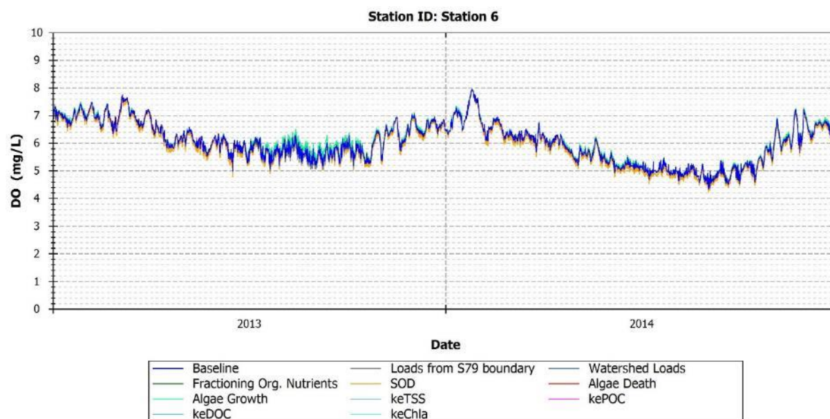
FIGURE 149: MODEL PREDICTIONS OF DO FOR BASELINE AND PERTURBED MODEL CONDITIONS - STATION 6
