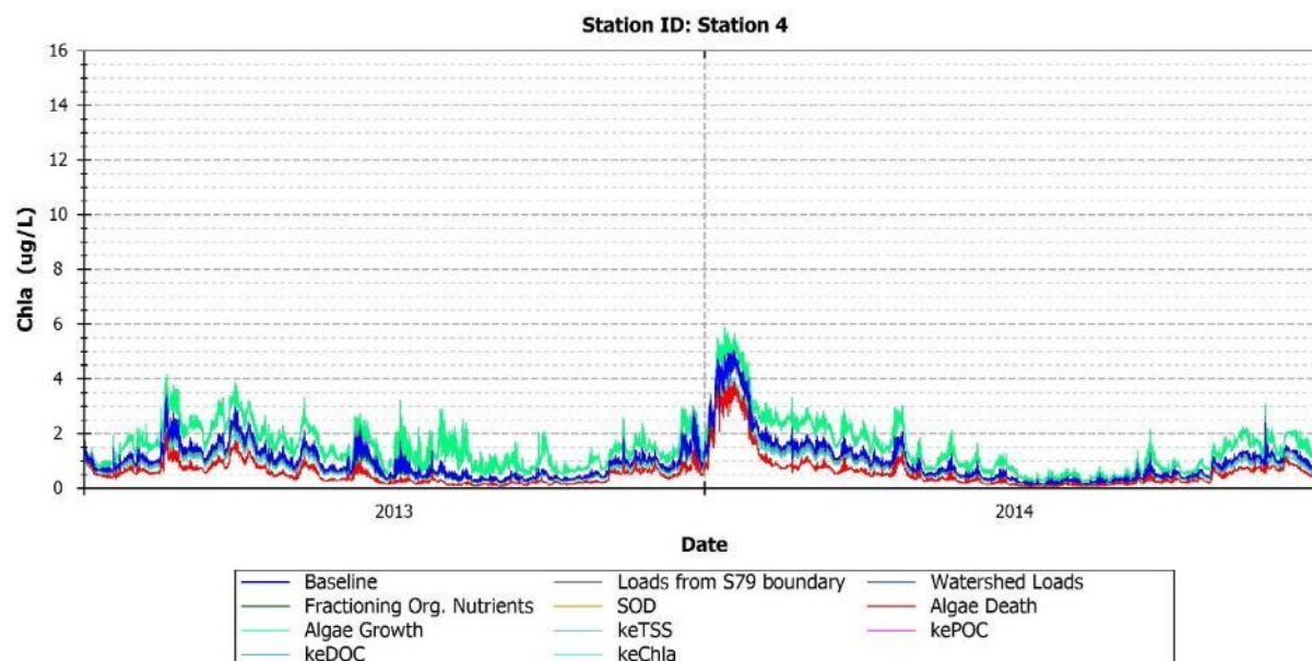
FIGURE 153: MODEL PREDICTIONS OF PHYTOPLANKTON BIOMASS FOR BASELINE AND PERTURBED MODEL CONDITIONS - STATION 4
