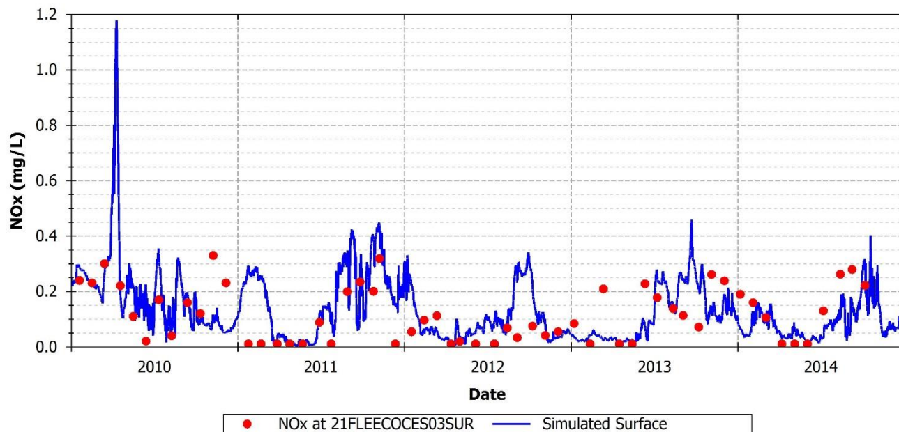
FIGURE 110: SIMULATED AND OBSERVED NO x AT 21FLEECOCES03SUR
