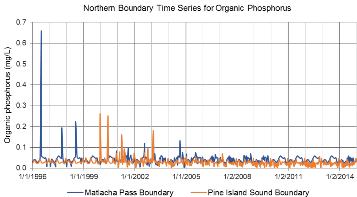
FIGURE 65: NORTHERN BOUNDARY 2017 MODEL INPUT TIME SERIES FOR ORGP (MG/L)
