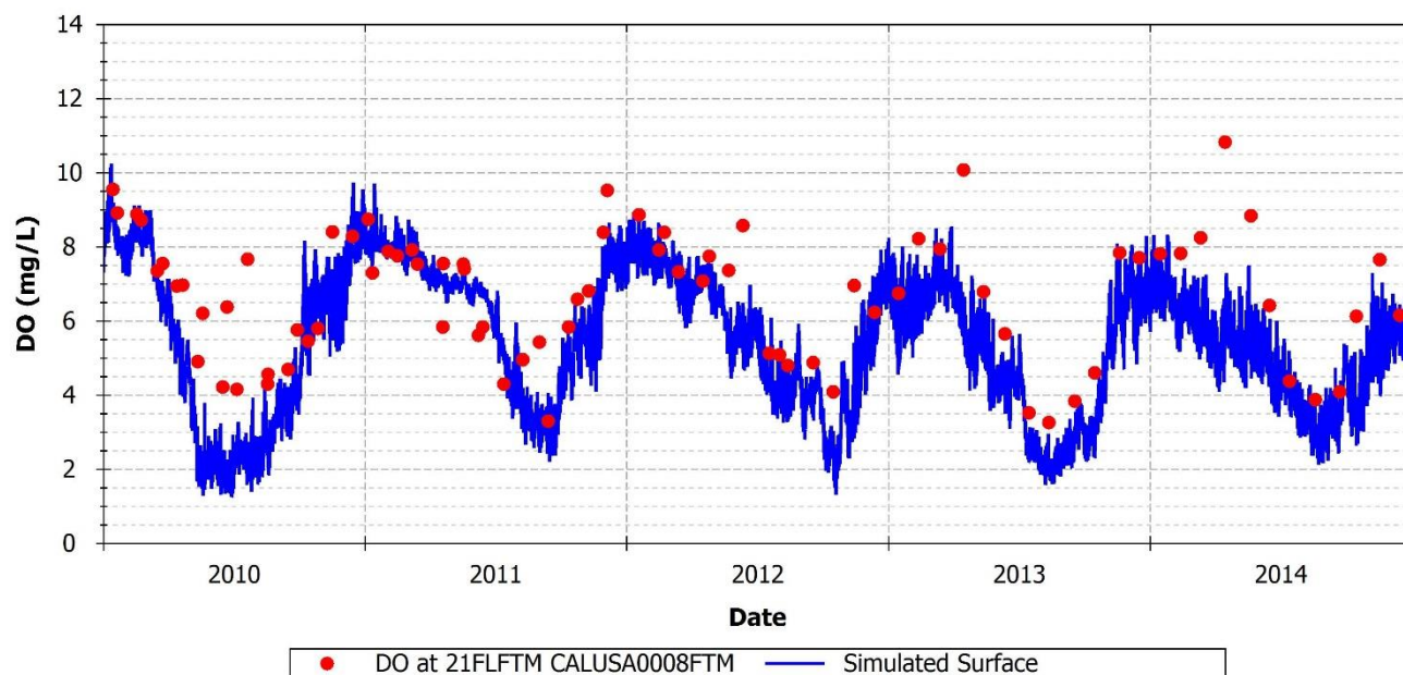
FIGURE 97: SIMULATED AND OBSERVED DO AT 21FLFTM CALUSA0008FTM
