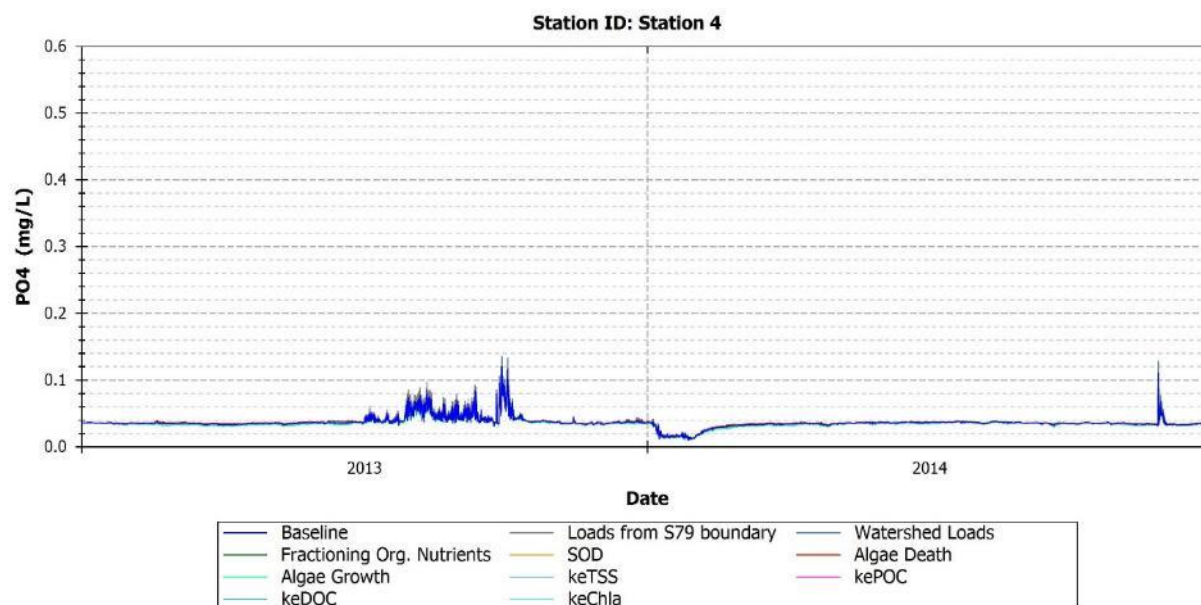
FIGURE 171: MODEL PREDICTIONS OF PO 4 FOR BASELINE AND PERTURBED MODEL CONDITIONS - STATION 4
