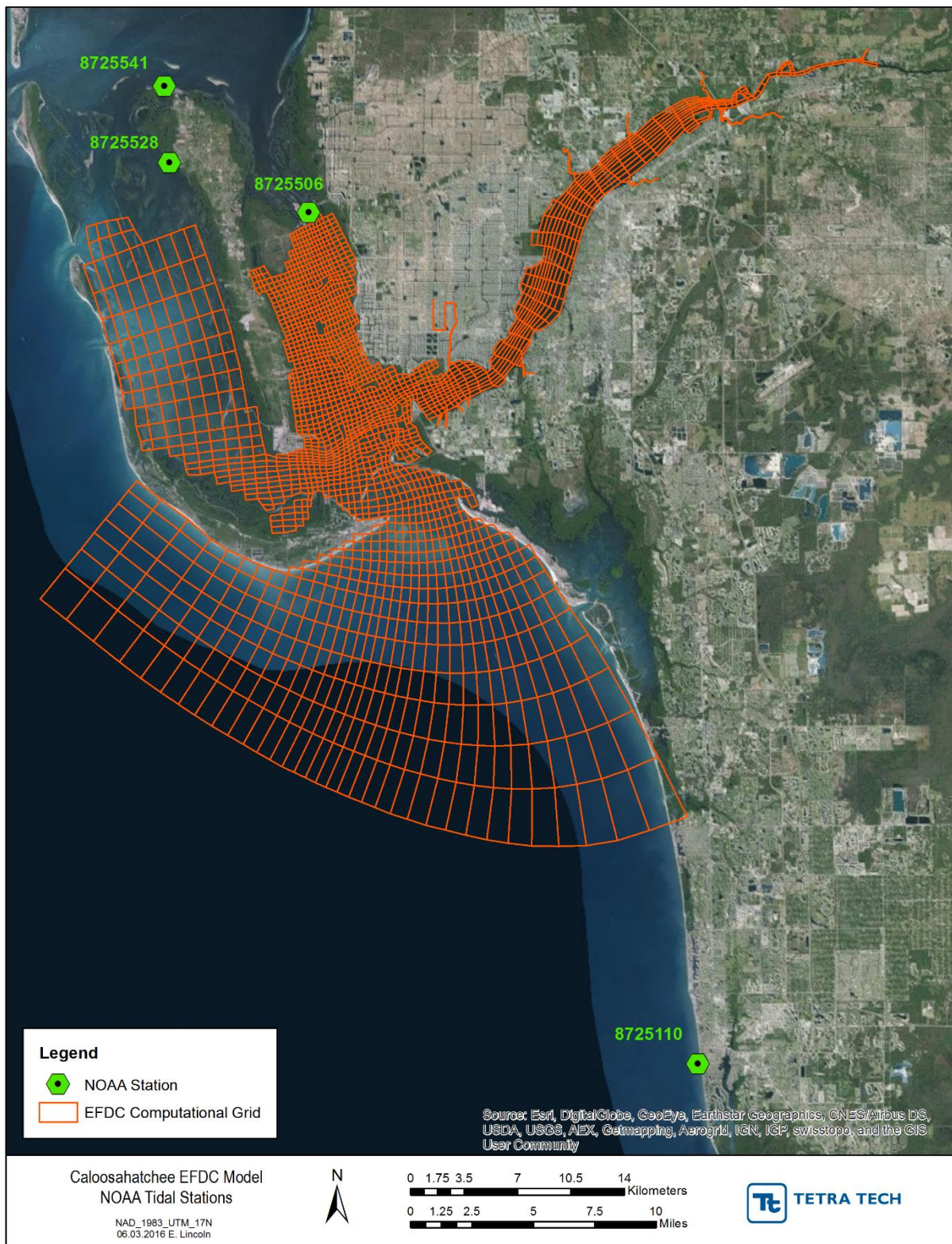
FIGURE 49: 2017 EFDC MODEL WATER SURFACE ELEVATION BOUNDARY STATION LOCATIONS
