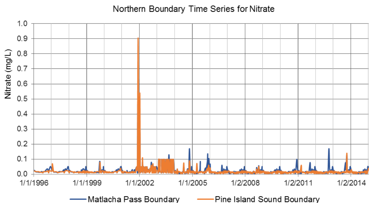
FIGURE 61: NORTHERN BOUNDARY 2017 MODEL INPUT TIME SERIES FOR \text{NO}_3 (MG/L)
