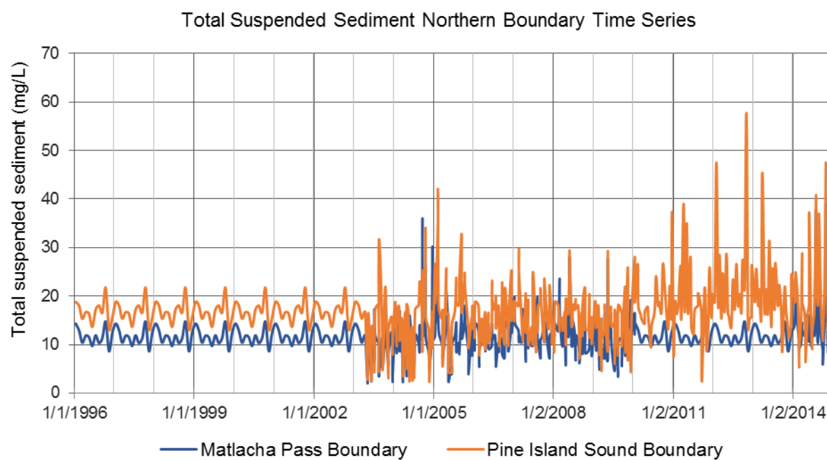
FIGURE 67: NORTHERN BOUNDARY 2017 MODEL INPUT TIME SERIES FOR TSS (MG/L)
