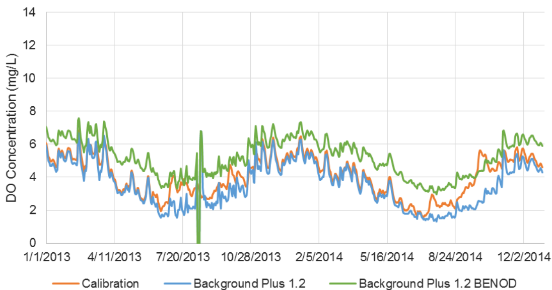
FIGURE 44: 9 MILE CANAL RCHRES 214 DO CONCENTRATION COMPARISON FOR THE CALIBRATION, BACKGROUND PLUS 1.2, AND BACKGROUND PLUS 1.2 BENOD
