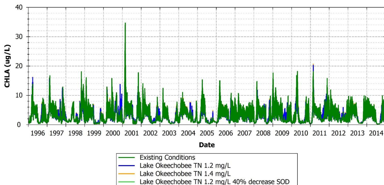
FIGURE 166: PHYTOPLANKTON BIOMASS COMPARISON BETWEEN EXISTING AND SCENARIOS AT 21FLEECOCES10SUR, CALOOSAHATCHEE WATERWAY NEAR MOUTH
