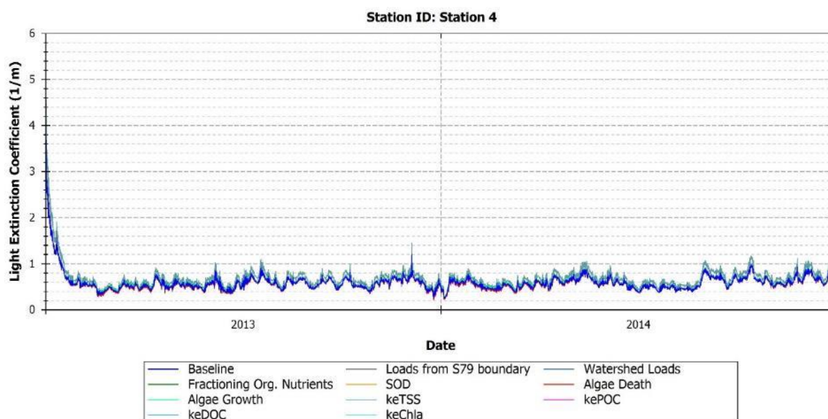
FIGURE 177: MODEL PREDICTIONS OF KE FOR BASELINE AND PERTURBED MODEL CONDITIONS - STATION 4
