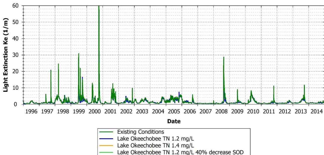
FIGURE 187: LIGHT EXTINCTION COMPARISON BETWEEN EXISTING AND SCENARIOS AT 21FLFTM CALUSA0008FTM, CALOOSAHATCHEE WATERWAY, MARKER 22
