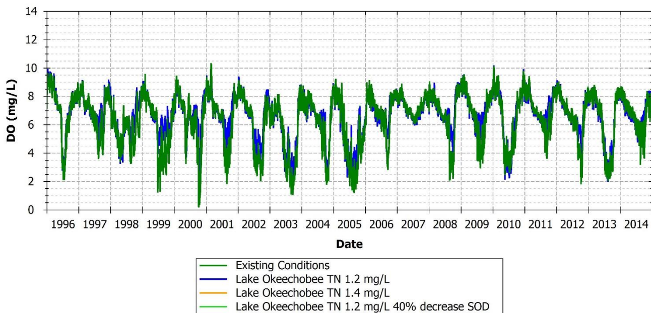
FIGURE 194: DO COMPARISON BETWEEN EXISTING AND SCENARIOS AT 21FLFTM CALUSA0011FTM, CALOOSAHATCHEE WATERWAY, MARKER 52
