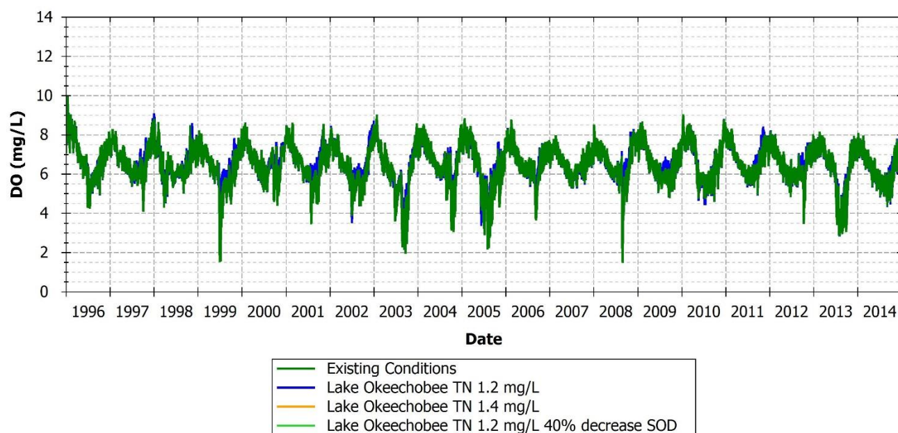
FIGURE 148: DO COMPARISON BETWEEN EXISTING AND SCENARIOS AT 21FLEECOCES10SUR, CALOOSAHATCHEE WATERWAY NEAR MOUTH
