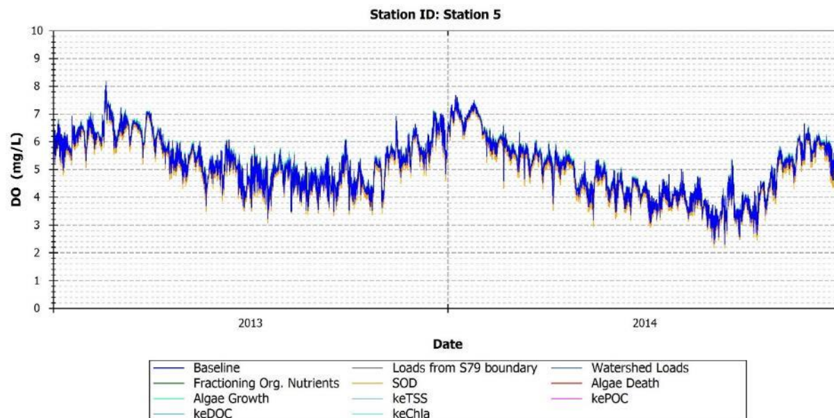
FIGURE 148: MODEL PREDICTIONS OF DO FOR BASELINE AND PERTURBED MODEL CONDITIONS - STATION 5
