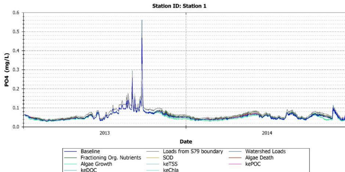
FIGURE 168: MODEL PREDICTIONS OF PO 4 FOR BASELINE AND PERTURBED MODEL CONDITIONS - STATION 1
