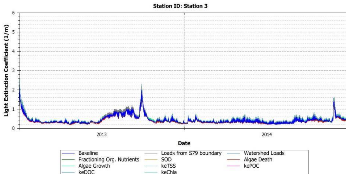
FIGURE 176: MODEL PREDICTIONS OF KE FOR BASELINE AND PERTURBED MODEL CONDITIONS - STATION 3
