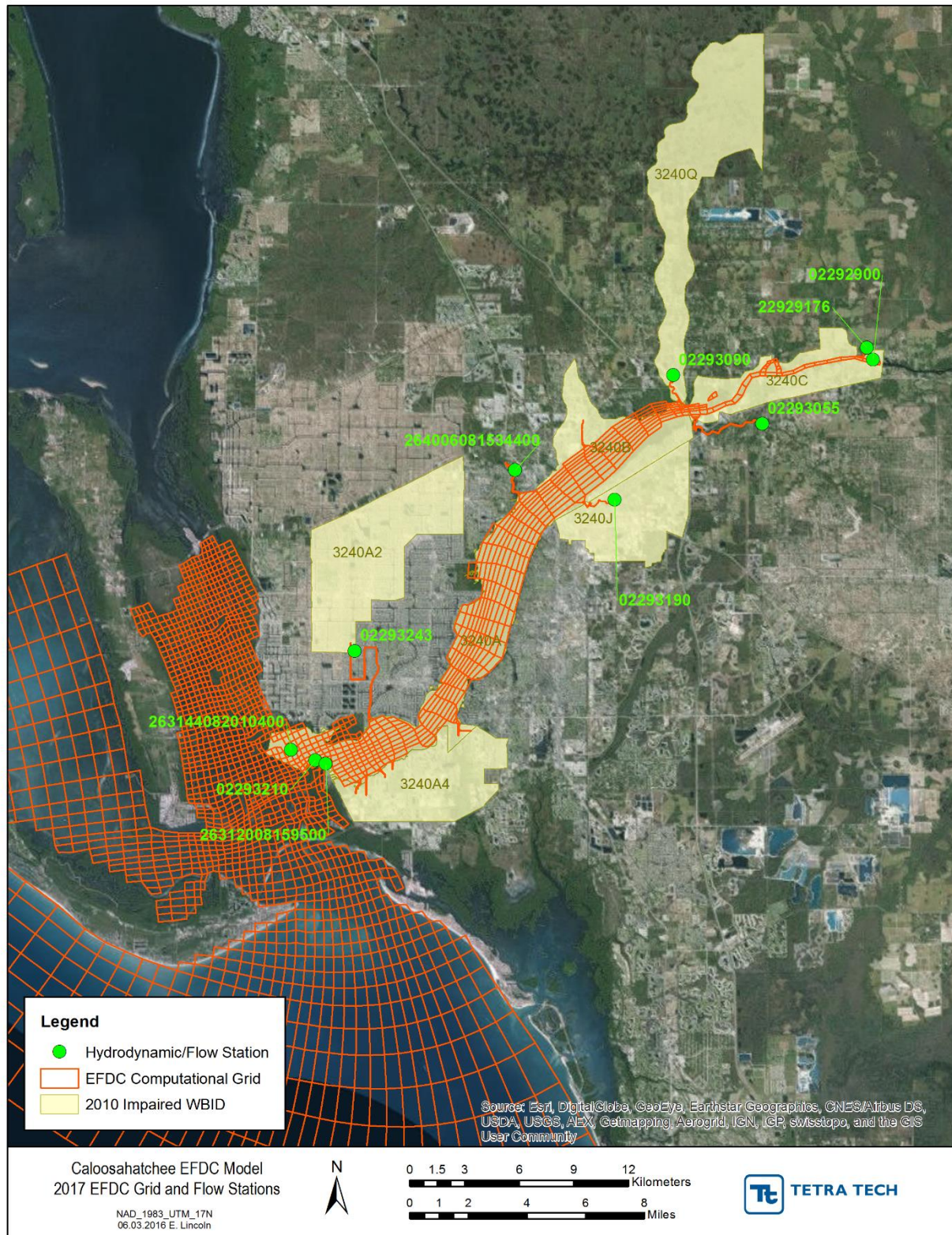
FIGURE 46: 2017 EFDC MODEL GRID TRIBUTARY AND INLET EXTENSION LOCATIONS
