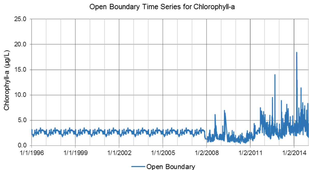
FIGURE 69: SOUTHERN BOUNDARY 2017 MODEL INPUT TIME SERIES FOR CHLOROPHYLL-A (MG/L)
