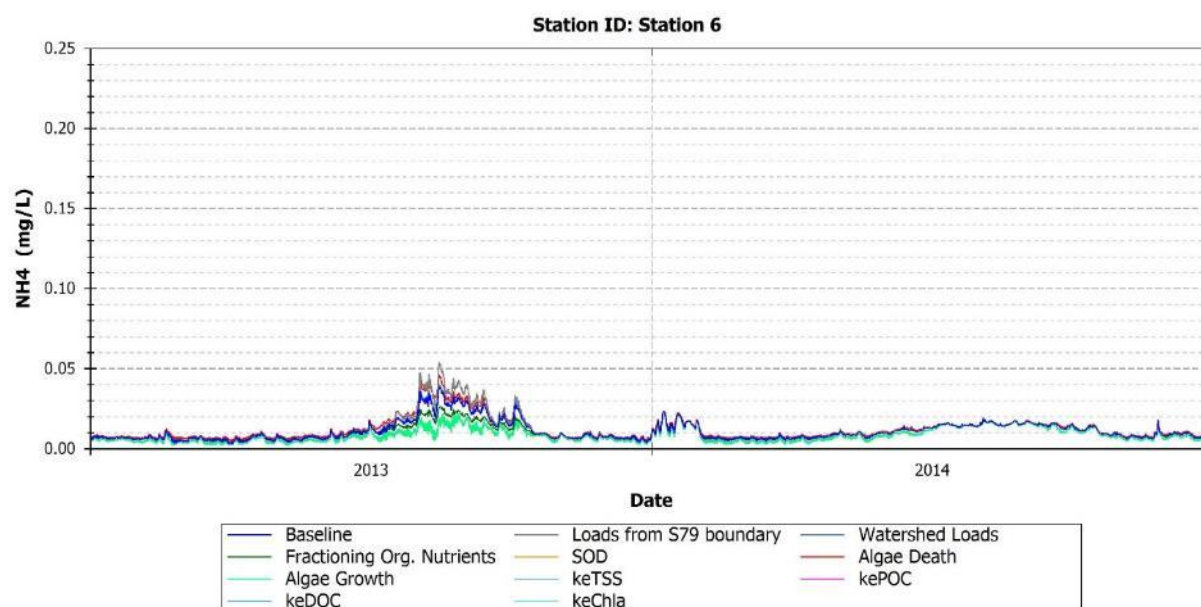
FIGURE 161: MODEL PREDICTIONS OF \text{NH}_4 FOR BASELINE AND PERTURBED MODEL CONDITIONS - STATION 6
