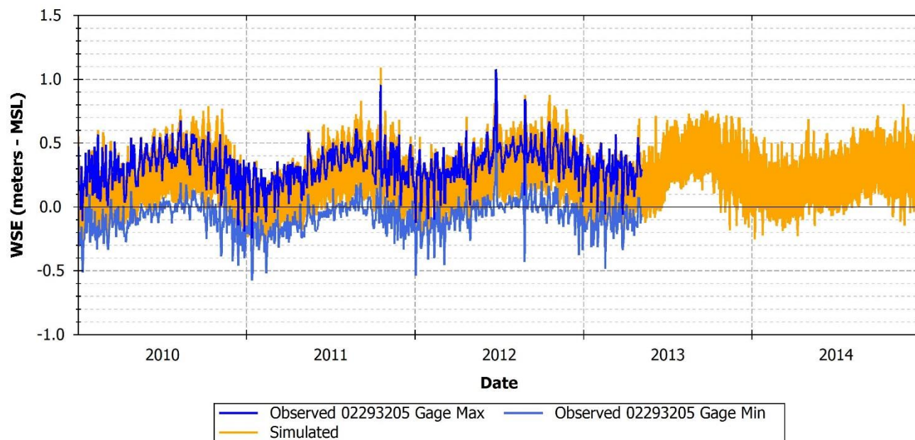
FIGURE 75: SIMULATED AND OBSERVED WSE AT USGS 02293205
