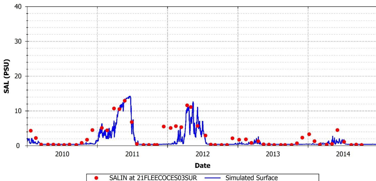
FIGURE 83: SIMULATED AND OBSERVED SALINITY AT 21FLEECOCES03SUR
