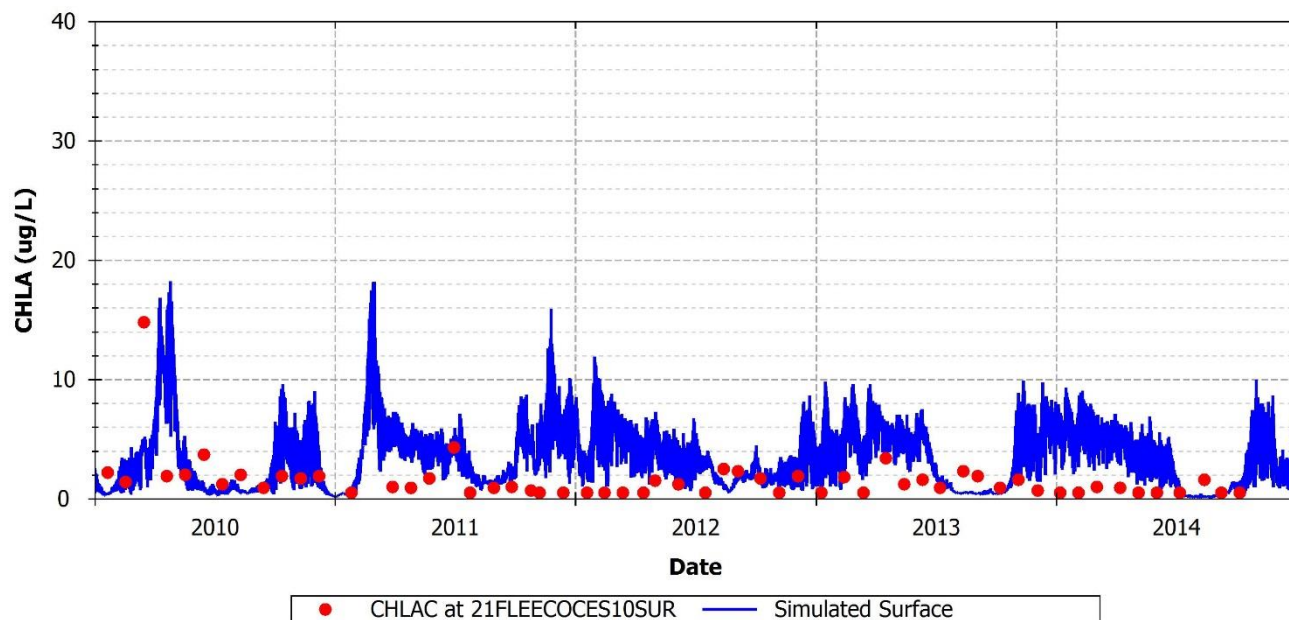
FIGURE 105: SIMULATED AND OBSERVED PHYTOPLANKTON BIOMASS AT 21FLEECOCES10SUR
