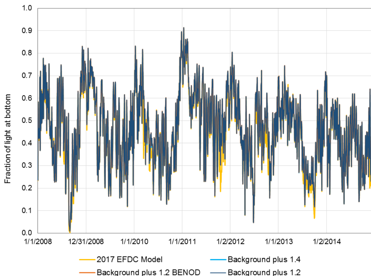
FIGURE 181: FRACTION OF LIGHT REACHING THE BOTTOM IN THE SAN CARLOS BAY REGION UNDER EXISTING CONDITIONS AND UNDER NATURAL CONDITIONS
