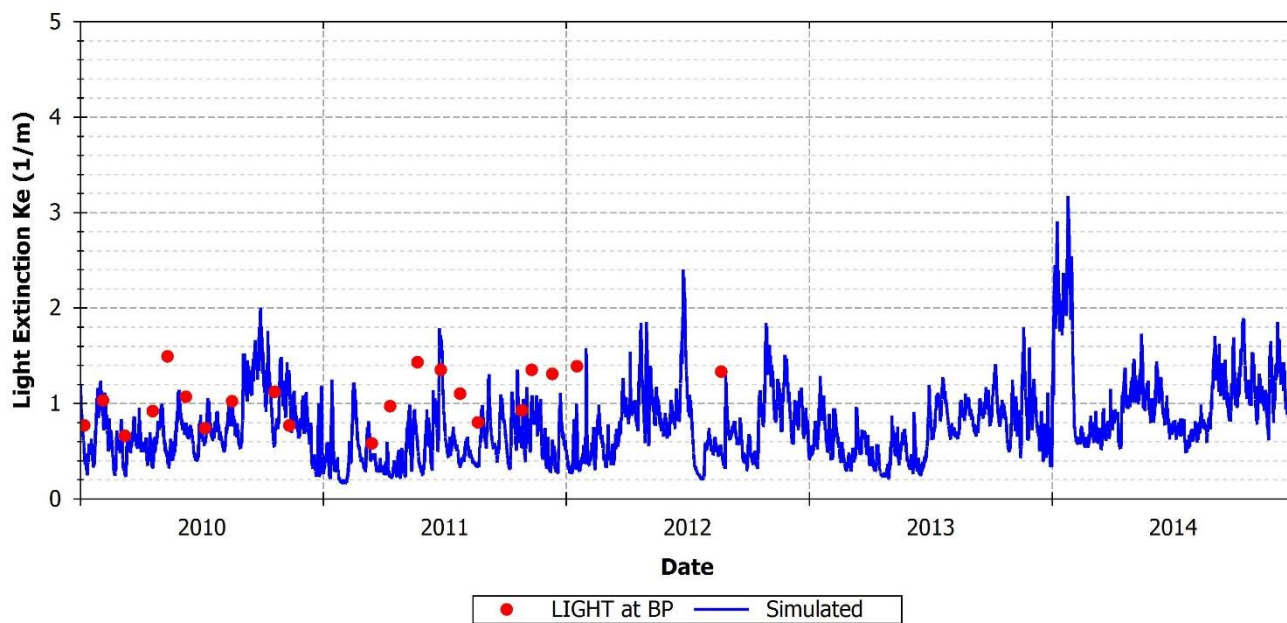
FIGURE 137: OBSERVED VERSUS PREDICTED LIGHT EXTINCTION AT SCCF STATION BP
