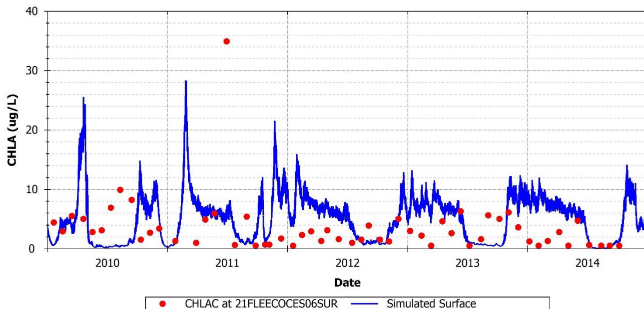
FIGURE 104: SIMULATED AND OBSERVED PHYTOPLANKTON BIOMASS AT 21FLEECOCES06SUR
