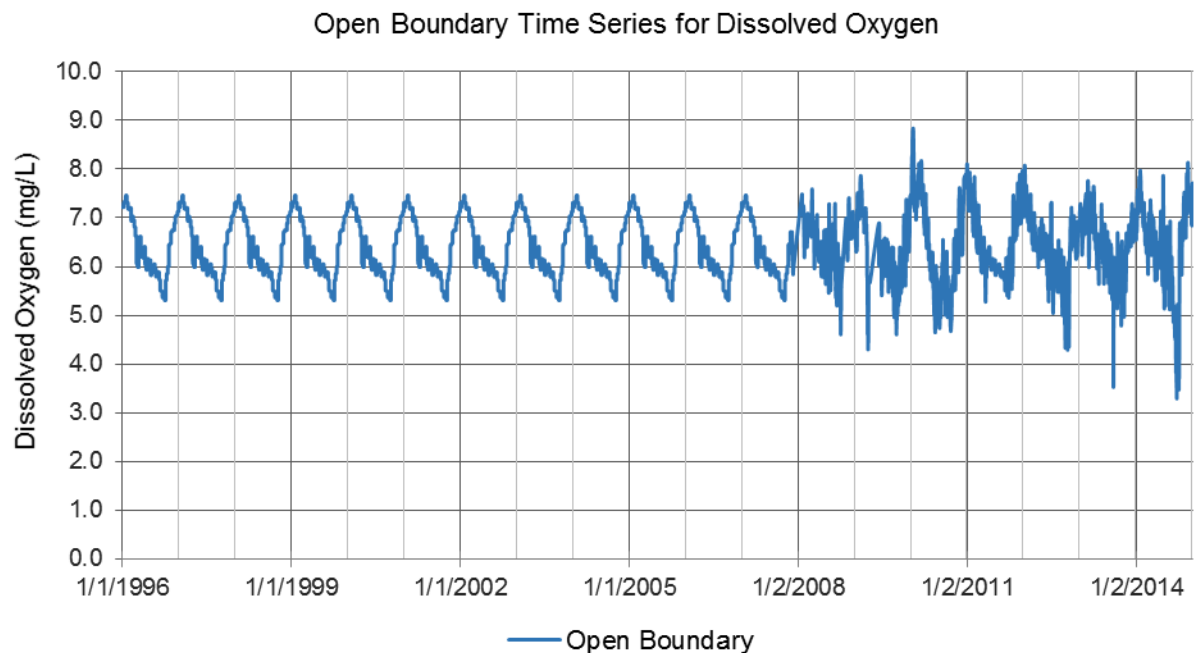
FIGURE 68: SOUTHERN BOUNDARY 2017 MODEL INPUT TIME SERIES FOR DO (MG/L)
