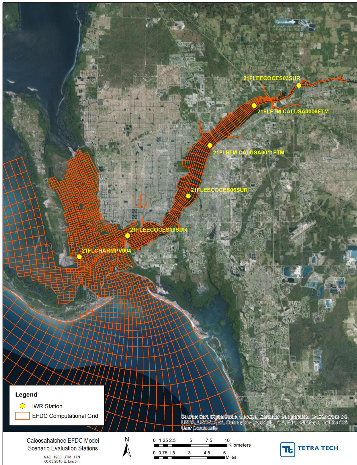
FIGURE 182: SELECTED CELLS FOR LIGHT, DO, AND NUTRIENT CONCENTRATION ANALYSES
