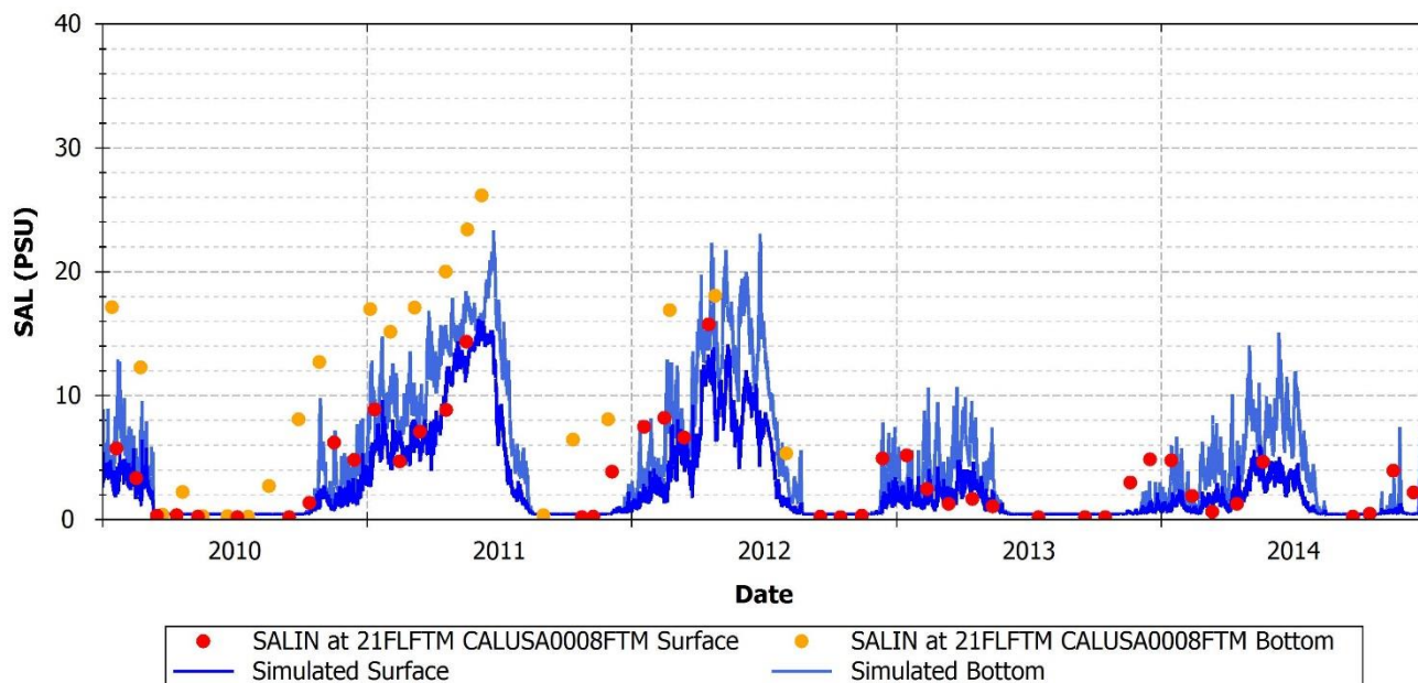
FIGURE 84: SIMULATED AND OBSERVED SALINITY AT 21FLFTM CALUSA0008FTM
