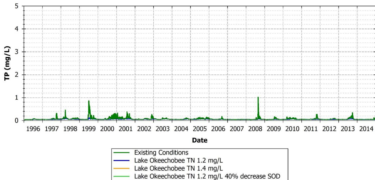
Figure 157: TP Comparison between Existing and Scenarios at 21CHARMPV004, Matlacha Pass
