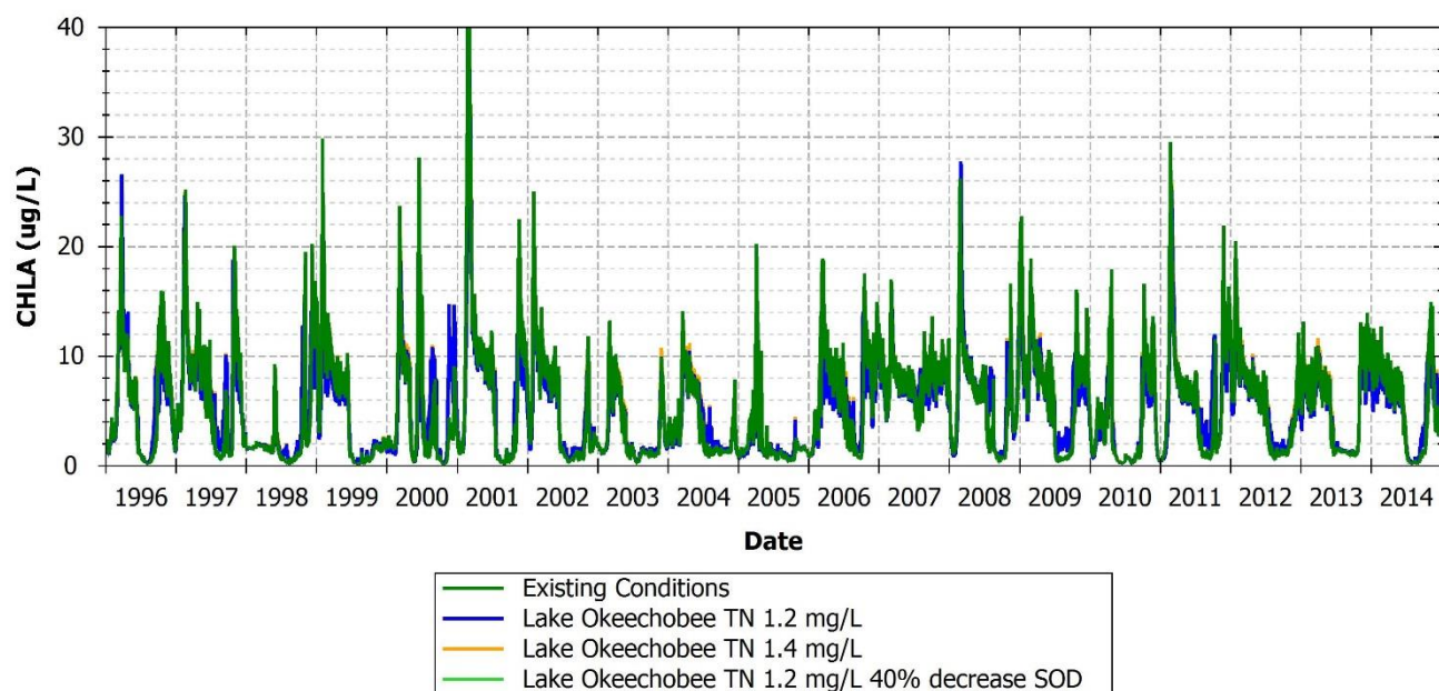
FIGURE 168: PHYTOPLANKTON BIOMASS COMPARISON BETWEEN EXISTING AND SCENARIOS AT 21FLFTM CALUSA0011FTM, CALOOSAHATCHEE WATERWAY, MARKER 52
