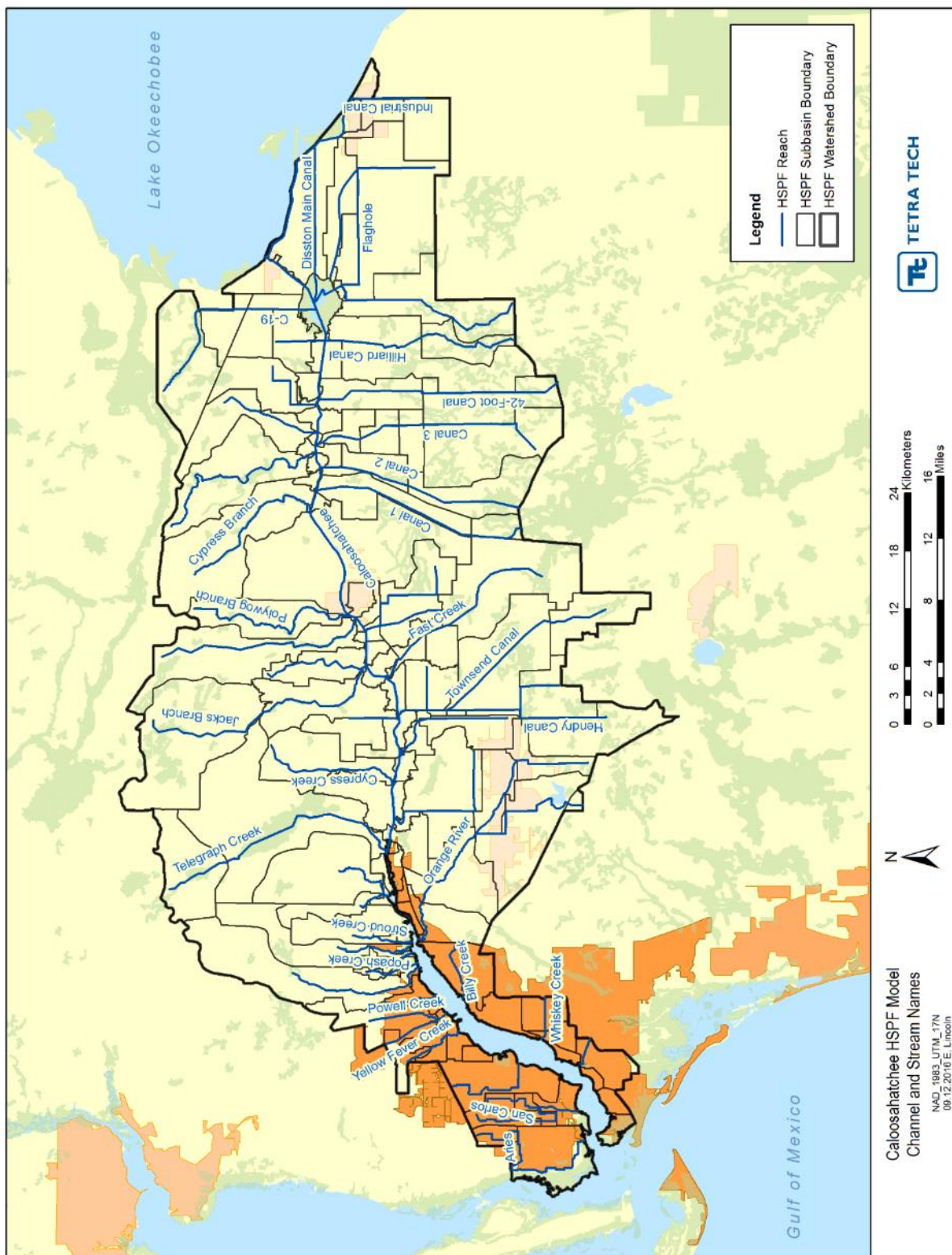
FIGURE 7: 2017 HSPF MODEL MAJOR CANAL AND STREAM NAMES
