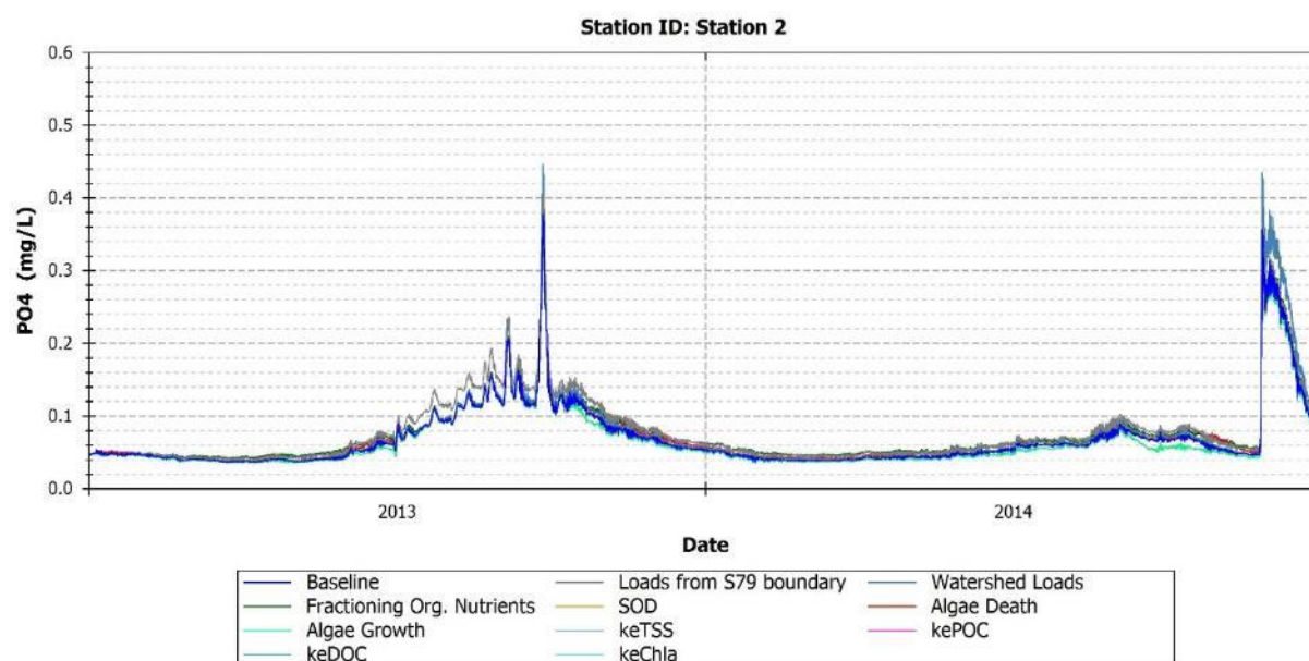
FIGURE 169: MODEL PREDICTIONS OF PO 4 FOR BASELINE AND PERTURBED MODEL CONDITIONS - STATION 2
