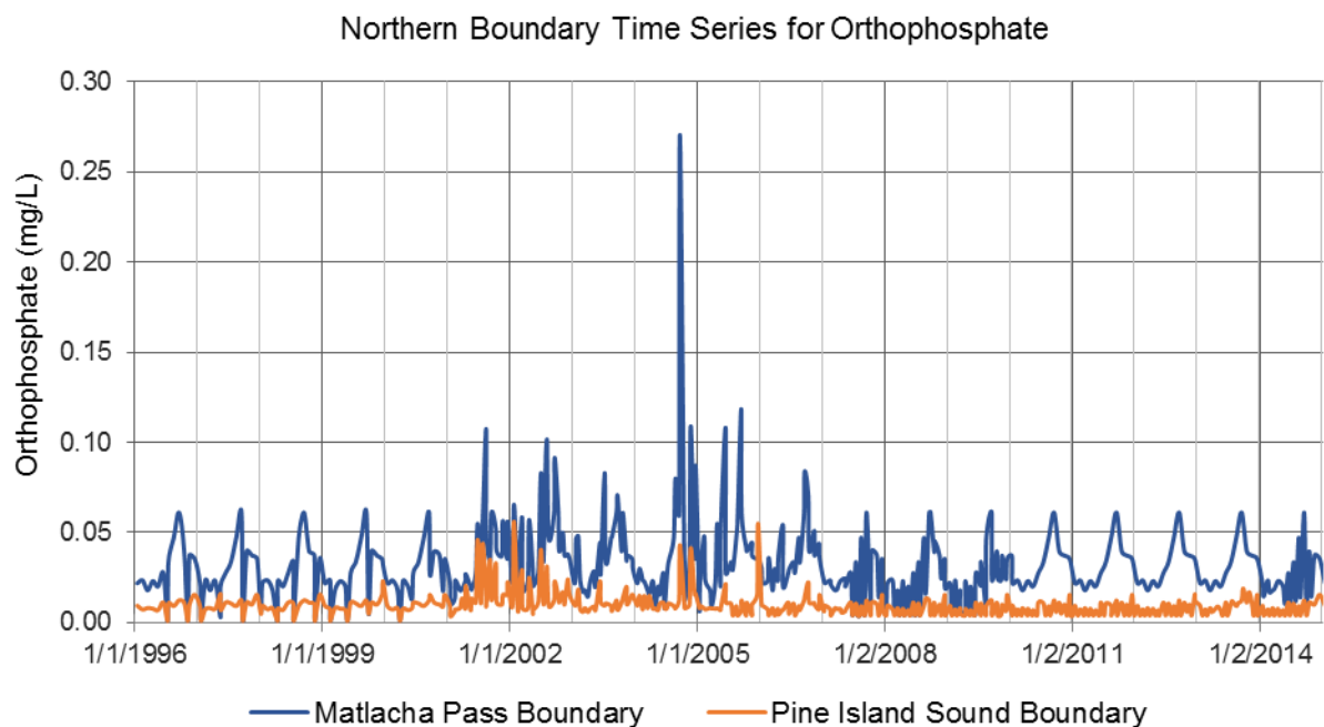
FIGURE 64: NORTHERN BOUNDARY 2017 MODEL INPUT TIME SERIES FOR \text{PO}_4 (MG/L)
