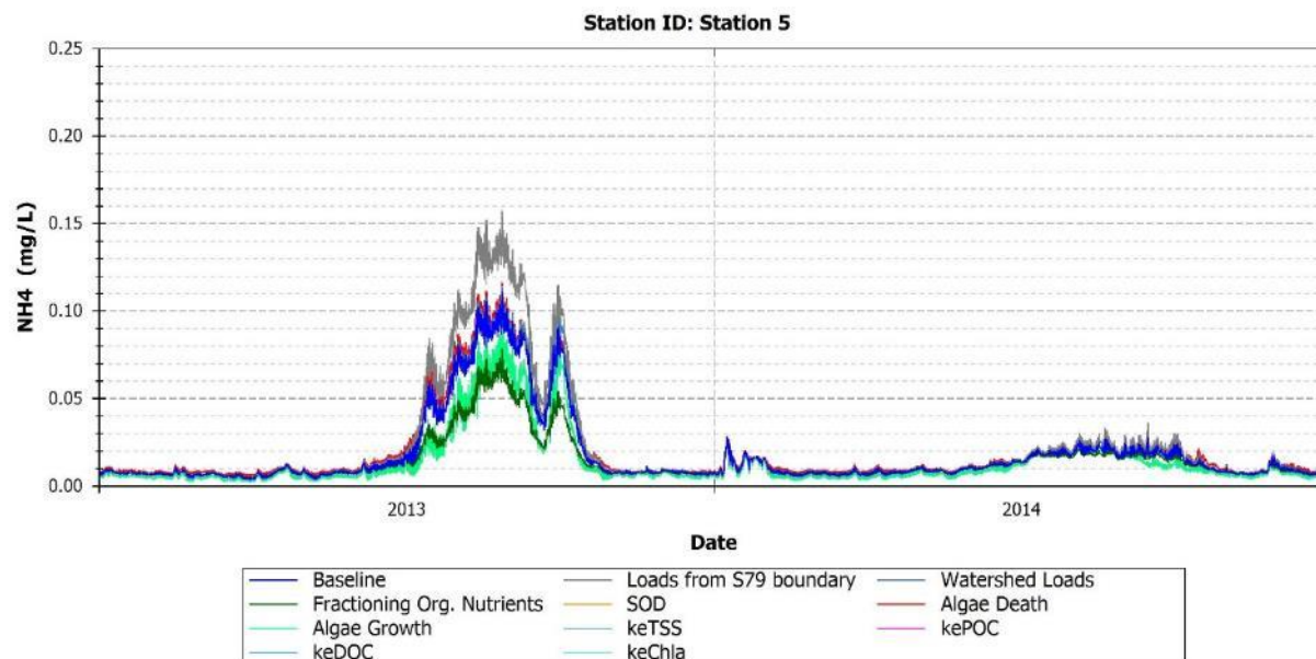
FIGURE 160: MODEL PREDICTIONS OF \text{NH}_4 FOR BASELINE AND PERTURBED MODEL CONDITIONS - STATION 5
