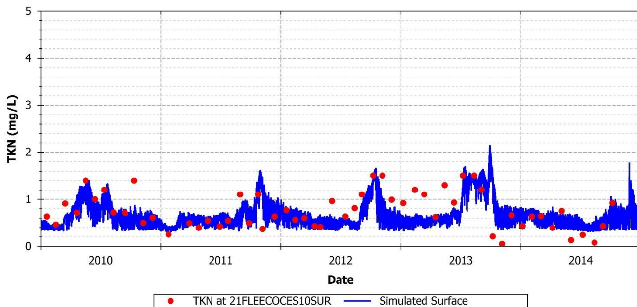
FIGURE 120: SIMULATED AND OBSERVED TKN AT 21FLEECOCES10SUR
