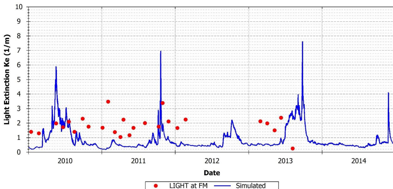
FIGURE 138: OBSERVED VERSUS PREDICTED LIGHT EXTINCTION AT SCCF STATION FM
