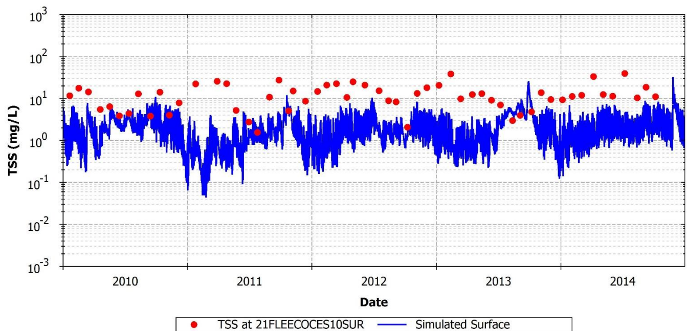
FIGURE 128: SIMULATED AND OBSERVED TSS AT 21FLEECOCES10SUR
