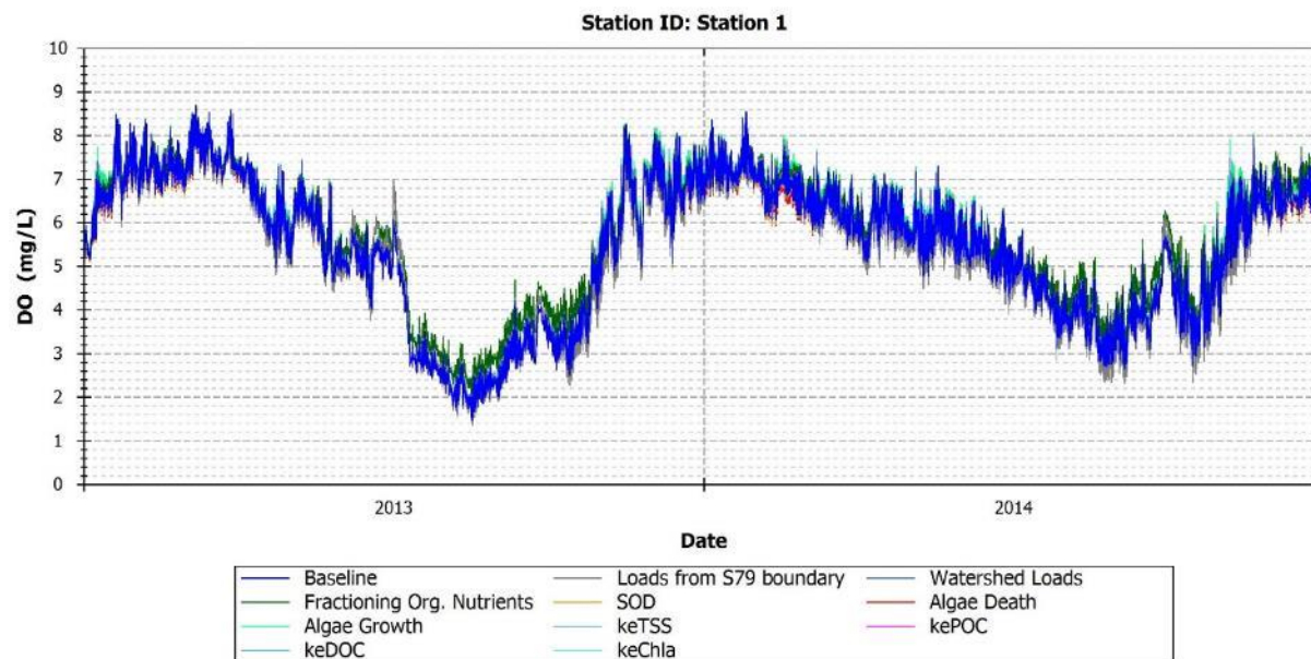
FIGURE 144: MODEL PREDICTIONS OF DO FOR BASELINE AND PERTURBED MODEL CONDITIONS - STATION 1
