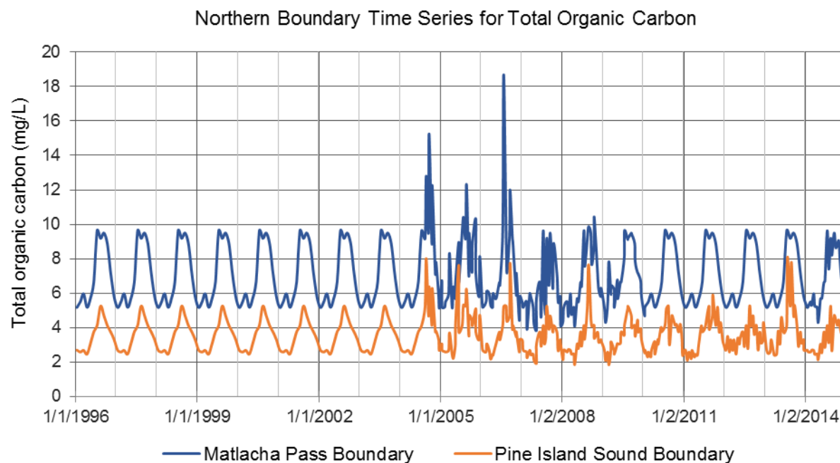
FIGURE 66: NORTHERN BOUNDARY 2017 MODEL INPUT TIME SERIES FOR TOC (MG/L)
