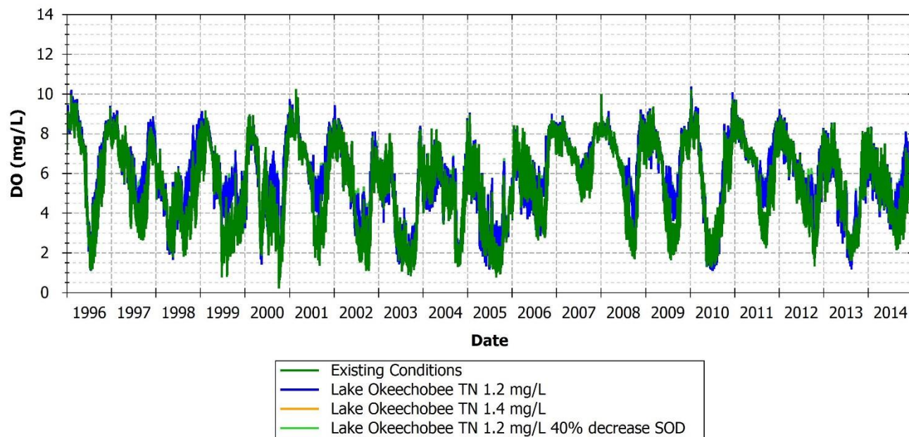
FIGURE 149: DO COMPARISON BETWEEN EXISTING AND SCENARIOS AT 21FLFTM CALUSA0008FTM, CALOOSAHATCHEE WATERWAY, MARKER 22
