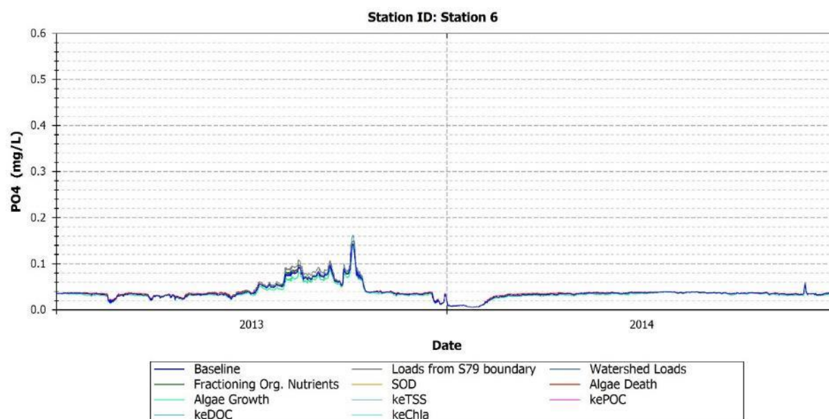
FIGURE 173: MODEL PREDICTIONS OF PO 4 FOR BASELINE AND PERTURBED MODEL CONDITIONS - STATION 6
