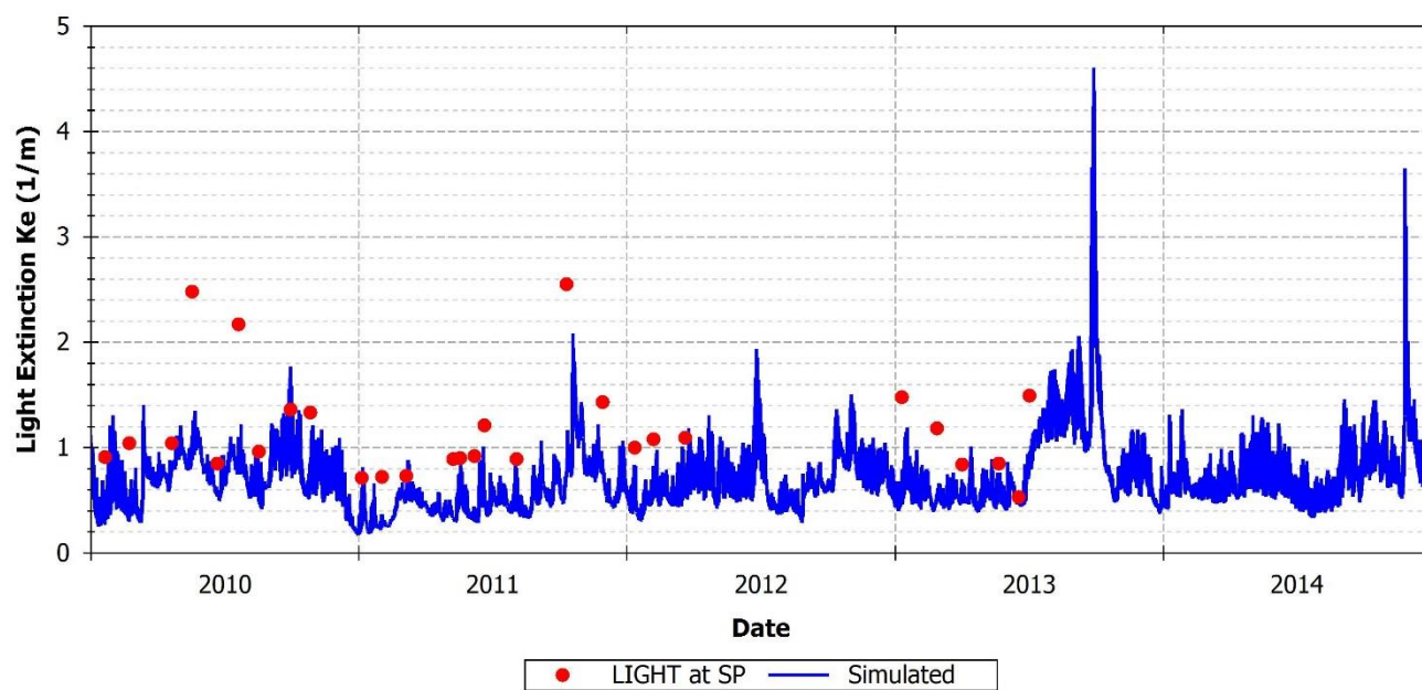
FIGURE 141: OBSERVED VERSUS PREDICTED LIGHT EXTINCTION AT SCCF STATION SP
