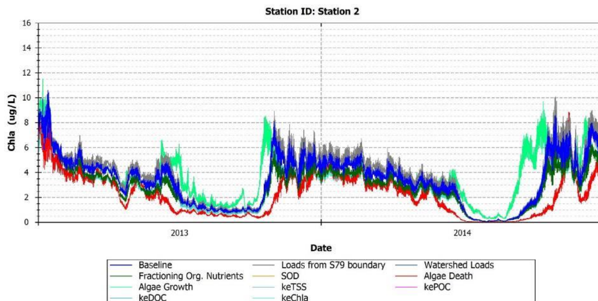
FIGURE 151: MODEL PREDICTIONS OF PHYTOPLANKTON BIOMASS FOR BASELINE AND PERTURBED MODEL CONDITIONS - STATION 2
