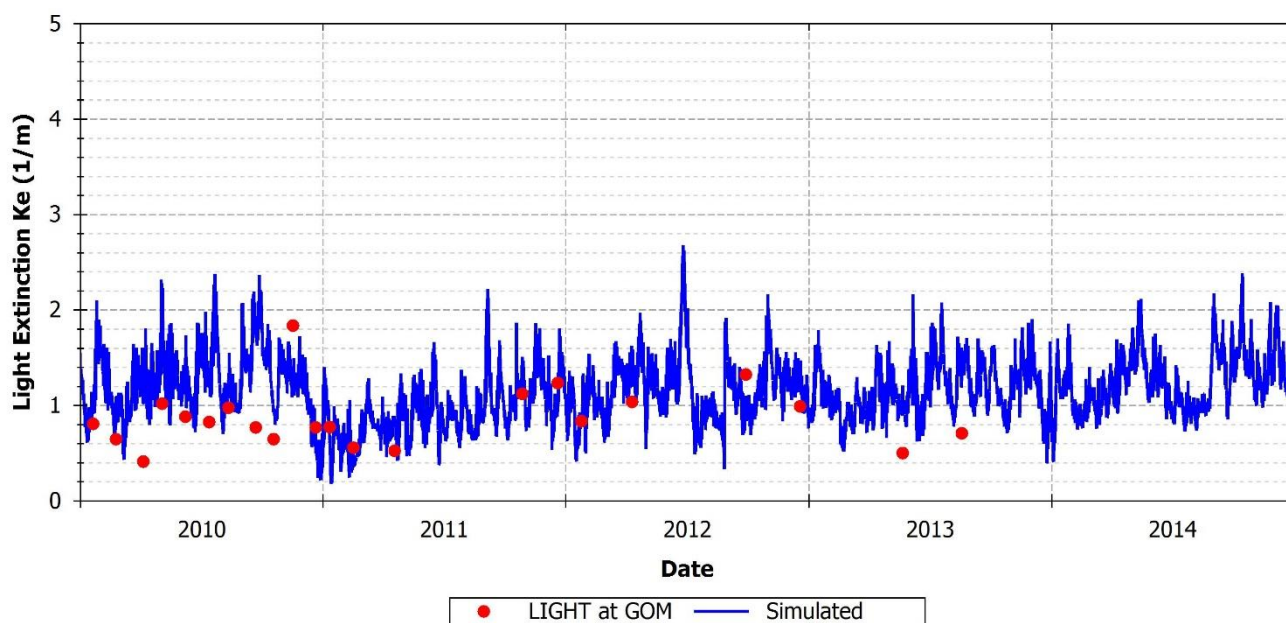
FIGURE 139: OBSERVED VERSUS PREDICTED LIGHT EXTINCTION AT SCCF STATION GULF OF MEXICO
