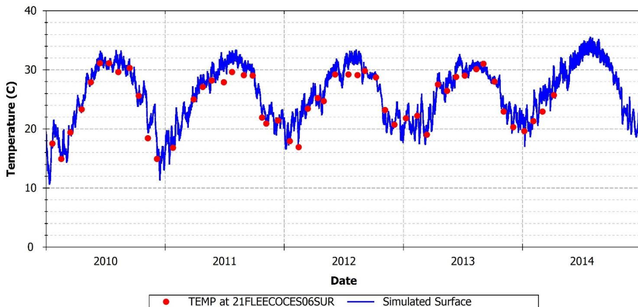
FIGURE 80: SIMULATED AND OBSERVED TEMPERATURE AT 21FLEECOCES06SUR
