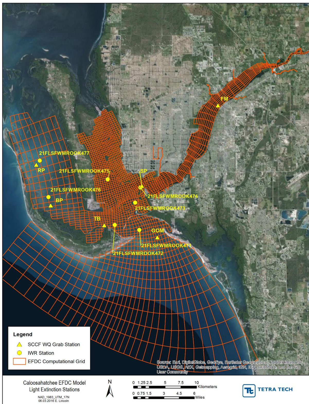
FIGURE 129: MONITORING STATIONS WITH MEASUREMENTS OF LIGHT EXTINCTION
