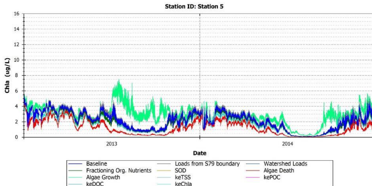
FIGURE 154: MODEL PREDICTIONS OF PHYTOPLANKTON BIOMASS FOR BASELINE AND PERTURBED MODEL CONDITIONS - STATION 5
