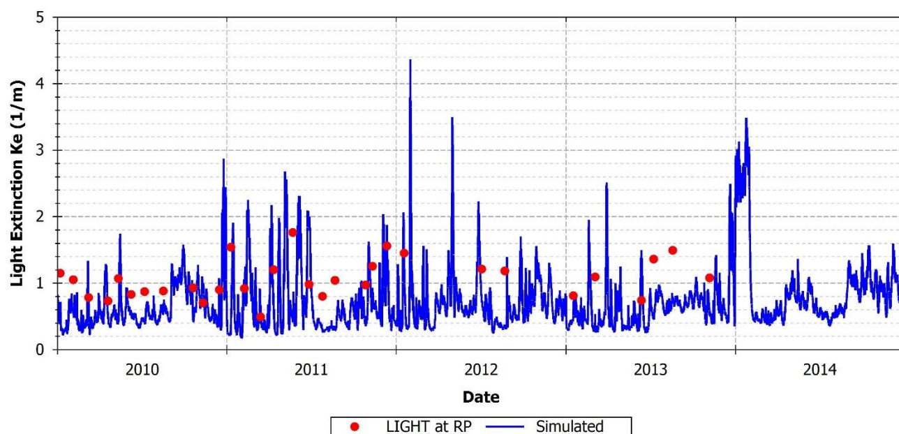
FIGURE 140: OBSERVED VERSUS PREDICTED LIGHT EXTINCTION AT SCCF STATION REDFISH PASS
