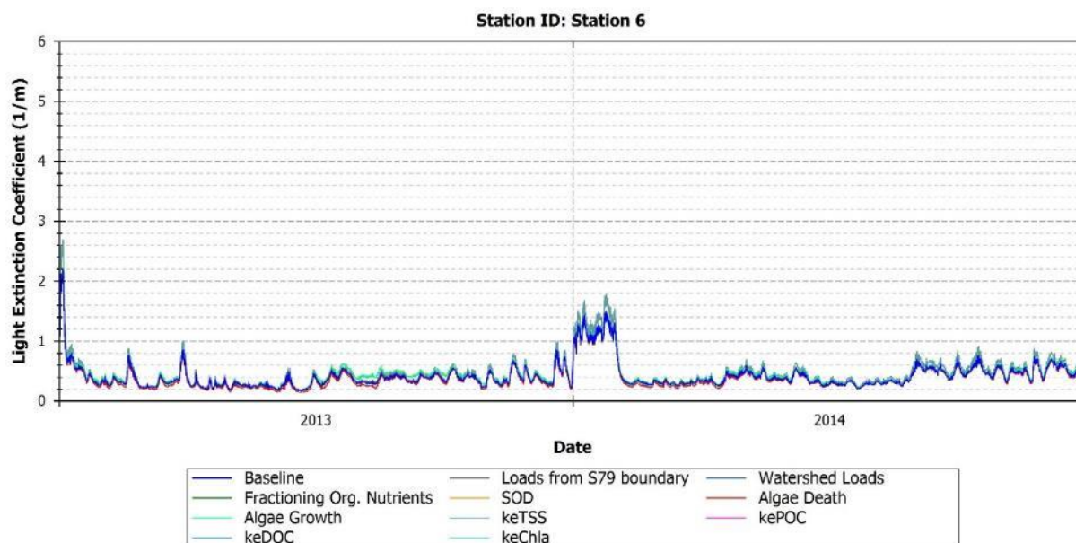
FIGURE 179: MODEL PREDICTIONS OF KE FOR BASELINE AND PERTURBED MODEL CONDITIONS - STATION 6
