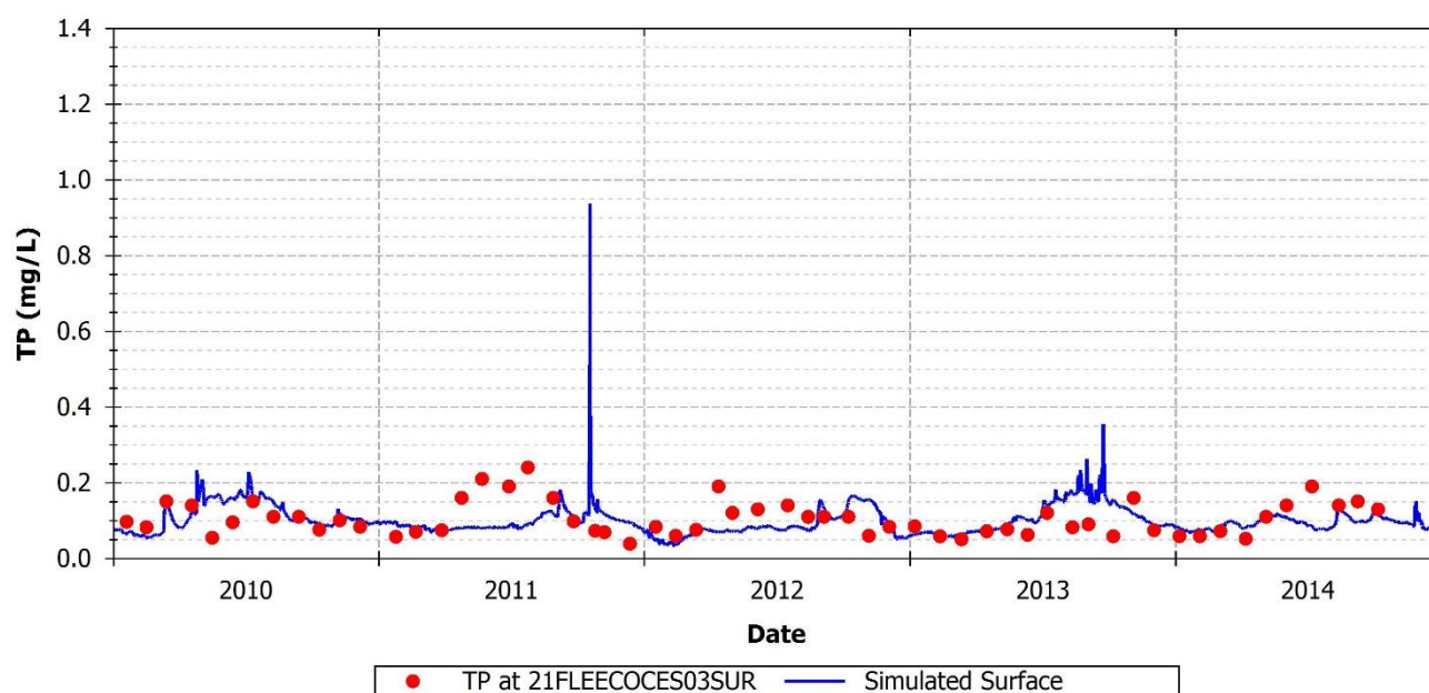
FIGURE 121: SIMULATED AND OBSERVED TP AT 21FLEECOCES03SUR
