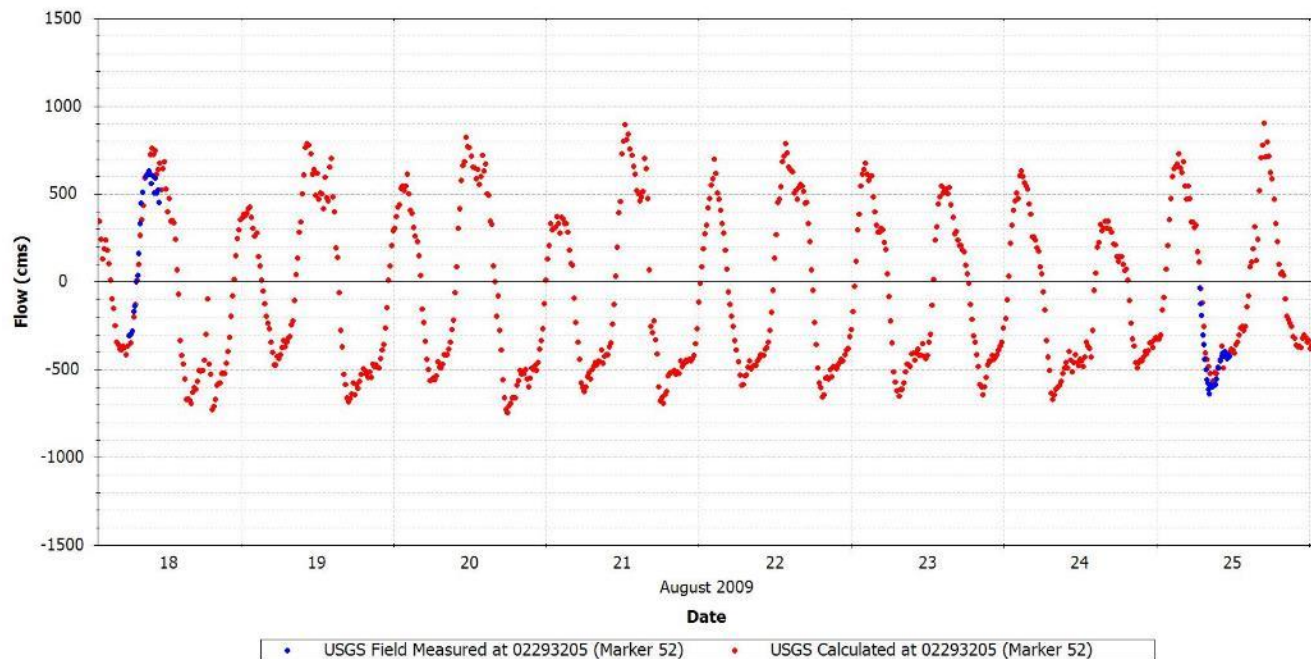
FIGURE 89: COMPARISON OF FLOWS MEASURED AND CALCULATED BY USGS AT STATION 02293205
