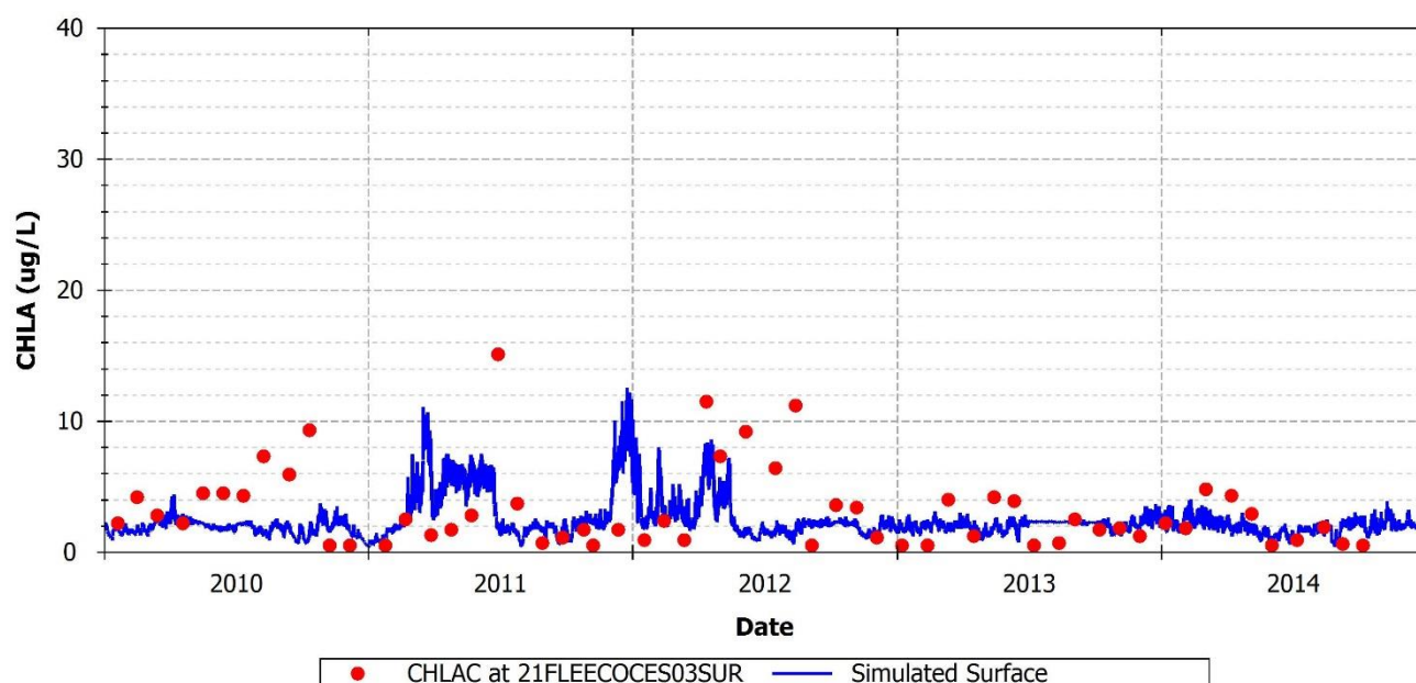
FIGURE 101: SIMULATED AND OBSERVED PHYTOPLANKTON BIOMASS AT 21FLEECOCES03SUR
