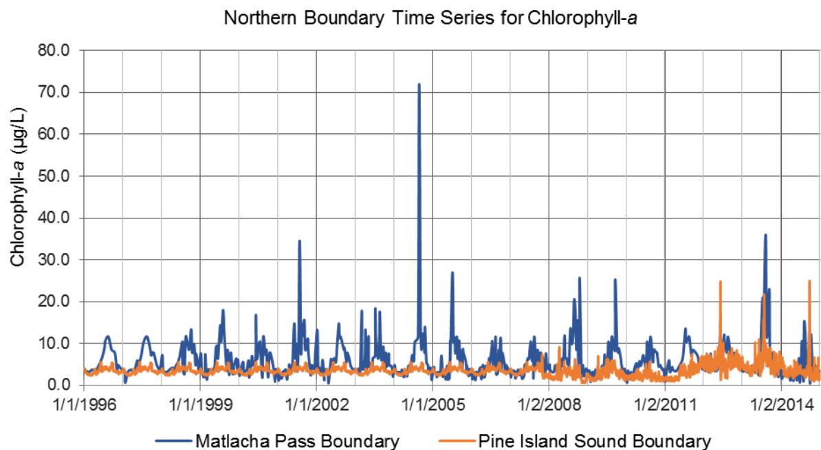
FIGURE 60: NORTHERN BOUNDARY 2017 MODEL INPUT TIME SERIES FOR CHLOROPHYLL-A (MG/L)
