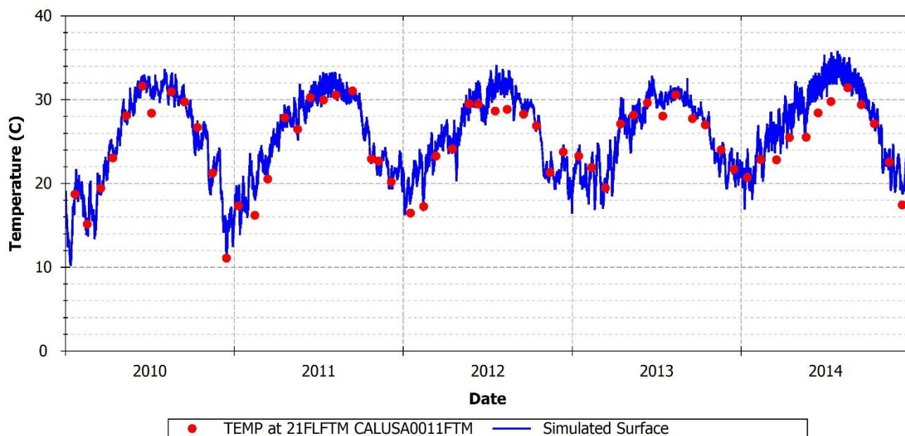
FIGURE 79: SIMULATED AND OBSERVED TEMPERATURE AT 21FLFTM CALUSA0011FTM
