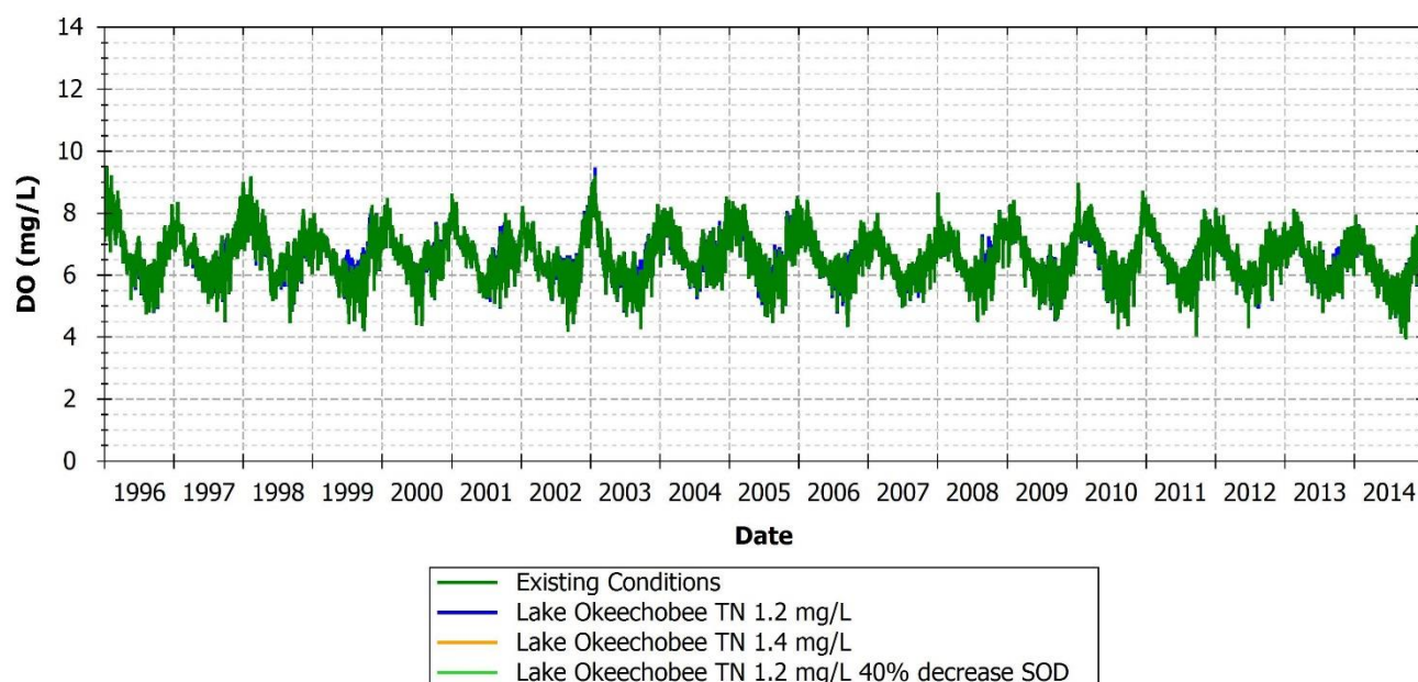
FIGURE 189: DO COMPARISON BETWEEN EXISTING AND SCENARIOS AT 21CHARMPV004, MATLACHA PASS
