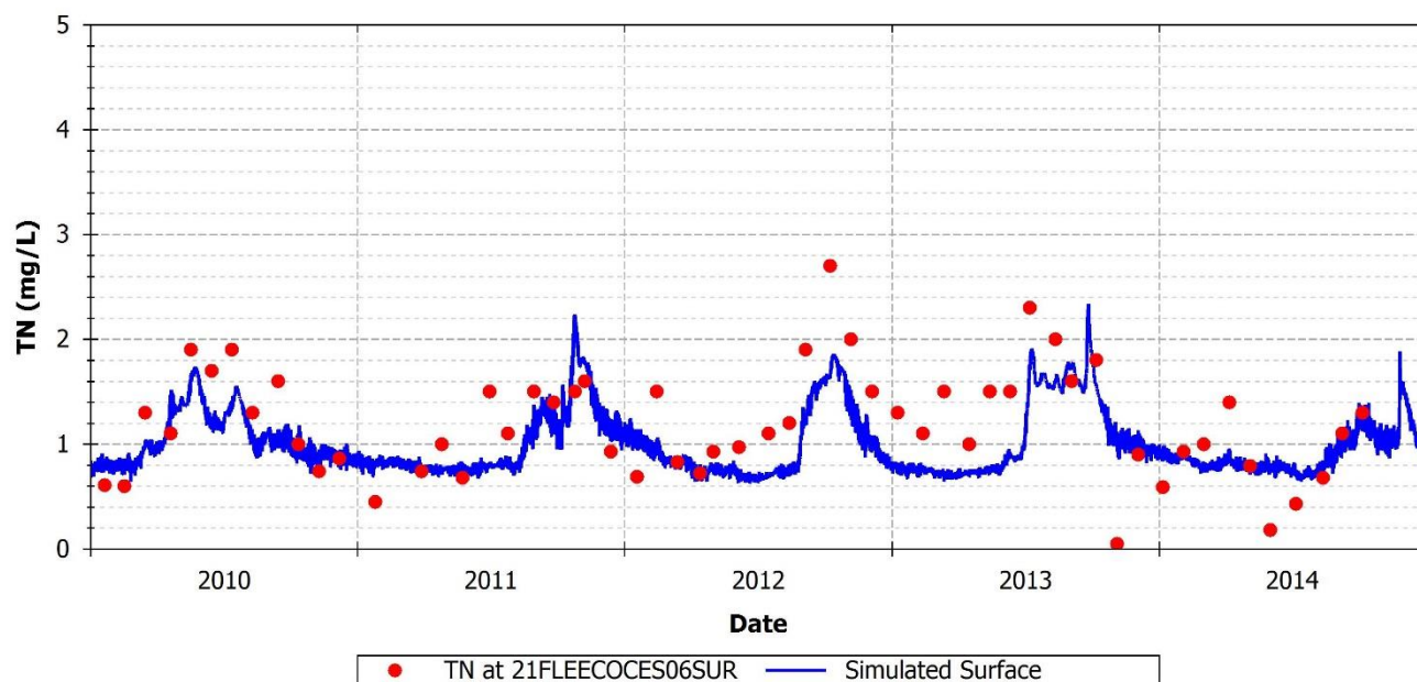
FIGURE 108: SIMULATED AND OBSERVED TN AT 21FLEECOCES06SUR
