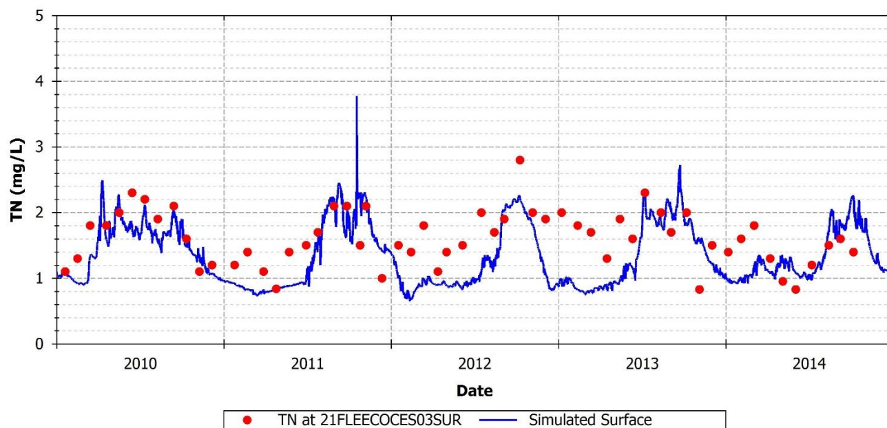
FIGURE 106: SIMULATED AND OBSERVED TN AT 21FLEECOCES03SUR
