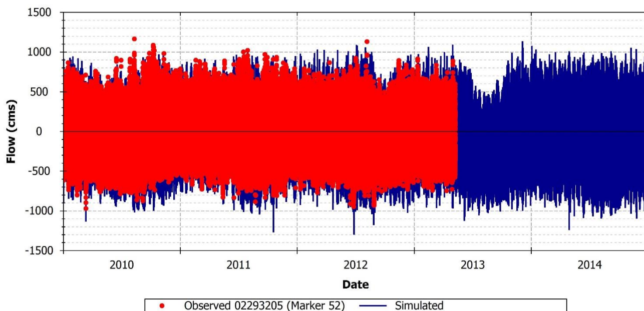
FIGURE 91: SIMULATED AND OBSERVED FLOW AT USGS 02293205 (MARKER 52), 2010 – 2014
