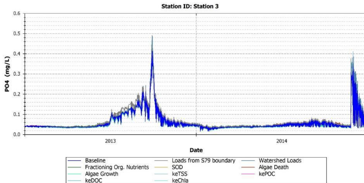
FIGURE 170: MODEL PREDICTIONS OF PO 4 FOR BASELINE AND PERTURBED MODEL CONDITIONS - STATION 3
