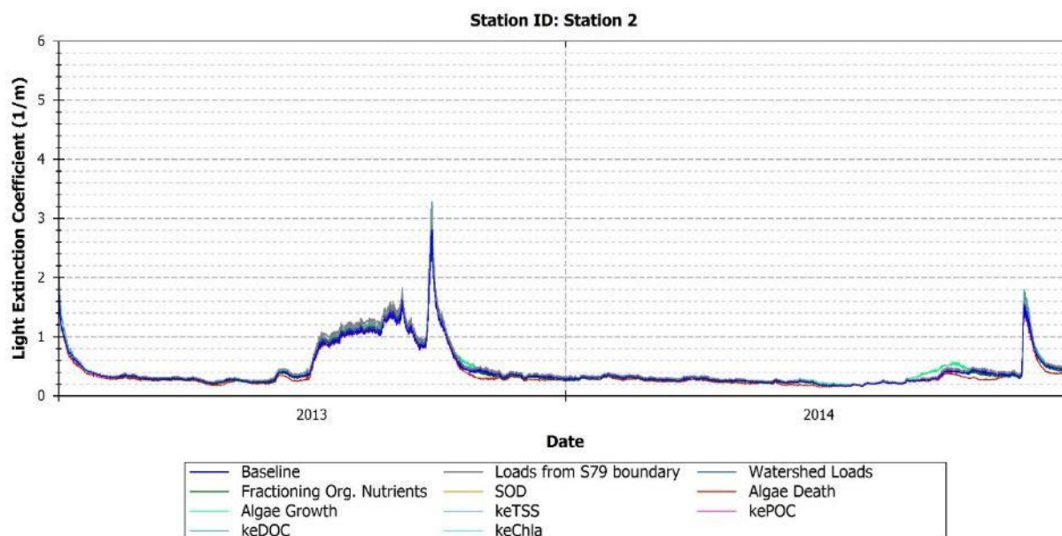
FIGURE 175: MODEL PREDICTIONS OF KE FOR BASELINE AND PERTURBED MODEL CONDITIONS - STATION 2
