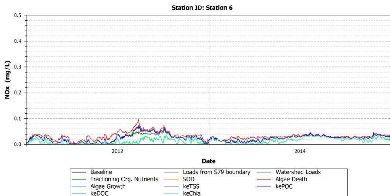
FIGURE 167: MODEL PREDICTIONS OF NO x FOR BASELINE AND PERTURBED MODEL CONDITIONS - STATION 6
