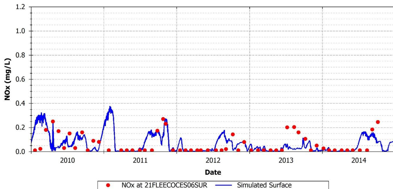
FIGURE 112: SIMULATED AND OBSERVED NO x AT 21FLEECOCES06SUR
