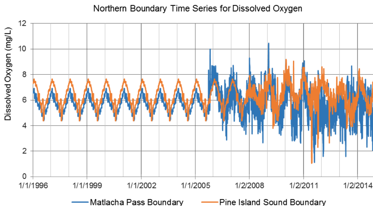
FIGURE 59: NORTHERN BOUNDARY 2017 MODEL INPUT TIME SERIES FOR DO (MG/L)
