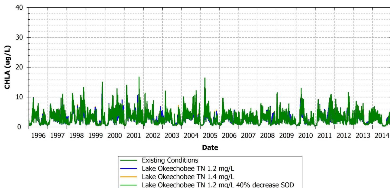
FIGURE 163: PHYTOPLANKTON BIOMASS COMPARISON BETWEEN EXISTING AND SCENARIOS AT 21CHARMPV004, MATLACHA PASS
