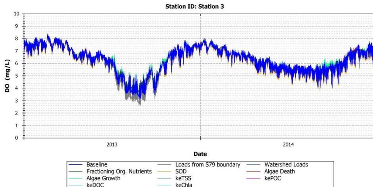
FIGURE 146: MODEL PREDICTIONS OF DO FOR BASELINE AND PERTURBED MODEL CONDITIONS - STATION 3
