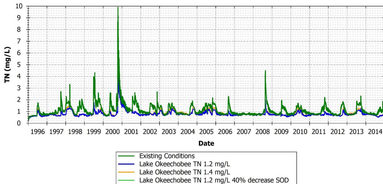
FIGURE 153: TN COMPARISON BETWEEN EXISTING AND SCENARIOS AT 21FLEECOCES06SUR, CALOOSAHATCHEE WATERWAY, MARKER 66
