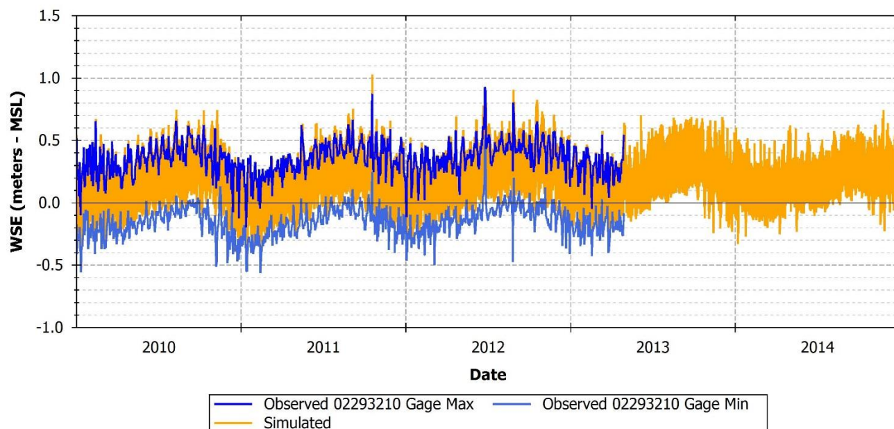
FIGURE 76: SIMULATED AND OBSERVED WSE AT USGS 02293210
