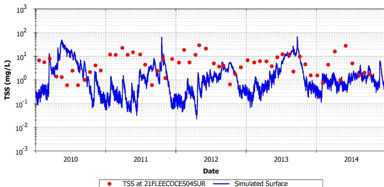
FIGURE 127: SIMULATED AND OBSERVED TSS AT 21FLEECOCES04SUR
