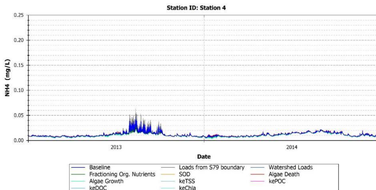
FIGURE 159: MODEL PREDICTIONS OF \text{NH}_4 FOR BASELINE AND PERTURBED MODEL CONDITIONS - STATION 4
