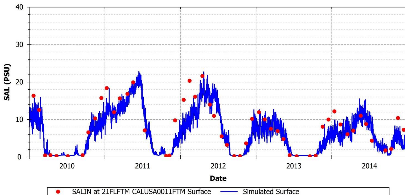
FIGURE 85: SIMULATED AND OBSERVED SALINITY AT 21FLFTM CALUSA0011FTM
