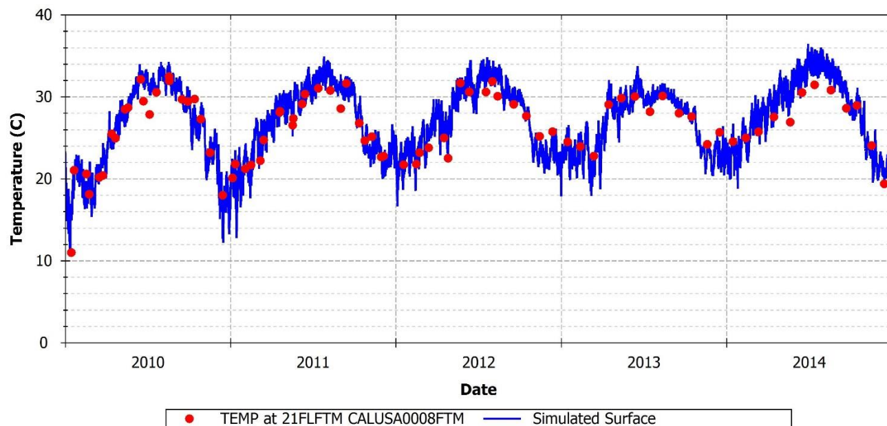
FIGURE 78: SIMULATED AND OBSERVED TEMPERATURE AT 21FLFTM CALUSA0008FTM
