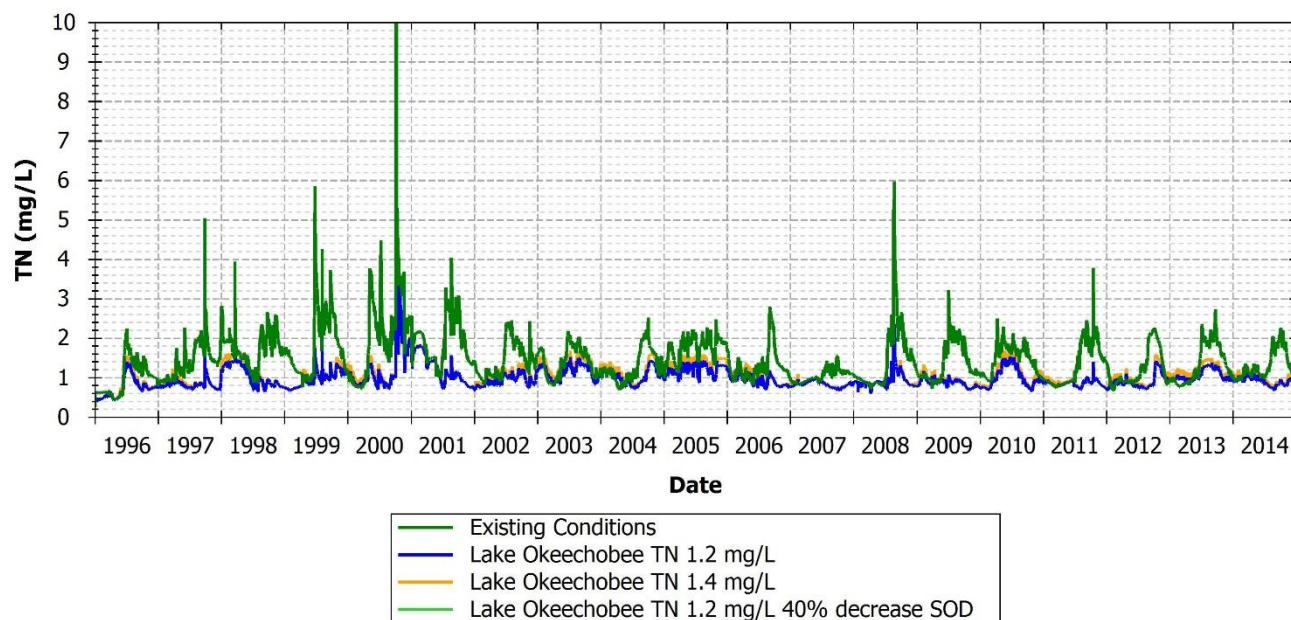
FIGURE 152: TN COMPARISON BETWEEN EXISTING AND SCENARIOS AT 21FLEECOCES03SUR, CALOOSAHATCHEE WATERWAY, ROUTE 31
