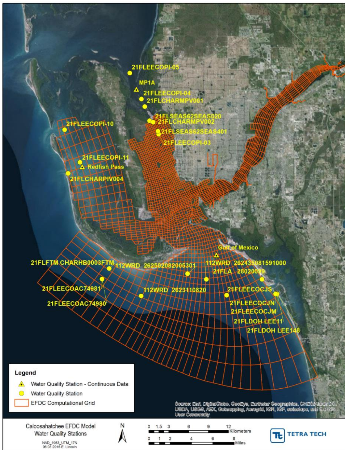
FIGURE 58: 2017 EFDC MODEL OPEN BOUNDARY WATER QUALITY STATION LOCATIONS
