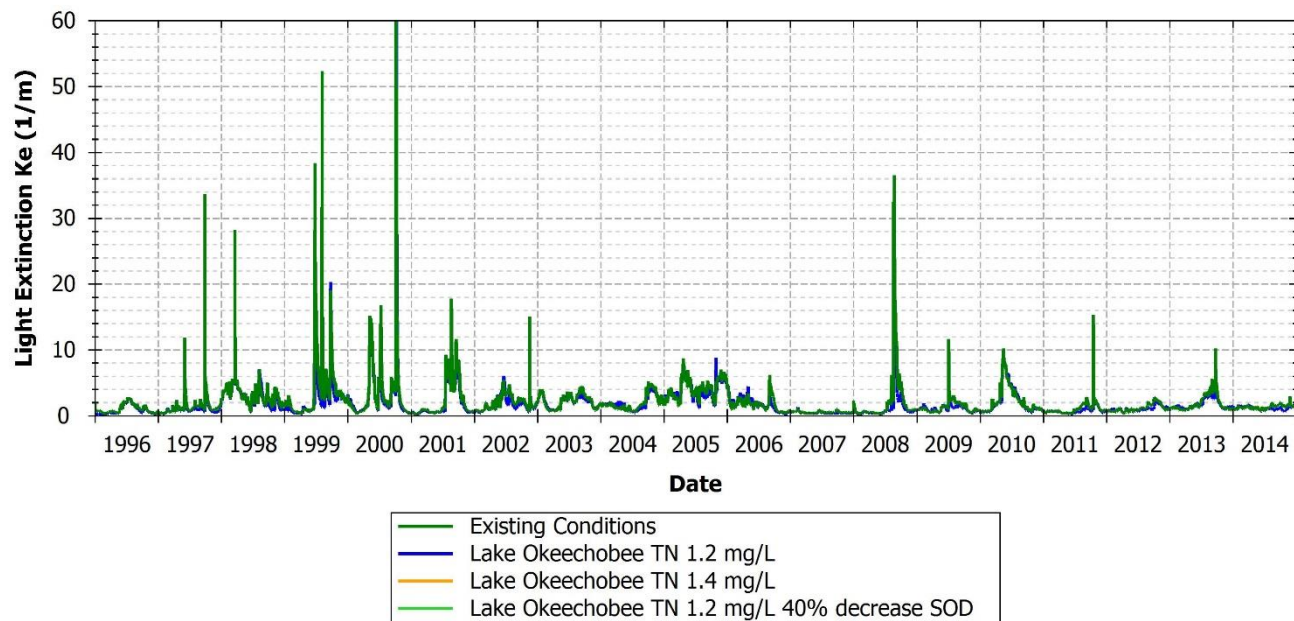
FIGURE 184: LIGHT EXTINCTION COMPARISON BETWEEN EXISTING AND SCENARIOS AT 21FLEECOCES03SUR, CALOOSAHATCHEE WATERWAY, ROUTE 31
