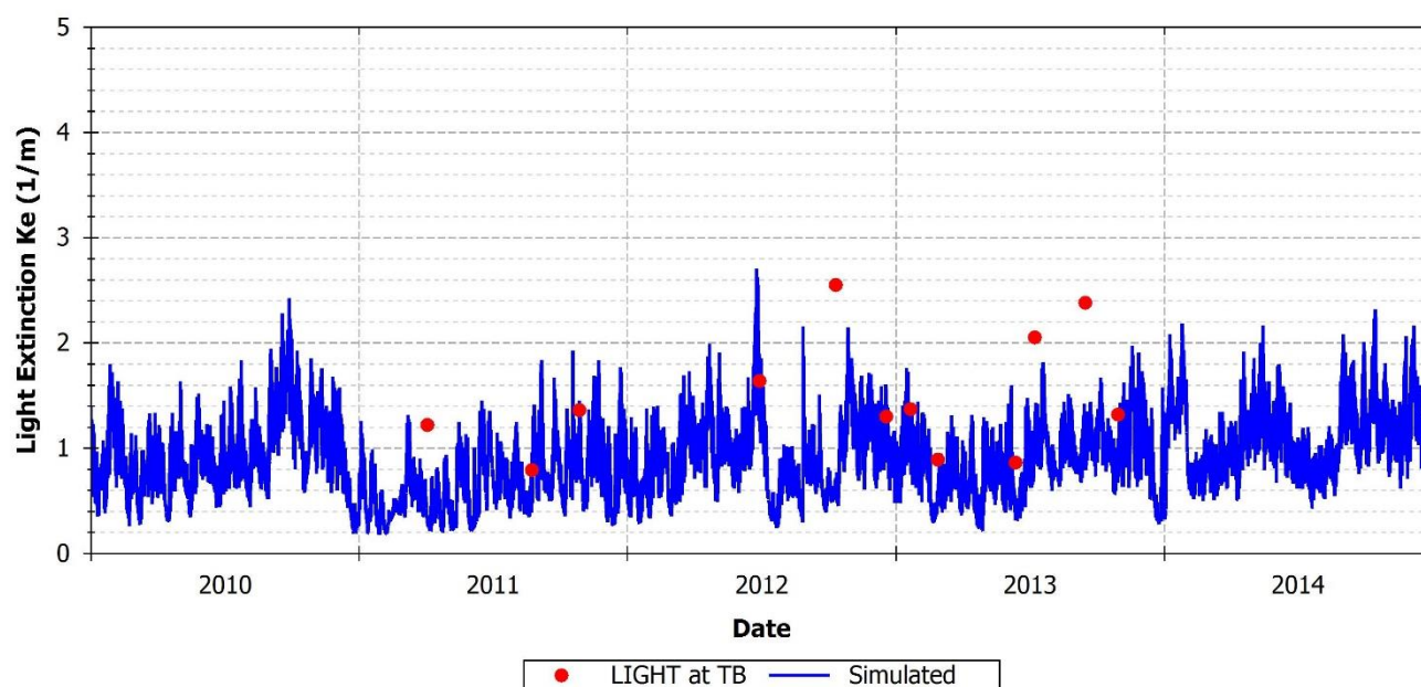
FIGURE 142: OBSERVED VERSUS PREDICTED LIGHT EXTINCTION AT SCCF STATION TB
