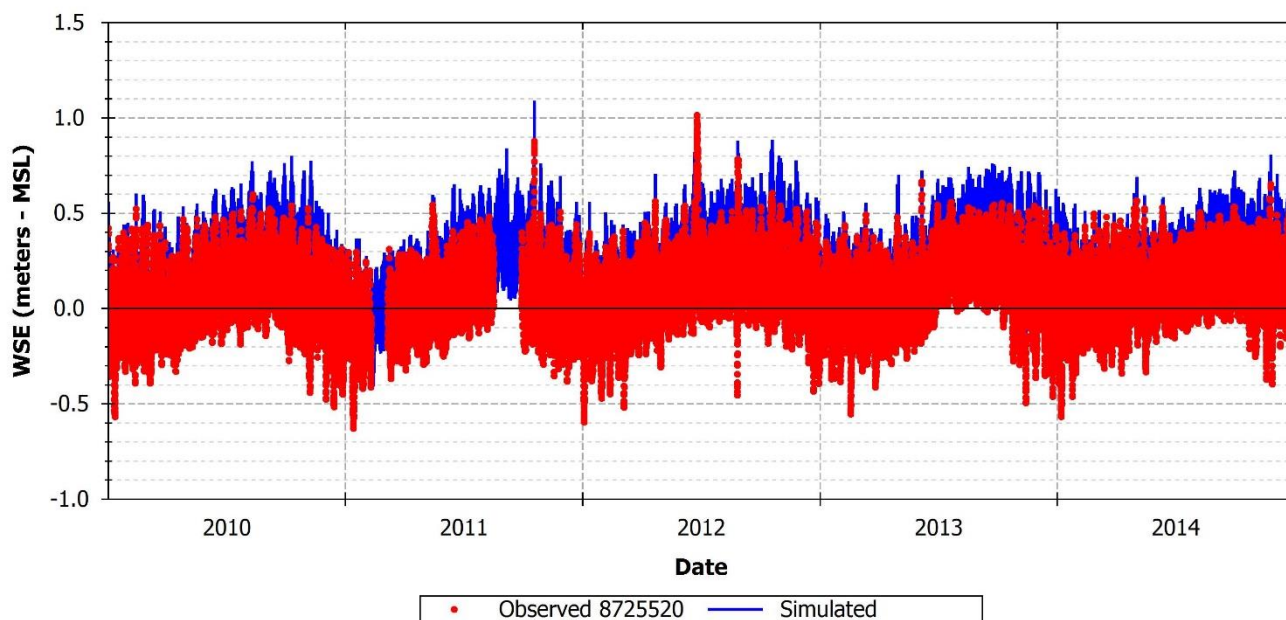
FIGURE 72: SIMULATED AND OBSERVED WSE AT NOAA STATION 8725520, 2010 – 2014
