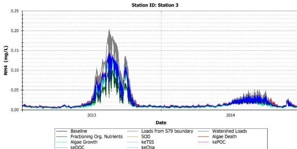
FIGURE 158: MODEL PREDICTIONS OF \text{NH}_4 FOR BASELINE AND PERTURBED MODEL CONDITIONS - STATION 3
