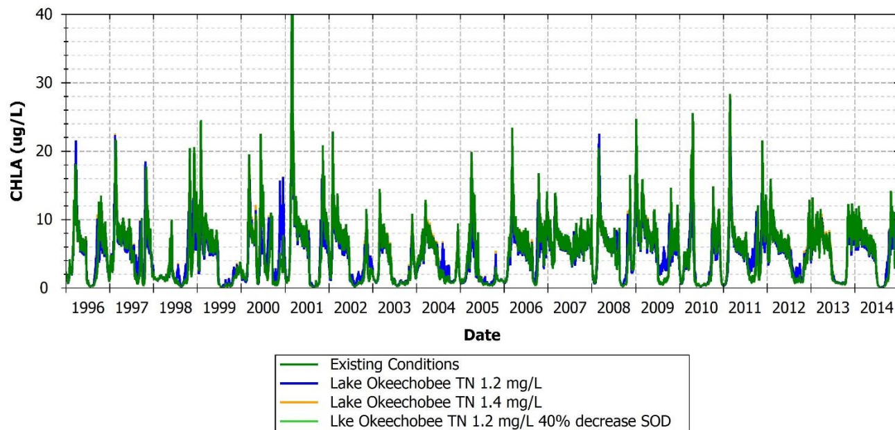
FIGURE 165: PHYTOPLANKTON BIOMASS COMPARISON BETWEEN EXISTING AND SCENARIOS AT 21FLEECOCES06SUR, CALOOSAHATCHEE WATERWAY, MARKER 66
