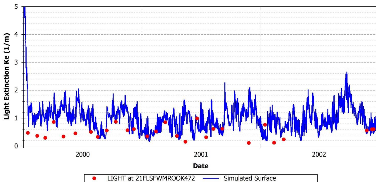
FIGURE 131: OBSERVED VERSUS PREDICTED LIGHT EXTINCTION AT 21FLSWMROOK472
