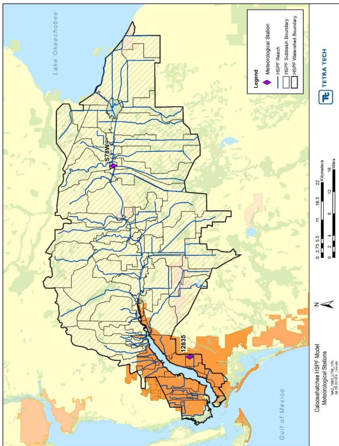
FIGURE 12: METEOROLOGICAL STATIONS USED FOR HSPF MODEL CLIMATE DATA PROCESSING
