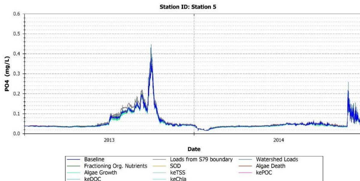
FIGURE 172: MODEL PREDICTIONS OF PO 4 FOR BASELINE AND PERTURBED MODEL CONDITIONS - STATION 5
