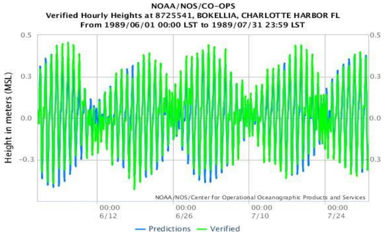
FIGURE 50: PREDICTED VERSUS OBSERVED WATER LEVELS AT NOAA STATION 8725541
