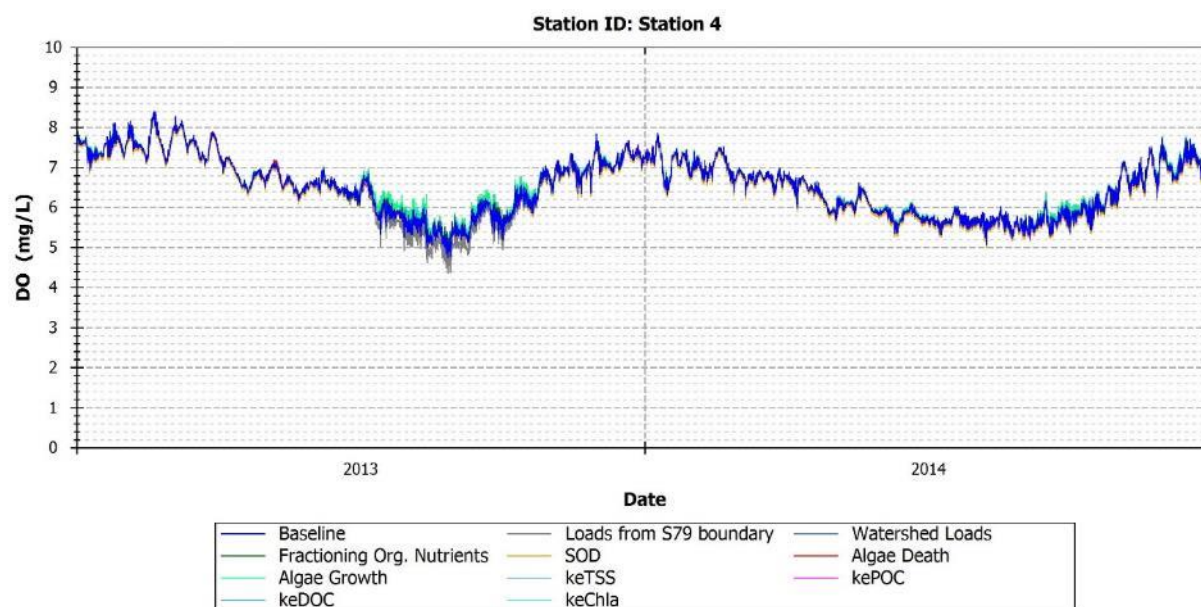
FIGURE 147: MODEL PREDICTIONS OF DO FOR BASELINE AND PERTURBED MODEL CONDITIONS - STATION 4
