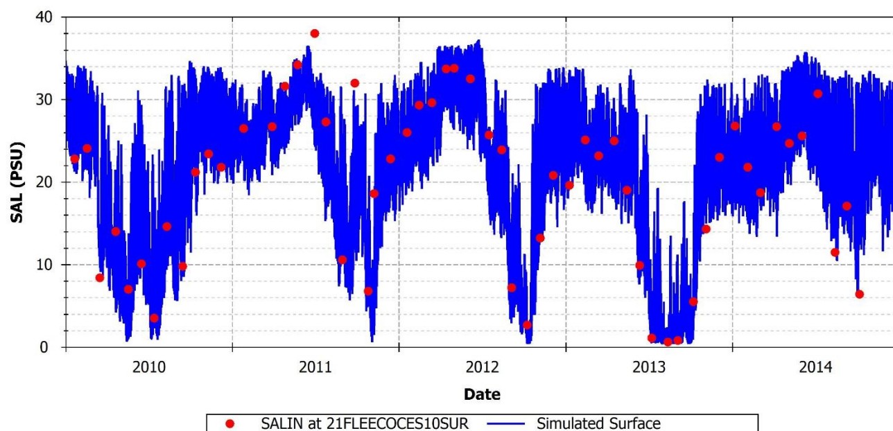
FIGURE 87: SIMULATED AND OBSERVED SALINITY AT 21FLEECOCES10SUR
