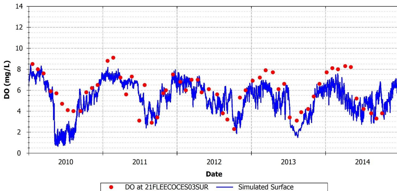
FIGURE 96: SIMULATED AND OBSERVED DO AT 21FLEECOCES03SUR
