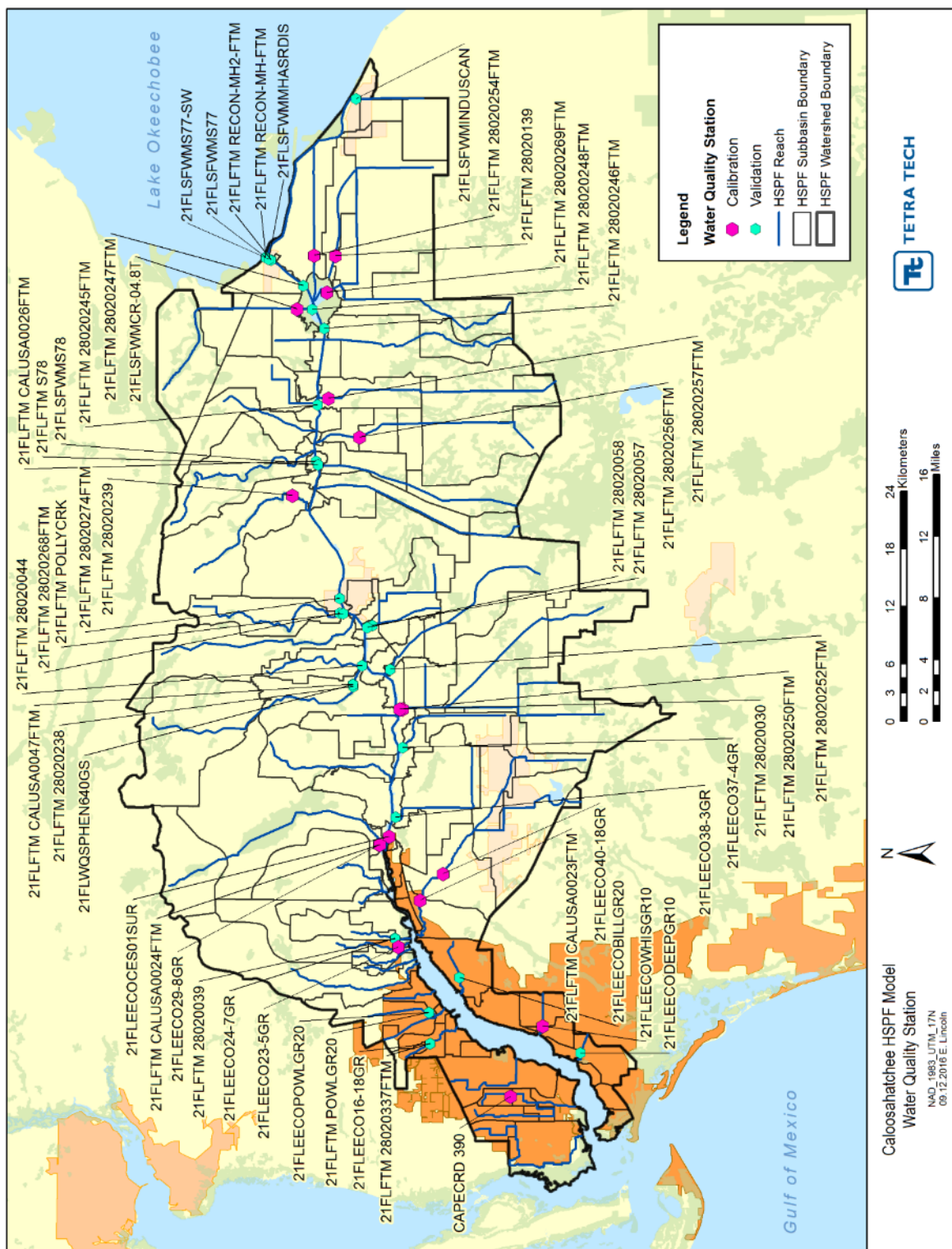
FIGURE 40: LOCATION OF THE WATER QUALITY CALIBRATION AND VALIDATION STATIONS IN THE CALOOSAHATCHEE RIVER WATERSHED
