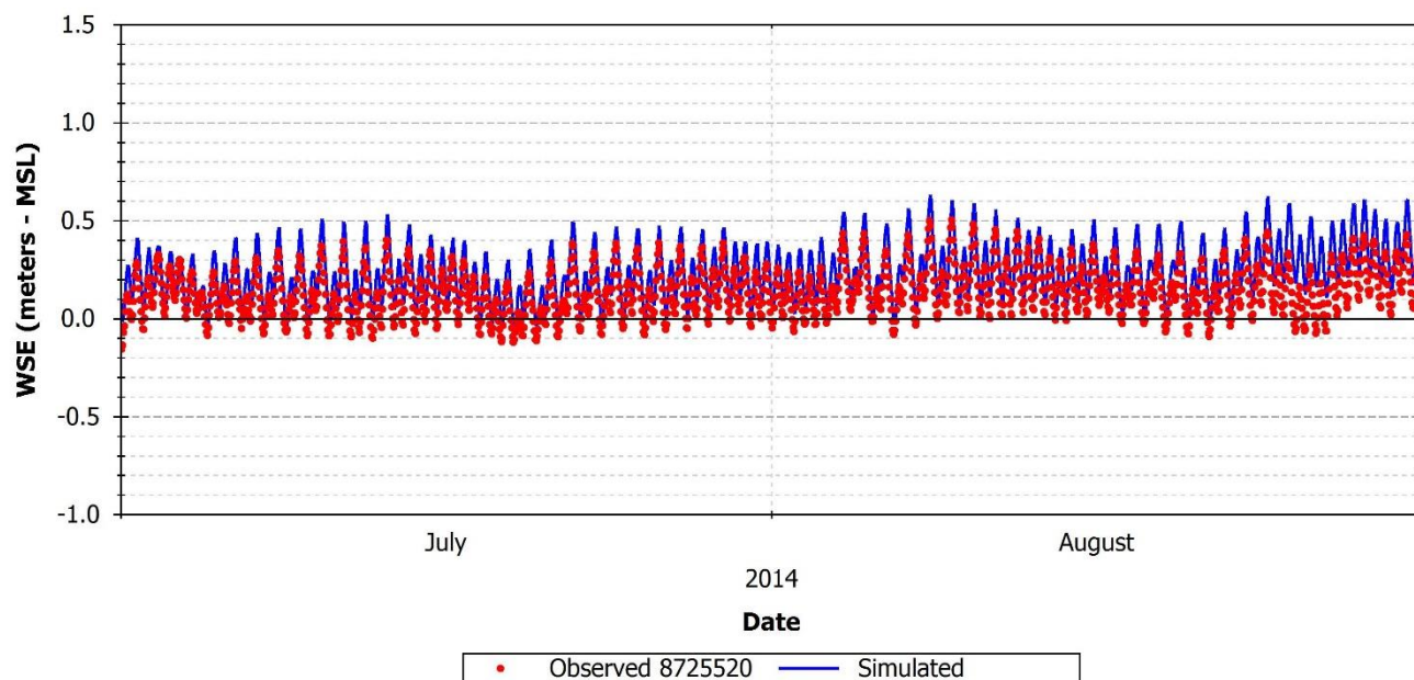
FIGURE 74: SIMULATED AND OBSERVED WSE AT NOAA STATION 8525520, JULY – AUGUST, 2014
