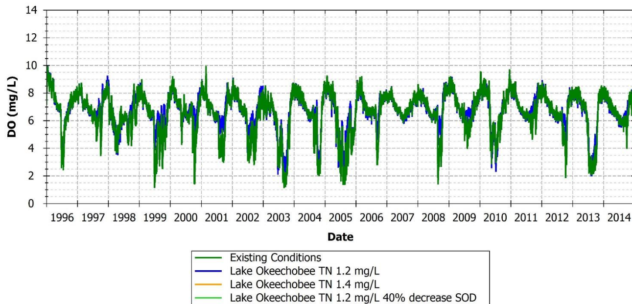
FIGURE 147: DO COMPARISON BETWEEN EXISTING AND SCENARIOS AT 21FLEECOCES06SUR, CALOOSAHATCHEE WATERWAY, MARKER 66
