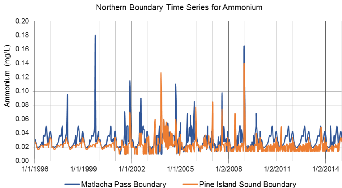
FIGURE 62: NORTHERN BOUNDARY 2017 MODEL INPUT TIME SERIES FOR \text{NH}_4 (MG/L)
