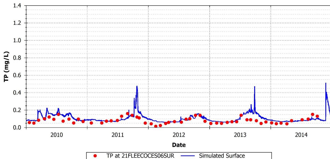
FIGURE 123: SIMULATED AND OBSERVED TP AT 21FLEECOCES06SUR
