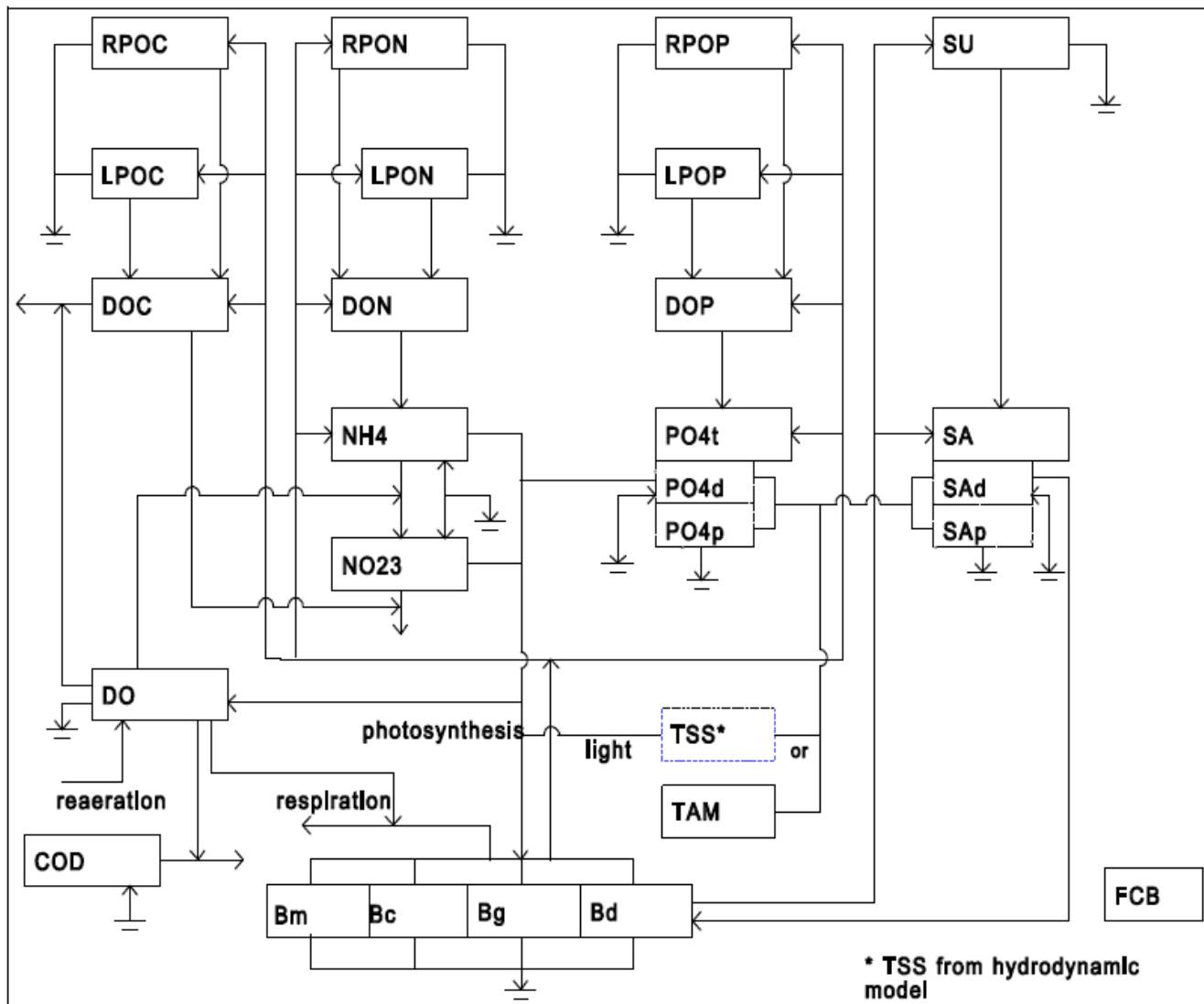
FIGURE 94: SCHEMATIC REPRESENTATION OF THE EFDC WATER QUALITY MODULE
