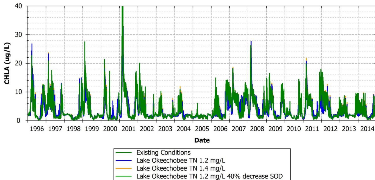
FIGURE 167: PHYTOPLANKTON BIOMASS COMPARISON BETWEEN EXISTING AND SCENARIOS AT 21FLFTM CALUSA0008FTM, CALOOSAHATCHEE WATERWAY, MARKER 22
