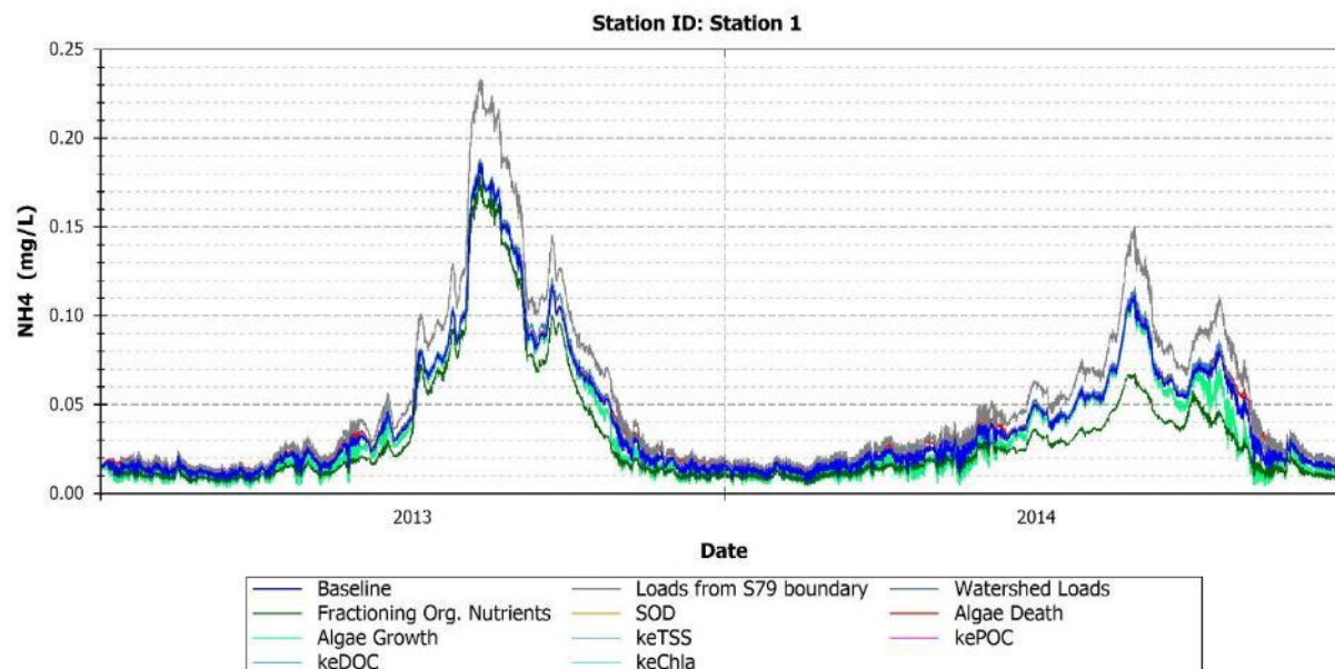
FIGURE 156: MODEL PREDICTIONS OF \text{NH}_4 FOR BASELINE AND PERTURBED MODEL CONDITIONS - STATION 1
