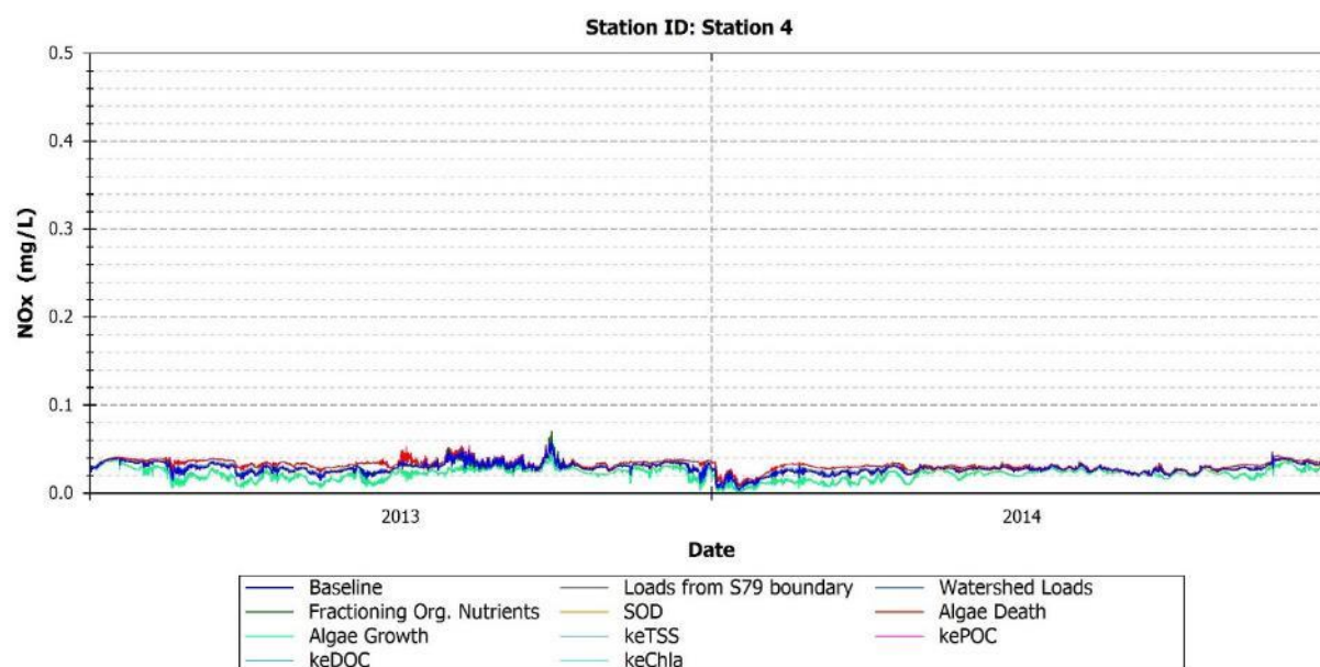
FIGURE 165: MODEL PREDICTIONS OF NO x FOR BASELINE AND PERTURBED MODEL CONDITIONS - STATION 4
