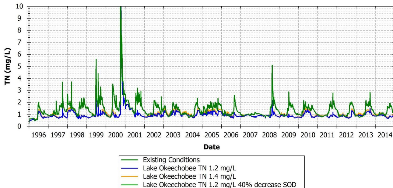
FIGURE 155: TN COMPARISON BETWEEN EXISTING AND SCENARIOS AT 21FLFTM CALUSA0008FTM, CALOOSAHATCHEE WATERWAY, MARKER 22
