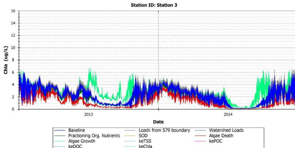
FIGURE 152: MODEL PREDICTIONS OF PHYTOPLANKTON BIOMASS FOR BASELINE AND PERTURBED MODEL CONDITIONS - STATION 3
