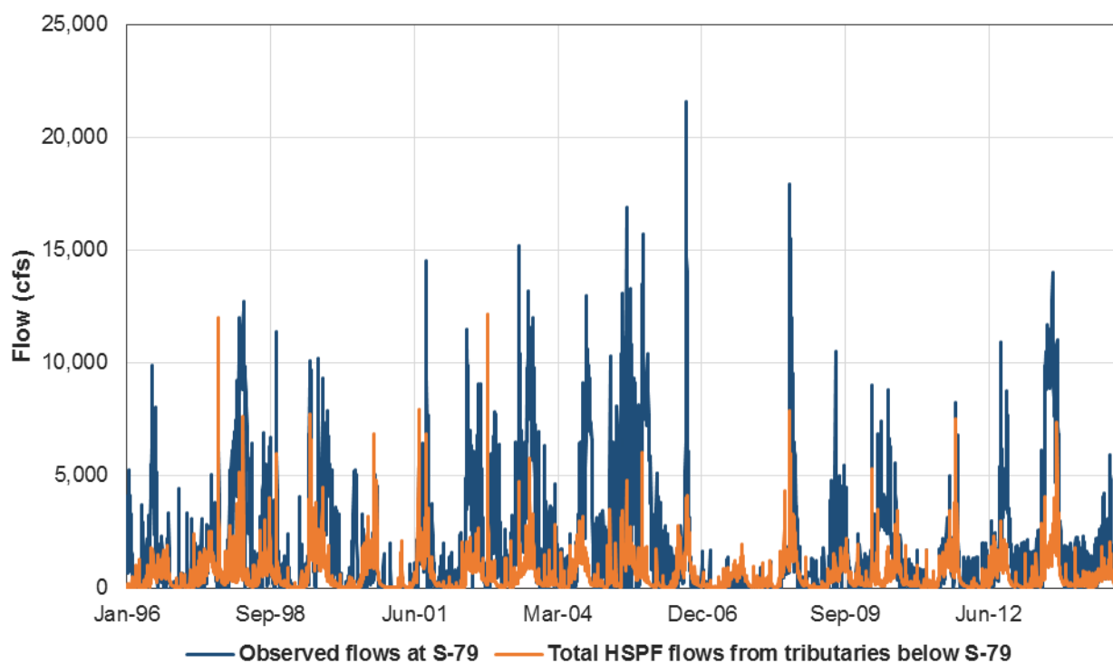
FIGURE 52: FRESHWATER INPUTS AT S-79 AND TOTAL TRIBUTARIES BELOW S-79 IN THE 2017 CALOOSAHATCHEE RIVER MODEL
