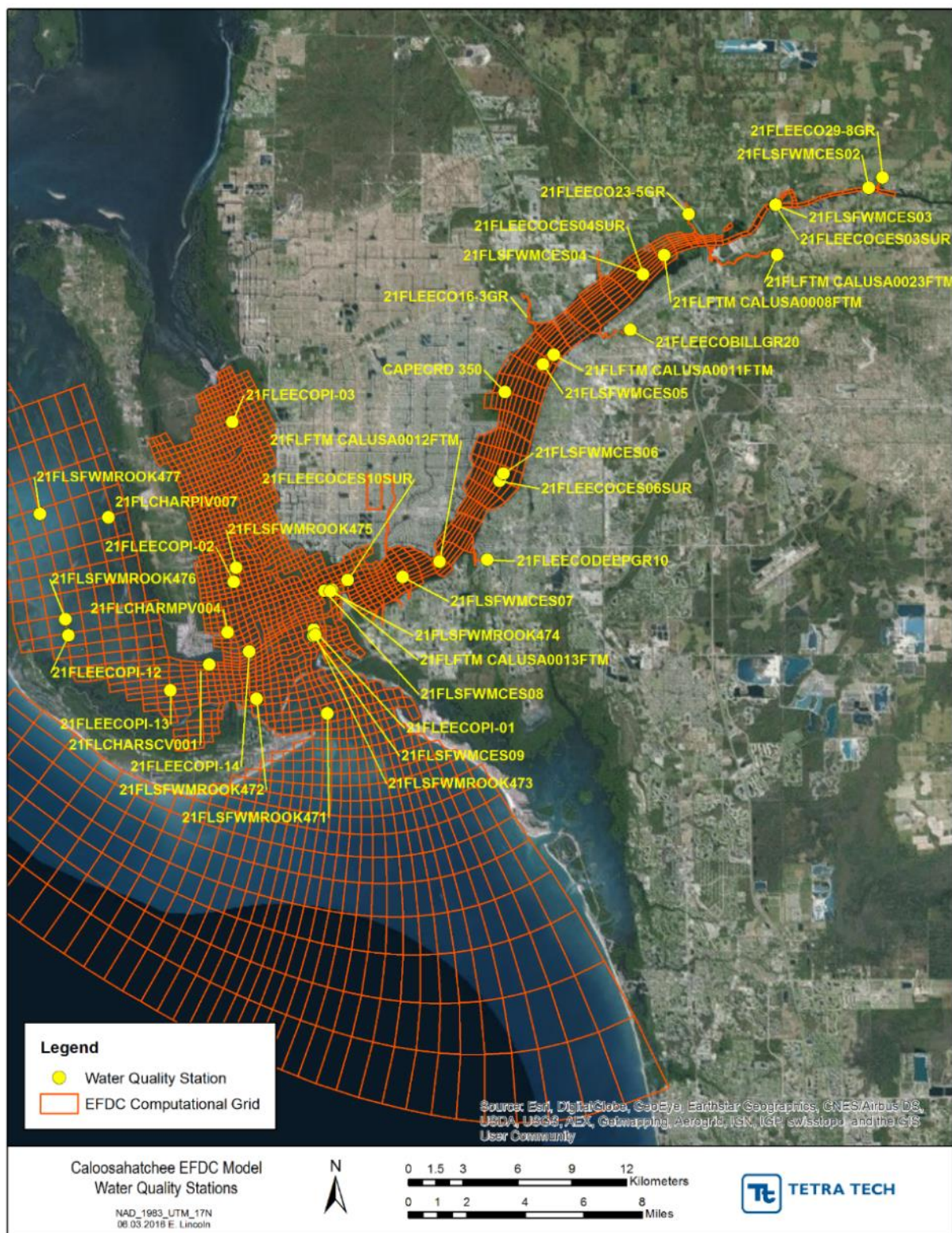
FIGURE 95: SUBSET OF WATER QUALITY STATIONS DISTRIBUTED ACROSS THE CALOOSA HATCHEE RIVER
