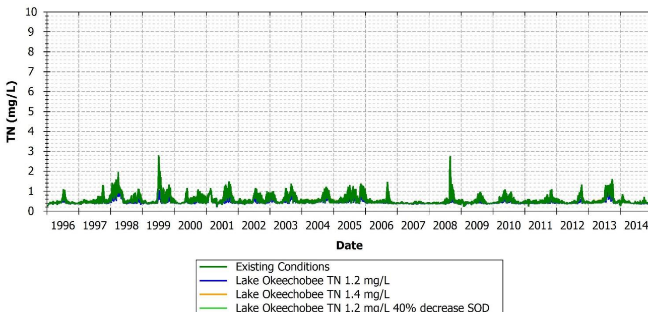
FIGURE 151: TN COMPARISON BETWEEN EXISTING AND SCENARIOS AT 21CHARMPV004, MATLACHA PASS
