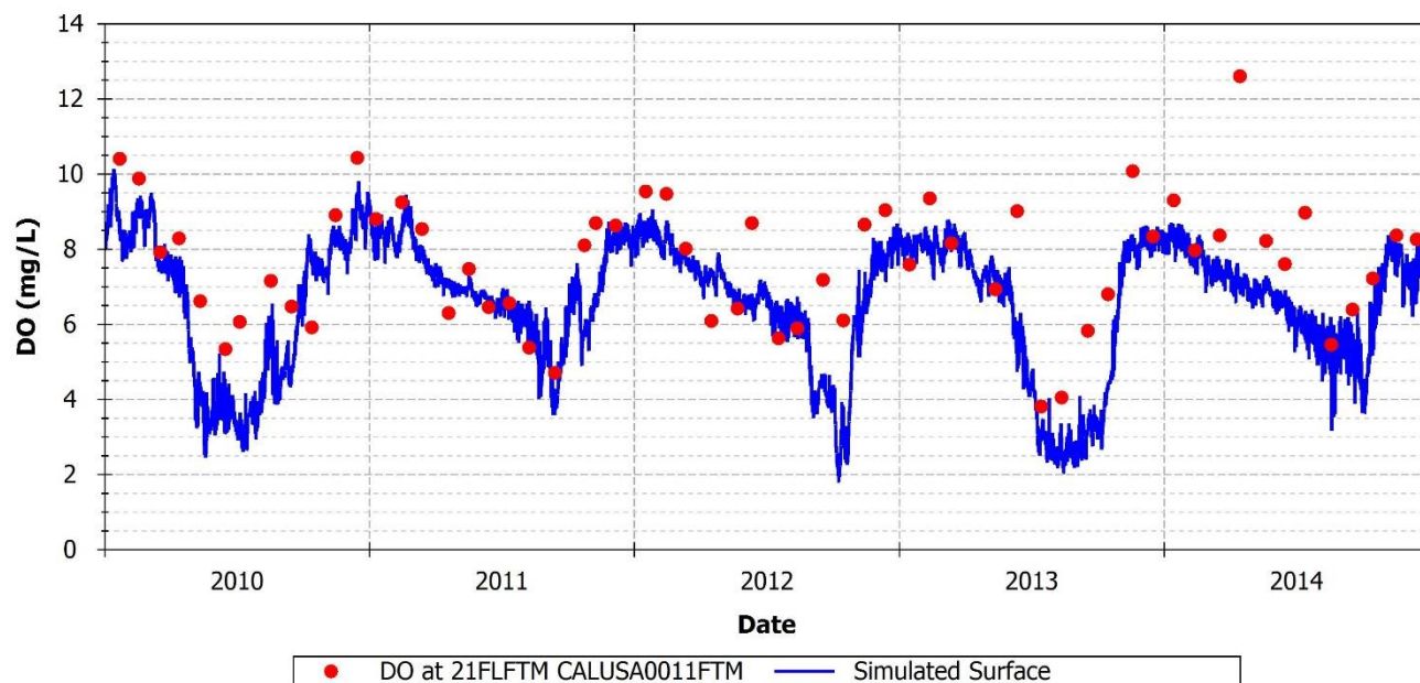
FIGURE 98: SIMULATED AND OBSERVED DO AT 21FLFTM CALUSA0011FTM
