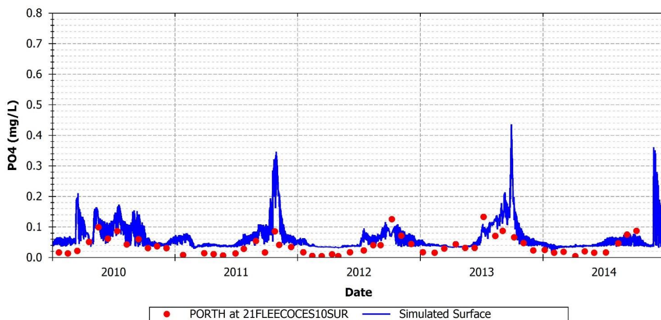
FIGURE 126: SIMULATED AND OBSERVED PO 4 AT 21FLEECOCES10SUR
