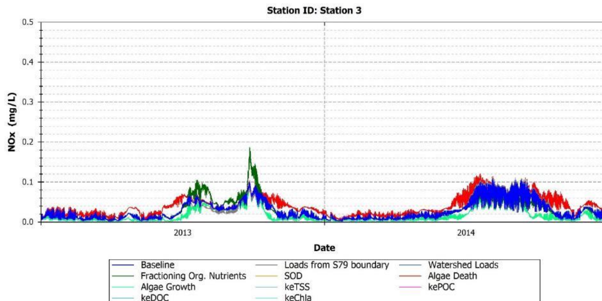
FIGURE 164: MODEL PREDICTIONS OF NO x FOR BASELINE AND PERTURBED MODEL CONDITIONS - STATION 3
