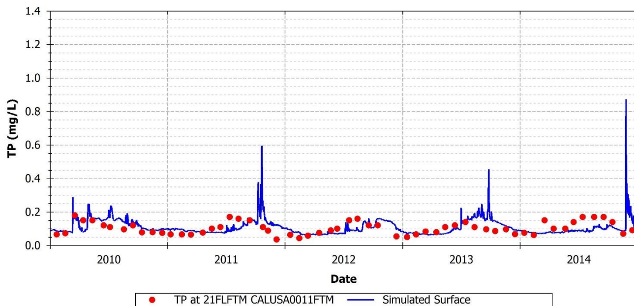
FIGURE 122: SIMULATED AND OBSERVED TP AT 21FLFTM CALUSA0011FTM
