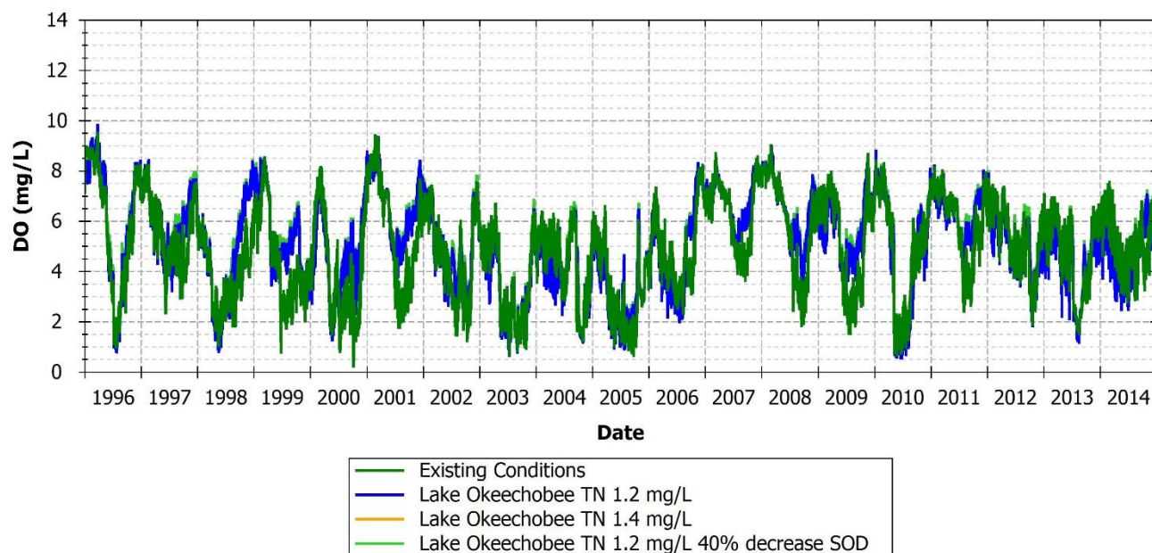
FIGURE 146: DO COMPARISON BETWEEN EXISTING AND SCENARIOS AT 21FLEECOCES03SUR, CALOOSAHATCHEE WATERWAY, ROUTE 31
