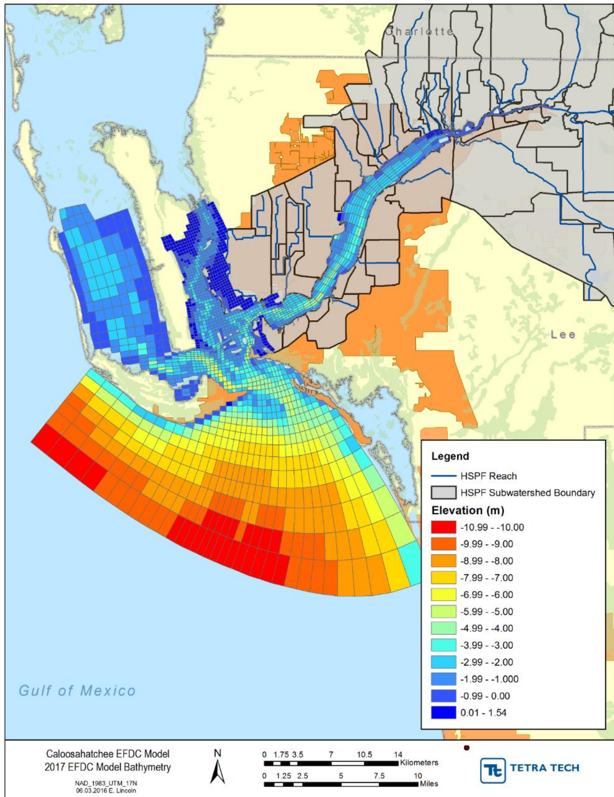
FIGURE 48: 2017 EFDC MODEL BATHYMETRY
