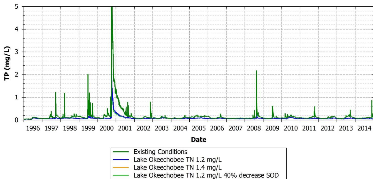
FIGURE 162: TP COMPARISON BETWEEN EXISTING AND SCENARIOS AT 21FLFTM CALUSA0011FTM, CALOOSAHATCHEE WATERWAY, MARKER 52
