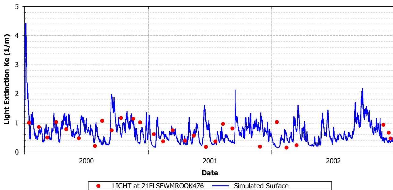
FIGURE 135: OBSERVED VERSUS PREDICTED LIGHT EXTINCTION AT 21FLSWMROOK476
