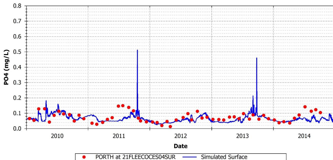
FIGURE 125: SIMULATED AND OBSERVED PO 4 AT 21FLEECOCES04SUR
