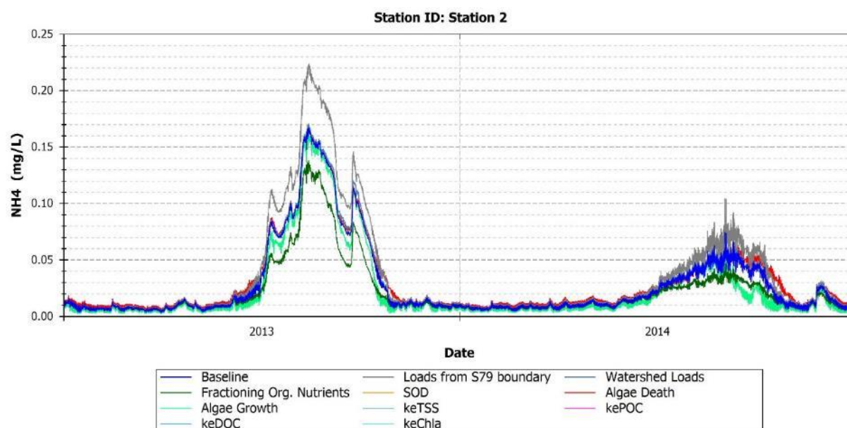
FIGURE 157: MODEL PREDICTIONS OF \text{NH}_4 FOR BASELINE AND PERTURBED MODEL CONDITIONS - STATION 2
