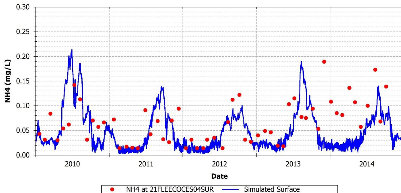
FIGURE 114: SIMULATED AND OBSERVED NH 4 AT 21FLEECOCES04SUR
