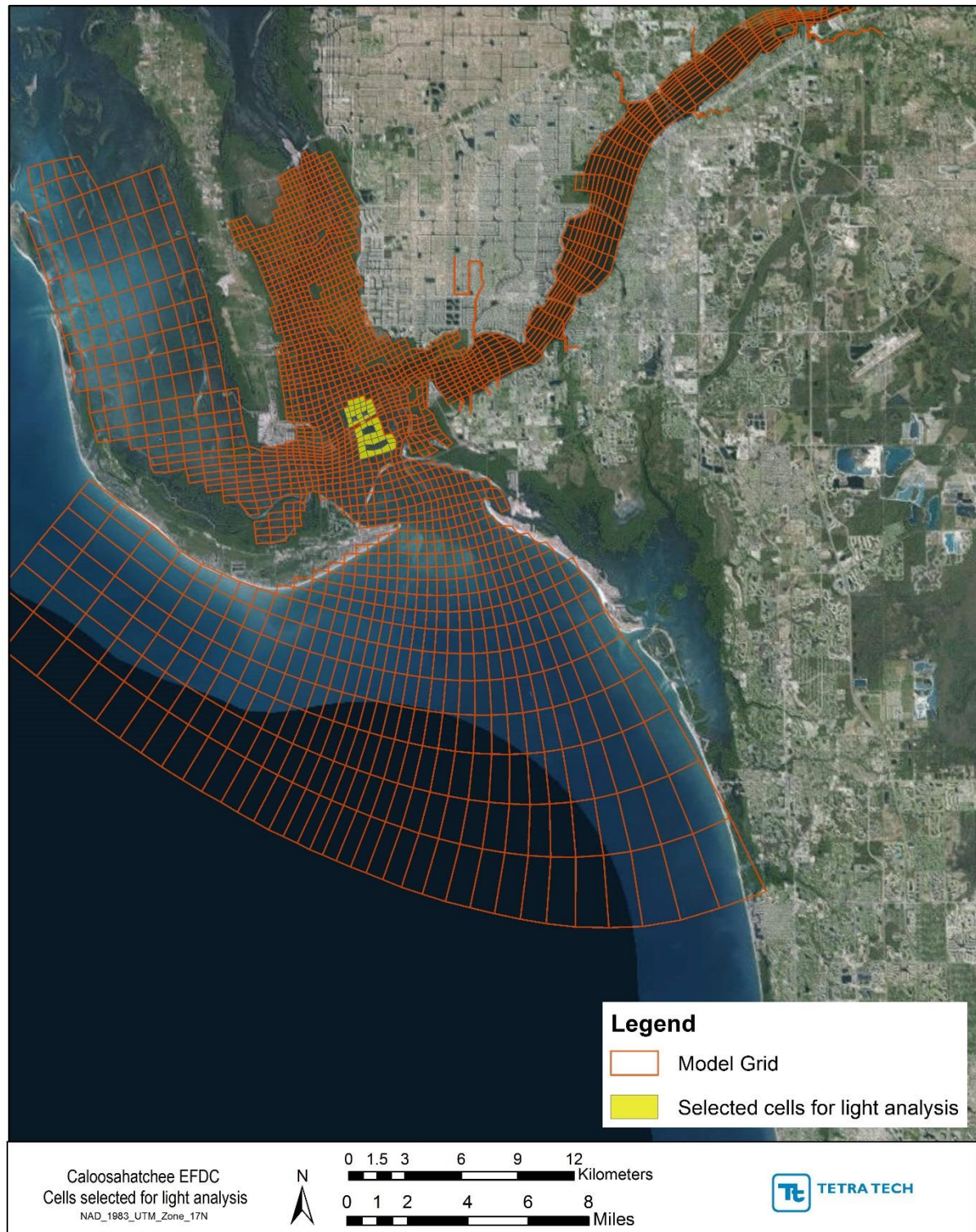
FIGURE 180: SAN CARLOS BAY SELECTED CELLS FOR LIGHT ANALYSIS THAT HAVE A MAXIMUM DEPTH OF 2.2 METERS
