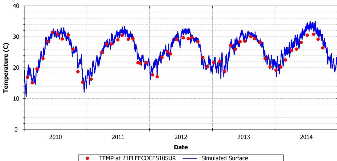
FIGURE 81: SIMULATED AND OBSERVED TEMPERATURE AT 21FLEECOCES10SUR
