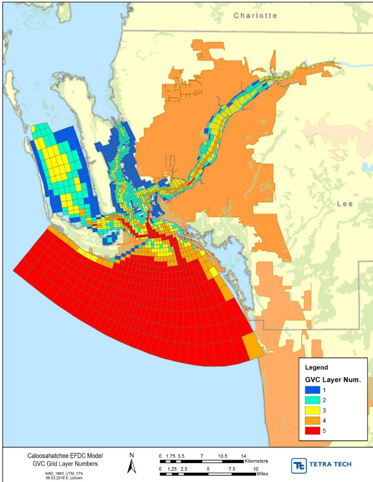
FIGURE 47: 2017 EFDC MODEL GRID GVC LAYER NUMBERS
