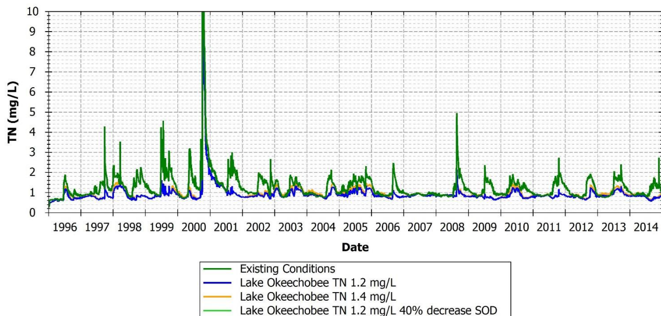
FIGURE 156: TOTAL NITROGEN COMPARISON BETWEEN EXISTING AND SCENARIOS AT 21FLFTM CALUSA0011FTM, CALOOSAHATCHEE WATERWAY, MARKER 52
