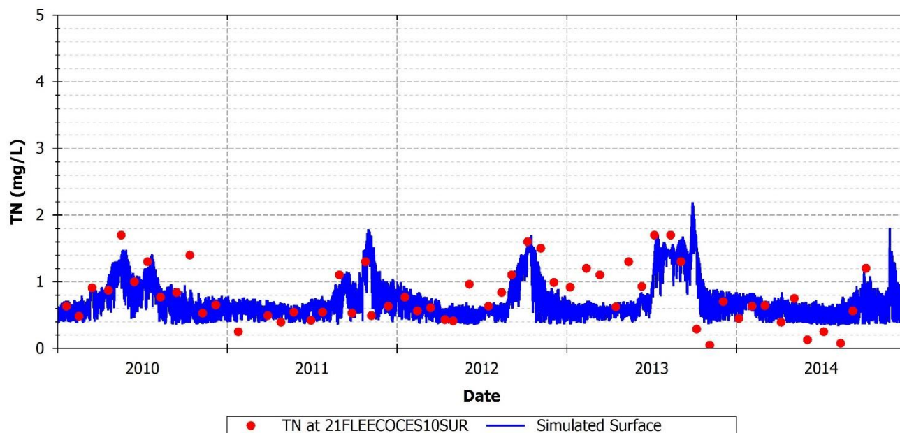
FIGURE 109: SIMULATED AND OBSERVED TN AT 21FLEECOCES10SUR
