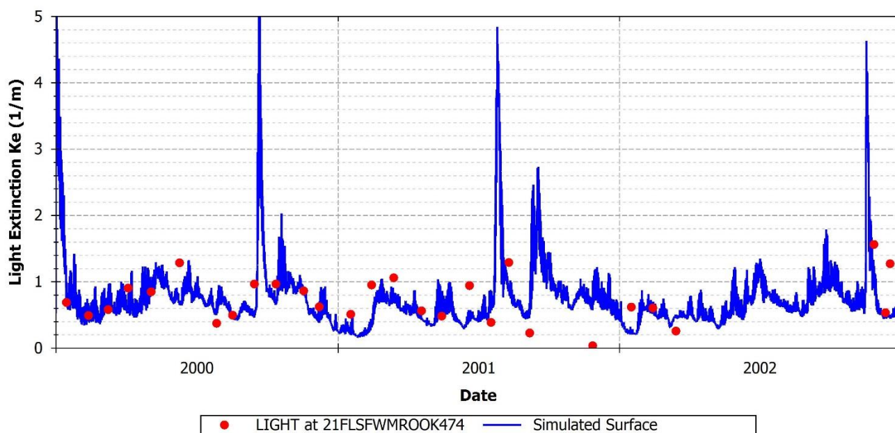
FIGURE 133: OBSERVED VERSUS PREDICTED LIGHT EXTINCTION AT 21FLSWMROOK474
