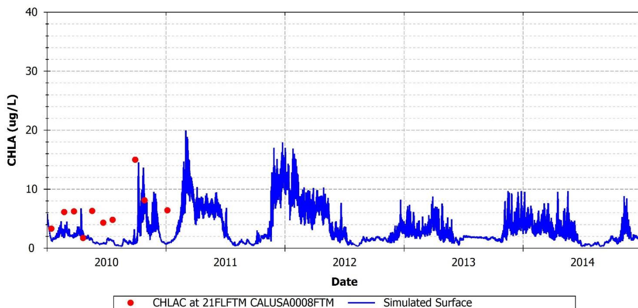
FIGURE 102: SIMULATED AND OBSERVED PHYTOPLANKTON BIOMASS AT 21FLFTM CALUSA0008FTM
