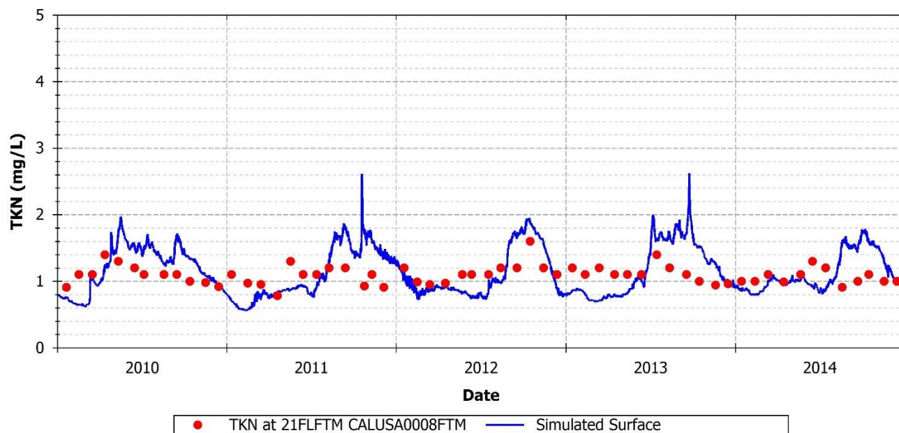
FIGURE 117: SIMULATED AND OBSERVED TKN AT 21FLFTM CALUSA0008FTM
