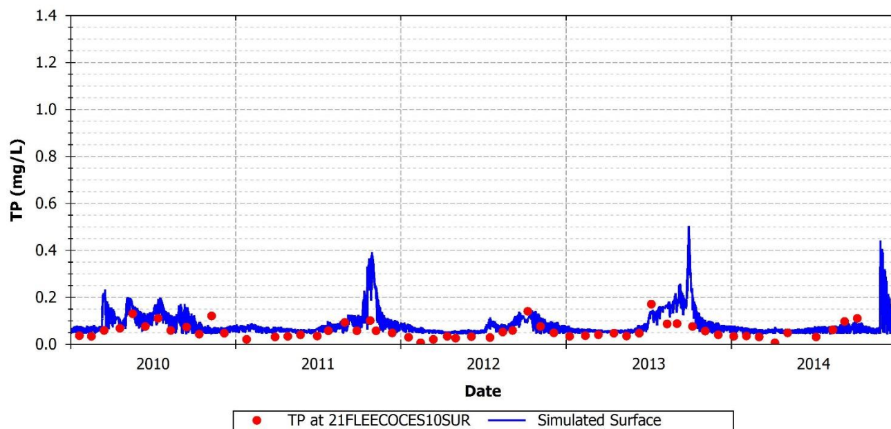
FIGURE 124: SIMULATED AND OBSERVED TP AT 21FLEECOCES10SUR
