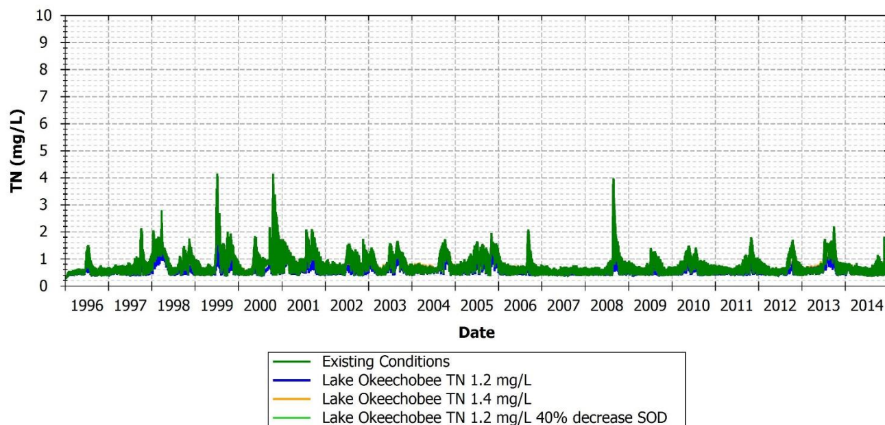
FIGURE 154: TN COMPARISON BETWEEN EXISTING AND SCENARIOS AT 21FLEECOCES10SUR, CALOOSAHATCHEE WATERWAY NEAR MOUTH
