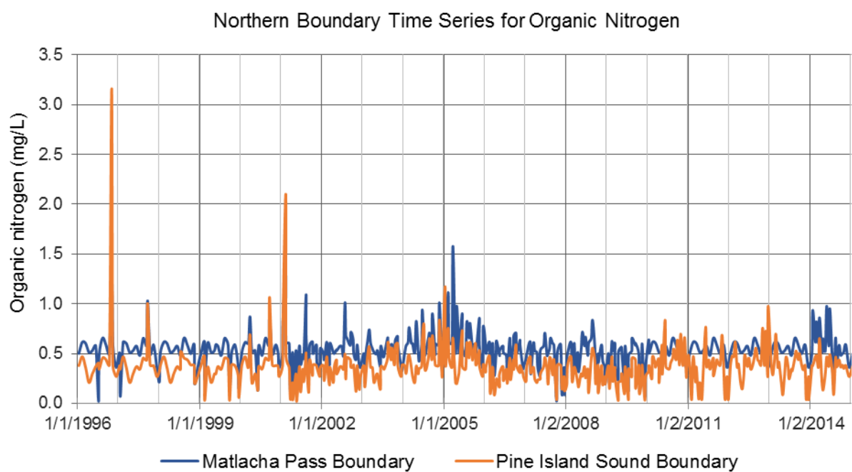
FIGURE 63: NORTHERN BOUNDARY 2017 MODEL INPUT TIME SERIES FOR ORGN (MG/L)
