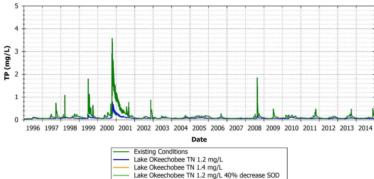
FIGURE 159: TP COMPARISON BETWEEN EXISTING AND SCENARIOS AT 21FLEECOCES06SUR, CALOOSAHATCHEE WATERWAY, MARKER 66
