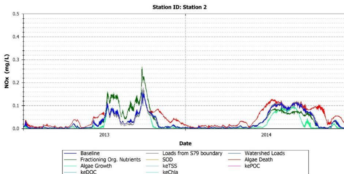
FIGURE 163: MODEL PREDICTIONS OF NO x FOR BASELINE AND PERTURBED MODEL CONDITIONS - STATION 2
