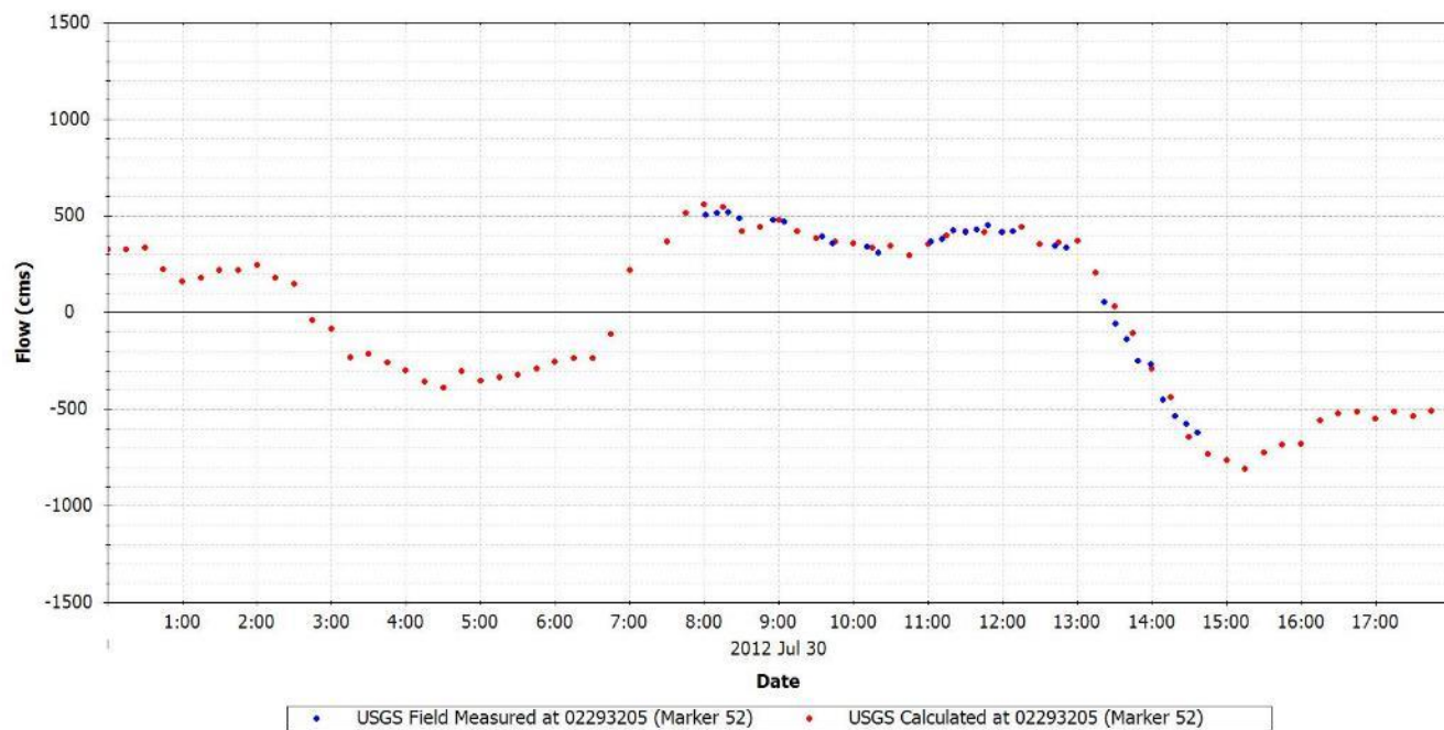
FIGURE 90: COMPARISON OF FLOWS MEASURED AND CALCULATED BY USGS AT STATION 02293205 (CONT.)
