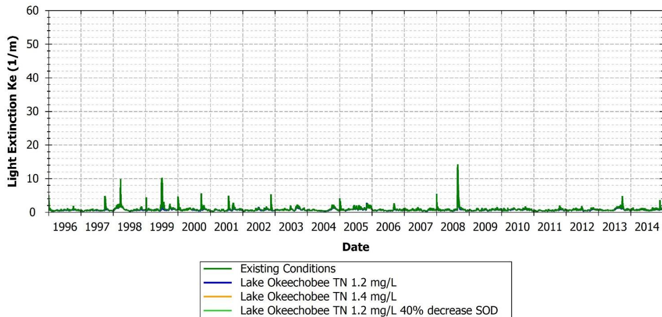
FIGURE 186: LIGHT EXTINCTION COMPARISON BETWEEN EXISTING AND SCENARIOS AT 21FLEECOCES10SUR, CALOOSAHATCHEE WATERWAY NEAR MOUTH
