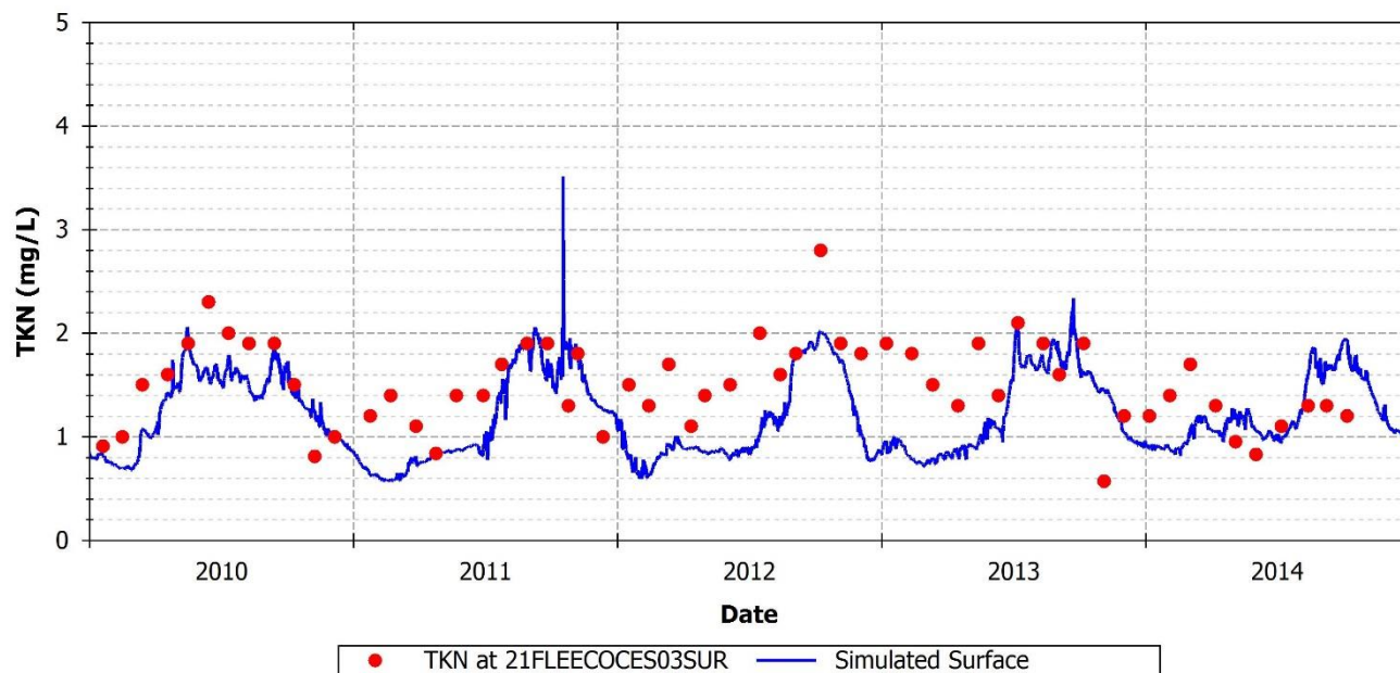
FIGURE 116: SIMULATED AND OBSERVED TKN AT 21FLEECOCES03SUR
