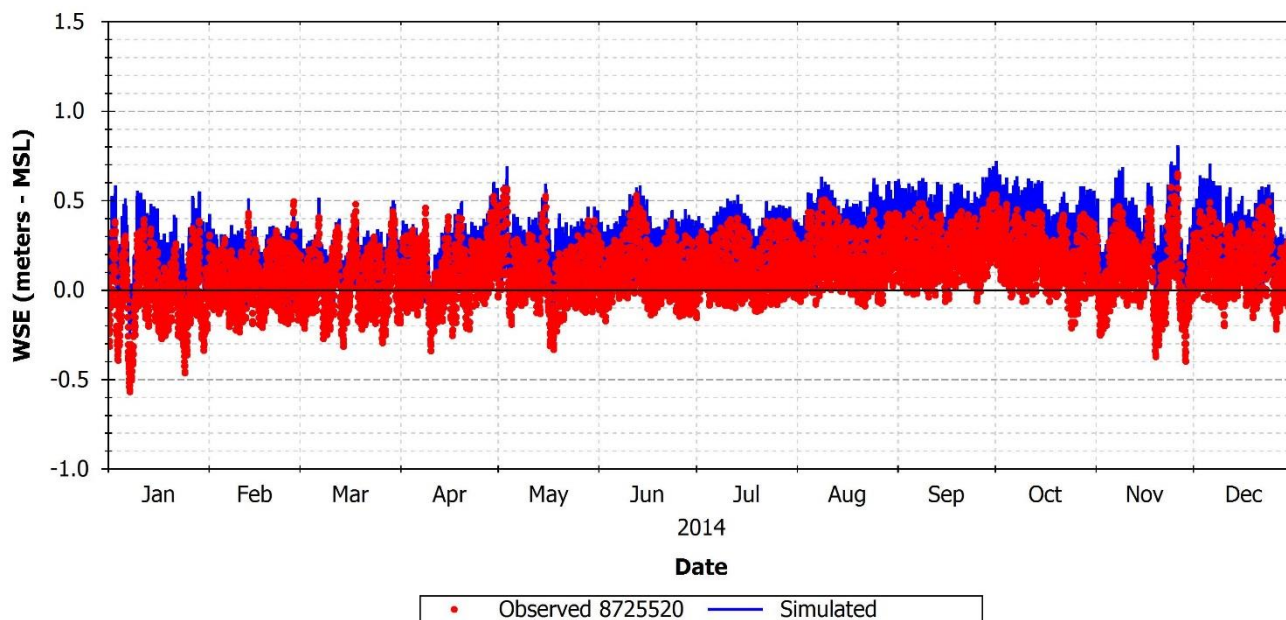
FIGURE 73: SIMULATED AND OBSERVED WSE AT NOAA STATION 8725520, 2014
