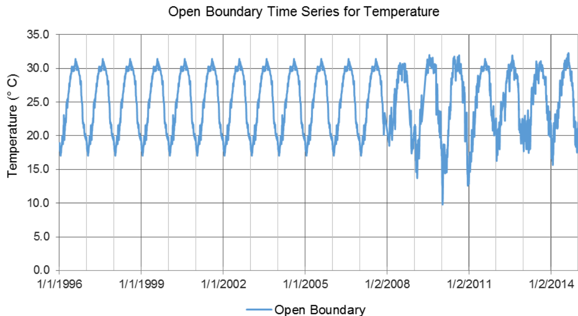
FIGURE 54: NORTHERN BOUNDARY 2017 MODEL INPUT TIME SERIES FOR TEMPERATURE (°C)
