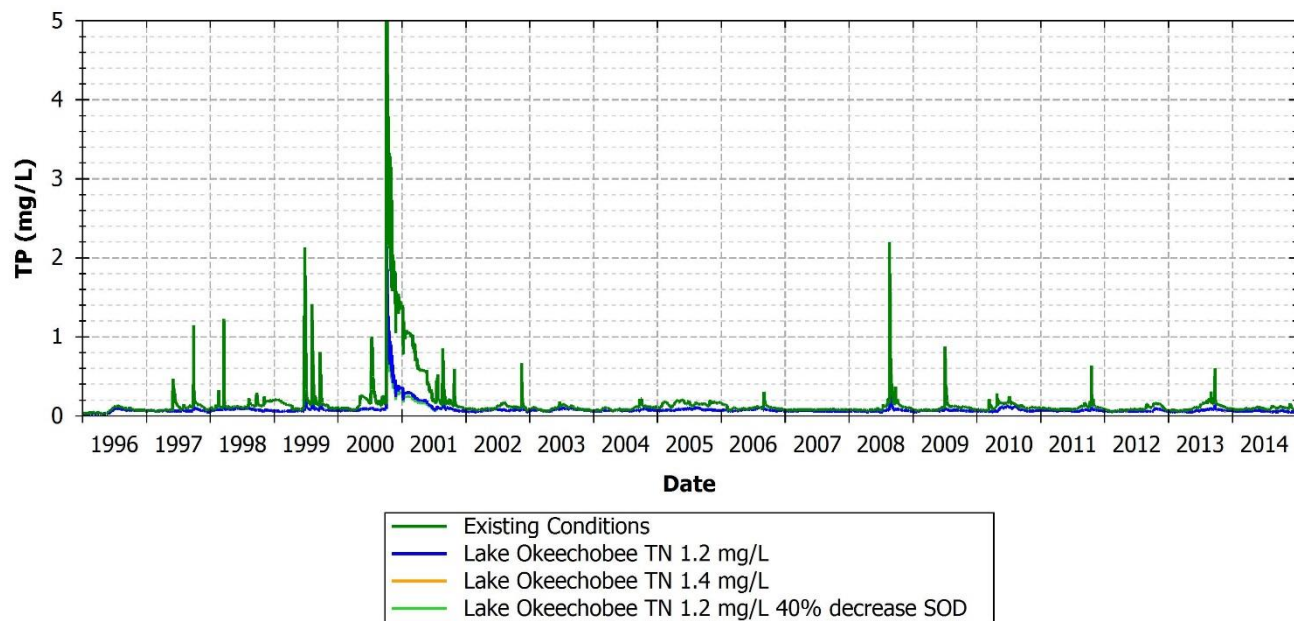
FIGURE 161: TP COMPARISON BETWEEN EXISTING AND SCENARIOS AT 21FLFTM CALUSA0008FTM, CALOOSAHATCHEE WATERWAY, MARKER 22
