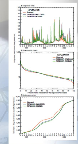
Figure 4. TOPMODEL streamflow simulations in relation to A, daily mean flows, B, flow-duration curves, and C, single-mass curves at McTier Creek near Monetta (02172300), for June 13, 2007, to September 30, 2009.
