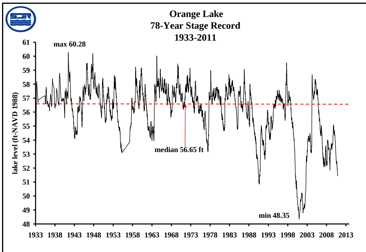
Figure 19. Daily lake level (stage) in Orange Lake for the 78-year period of record (1933-2011).
