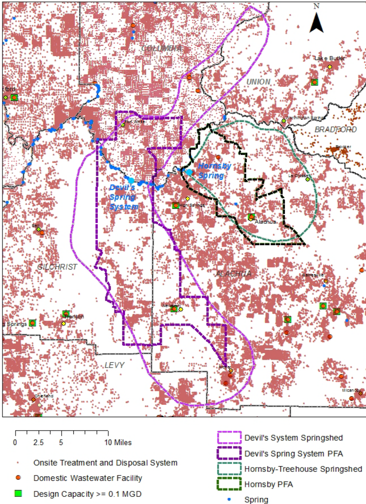
Figure 8. OSTDS, domestic WWTFs, and PFAs
