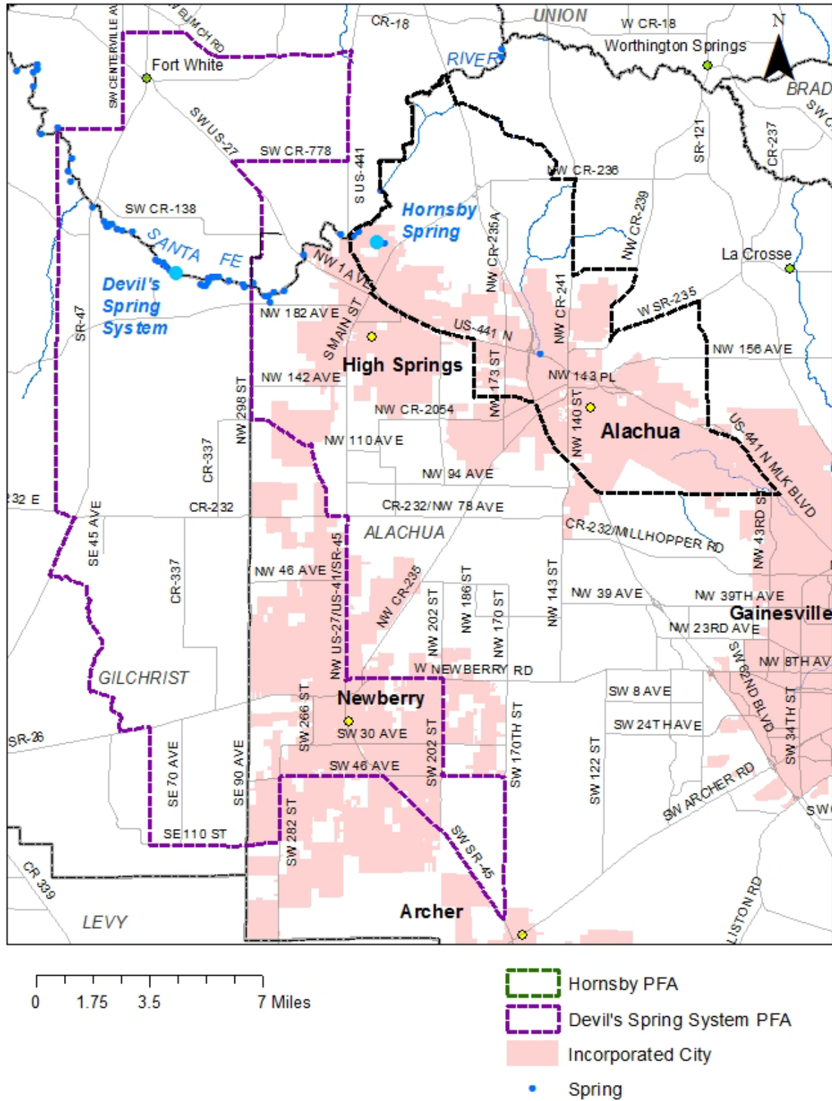
Figure 9. PFA boundaries for Devil's Spring System and Hornsby Spring
