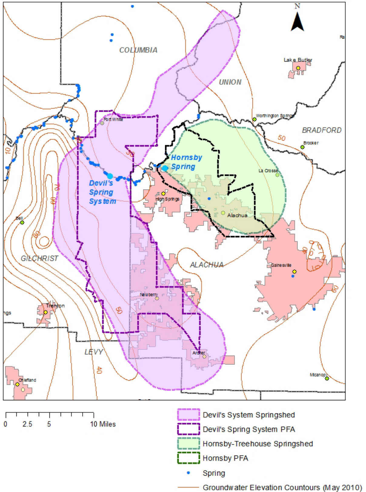
Figure 1. Devil's System and Hornsby springsheds and PFAs and groundwater elevation contours (ft-MSL)
