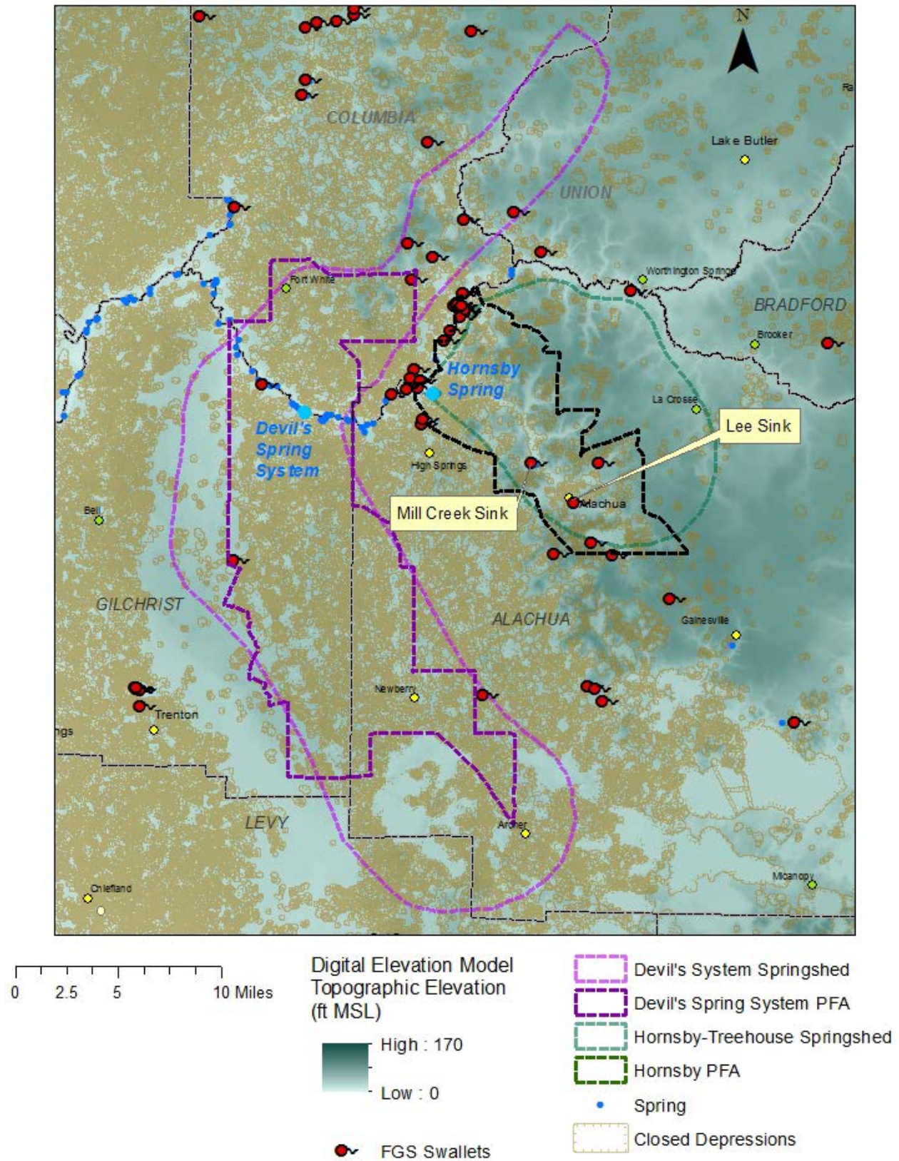
Figure 4. Digital elevation model, closed depressions and swallets in springsheds
