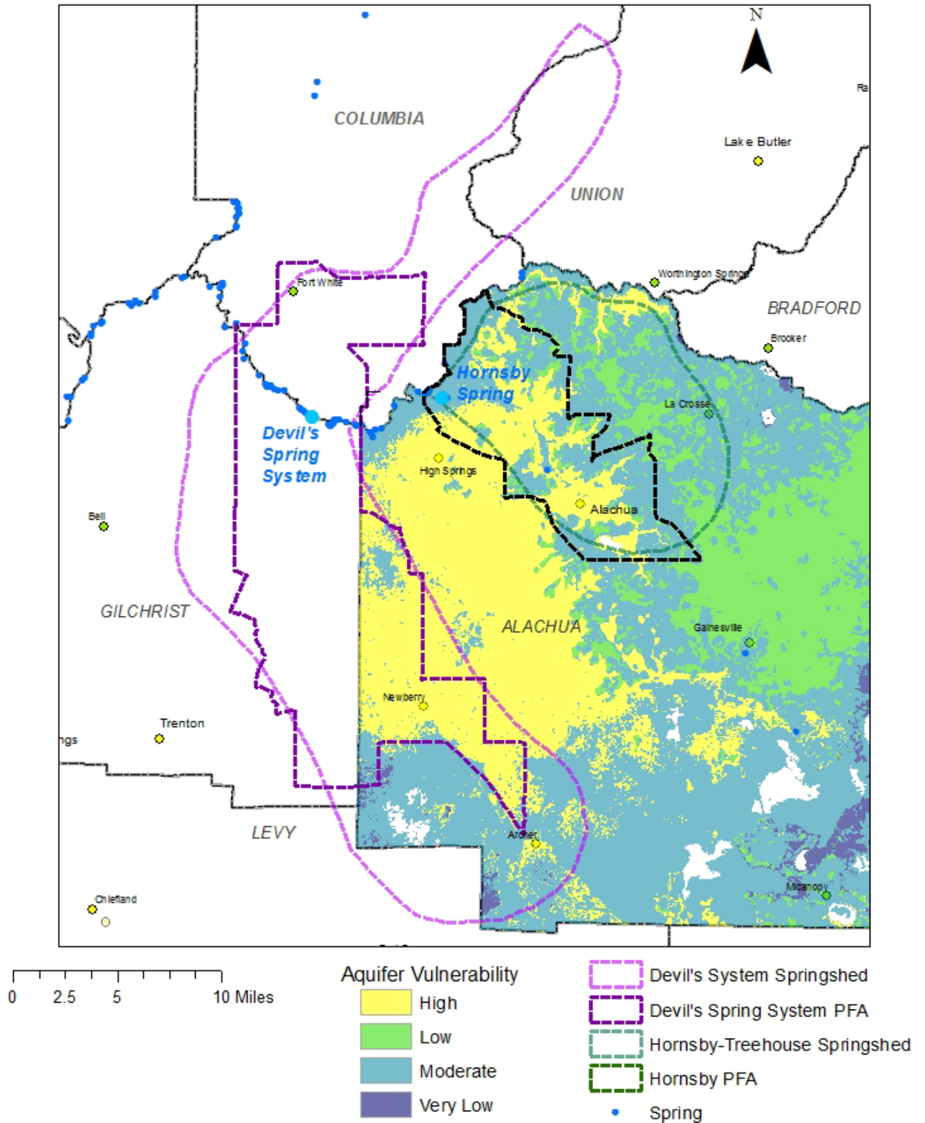
Figure 3. Floridan Aquifer Vulnerability in Alachua County portion of the springsheds
