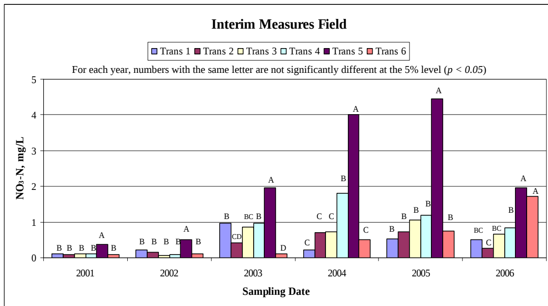
Figure 6. Average annual groundwater nitrate-N at the interim measures field.
