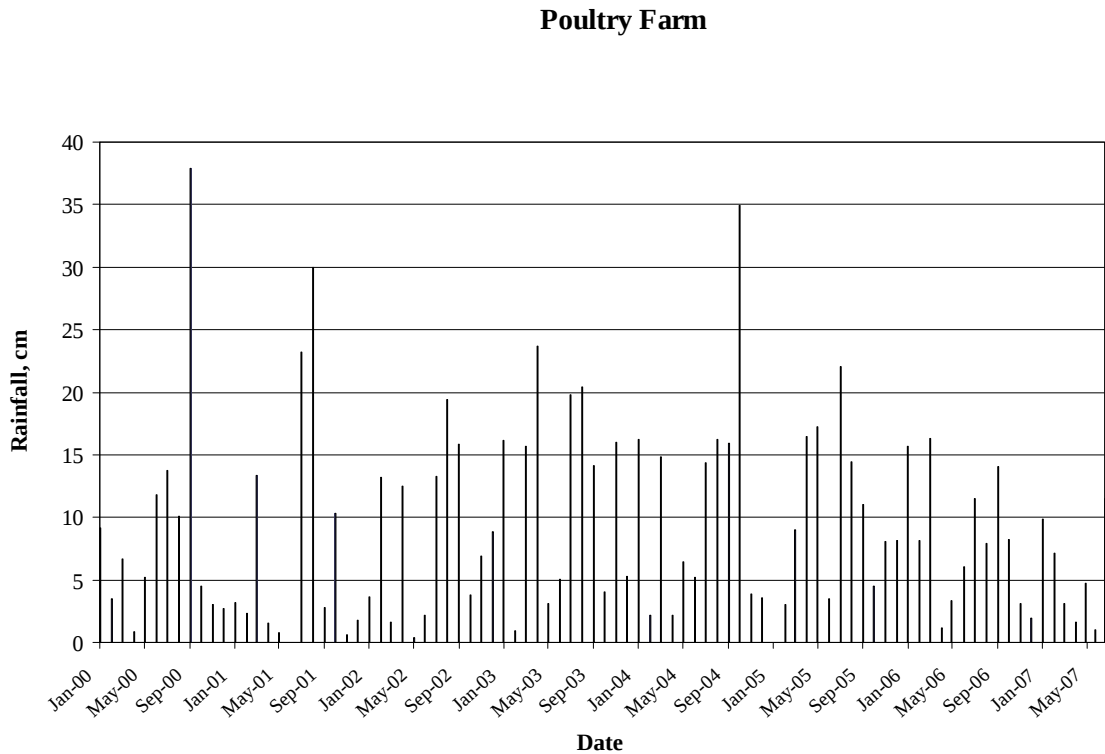
Figure 19. Monthly rainfall totals at the poultry farm.
