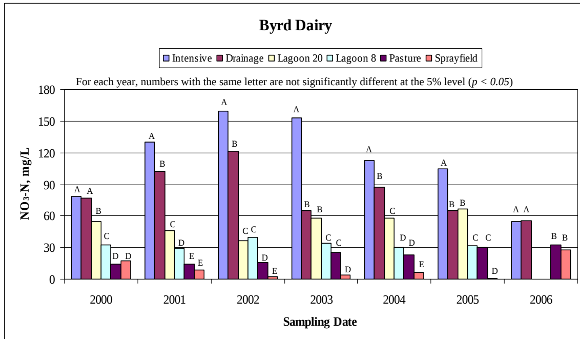
Figure 27. Average annual groundwater nitrate nitrogen at the dairy farm.
