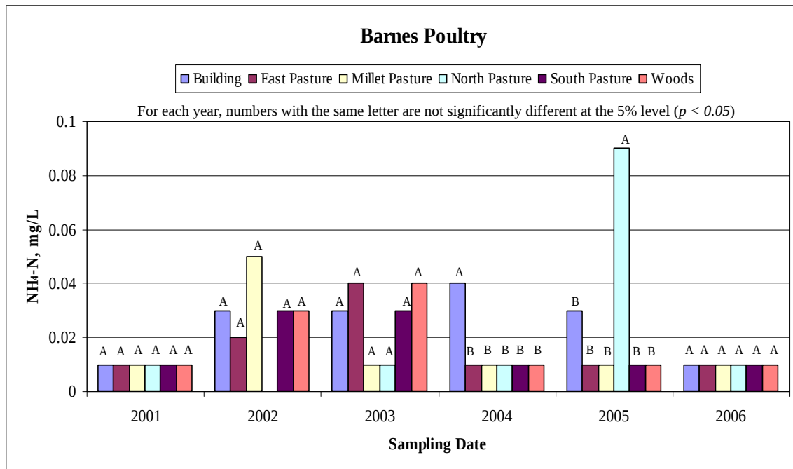
Figure 22. Average annual groundwater ammonium nitrogen at the poultry farm.
