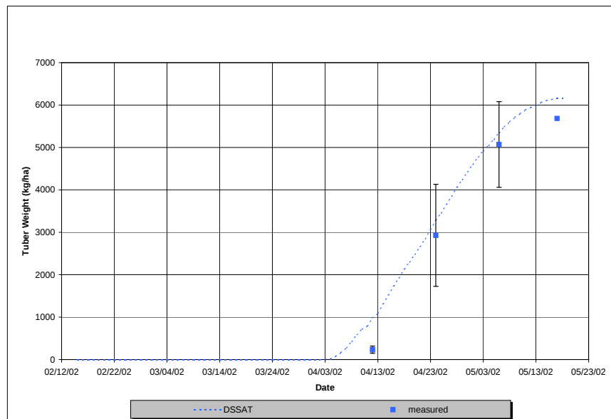
Figure 10. Measured versus predicted yield for the Spring 2002 potato crop.
