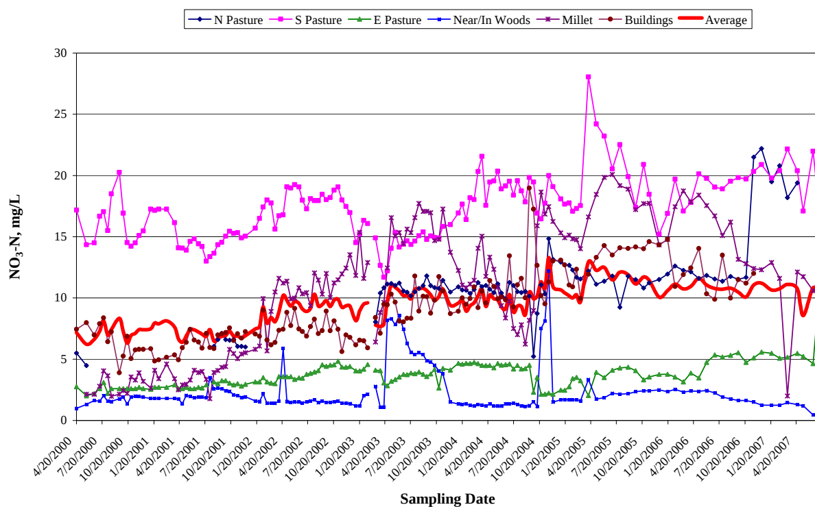
Figure 20. Groundwater nitrate-N concentrations at the poultry farm.
