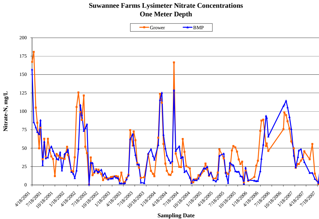
Figure 37. Nitrate-N concentrations in the one-meter lysimeters samples (soil solution) for the “grower” and “BMP” sides of the pivot.
