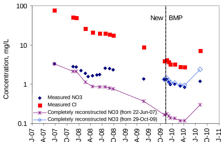
Figure 37 Measured \text{NO}_3^- and \text{Cl}^- concentrations and completely reconstructed \text{NO}_3^- concentrations at the Hunters Trace well M-0506.
