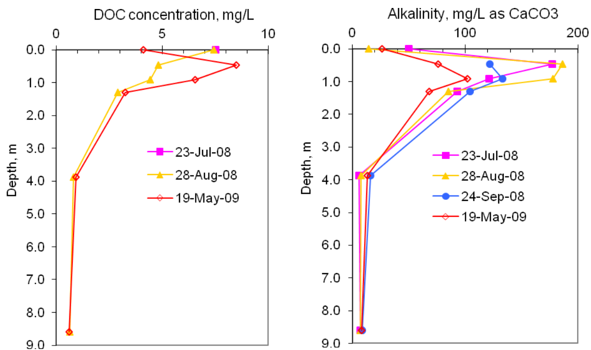
Figure 9 Soil-water and ground water chemistry profiles beneath the Hunter's Trace stormwater infiltration basin (continued on next page).
