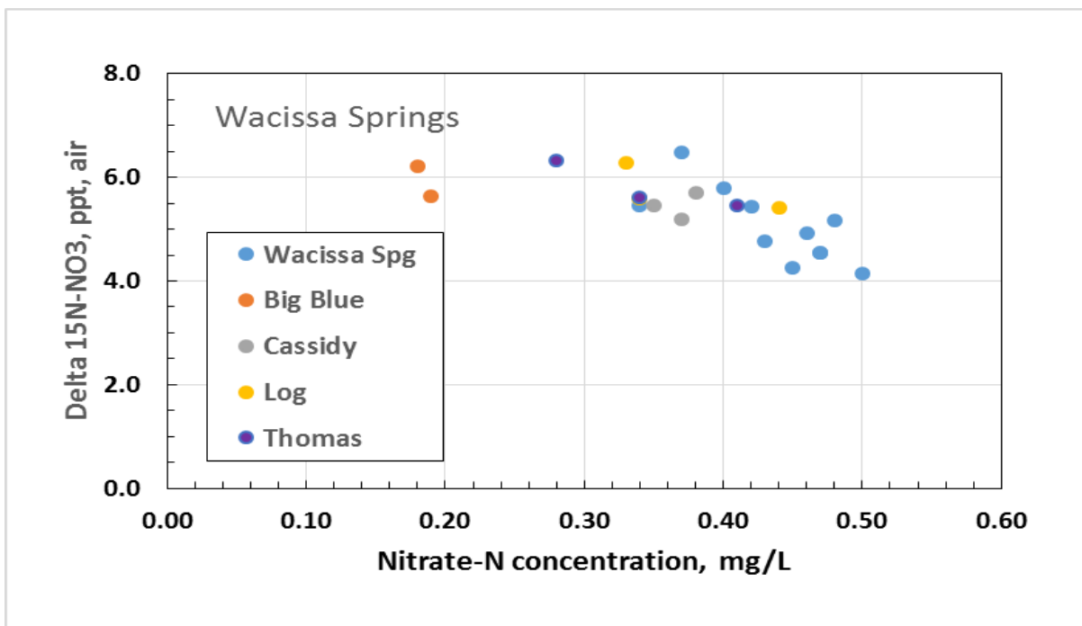
Figure 4.6. Inverse relation between nitrogen isotope values of nitrate and nitrate-N concentrations in water samples collected from Wacissa Springs, 2011–14
