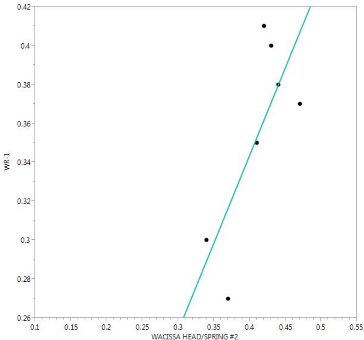
Figure 5.2. Nitrate attenuation and dilution of Wacissa Spring vs. Wacissa River (concentrations in mg/L)
