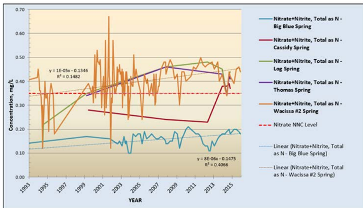
Figure 2.9. Nitrate trends in Big Blue, Cassidy, Log, Thomas and Wacissa #2 Springs, 1993–2015
