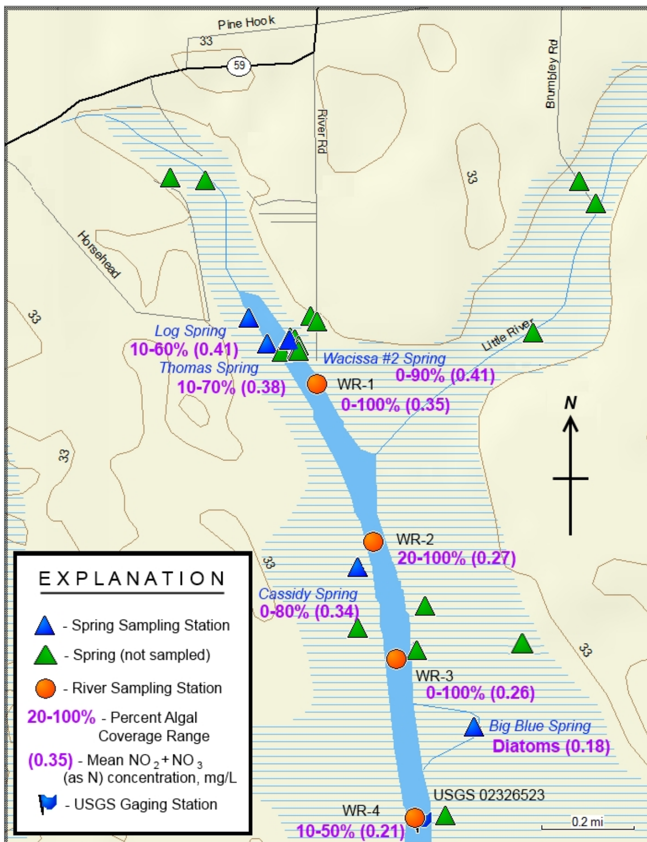
Figure 5.1. Range in filamentous algae coverage and mean \text{NO}_3 + \text{NO}_2 concentrations at vegetation survey stations
