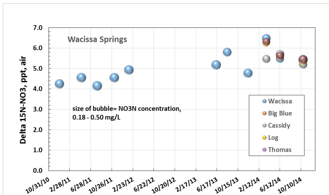
Figure 4.5. Nitrogen isotope values of nitrate in water samples collected from Wacissa Springs, 2011–14. Size of bubble is proportional to nitrate-N concentrations, which range from 0.34 to 0.50 mg/L.
