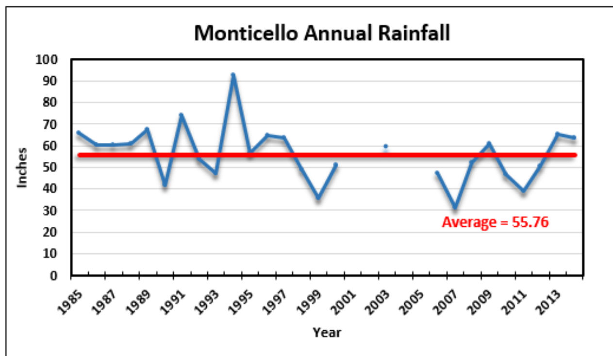
Figure 2.4. Thirty-year precipitation for Monticello, Florida, January 1985–December 2014 (FAWN and NOAA NCEI Monticello 3W Station data)
