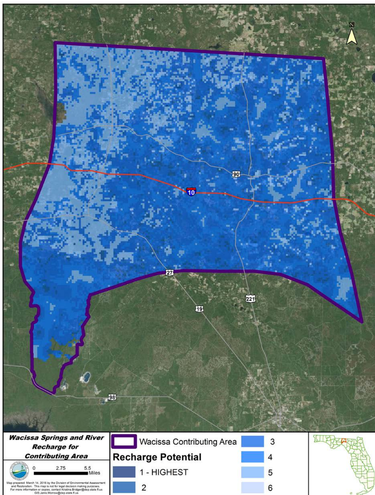
Figure 1.5. Aquifer recharge in the Wacissa River and Springs contributing area in Florida
