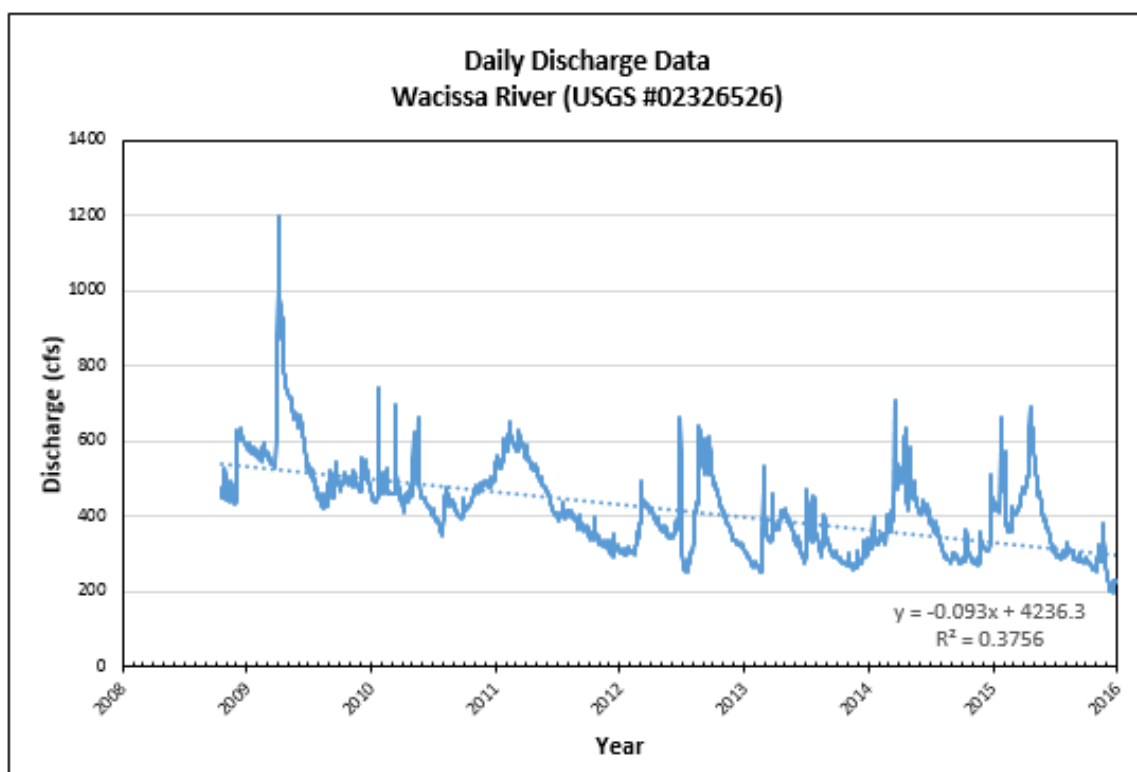
Figure 2.5. Daily mean discharge data for the Wacissa River (#02326526), October 2008–December 2015
