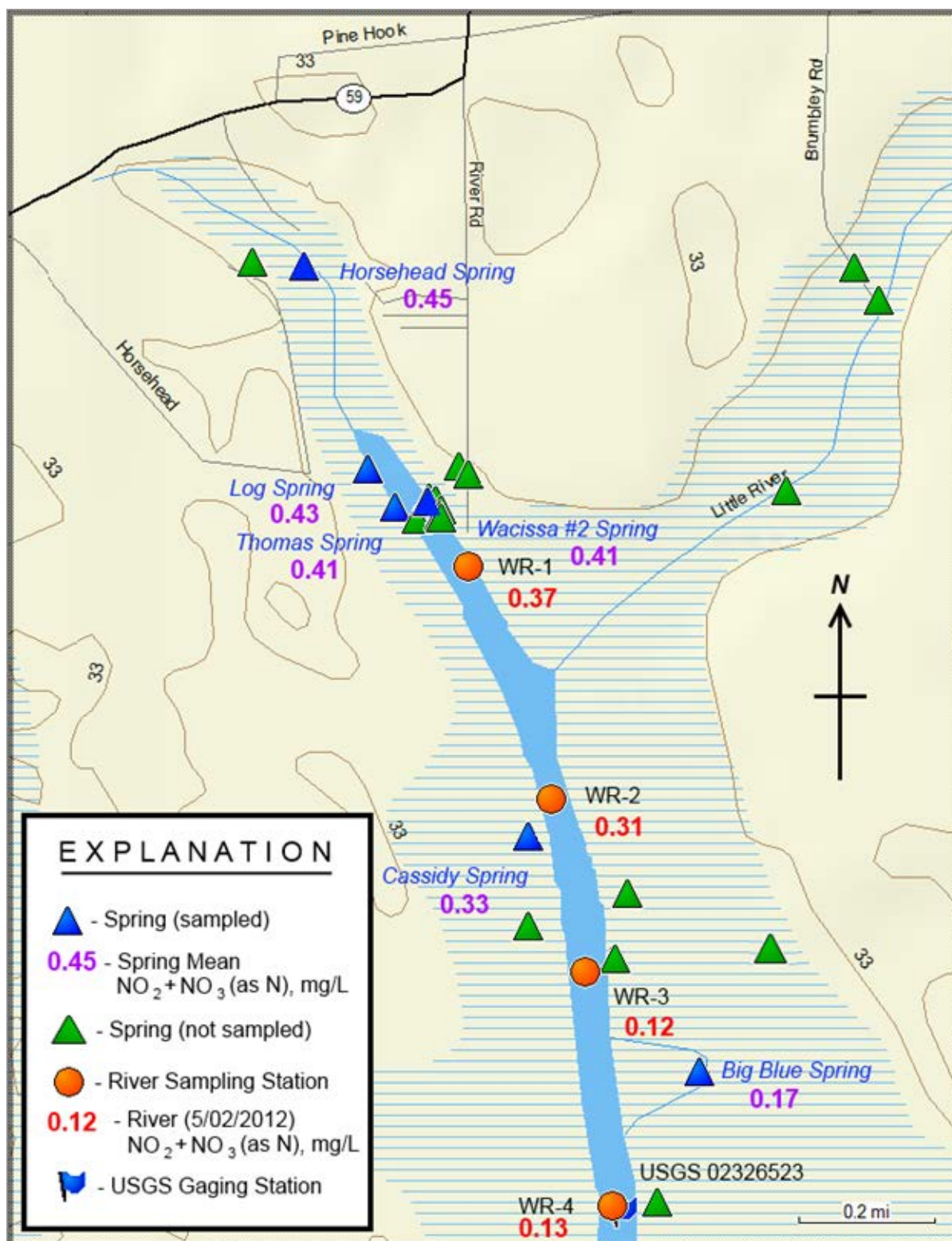
Figure 2.6. Mean nitrate values for selected springs sampled during the TMDL verified period through the present (January 2005–December 2015), along with nitrate values from Wacissa River surface water stations sampled on May 2, 2012
