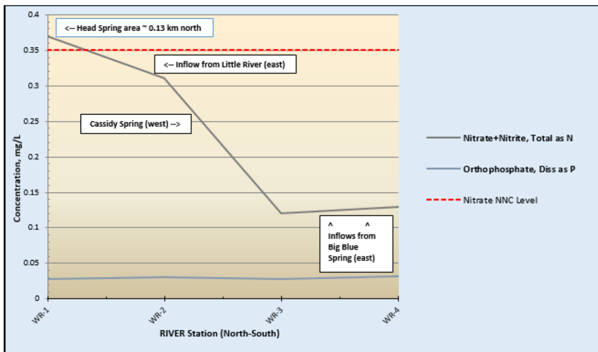
Figure 2.7. Nitrate + nitrite values in the upper Wacissa River, from surface water samples collected on May 2, 2012. See Figure 2.3 for surface water station locations.
