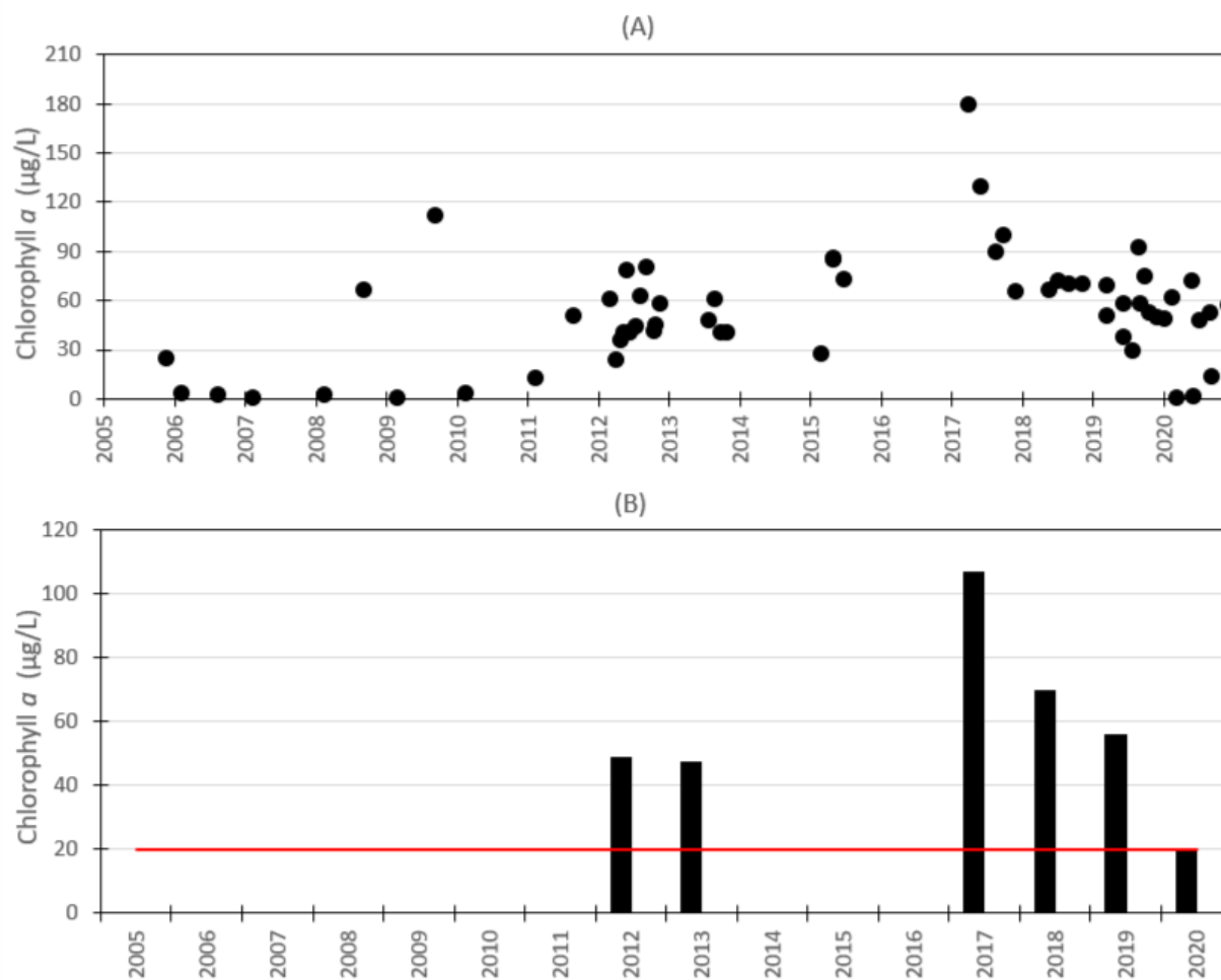
Figure 2.2. Chlorophyll a corrected measured in WBID 1547A: (a) individual sampling results, (b) AGMs in the POR. Red line represents the chlorophyll a NNC value of 20 µg/L, expressed as an AGM.
