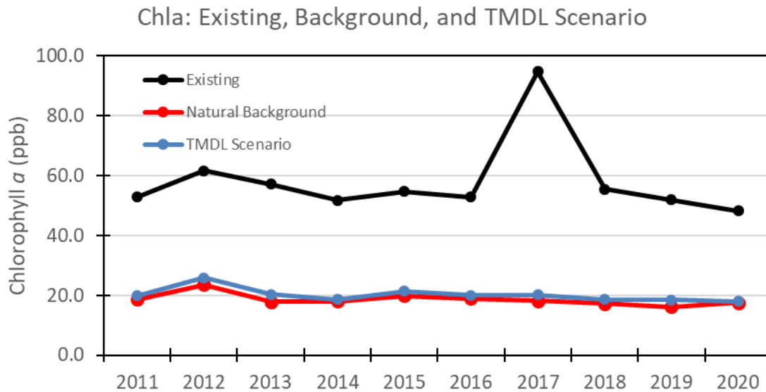
Figure 5.6. Chlorophyll a concentrations in existing, natural background, and target conditions in Lake Valrico during the BATHTUB modeling period, 2011–20
