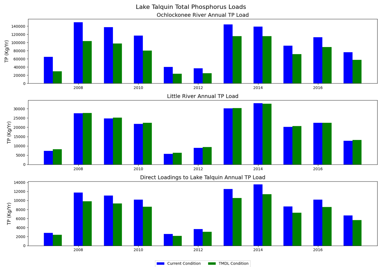
Figure 5.10. Modeled TP loads under the current condition scenario and TMDL scenario
