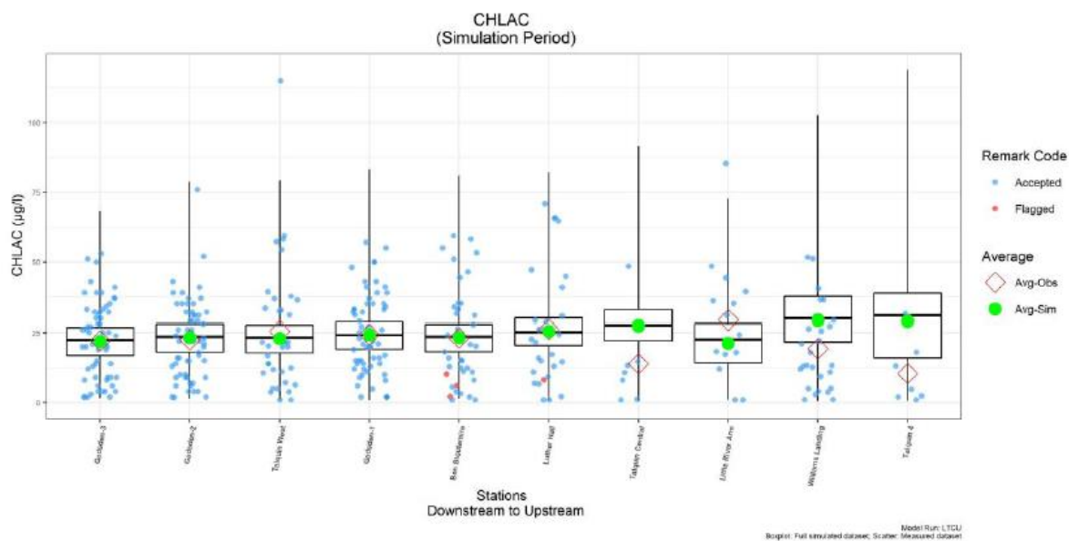
Figure 5.4. Lake Talquin chlorophyll a calibration
