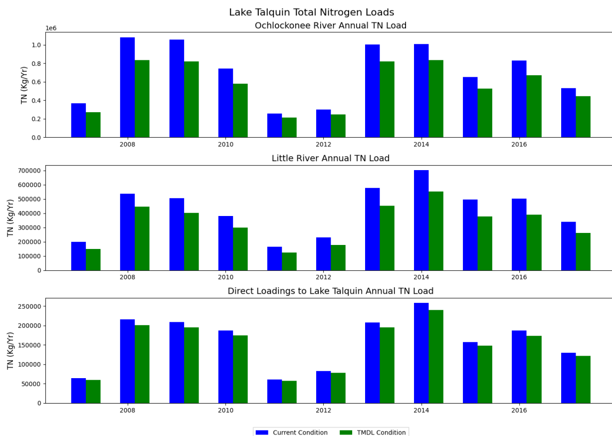
Figure 5.9. Modeled TN loads under the current condition scenario and TMDL scenario
