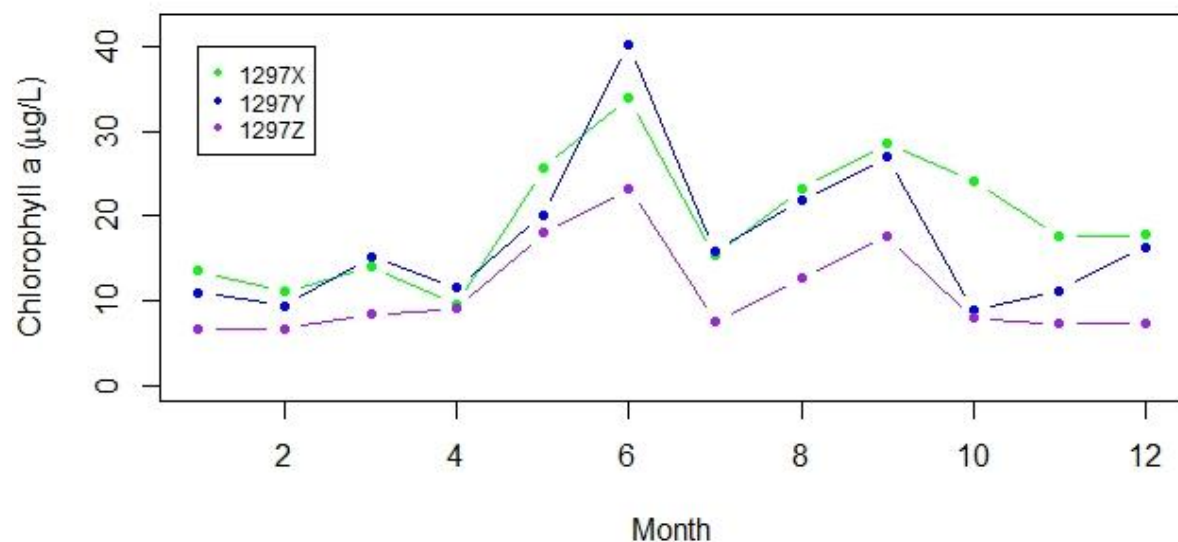
Figure 5.6. Monthly chlorophyll data in the Lake Talquin WBIDs
