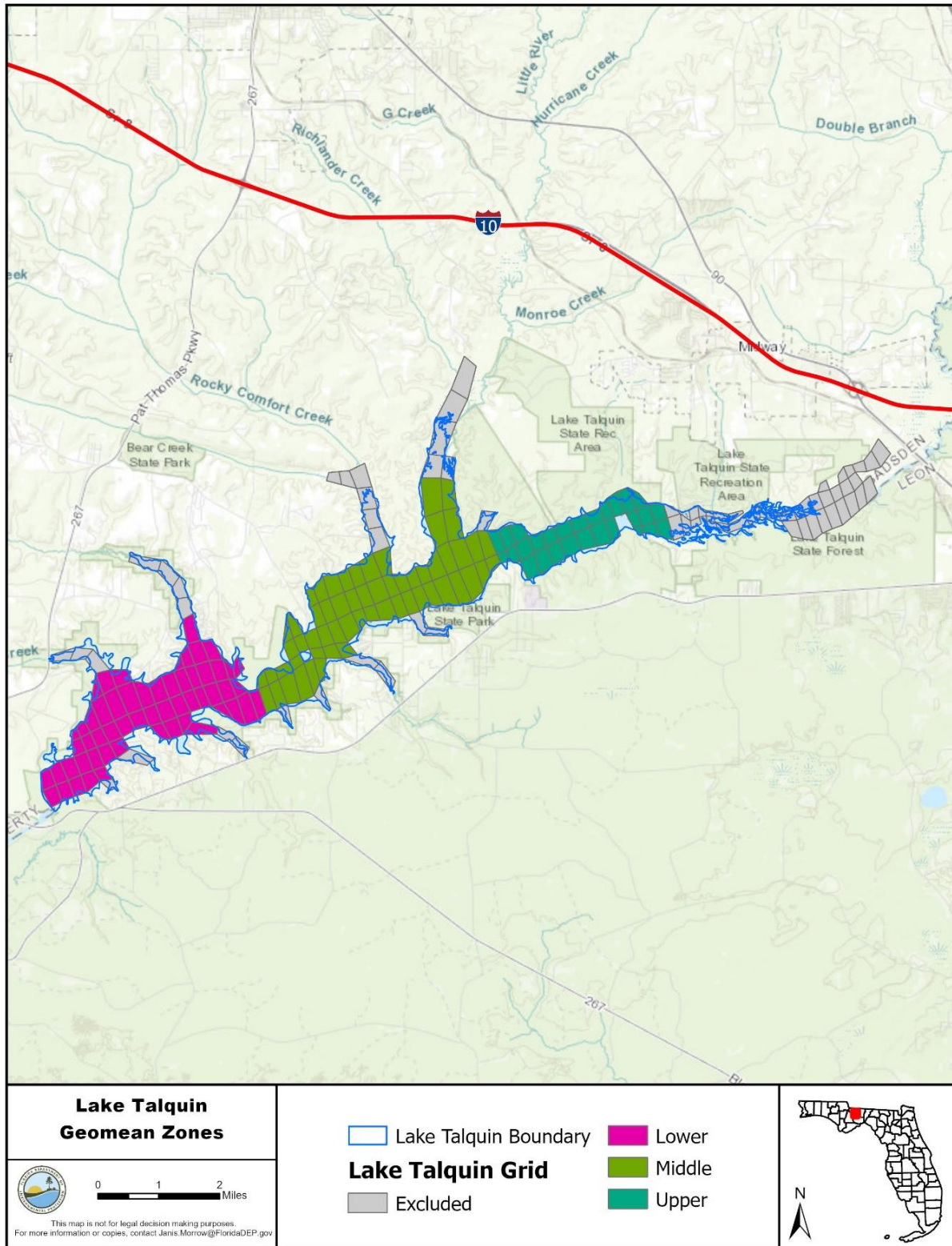
Figure 5.5. Lake Talquin model evaluation zones
