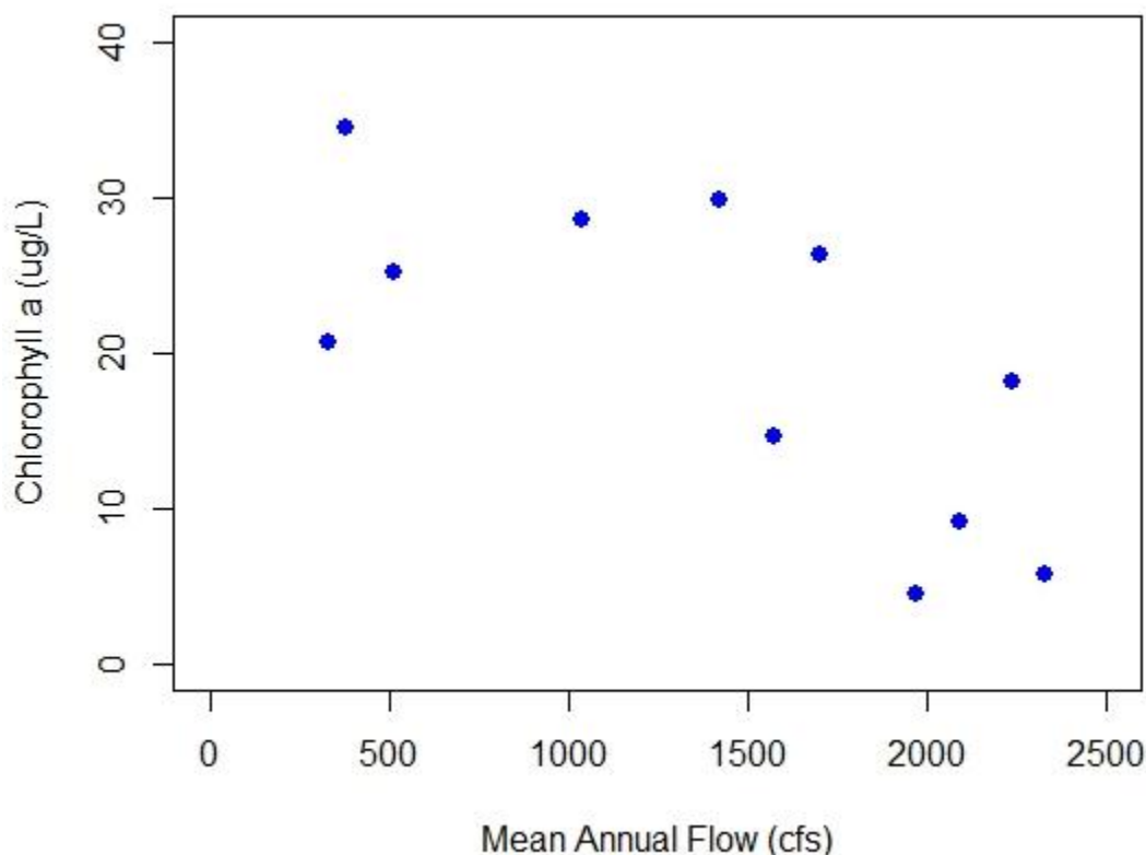
Figure 5.7. AGM chlorophyll a in the Lower Lake Talquin WBID plotted as a function of mean annual flow at the Bloxom Cutoff Road USGS station (2008–18)
