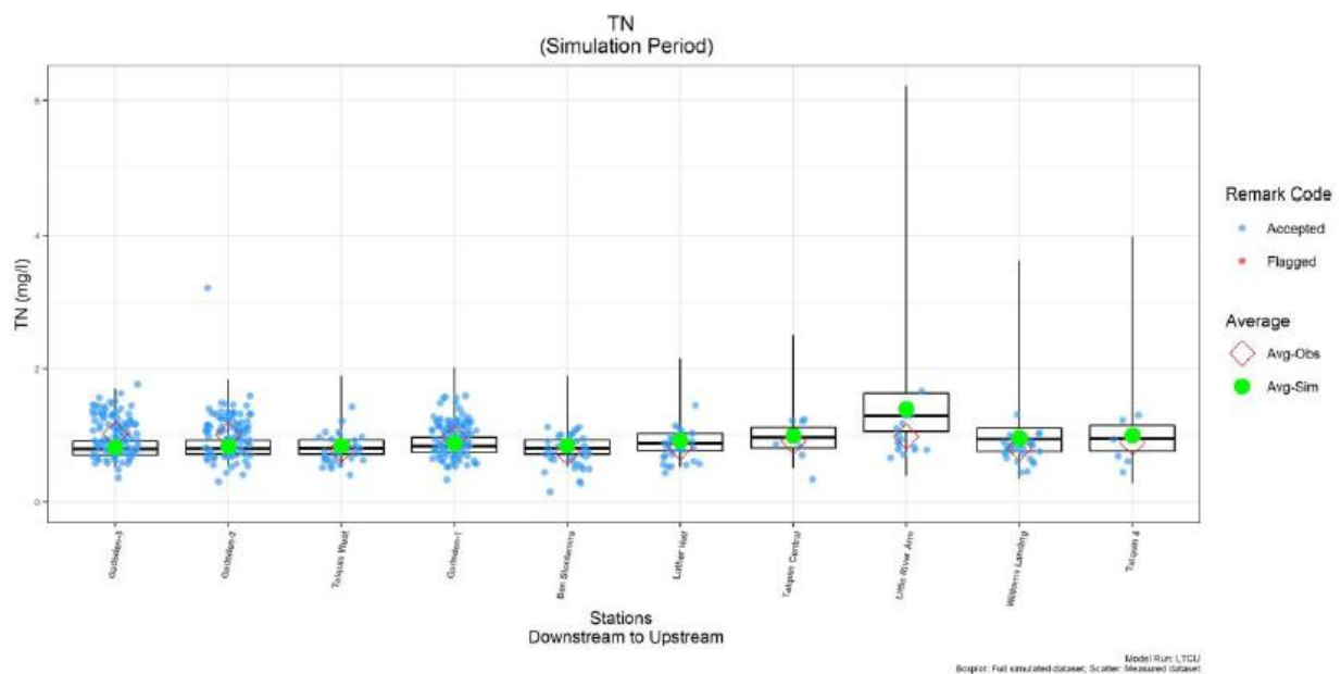
Figure 5.2. Lake Talquin TN calibration
