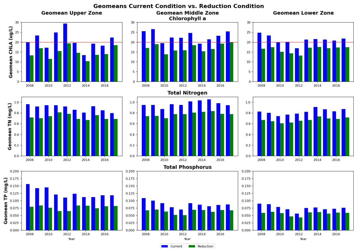
Figure 5.8. Annual geometric mean TN, TP, and chlorophyll a in Lake Talquin
