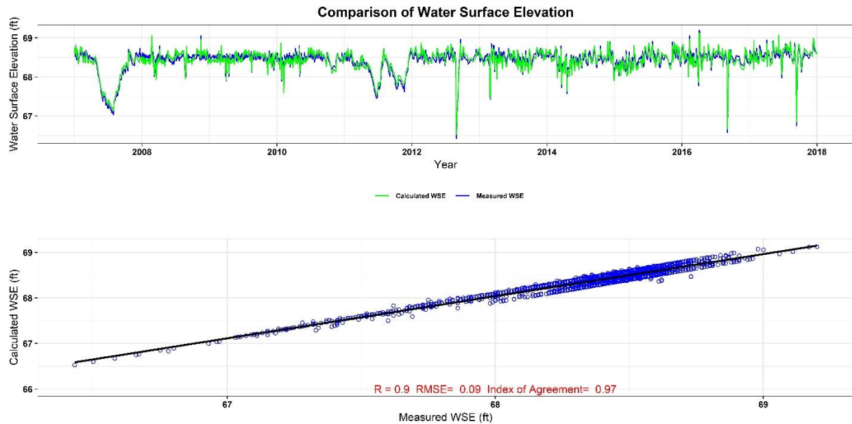
Figure 5.1. Lake surface elevation calibration in EFDC
