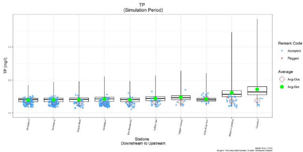
Figure 5.3. Lake Talquin TP calibration
