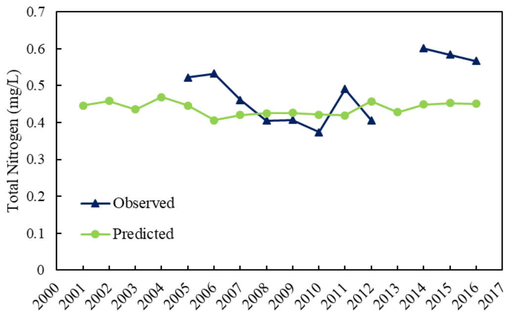
Figure 5.8. Predicted and observed TN concentrations for Lake McLeod
