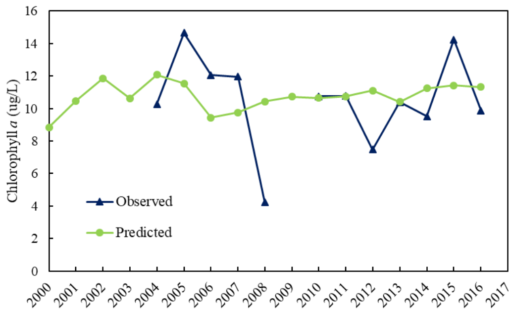
Figure 5.4. Predicted and observed chlorophyll a concentrations for Lake Agnes
