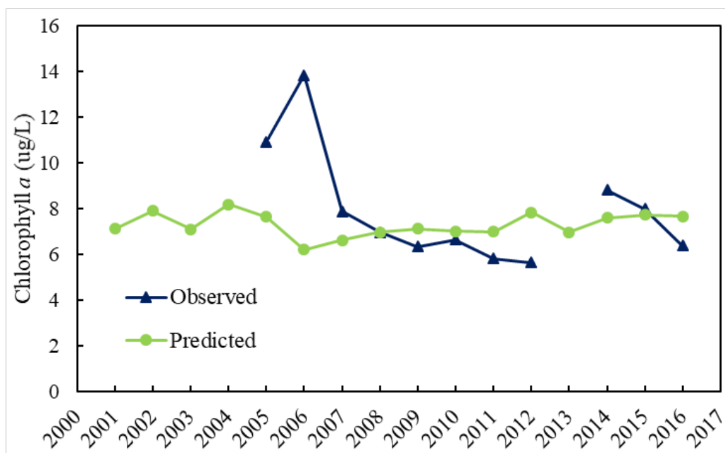
Figure 5.7. Predicted and observed chlorophyll a concentrations for Lake McLeod
