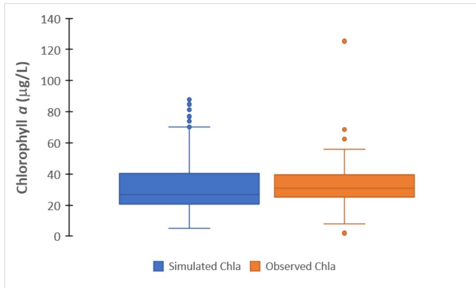
Figure 5.11. Box-whisker plot of simulated versus observed chlorophyll a (µg/L) in Lake Istokpoga
