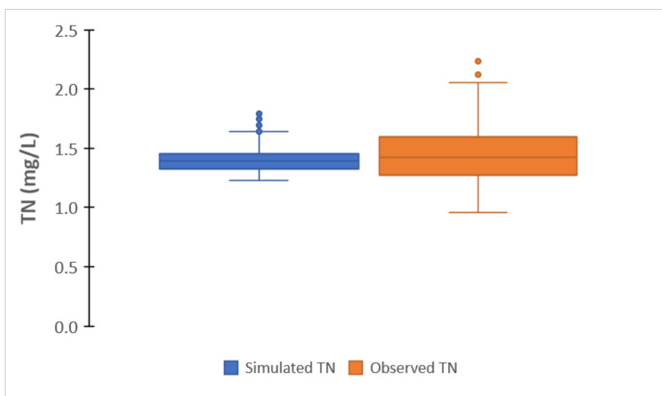
Figure 5.3. Box-whisker plot of simulated versus observed TN (mg/L) in Lake Istokpoga
