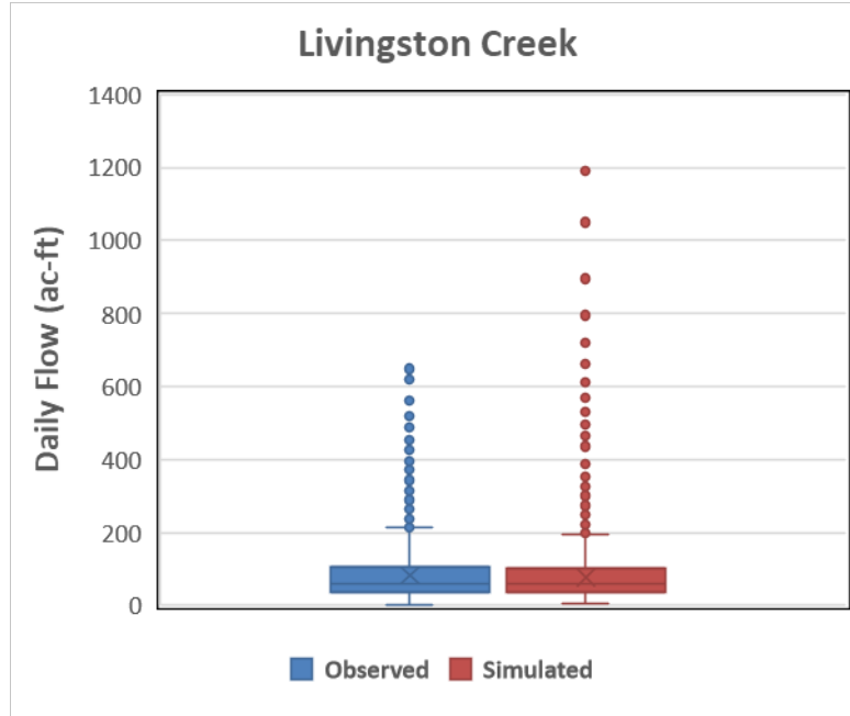
Figure D-6. Box-whisker plot of simulated versus observed daily flows at Livingston Creek during the calibration period
