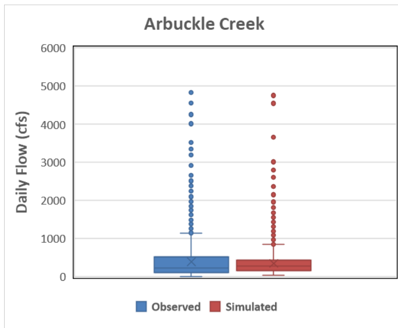
Figure 4.13. Box-whisker plot of simulated versus observed daily flow at Arbuckle Creek during the calibration period. The symbol X represents the mean.
