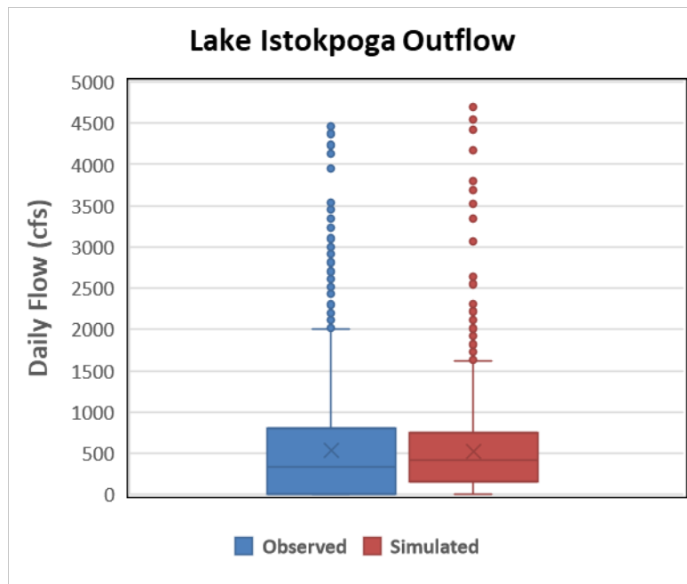
Figure 4.15. Box-whisker plot of simulated versus observed daily flow at S-68 during the calibration period. The symbol X represents the mean.
