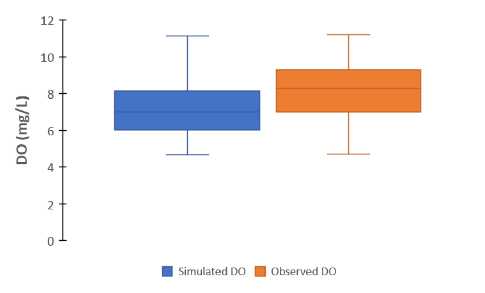
Figure D-12. Box-whisker plot of simulated versus observed DO (mg/L) in Lake Istokpoga
