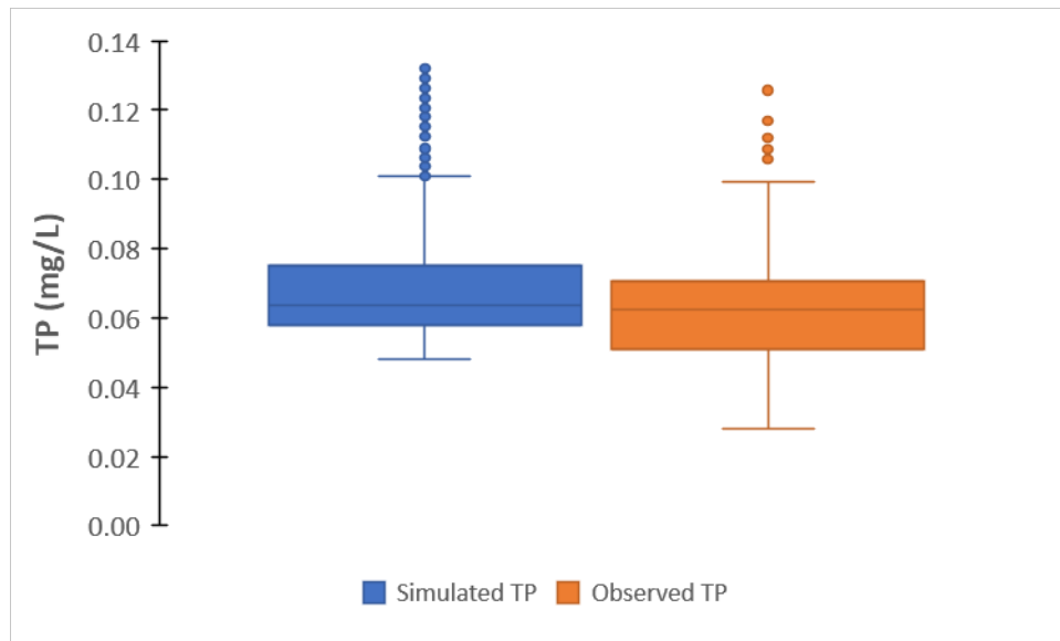
Figure 5.7. Box-whisker plot of simulated versus observed TP (mg/L) in Lake Istokpoga
