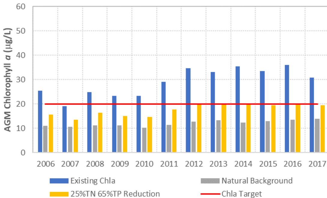
Figure 5.18. Chlorophyll a AGMs (µg/L) in Lake Istokpoga for existing, natural background, and load reduction conditions
