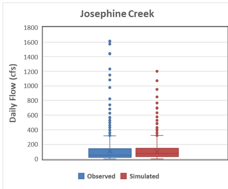
Figure 4.11. Box-whisker plot of simulated versus observed daily flow at Josephine Creek during the calibration period. The symbol X represents the mean.
