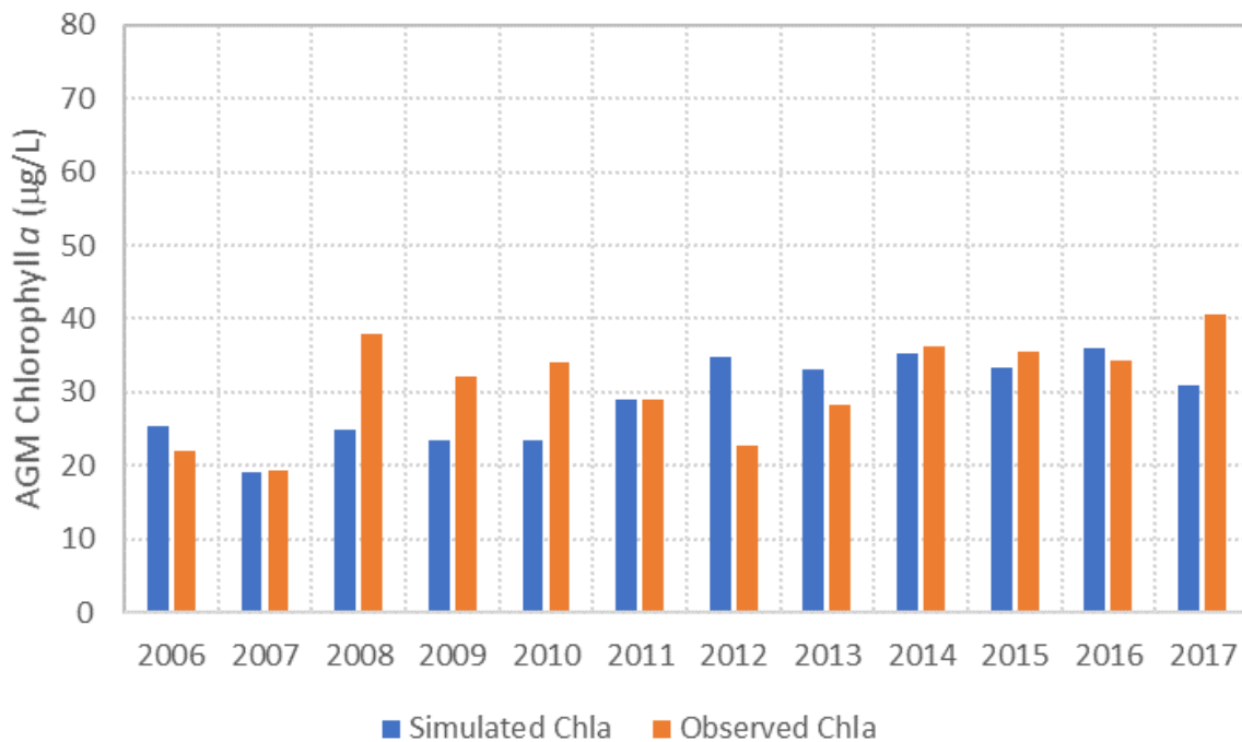
Figure 5.12. AGMs of simulated versus observed chlorophyll a (µg/L) in Lake Istokpoga
