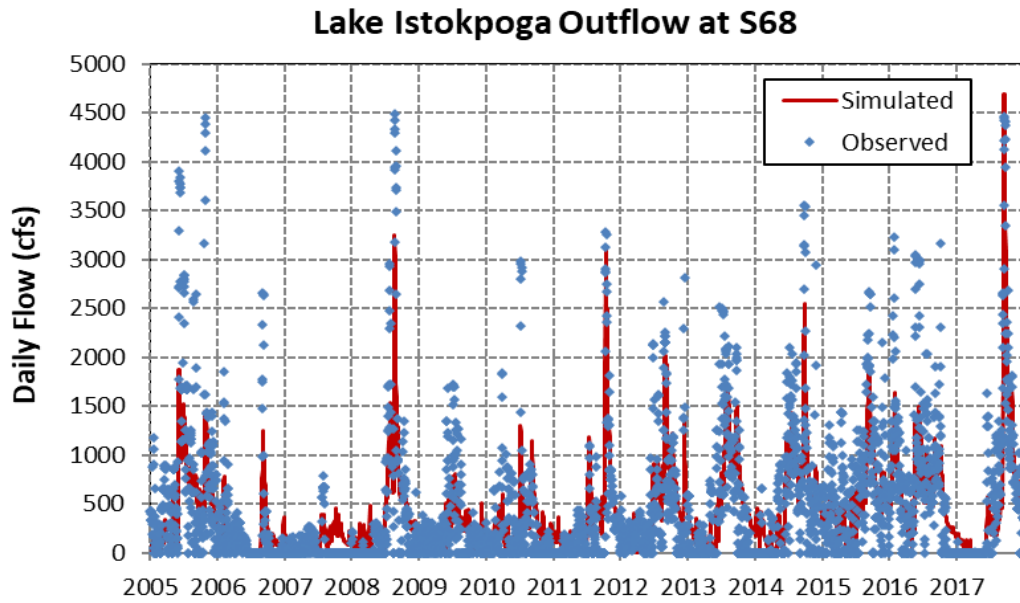
Figure 4.6. Time-series comparison of model results with observed flow at S-68
