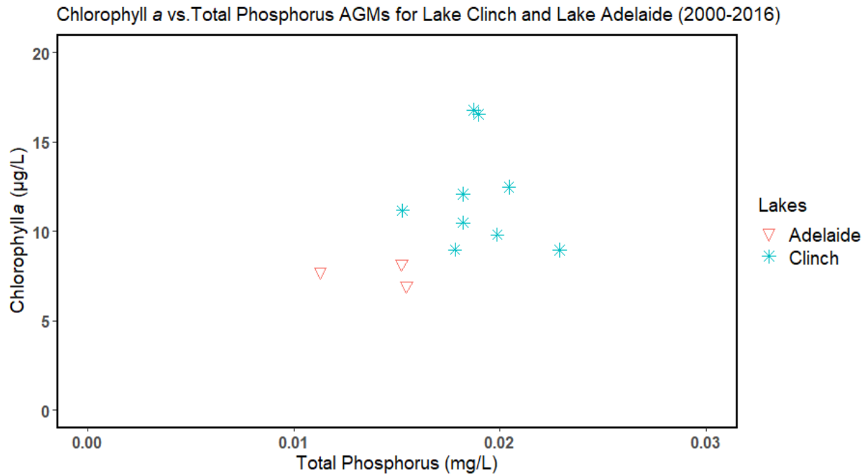
Figure 5.12. Relationship between AGM results for chlorophyll a and TP for Lake Clinch and Lake Adelaide (2000–16)
