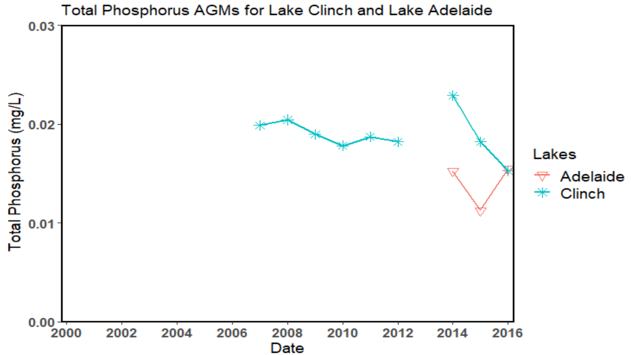
Figure 5.6. TP AGM values for Lake Clinch and Lake Adelaide (2000–16)
