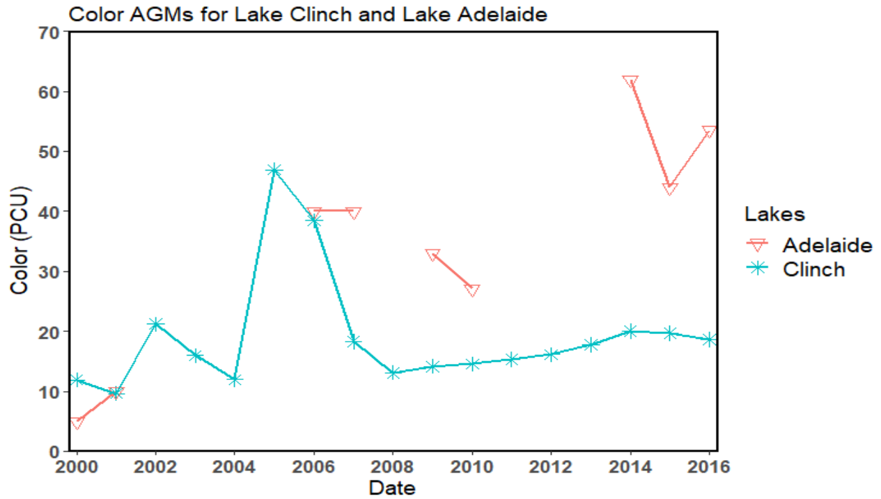
Figure 5.8. Color AGM values for Lake Clinch and Lake Adelaide (2000–16)
