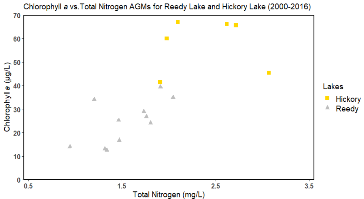
Figure 5.9. Relationship between AGM results for chlorophyll a and TN for Reedy Lake and Hickory Lake (2000–16)
