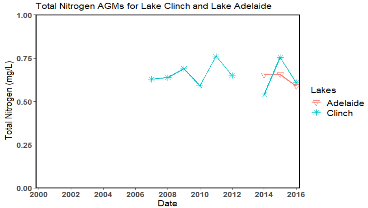
Figure 5.4. TN AGM values for Lake Clinch and Lake Adelaide (2000–16)
