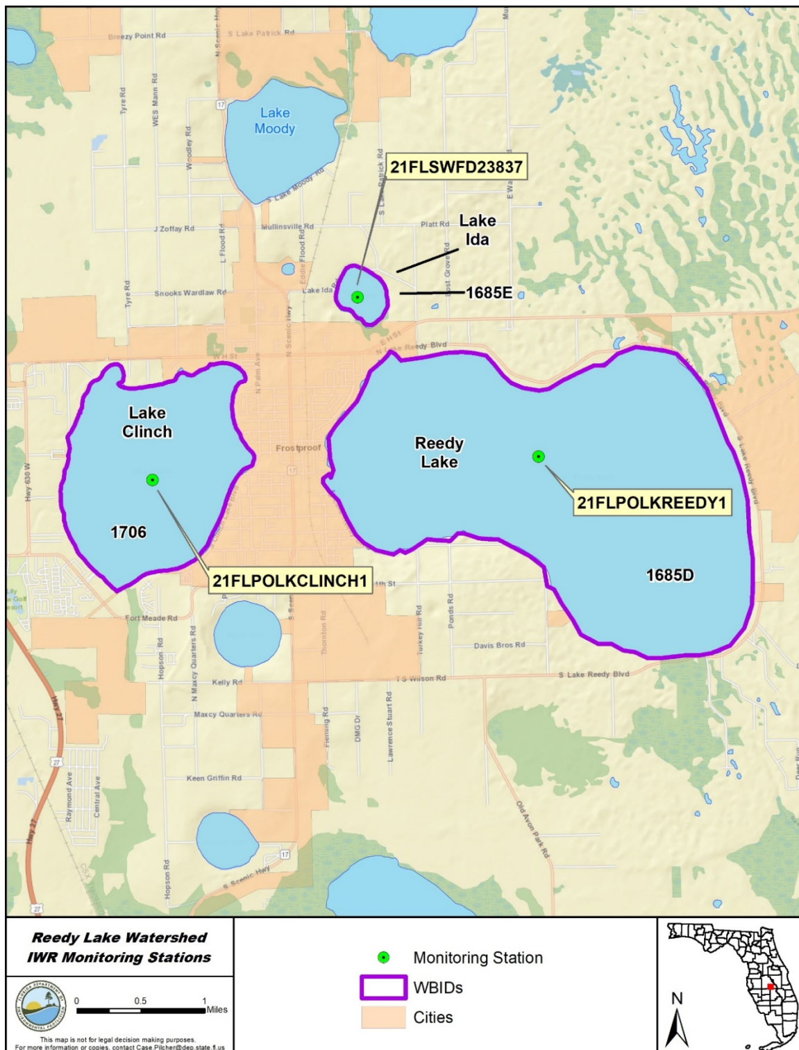
Figure 2.1. Monitoring stations in the Reedy Lake, Lake Ida, and Lake Clinch Watershed
