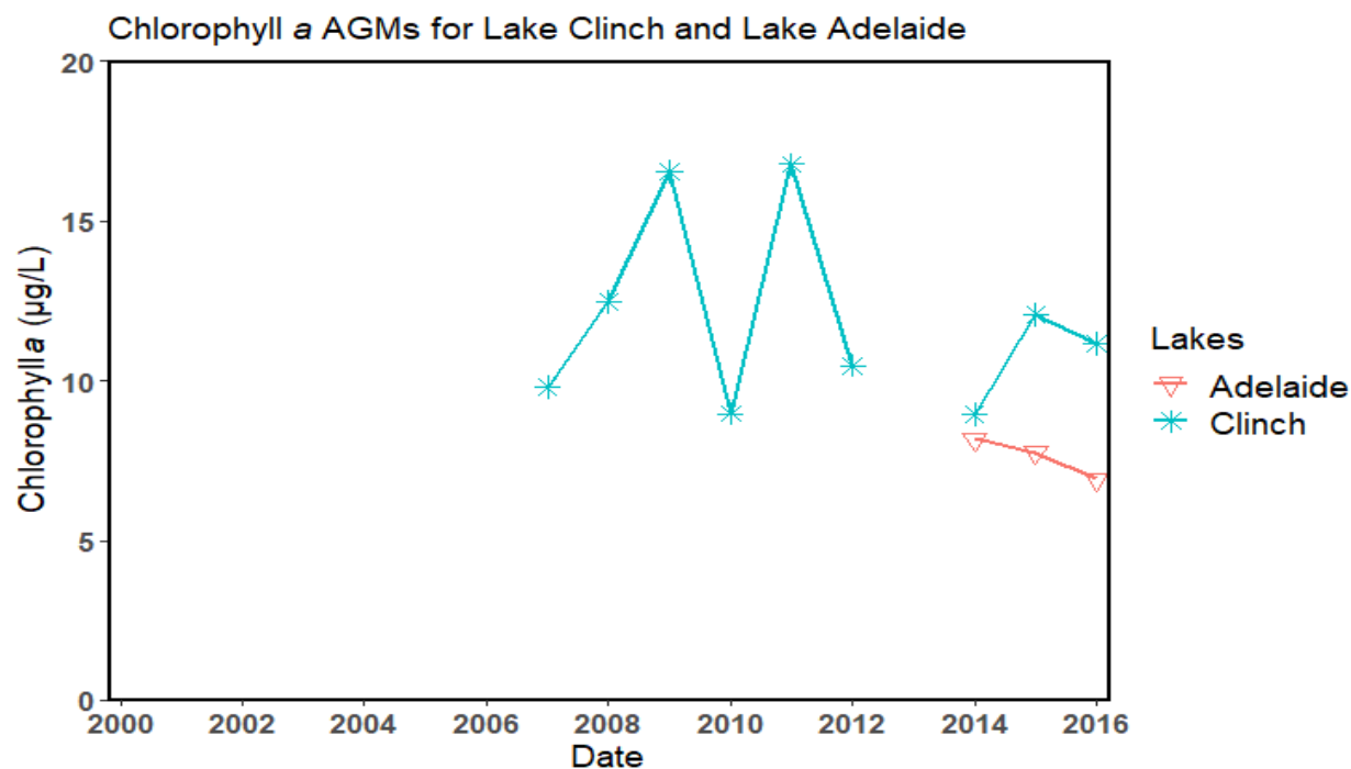
Figure 5.2. Chlorophyll a AGM values for Lake Clinch and Lake Adelaide (2000–16)
