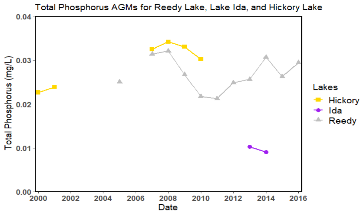
Figure 5.5. TP AGM values for Reedy Lake, Lake Ida, and Hickory Lake (2000–16)
