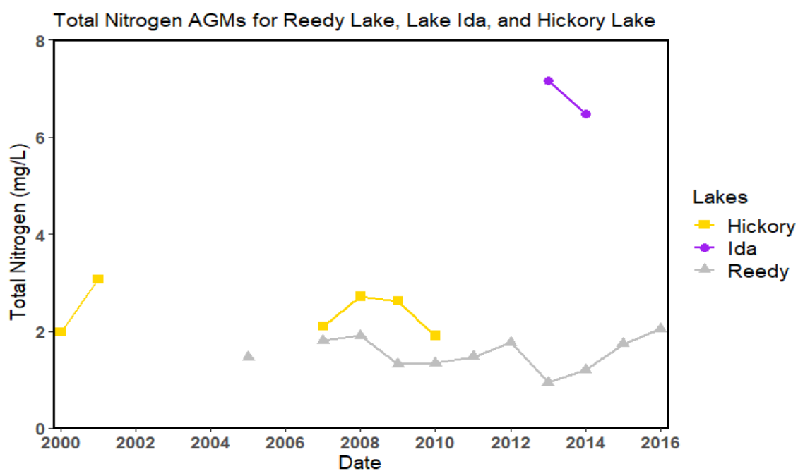
Figure 5.3. TN AGM values for Reedy Lake, Lake Ida, and Hickory Lake (2000–16)
