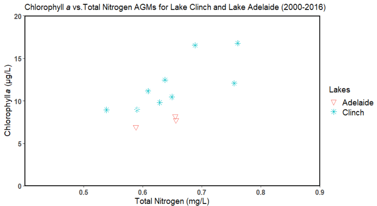
Figure 5.11. Relationship between AGM results for chlorophyll a and TN for Lake Clinch and Lake Adelaide (2000–16)
