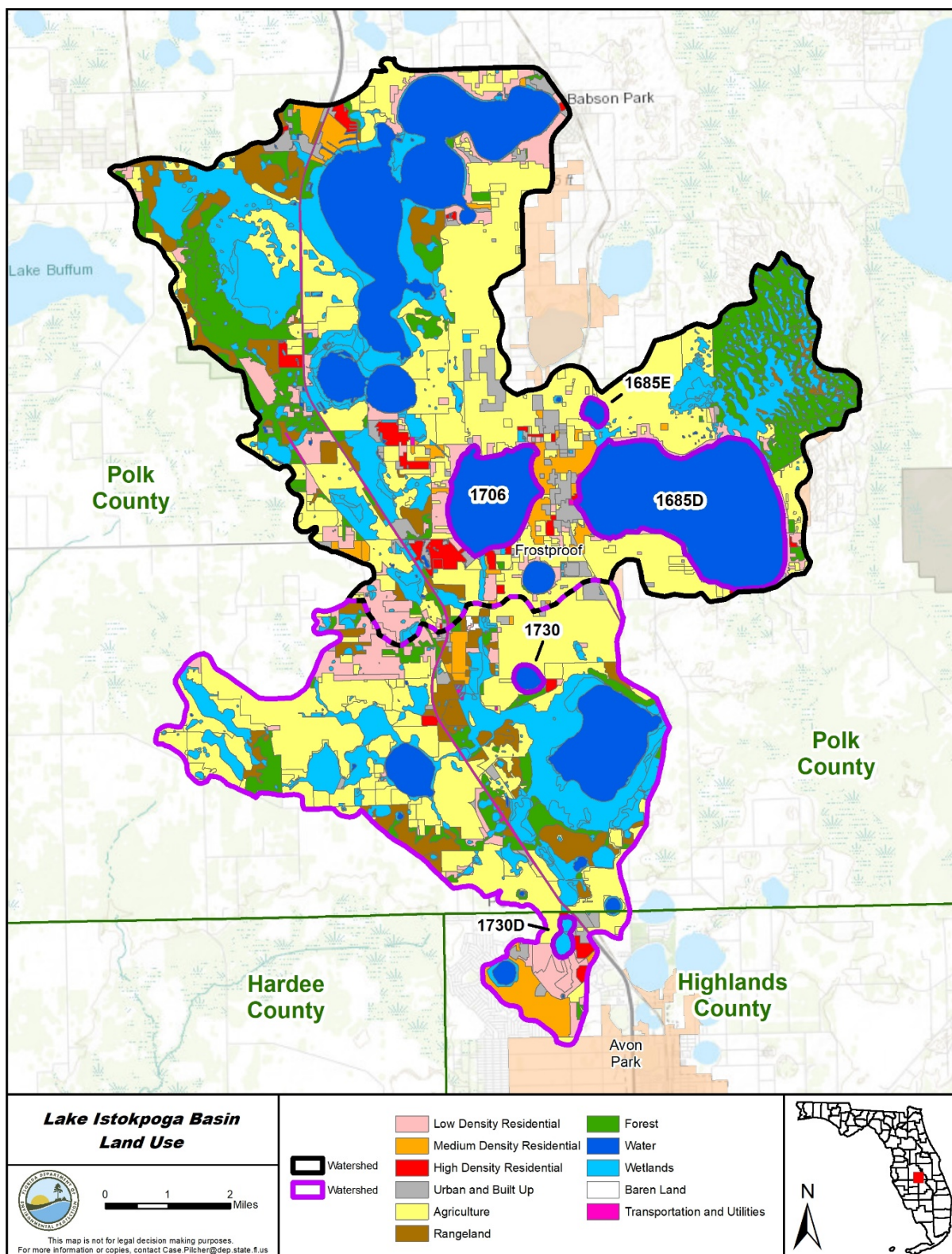
Figure 4.1. Land use in the two watersheds in 2014
