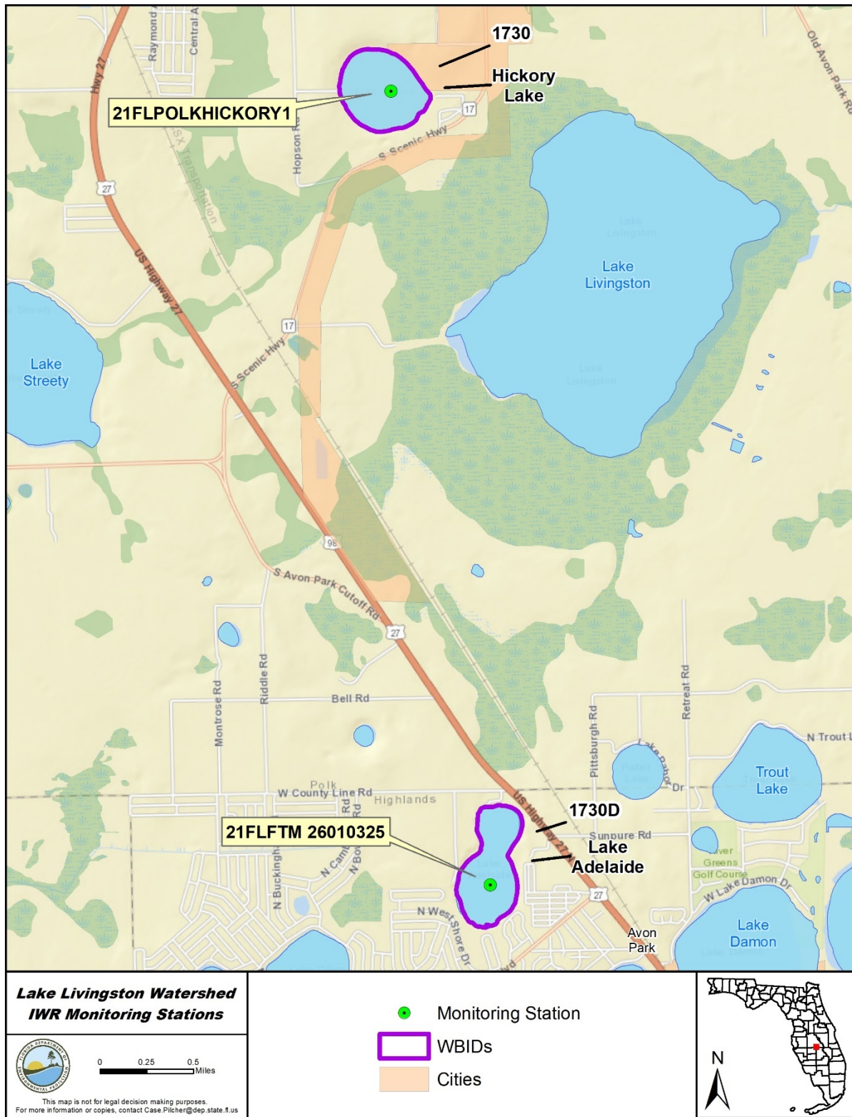
Figure 2.2. Monitoring stations in the Hickory Lake and Lake Adelaide Watershed
