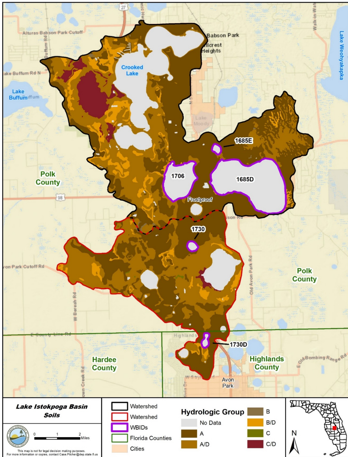
Figure 1.2. Hydrologic soil groups in the watersheds
