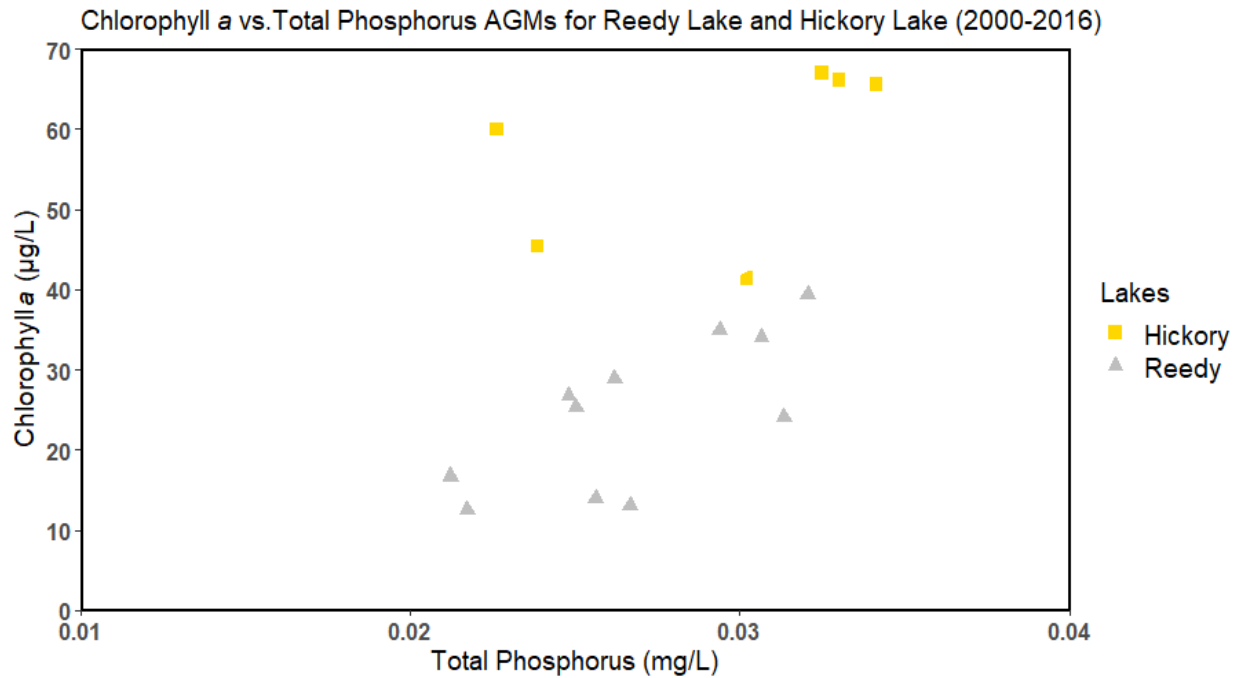
Figure 5.10. Relationship between AGM results for chlorophyll a and TP for Reedy Lake and Hickory Lake (2000–16)
