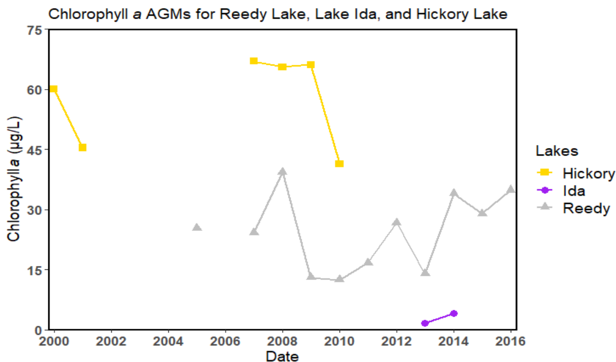
Figure 5.1. Chlorophyll a AGM values for Reedy Lake, Lake Ida, and Hickory Lake (2000–16)
