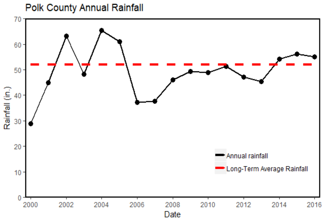
Figure 5.13. Annual rainfall in Polk County, 2000–16
