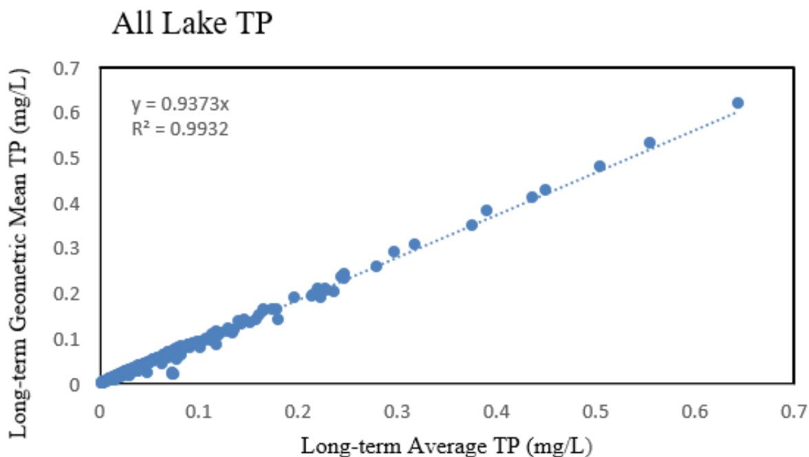
Figure 5.14. Relationship between TP AGMs and averages (arithmetic means) from lake results used in NNC development
