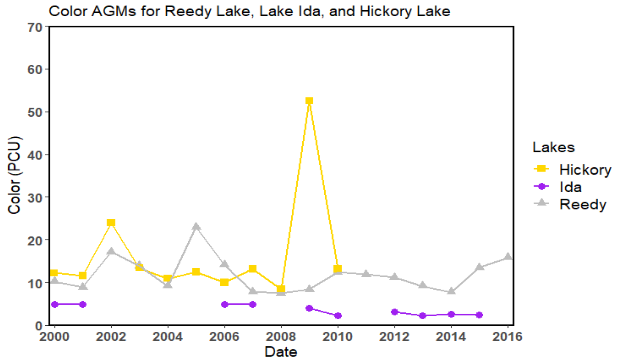
Figure 5.7. Color AGM values for Reedy Lake, Lake Ida, and Hickory Lake (2000–16)
