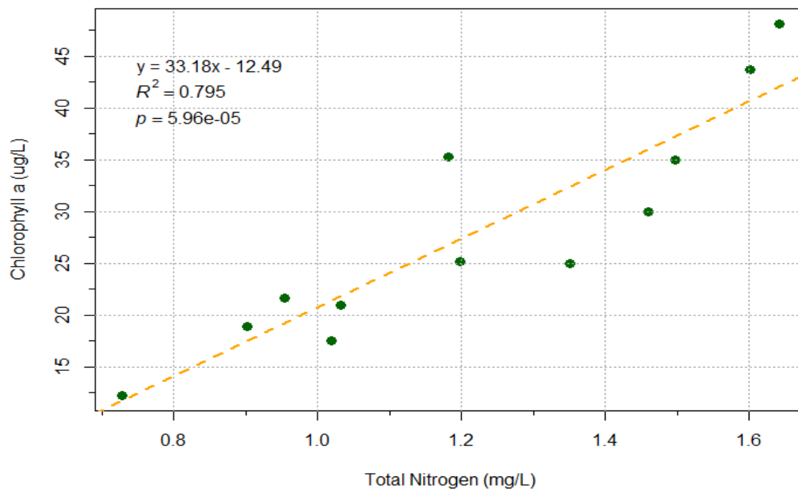
Figure 5.3. Relationship between Lake Wales chlorophyll a and TN AGMs, 2005–16
