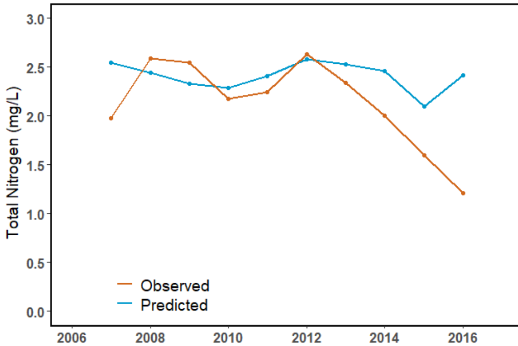
Figure 5.8. Predicted and observed TN for Lake Pierce
