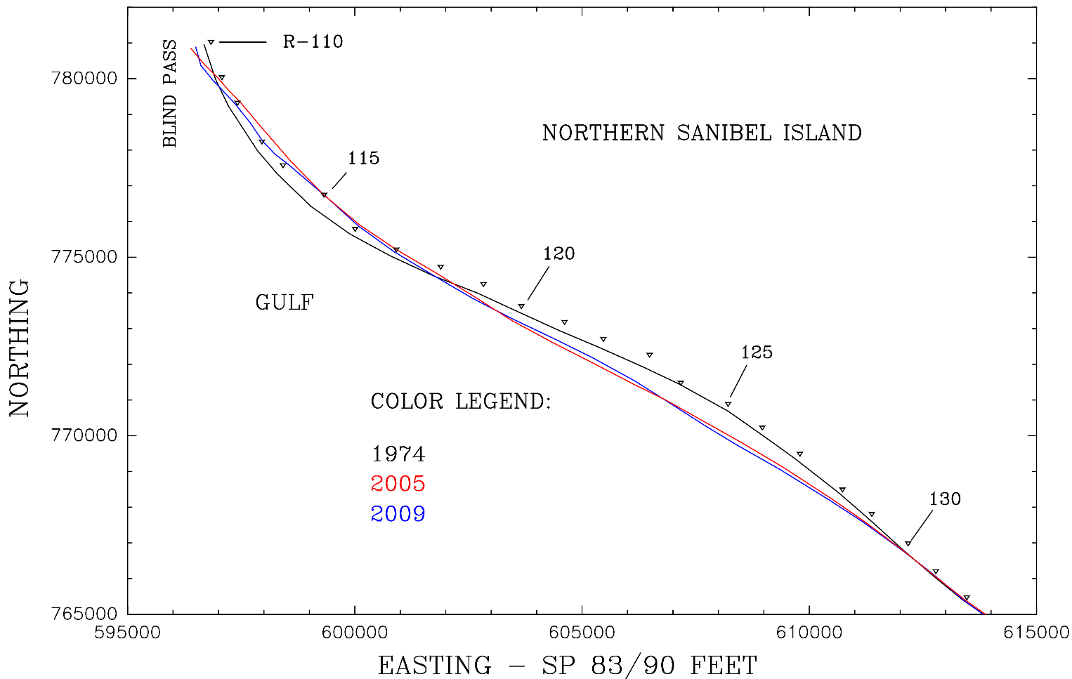
PLAN VIEW MHW SHORELINES - LEE CO., SANIBEL #1
