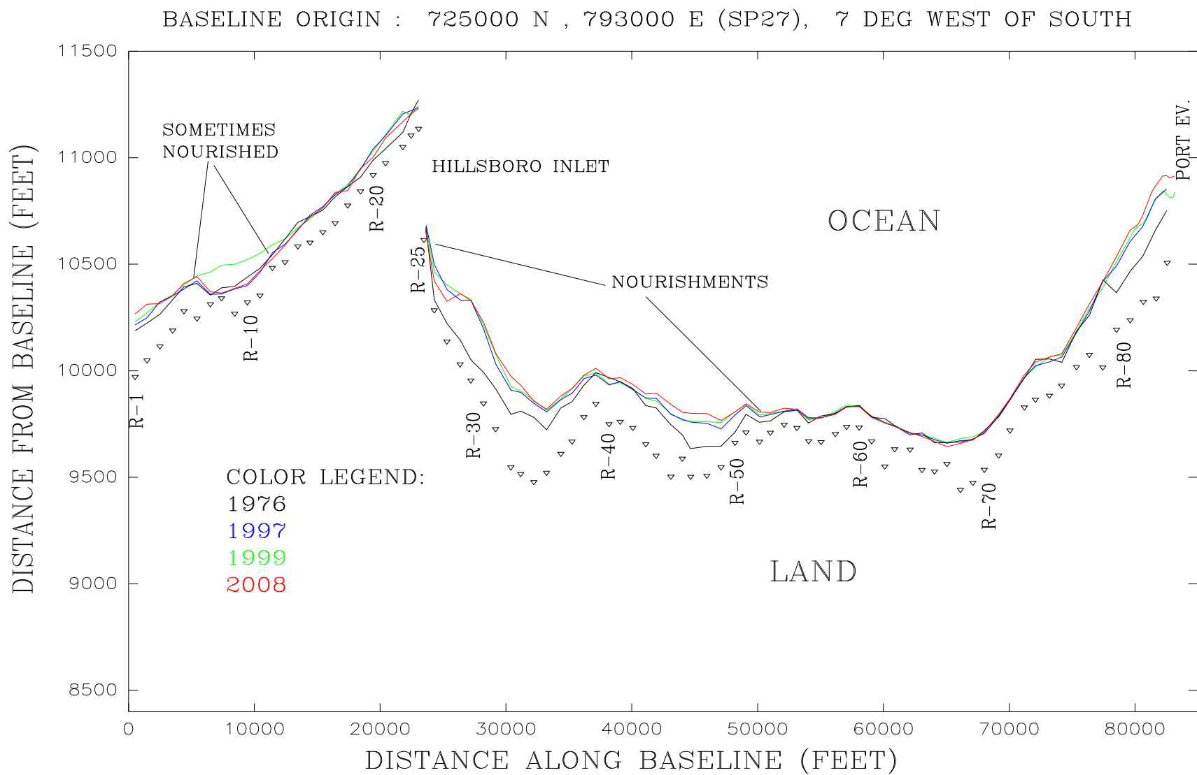
PLAN VIEW MHW SHORELINES – N. BROWARD
