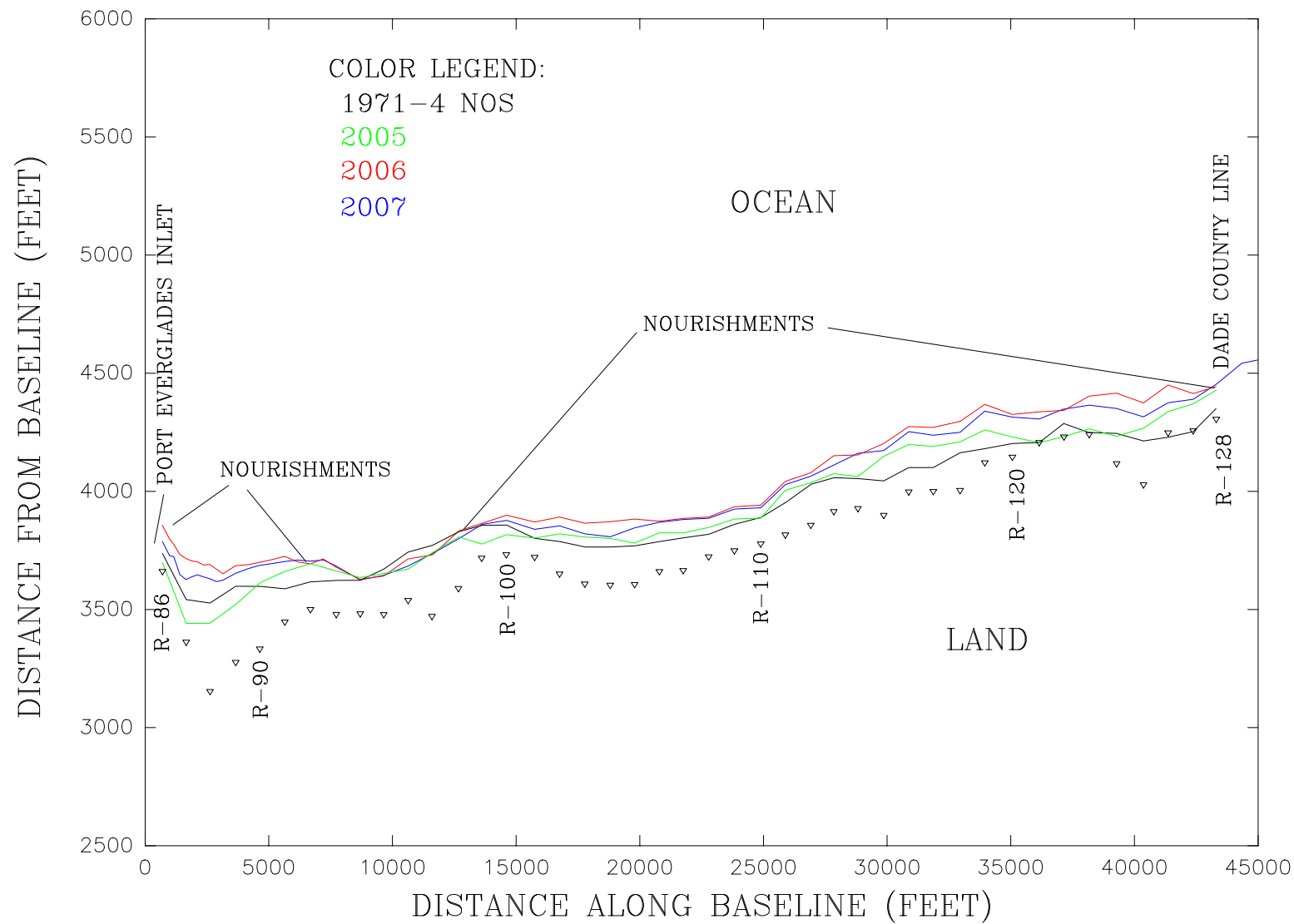
PLAN VIEW MHW SHORELINES – S. BROWARD
