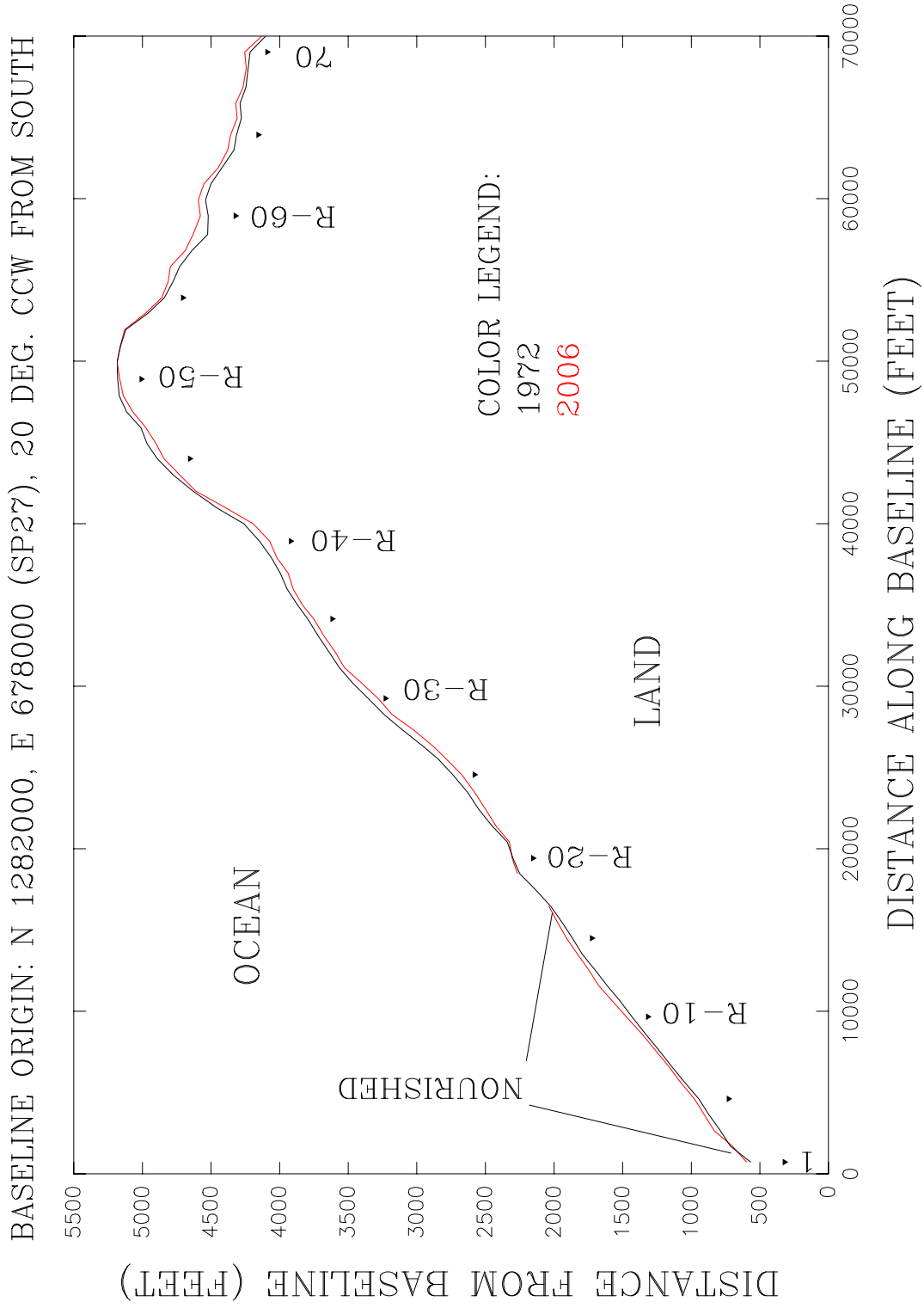
PLAN VIEW MHW SHORELINES - I. RIVER CO.
