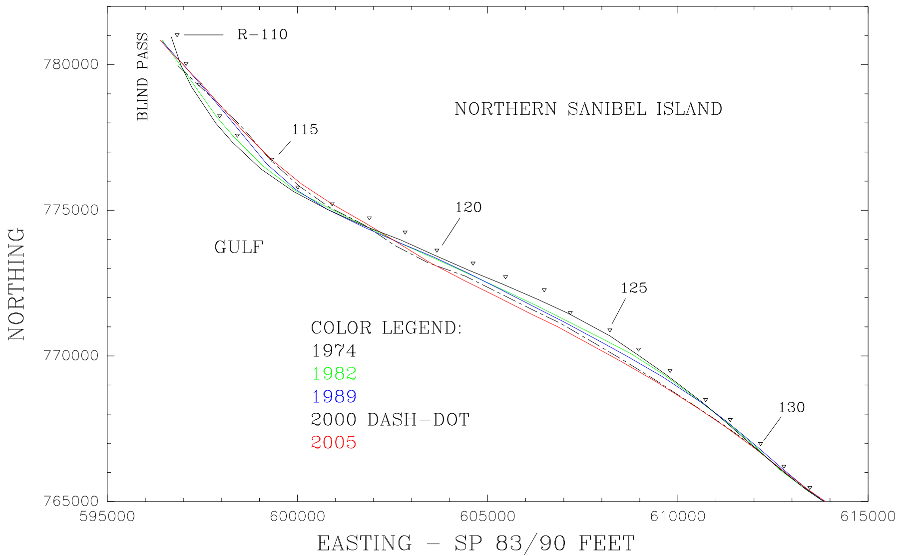
PLAN VIEW MHW SHORELINES - LEE CO., SANIBEL #1
