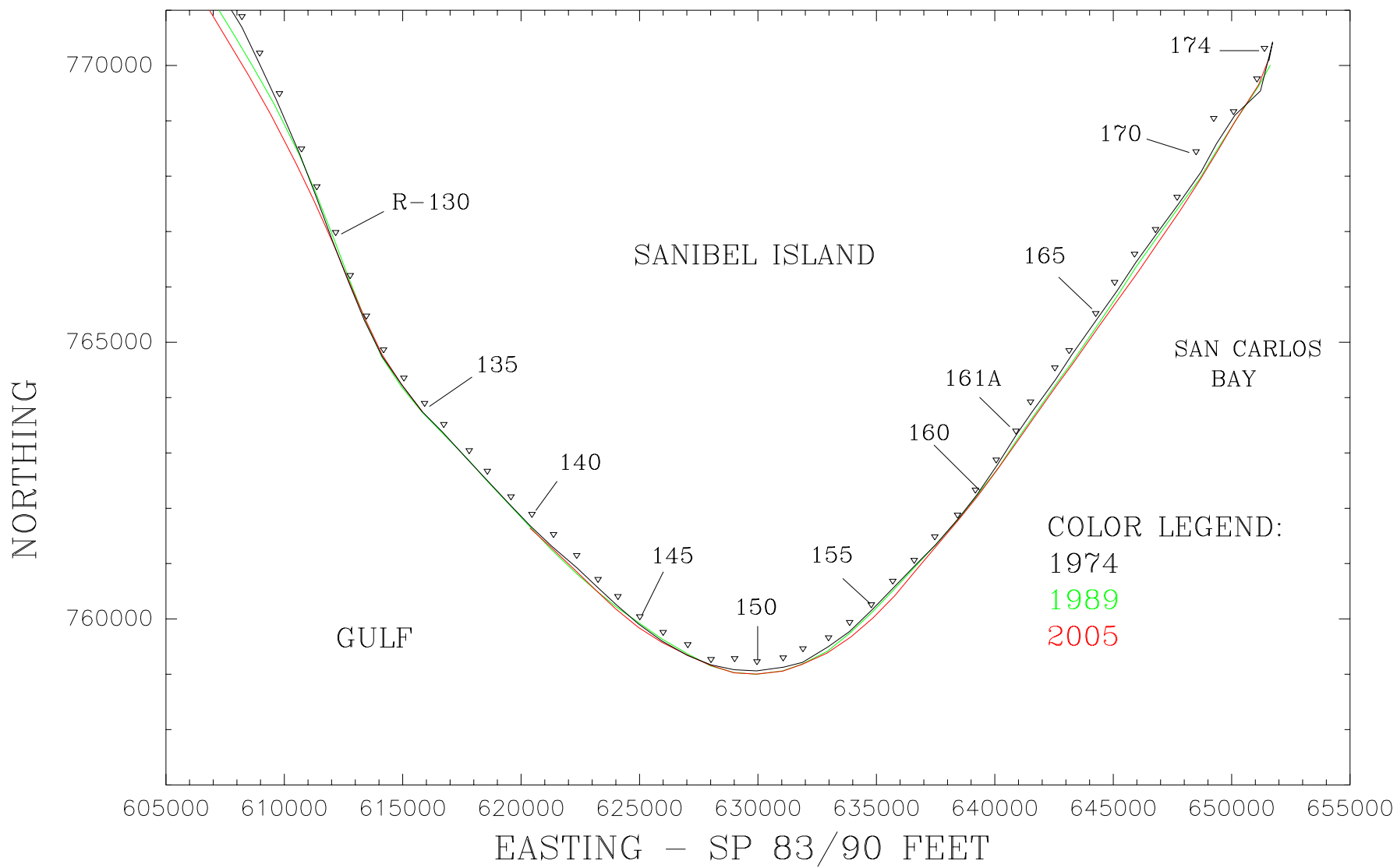
PLAN VIEW MHW SHORELINES - LEE CO., SANIBEL #2
