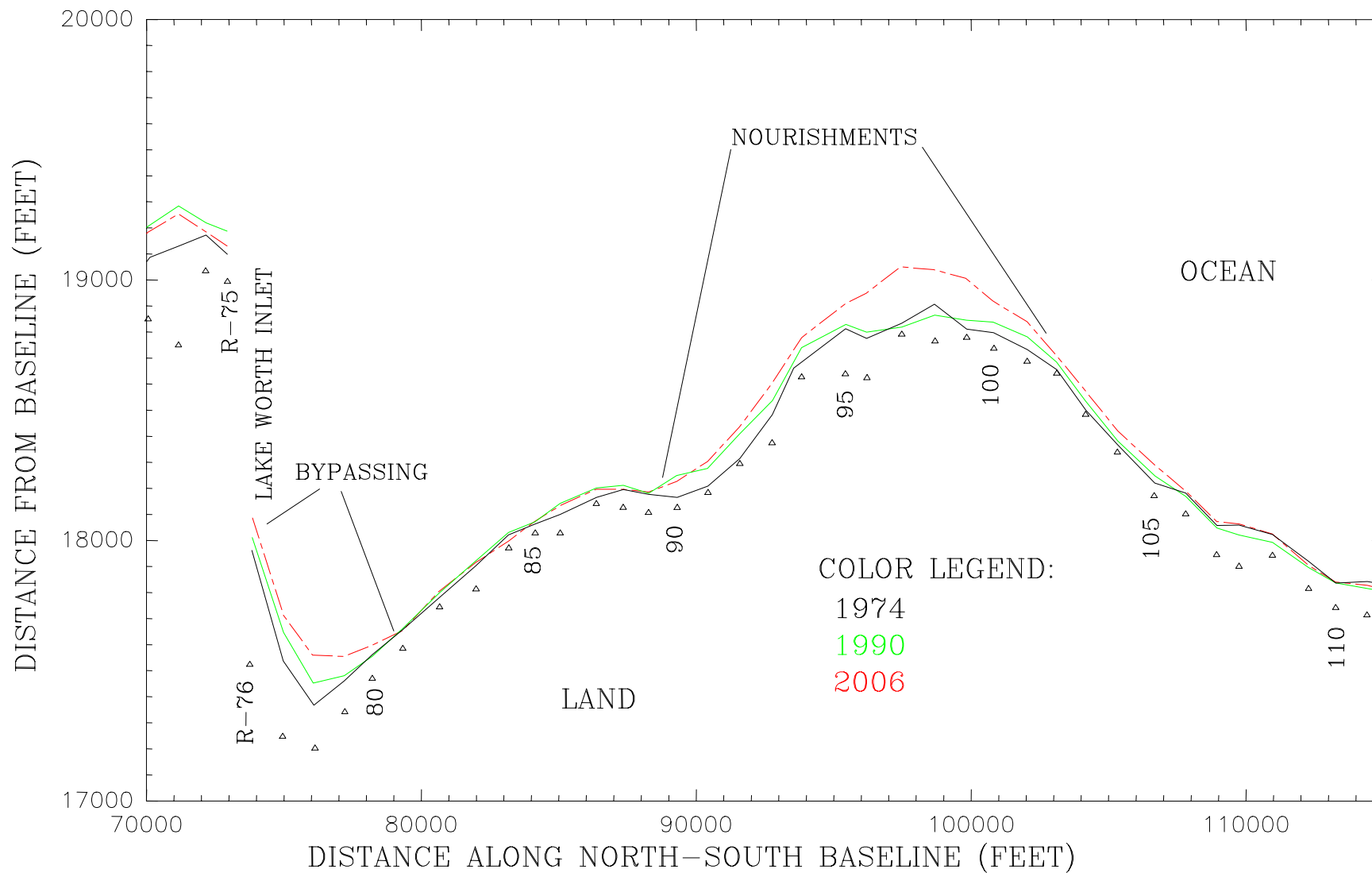
PLAN VIEW MHW SHORELINES – CENTRAL P. BEACH CO. #1
