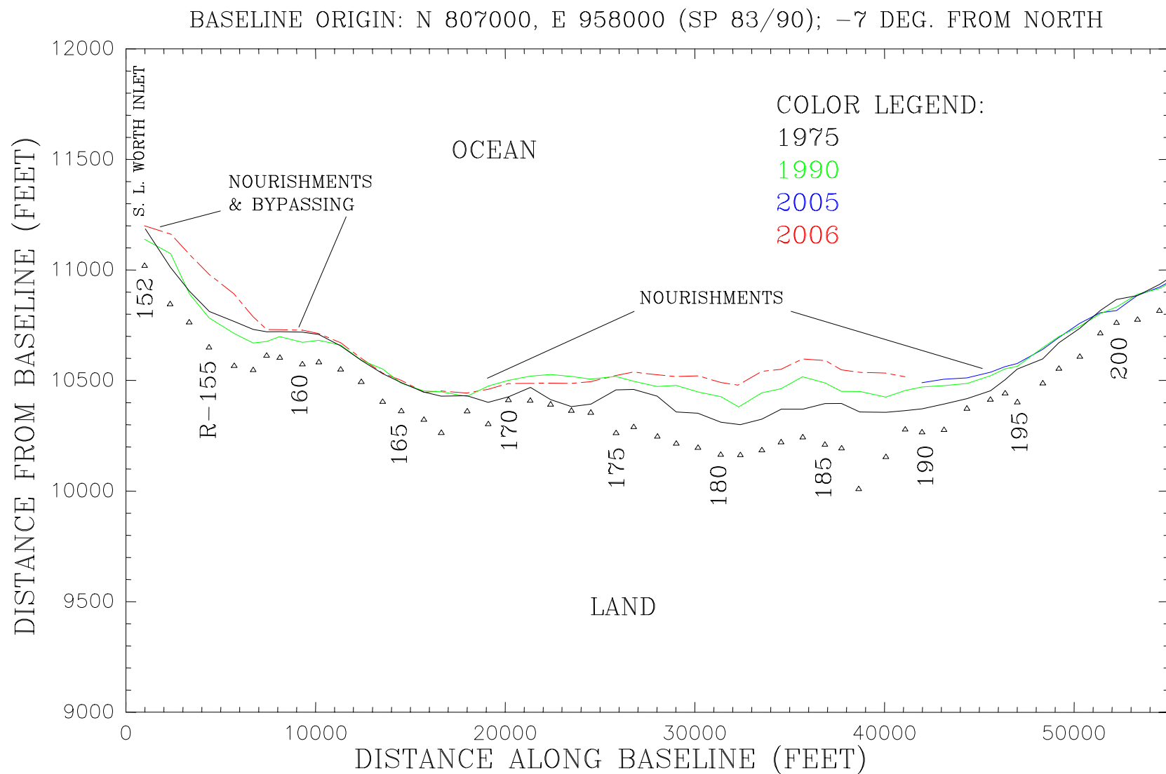
PLAN VIEW MHW SHORELINES – SOUTH P. BEACH CO. #1
