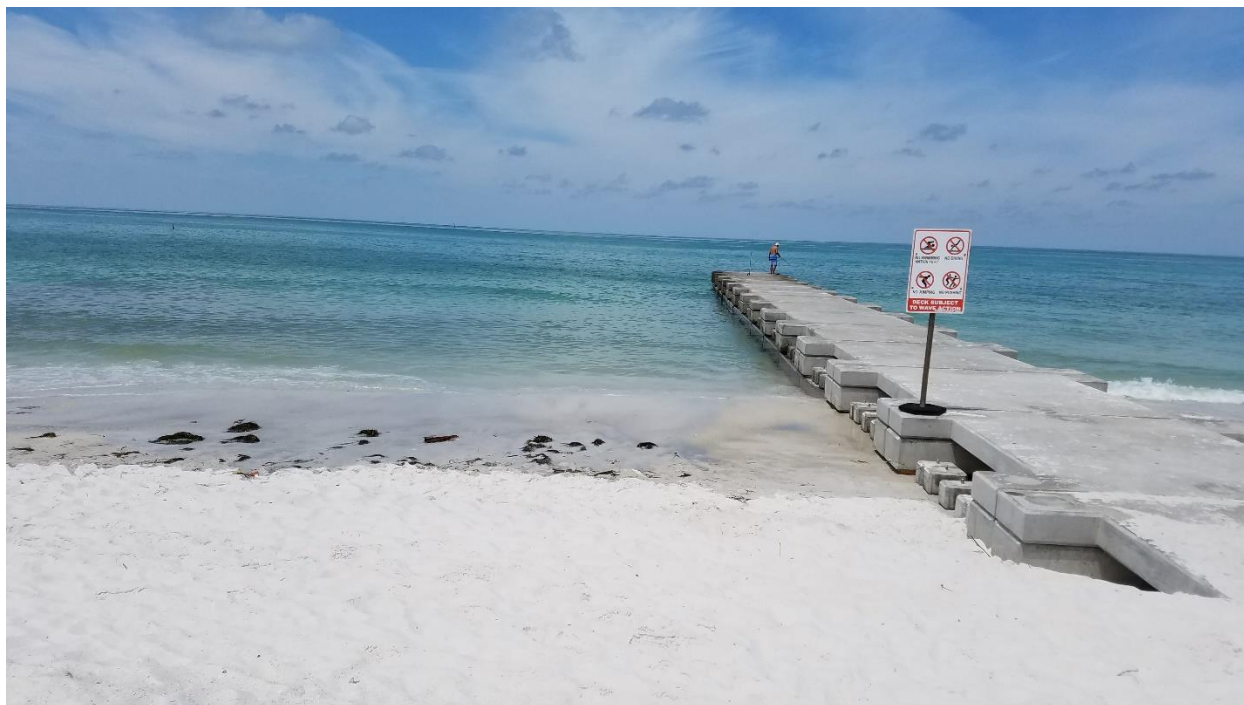
Photo 13: ME R-41 facing seaward (experimental groin structure)
