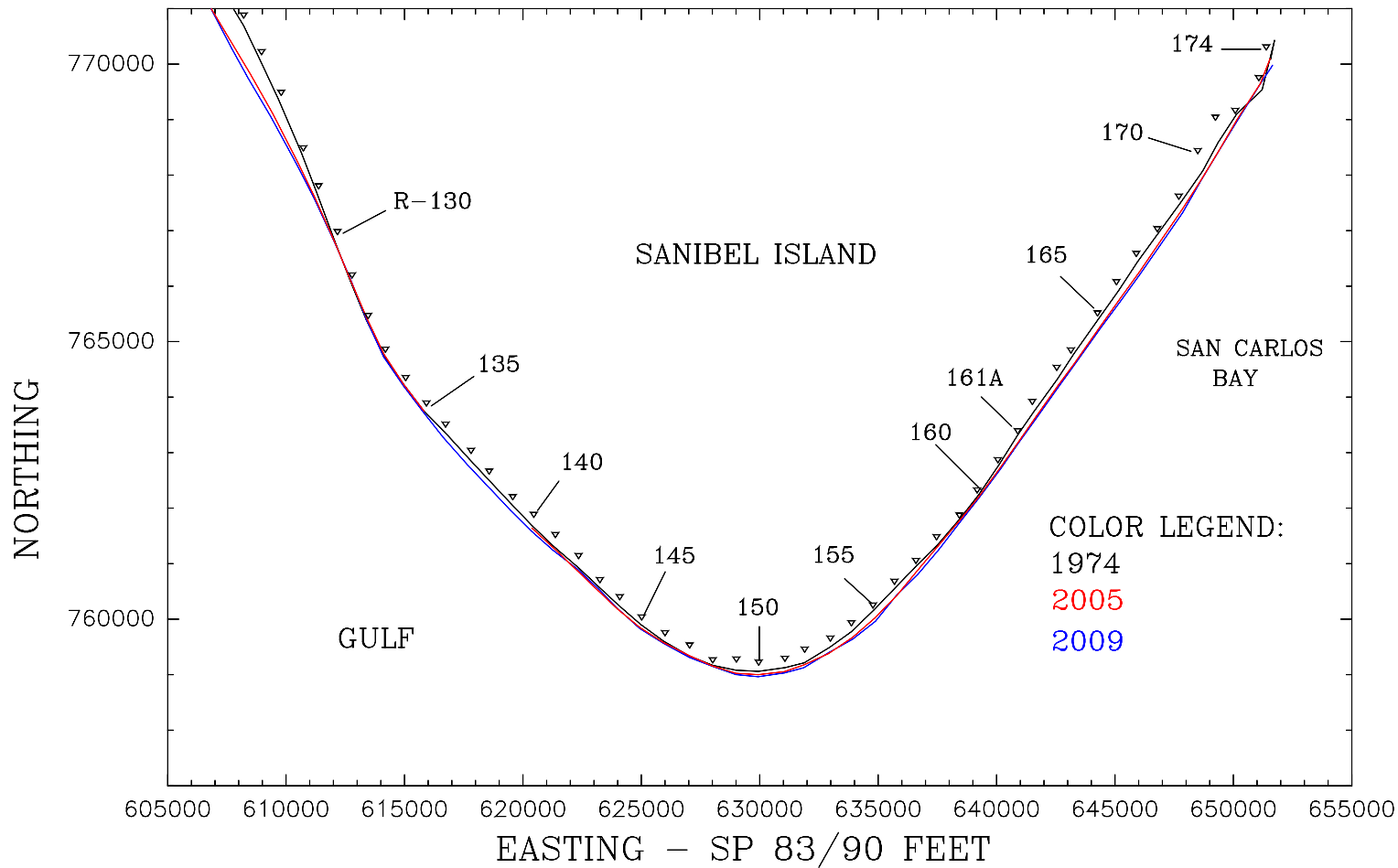
PLAN VIEW MHW SHORELINES - LEE CO., SANIBEL #2
