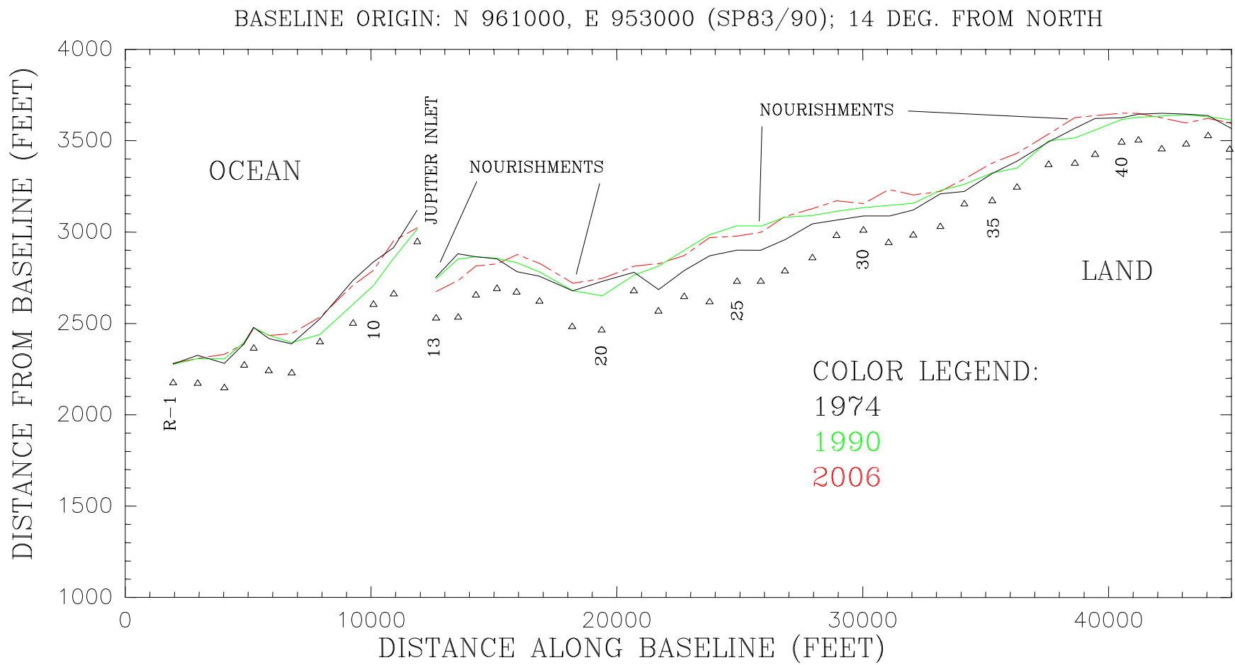
PLAN VIEW MHW SHORELINES – NORTH P. BEACH CO. #1
