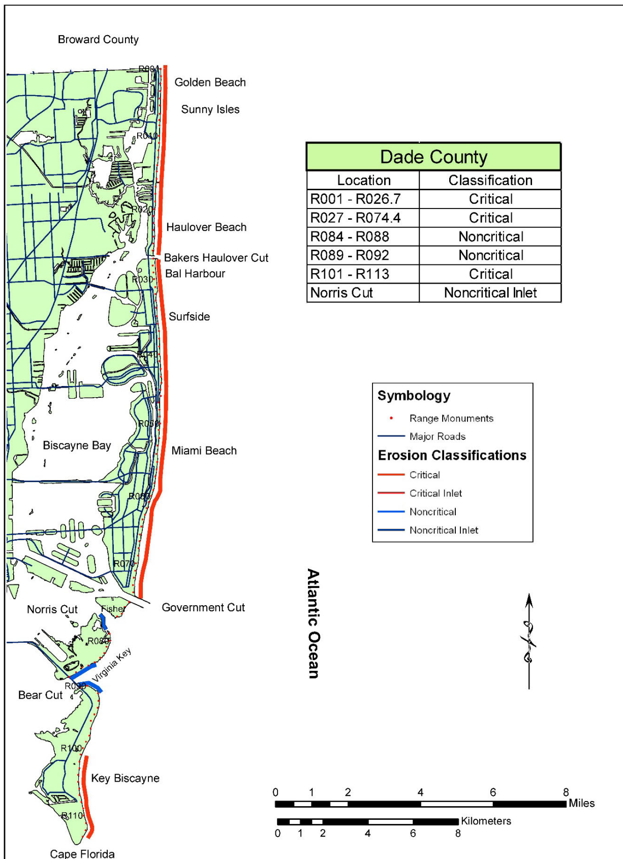
Figure 13. Critically eroded shoreline within Dade County.
