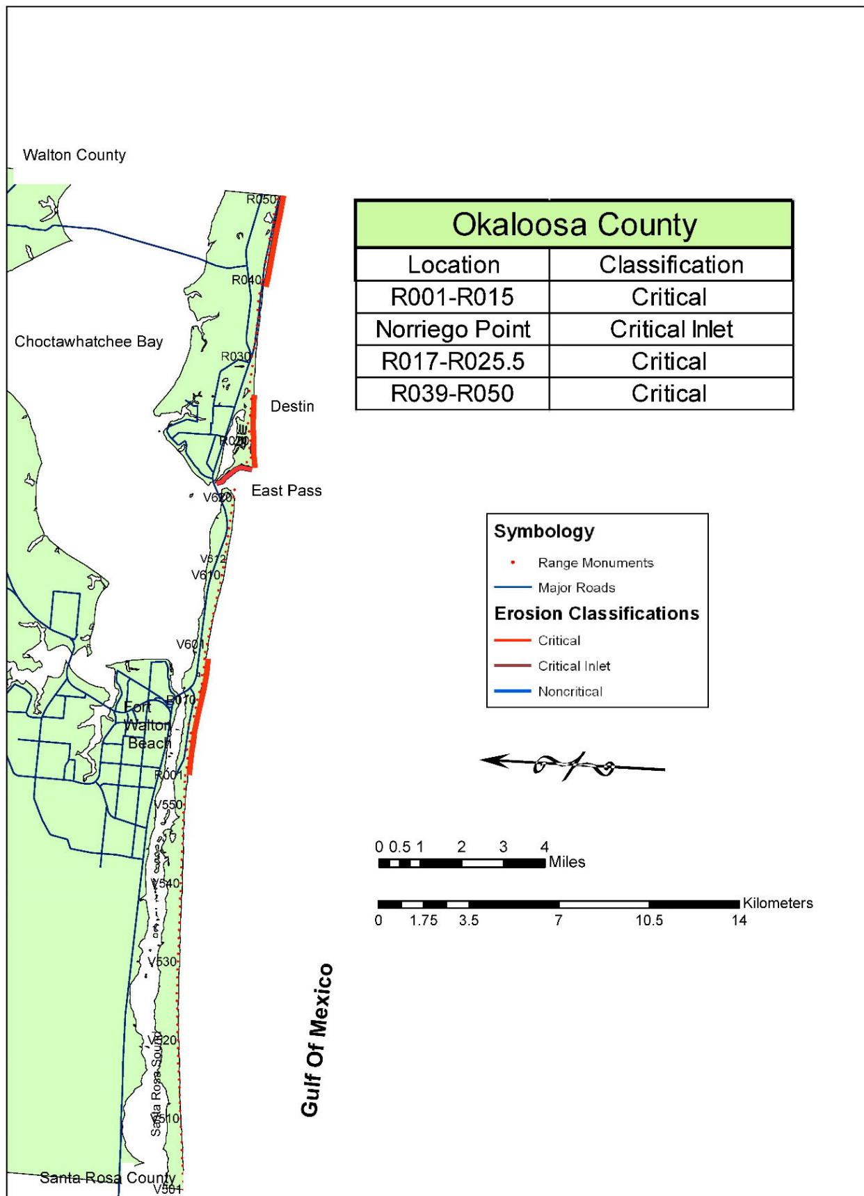
Figure 17. Critically eroded shoreline within Okaloosa County.
