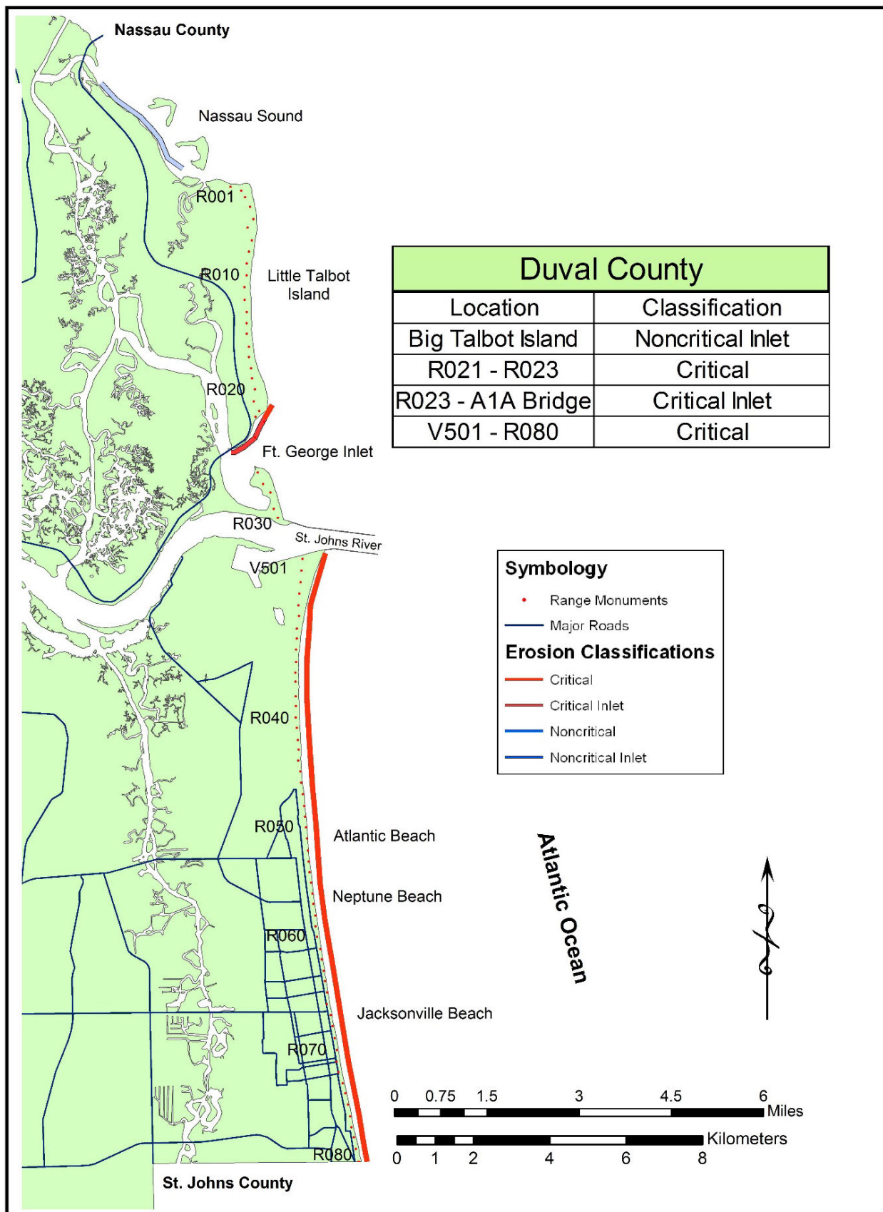
Figure 3. Critically eroded shoreline within Duval County.
