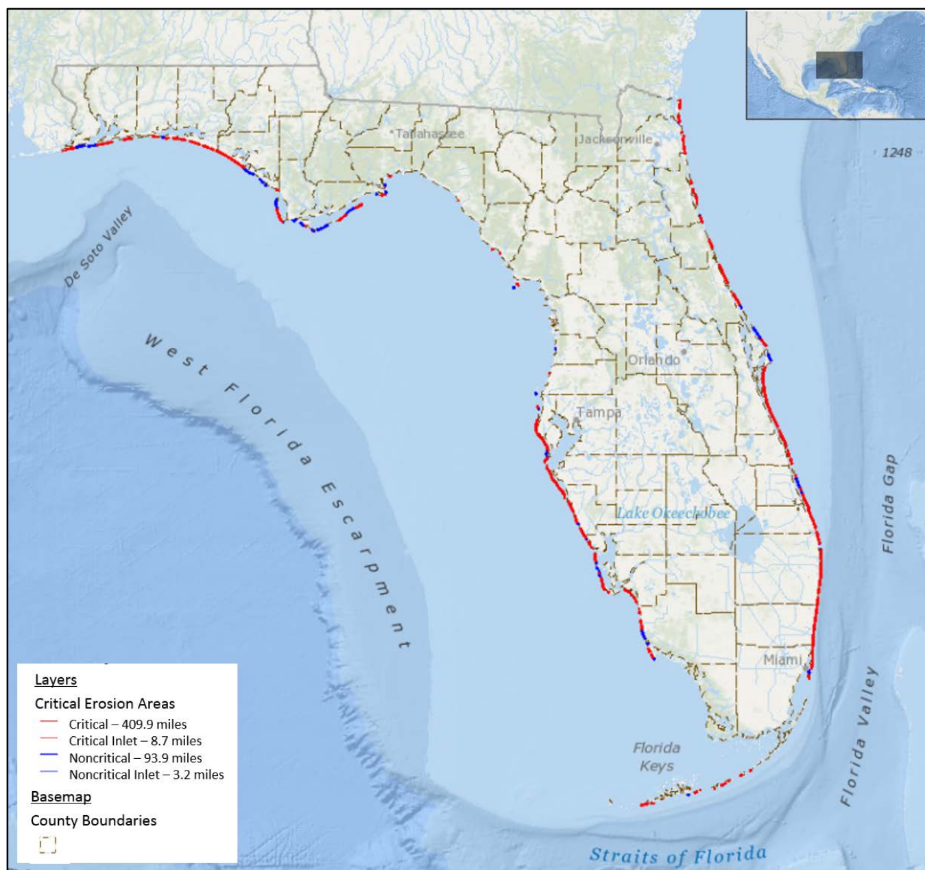
Figure 1. Statewide areas of critically and non-critically eroded shoreline [Graphic from ROSSI database ].
