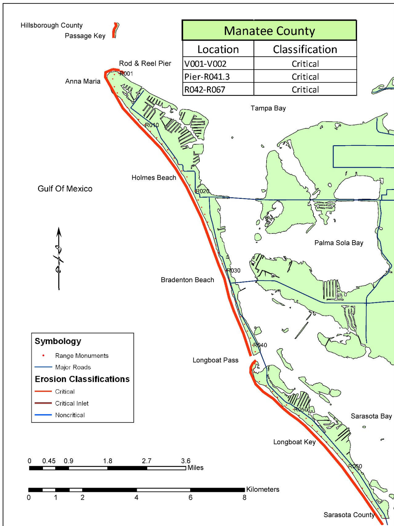
Figure 26. Critically eroded shoreline within Manatee County.
