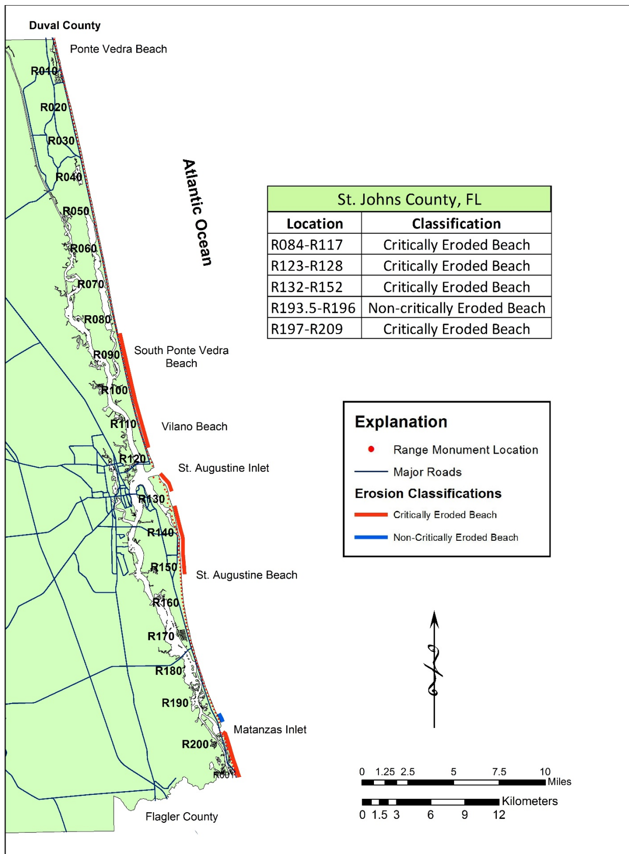
Figure 4. Critically eroded shoreline within St. Johns County.
