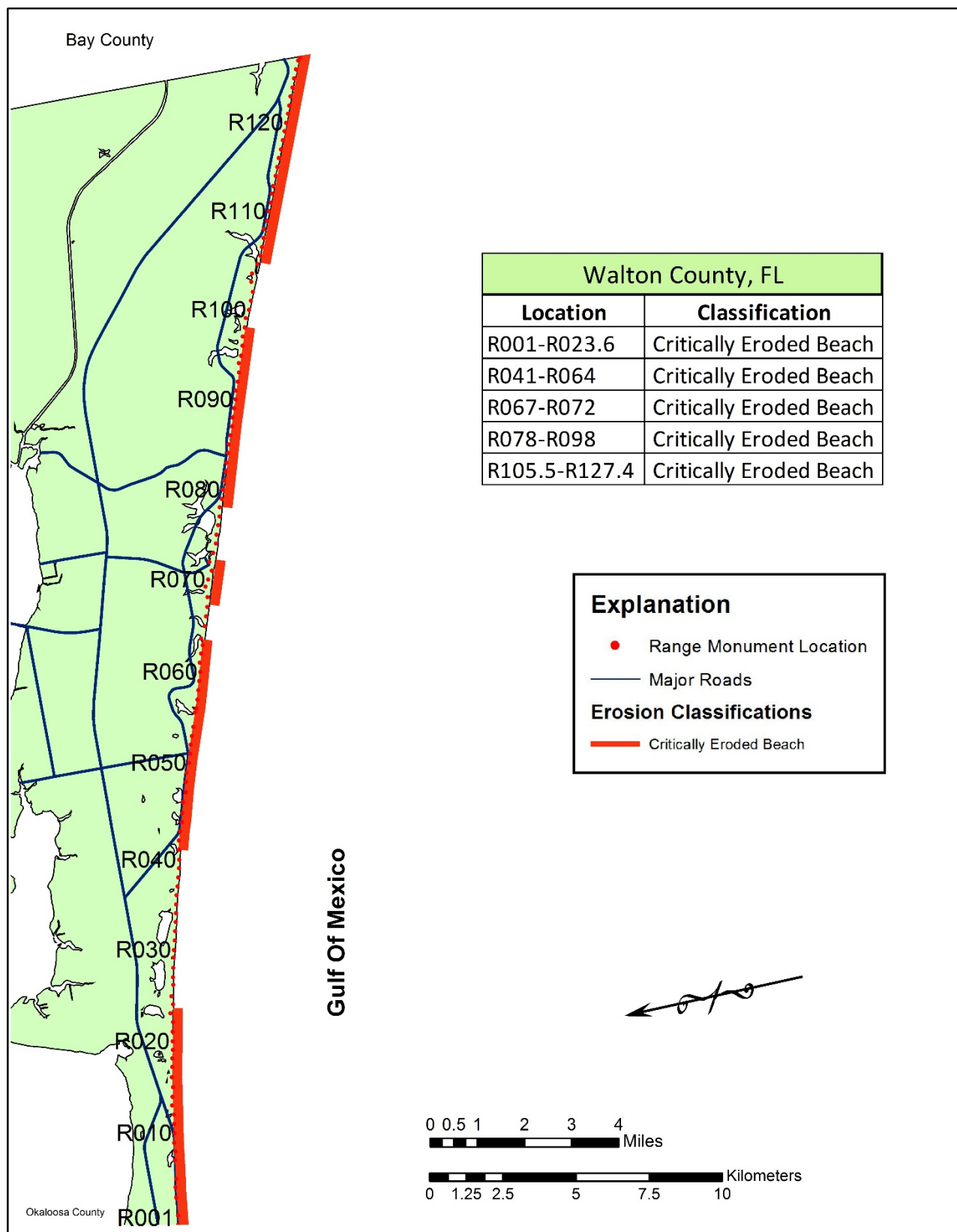
Figure 18. Critically eroded shoreline within Walton County.
