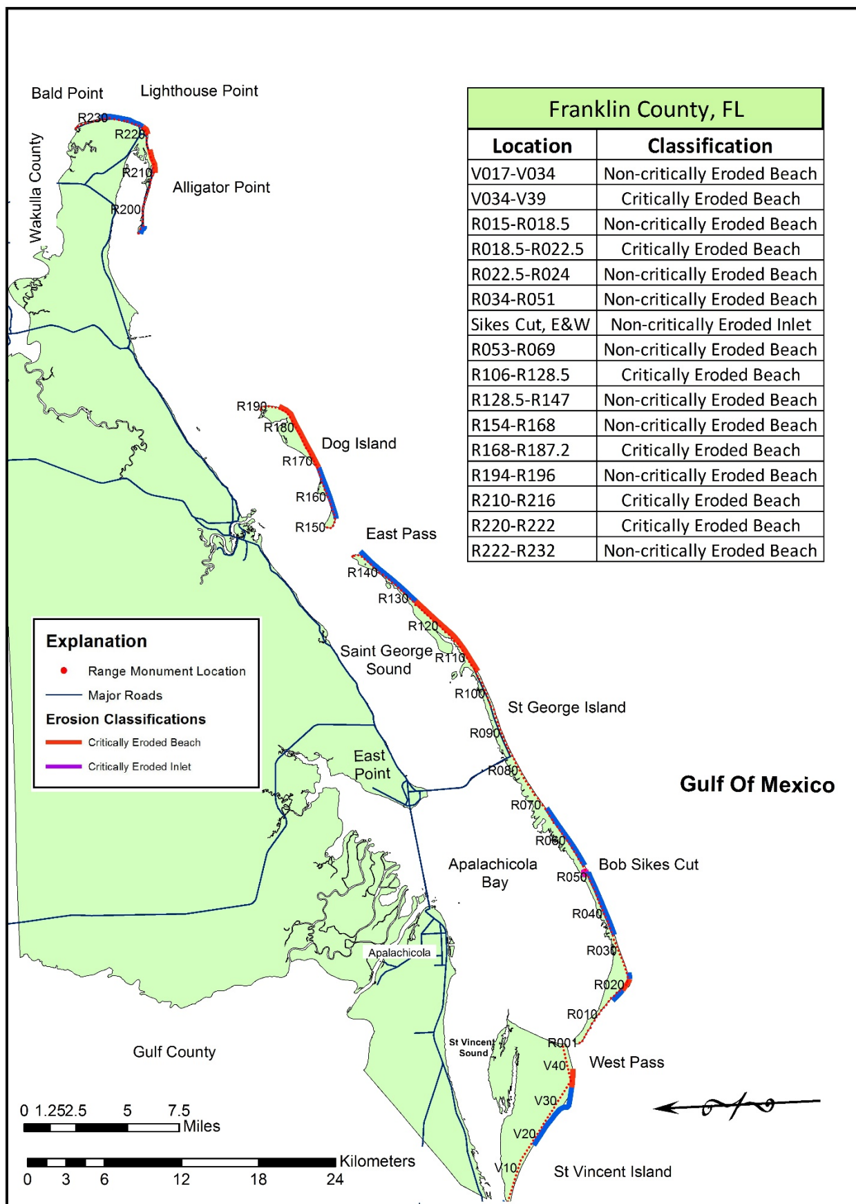
Figure 21. Critically eroded shoreline within Franklin County.
