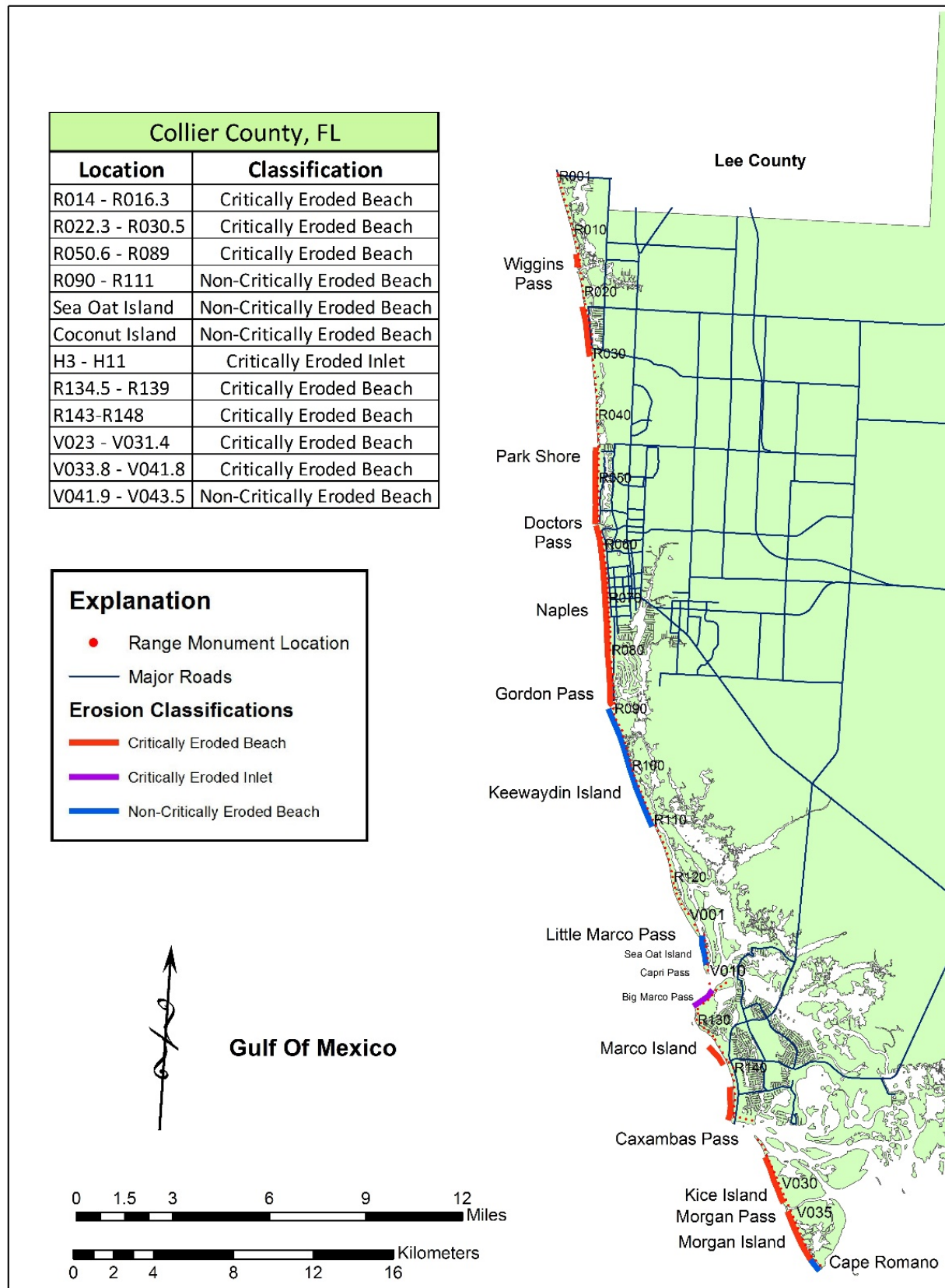
Figure 32. Critically eroded shoreline within Collier County.
